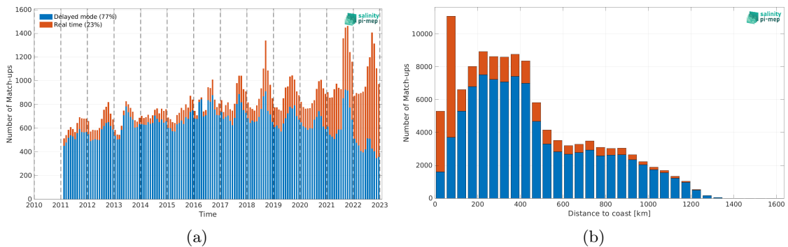
Figure 2: Number of match-ups between Argo and SMOS SSS L3 Arctic v4 - 9 Days (BEC) SSS as a function of time (a) and as function of the distance to coast (b) over the Global Ocean Pi-MEP region and for the full satellite product period.
