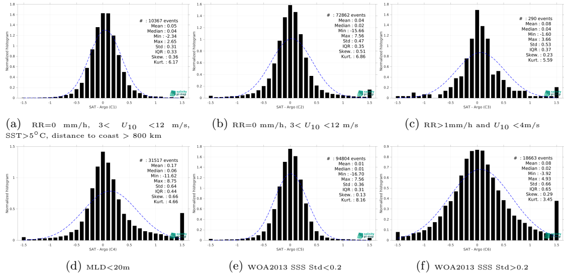
Figure 15: Normalized histogram of \Delta SSS (SMOS SSS L3 Arctic v4 - 9 Days (BEC) - Argo) for 6 different subdatasets corresponding to: RR=0 mm/h, 3 < U_{10} < 12 m/s, SST>5°C, distance to coast > 800 km (a), RR=0 mm/h, 3 < U_{10} < 12 m/s (b), RR>1mm/h and U_{10} < 4 m/s (c), MLD<20m (d), WOA2013 SSS Std<0.2 (e), WOA2013 SSS Std>0.2 (f).
