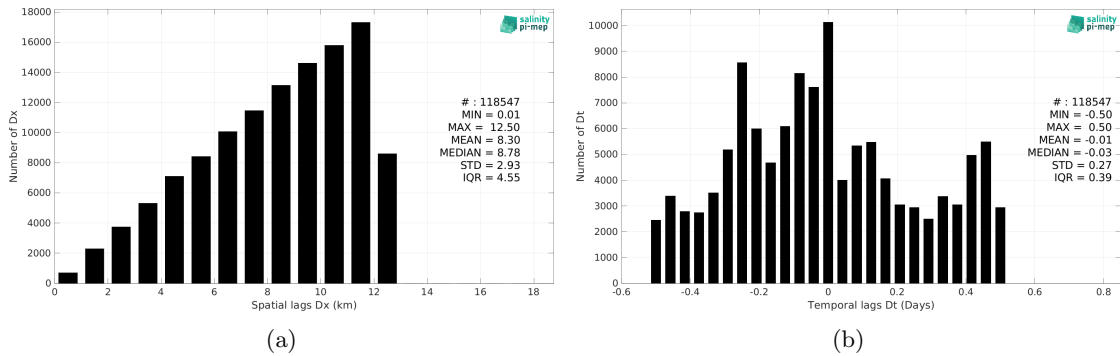
Figure 6: Histograms of the spatial (a) and temporal (b) lags between the location/time of the Argo measurement and the date of the corresponding SMOS SSS L3 Arctic v4 - 9 Days (BEC) SSS pixel.
