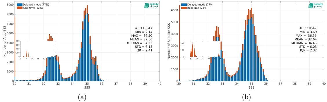
Figure 3: Histograms of SSS from Argo (a) and SMOS SSS L3 Arctic v4 - 9 Days (BEC) (b) considering all match-up pairs per bins of 0.1 over the Global Ocean Pi-MEP region and for the full satellite product period.
