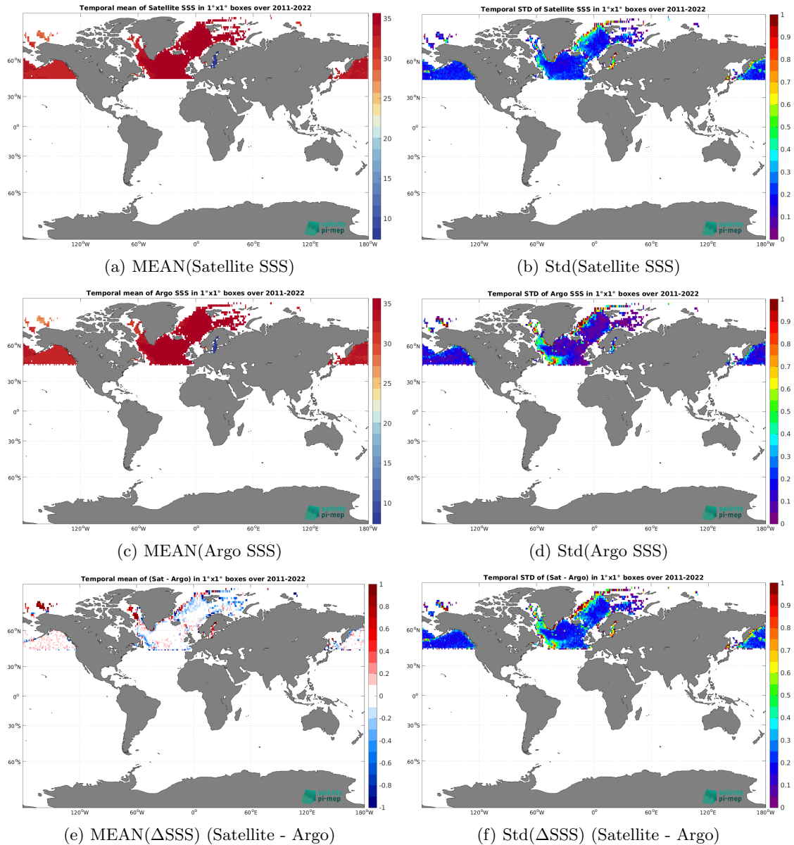
Figure 7: Temporal mean (left) and Std (right) of SSS from SMOS SSS L3 Arctic v4 - 9 Days (BEC) (top), Argo (middle), and of \Delta SSS (Satellite - Argo). Only match-up pairs are used to generate these maps.
