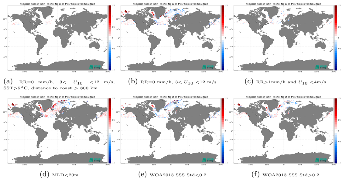
Figure 14: Temporal mean gridded over spatial boxes of size 1^\circ \times 1^\circ of \Delta SSS (SMOS SSS L3 Arctic v4 - 9 Days (BEC) - Argo) for 6 different subdatasets corresponding to:RR=0 mm/h, 3 < U_{10} < 12 m/s, SST >5^\circ C, distance to coast > 800 km (a), RR=0 mm/h, 3 < U_{10} < 12 m/s (b), RR >1 mm/h and U_{10} < 4 m/s (c),MLD <20 m (d),WOA2013 SSS Std <0.2 (e),WOA2013 SSS Std >0.2 (f).
