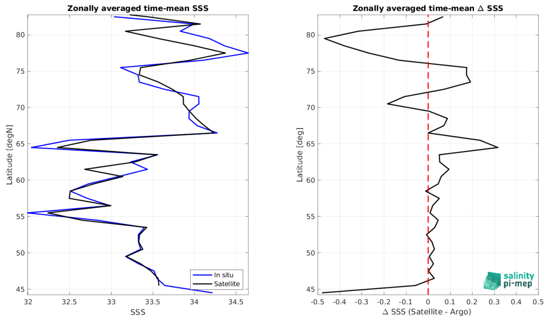
Figure 9: Left panel: Zonal mean SSS from SMOS SSS L3 Arctic v4 - 9 Days (BEC) satellite product (black) and from Argo (blue). Right panel: Zonal mean of \Delta SSS (Satellite - Argo) for all the collected Pi-MEP match-up pairs estimated over the full satellite product period.
