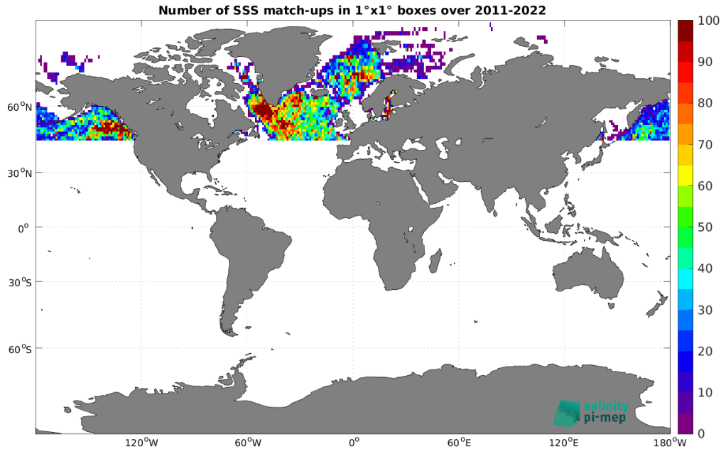
Figure 5: Number of SSS match-ups between Argo SSS and the SMOS SSS L3 Arctic v4 - 9 Days (BEC) SSS product for the Global Ocean Pi-MEP region over 1^\circ \times 1^\circ boxes and for the full satellite product period.
