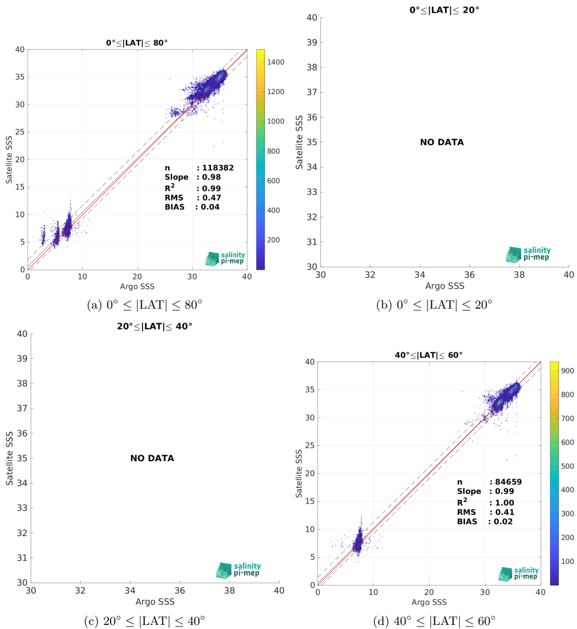
Figure 10: Contour maps of the concentration of SMOS SSS L3 Arctic v4 - 9 Days (BEC) SSS (y-axis) versus Argo SSS (x-axis) at match-up pairs for different latitude bands. For each plot, the red line shows x=y . The black thin and dashed lines indicate a linear fit through the data cloud and the \pm 95\% confidence levels, respectively. The number match-up pairs n , the slope and R^2 coefficient of the linear fit, the root mean square (RMS) and the mean bias between satellite and in situ data are indicated for each latitude band in each plots.
