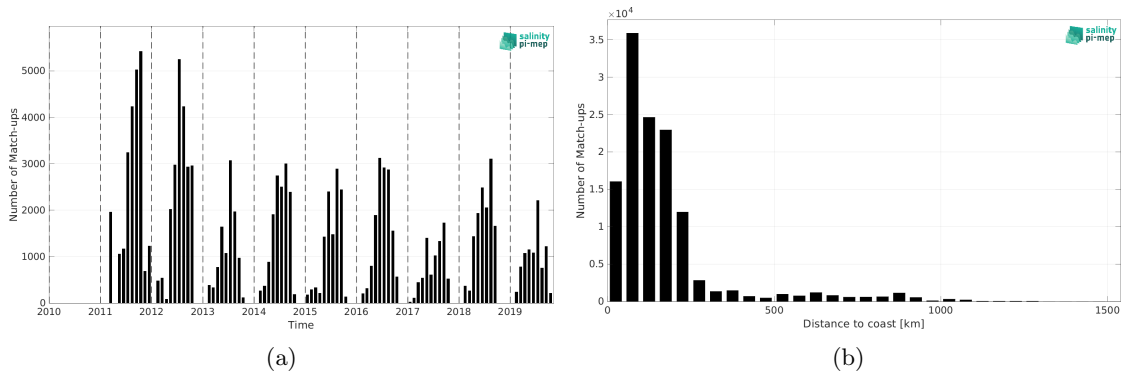
Figure 1: Number of match-ups between TSG (SAMOS) and SMOS SSS L3 Arctic v3.1 - 9 Days (BEC) SSS as a function of time (a) and as function of the distance to coast (b) over the Global Ocean Pi-MEP region and for the full satellite product period.
