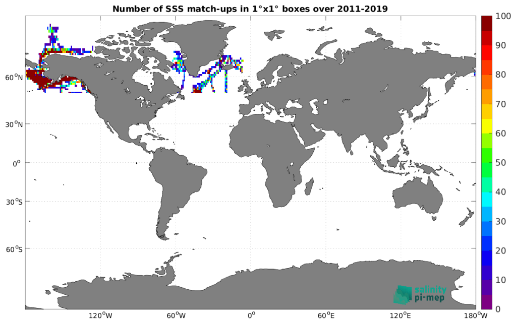
Figure 4: Number of SSS match-ups between TSG (SAMOS) SSS and the SMOS SSS L3 Arctic v3.1 - 9 Days (BEC) SSS product for the Global Ocean Pi-MEP region over 1^\circ \times 1^\circ boxes and for the full satellite product period.
