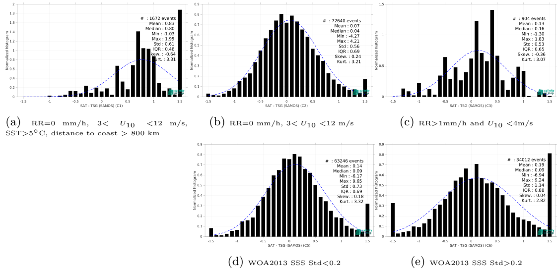
Figure 13: Normalized histogram of \Delta SSS (SMOS SSS L3 Arctic v3.1 - 9 Days (BEC) - TSG (SAMOS)) for 5 different subdatasets corresponding to: RR=0 mm/h, 3 < U_{10} < 12 m/s, SST > 5°C, distance to coast > 800 km (a), RR=0 mm/h, 3 < U_{10} < 12 m/s (b), RR > 1mm/h and U_{10} < 4 m/s (c), WOA2013 SSS Std < 0.2 (d), WOA2013 SSS Std > 0.2 (e).
