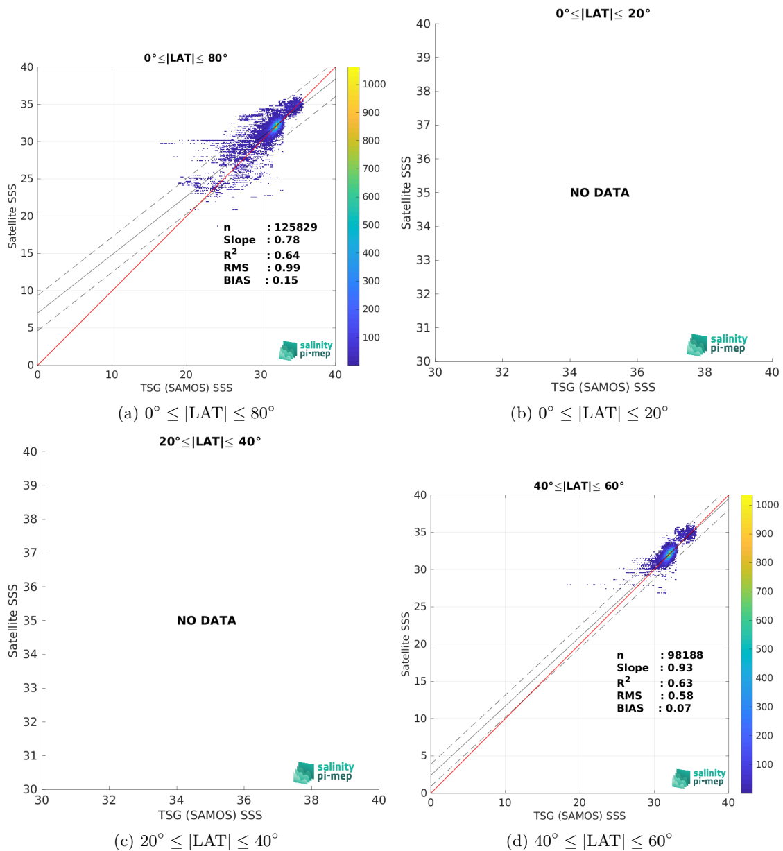
Figure 9: Contour maps of the concentration of SMOS SSS L3 Arctic v3.1 - 9 Days (BEC) SSS (y-axis) versus TSG (SAMOS) SSS (x-axis) at match-up pairs for different latitude bands. For each plot, the red line shows x=y . The black thin and dashed lines indicate a linear fit through the data cloud and the \pm 95\% confidence levels, respectively. The number match-up pairs n , the slope and R^2 coefficient of the linear fit, the root mean square (RMS) and the mean bias between satellite and in situ data are indicated for each latitude band in each plots.
