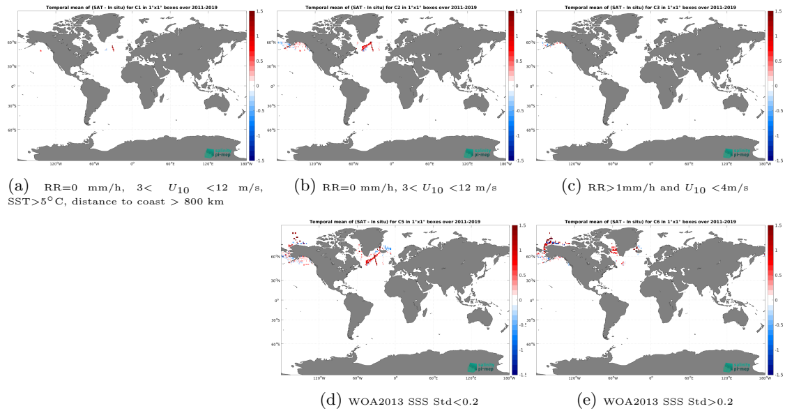
Figure 12: Temporal mean gridded over spatial boxes of size 1^{\circ}\times 1^{\circ} of \Delta\text{SSS} (SMOS SSS L3 Arctic v3.1 - 9 Days (BEC) - TSG (SAMOS)) for 5 different subdatasets corresponding to:RR=0 mm/h, 3 < U_{10} < 12 m/s, SST >5^{\circ}\text{C} , distance to coast > 800 km (a), RR=0 mm/h, 3 < U_{10} < 12 m/s (b), RR >1 mm/h and U_{10} < 4 m/s (c), WOA2013 SSS Std <0.2 (d), WOA2013 SSS Std >0.2 (e).
