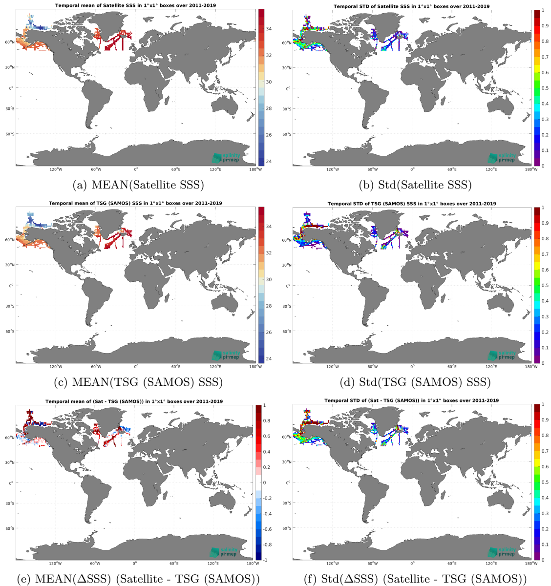
Figure 6: Temporal mean (left) and Std (right) of SSS from SMOS SSS L3 Arctic v3.1 - 9 Days (BEC) (top), TSG (SAMOS) (middle), and of \Delta SSS (Satellite - TSG (SAMOS)). Only match-up pairs are used to generate these maps.
