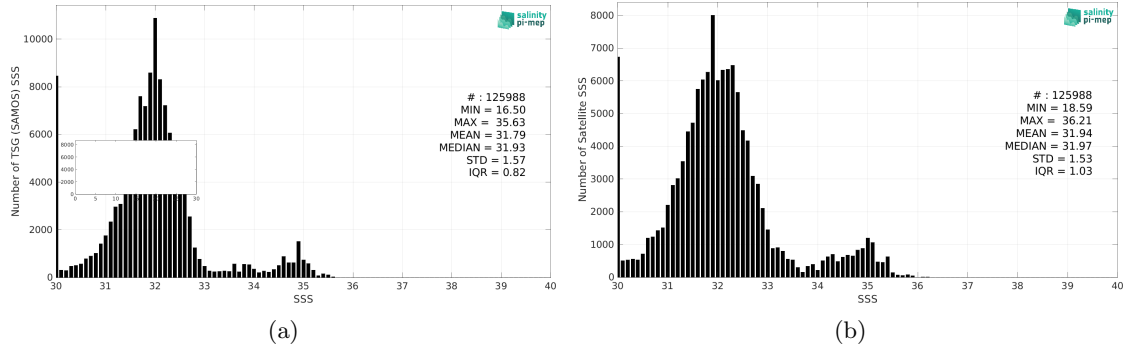
Figure 2: Histograms of SSS from TSG (SAMOS) (a) and SMOS SSS L3 Arctic v3.1 - 9 Days (BEC) (b) considering all match-up pairs per bins of 0.1 over the Global Ocean Pi-MEP region and for the full satellite product period.
