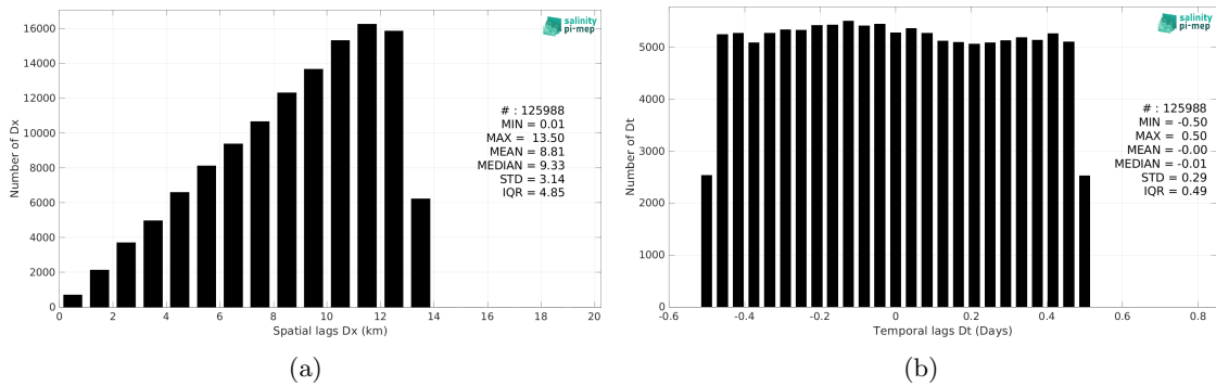
Figure 5: Histograms of the spatial (a) and temporal (b) lags between the location/time of the TSG (SAMOS) measurement and the date of the corresponding SMOS SSS L3 Arctic v3.1 - 9 Days (BEC) SSS pixel.
