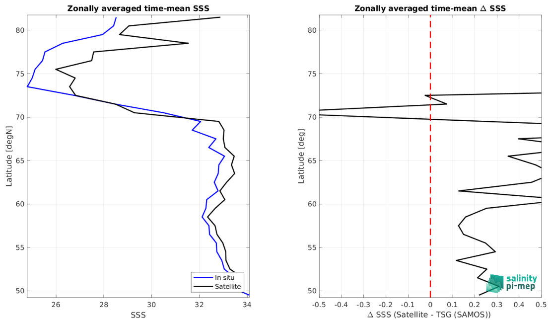
Figure 8: Left panel: Zonal mean SSS from SMOS SSS L3 Arctic v3.1 - 9 Days (BEC) satellite product (black) and from TSG (SAMOS) (blue). Right panel: Zonal mean of \Delta SSS (Satellite - TSG (SAMOS)) for all the collected Pi-MEP match-up pairs estimated over the full satellite product period.
