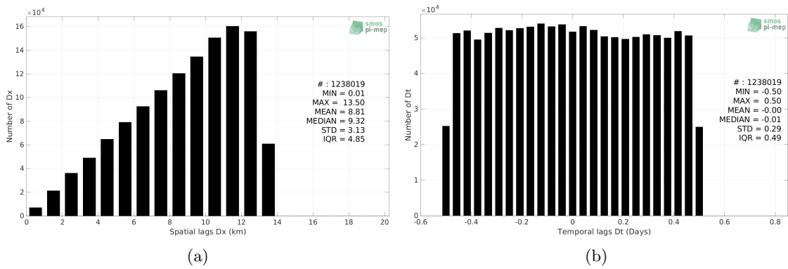
Figure 5: Histograms of the spatial (a) and temporal (b) lags between the location/time of the TSG (SAMOS) measurement and the date of the corresponding SMOS SSS L3 Arctic v3.1 - 9 Days (BEC) SSS pixel.
