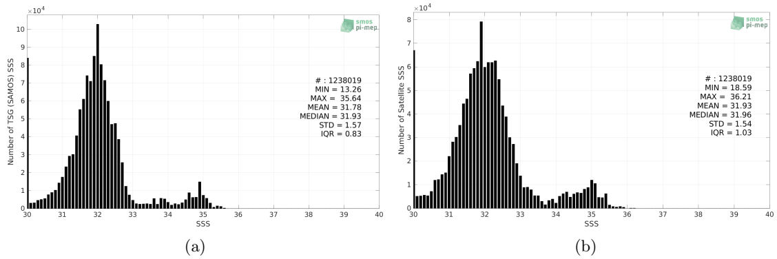
Figure 2: Histograms of SSS from TSG (SAMOS) (a) and SMOS SSS L3 Arctic v3.1 - 9 Days (BEC) (b) considering all match-up pairs per bins of 0.1 over the Global Ocean Pi-MEP region and for the full satellite product period.
