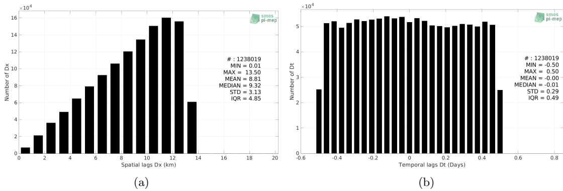
Figure 5: Histograms of the spatial (a) and temporal (b) lags between the location/time of the TSG (SAMOS) measurement and the date of the corresponding SMOS SSS L3 Arctic v3.1 - 9 Days (BEC) SSS pixel.
