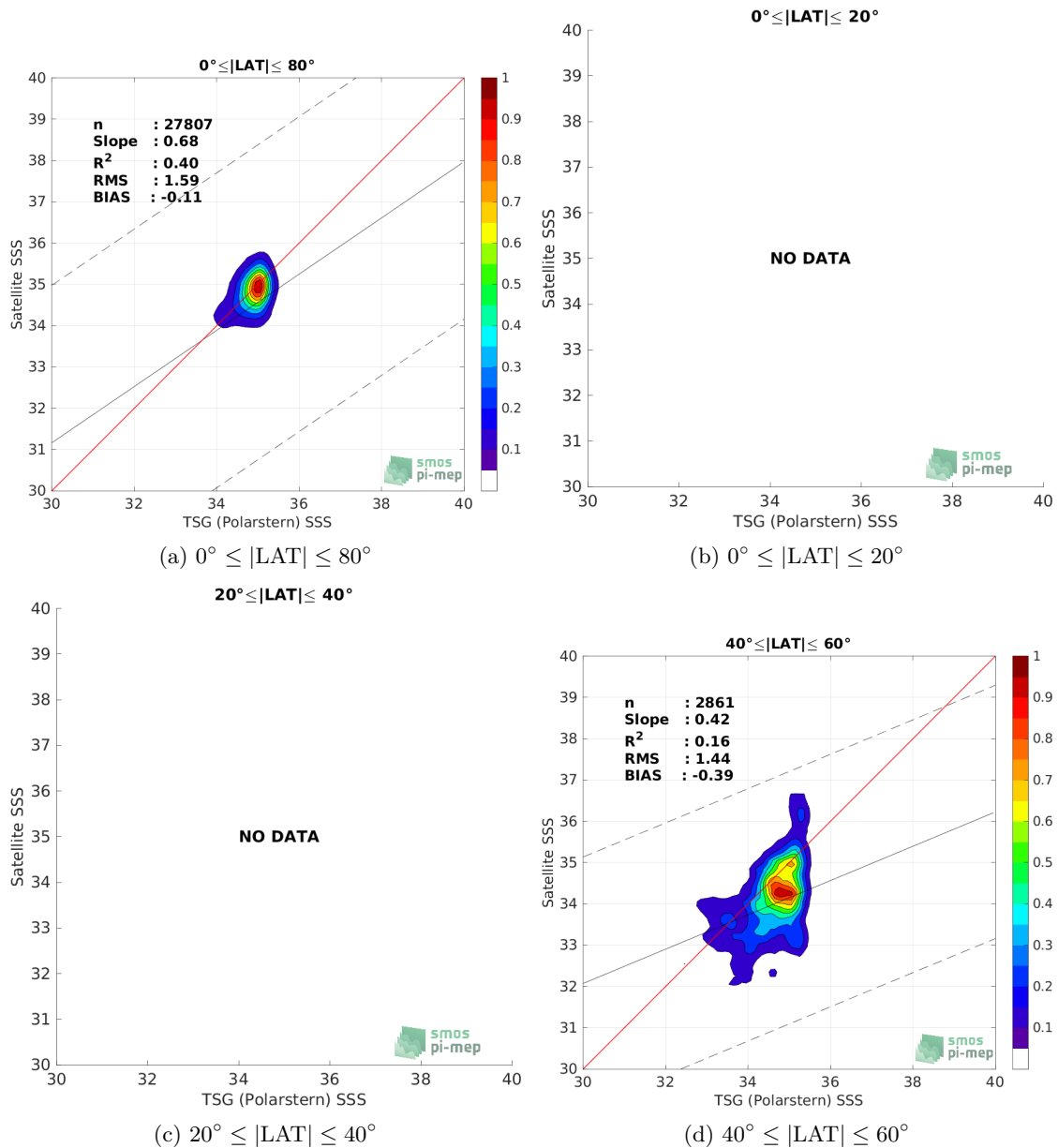
Figure 9: Contour maps of the concentration of SMOS SSS L3 Arctic v3.1 - 9 Days (BEC) SSS (y-axis) versus TSG (Polarstern) SSS (x-axis) at match-up pairs for different latitude bands. For each plot, the red line shows x=y . The black thin and dashed lines indicate a linear fit through the data cloud and the \pm 95\% confidence levels, respectively. The number match-up pairs n , the slope and R^2 coefficient of the linear fit, the root mean square (RMS) and the mean bias between satellite and in situ data are indicated for each latitude band in each plots.
