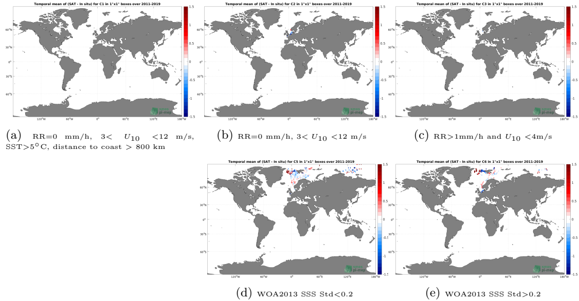
Figure 12: Temporal mean gridded over spatial boxes of size 1^{\circ}\times 1^{\circ} of \Delta\text{SSS} (SMOS SSS L3 Arctic v3.1 - 9 Days (BEC) - TSG (Polarstern)) for 5 different subdatasets corresponding to:RR=0 mm/h, 3 < U_{10} < 12 m/s, SST >5^{\circ}\text{C} , distance to coast > 800 km (a), RR=0 mm/h, 3 < U_{10} < 12 m/s (b), RR >1 mm/h and U_{10} < 4 m/s (c), WOA2013 SSS Std <0.2 (d), WOA2013 SSS Std >0.2 (e).
