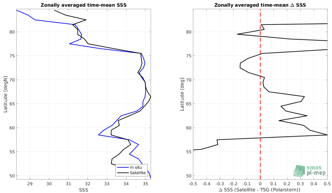
Figure 8: Left panel: Zonal mean SSS from SMOS SSS L3 Arctic v3.1 - 9 Days (BEC) satellite product (black) and from TSG (Polarstern) (blue). Right panel: Zonal mean of \Delta SSS (Satellite - TSG (Polarstern)) for all the collected Pi-MEP match-up pairs estimated over the full satellite product period.
