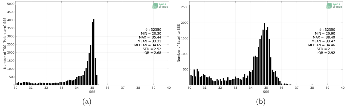
Figure 2: Histograms of SSS from TSG (Polarstern) (a) and SMOS SSS L3 Arctic v3.1 - 9 Days (BEC) (b) considering all match-up pairs per bins of 0.1 over the Global Ocean Pi-MEP region and for the full satellite product period.
