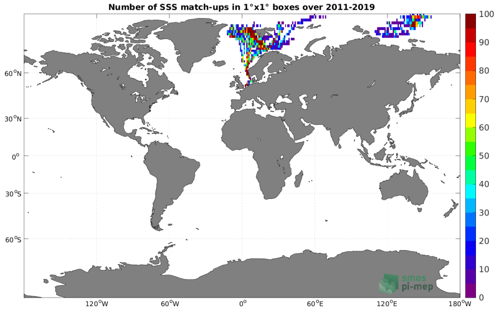
Figure 4: Number of SSS match-ups between TSG (Polarstern) SSS and the SMOS SSS L3 Arctic v3.1 - 9 Days (BEC) SSS product for the Global Ocean Pi-MEP region over 1^\circ \times 1^\circ boxes and for the full satellite product period.
