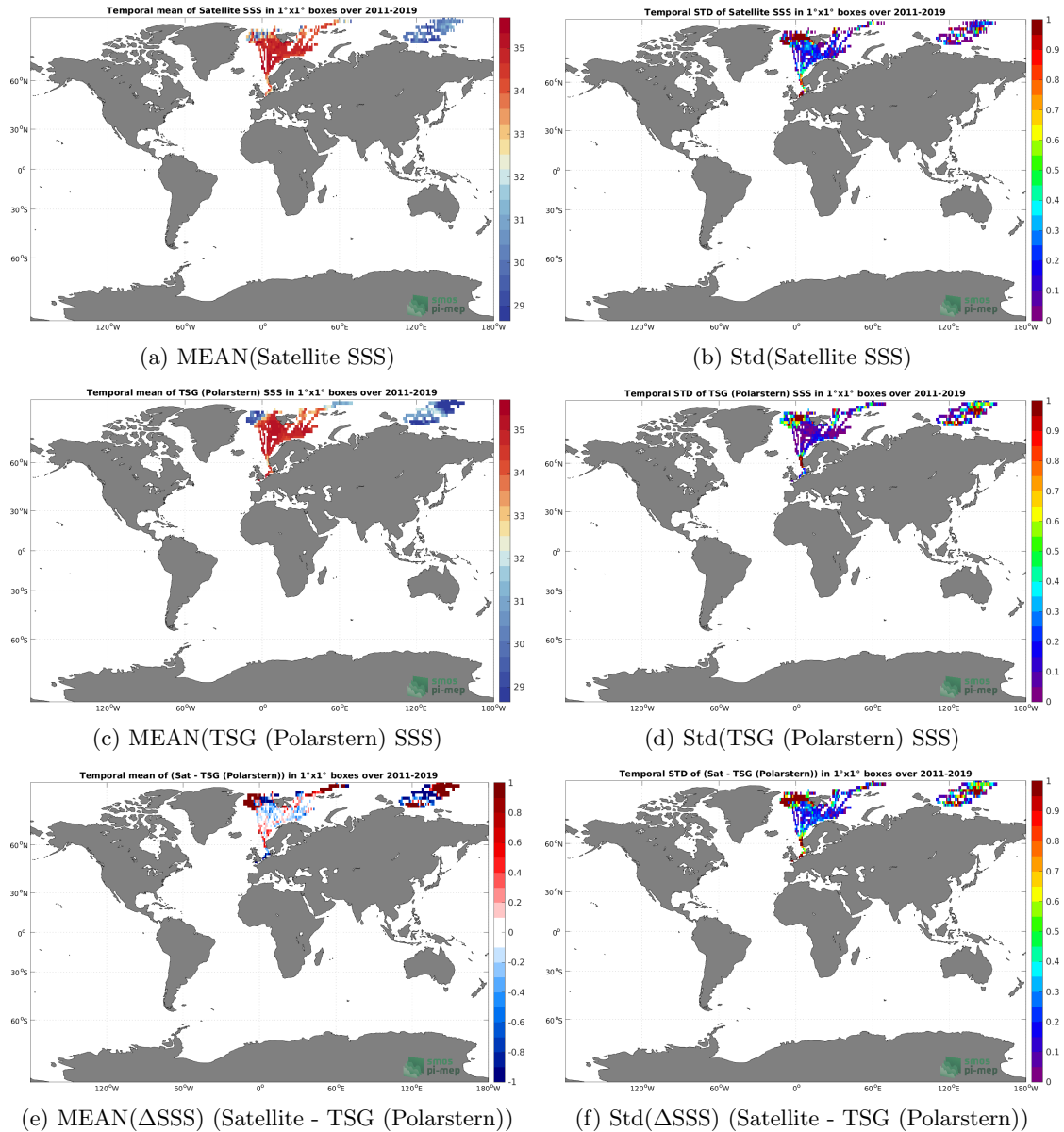
Figure 6: Temporal mean (left) and Std (right) of SSS from SMOS SSS L3 Arctic v3.1 - 9 Days (BEC) (top), TSG (Polarstern) (middle), and of \Delta SSS (Satellite - TSG (Polarstern)). Only match-up pairs are used to generate these maps.
