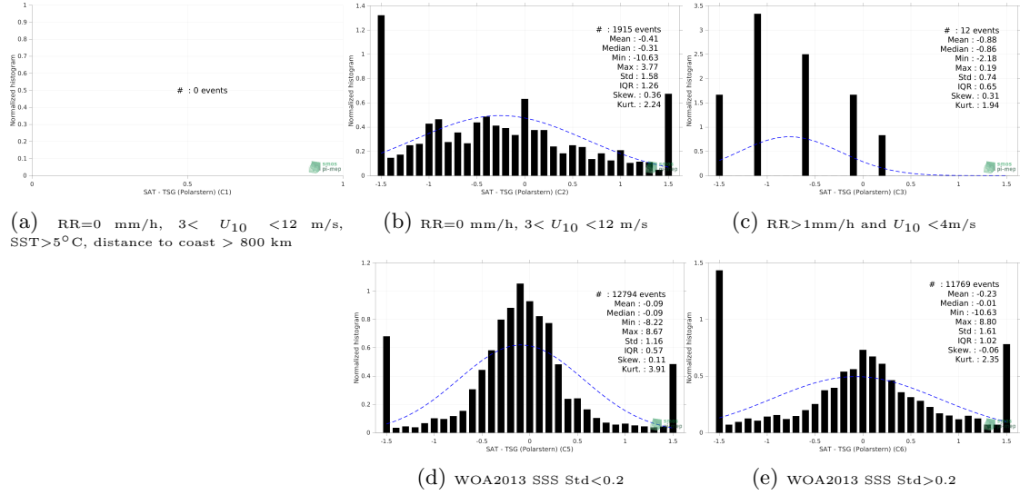
Figure 13: Normalized histogram of \Delta SSS (SMOS SSS L3 Arctic v3.1 - 9 Days (BEC) - TSG (Polarstern)) for 5 different subdatasets corresponding to: RR=0 mm/h, 3 < U_{10} < 12 m/s, SST > 5°C, distance to coast > 800 km (a), RR=0 mm/h, 3 < U_{10} < 12 m/s (b), RR > 1mm/h and U_{10} < 4 m/s (c), WOA2013 SSS Std < 0.2 (d), WOA2013 SSS Std > 0.2 (e).
