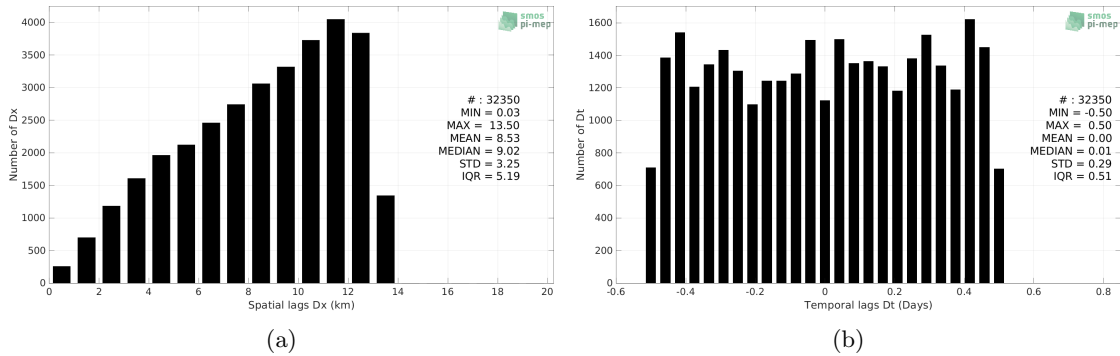
Figure 5: Histograms of the spatial (a) and temporal (b) lags between the location/time of the TSG (Polarstern) measurement and the date of the corresponding SMOS SSS L3 Arctic v3.1 - 9 Days (BEC) SSS pixel.
