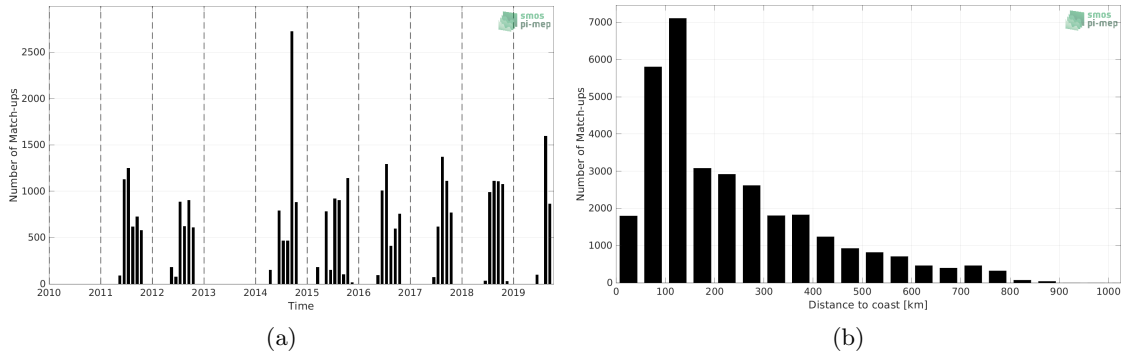
Figure 1: Number of match-ups between TSG (Polarstern) and SMOS SSS L3 Arctic v3.1 - 9 Days (BEC) SSS as a function of time (a) and as function of the distance to coast (b) over the Global Ocean Pi-MEP region and for the full satellite product period.
