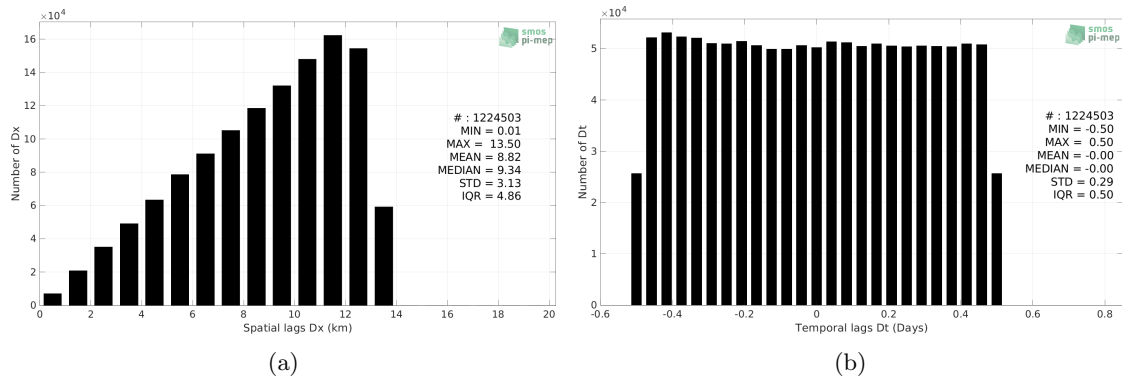
Figure 5: Histograms of the spatial (a) and temporal (b) lags between the location/time of the TSG (LEGOS-DM) measurement and the date of the corresponding SMOS SSS L3 Arctic v3.1 - 9 Days (BEC) SSS pixel.
