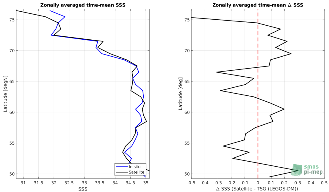
Figure 8: Left panel: Zonal mean SSS from SMOS SSS L3 Arctic v3.1 - 9 Days (BEC) satellite product (black) and from TSG (LEGOS-DM) (blue). Right panel: Zonal mean of \Delta SSS (Satellite - TSG (LEGOS-DM)) for all the collected Pi-MEP match-up pairs estimated over the full satellite product period.
