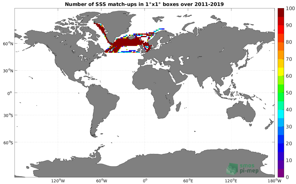
Figure 4: Number of SSS match-ups between TSG (LEGOS-DM) SSS and the SMOS SSS L3 Arctic v3.1 - 9 Days (BEC) SSS product for the Global Ocean Pi-MEP region over 1^\circ \times 1^\circ boxes and for the full satellite product period.
