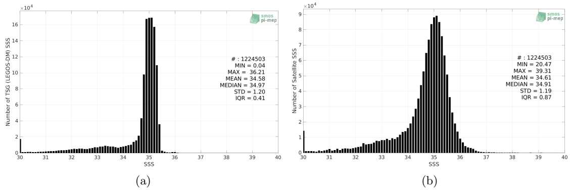
Figure 2: Histograms of SSS from TSG (LEGOS-DM) (a) and SMOS SSS L3 Arctic v3.1 - 9 Days (BEC) (b) considering all match-up pairs per bins of 0.1 over the Global Ocean Pi-MEP region and for the full satellite product period.
