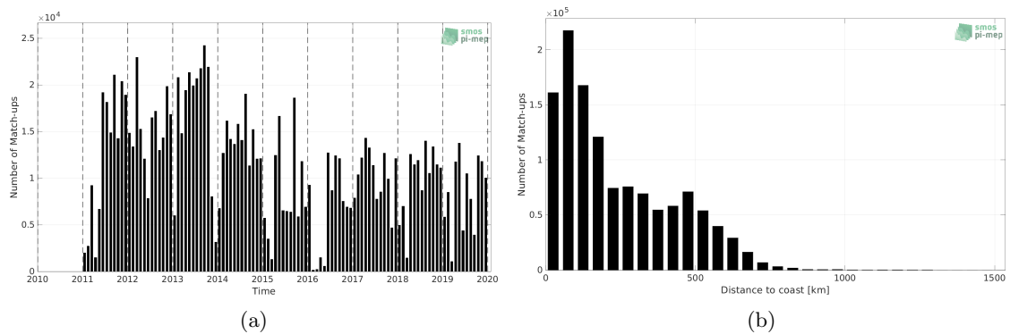
Figure 1: Number of match-ups between TSG (LEGOS-DM) and SMOS SSS L3 Arctic v3.1 - 9 Days (BEC) SSS as a function of time (a) and as function of the distance to coast (b) over the Global Ocean Pi-MEP region and for the full satellite product period.
