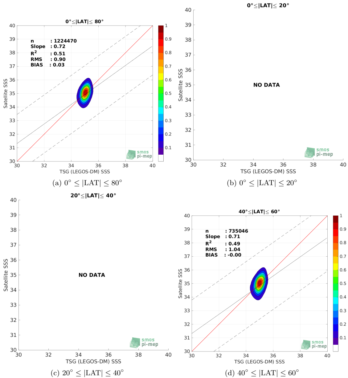
Figure 9: Contour maps of the concentration of SMOS SSS L3 Arctic v3.1 - 9 Days (BEC) SSS (y-axis) versus TSG (LEGOS-DM) SSS (x-axis) at match-up pairs for different latitude bands. For each plot, the red line shows x=y . The black thin and dashed lines indicate a linear fit through the data cloud and the \pm 95\% confidence levels, respectively. The number match-up pairs n , the slope and R^2 coefficient of the linear fit, the root mean square (RMS) and the mean bias between satellite and in situ data are indicated for each latitude band in each plots.
