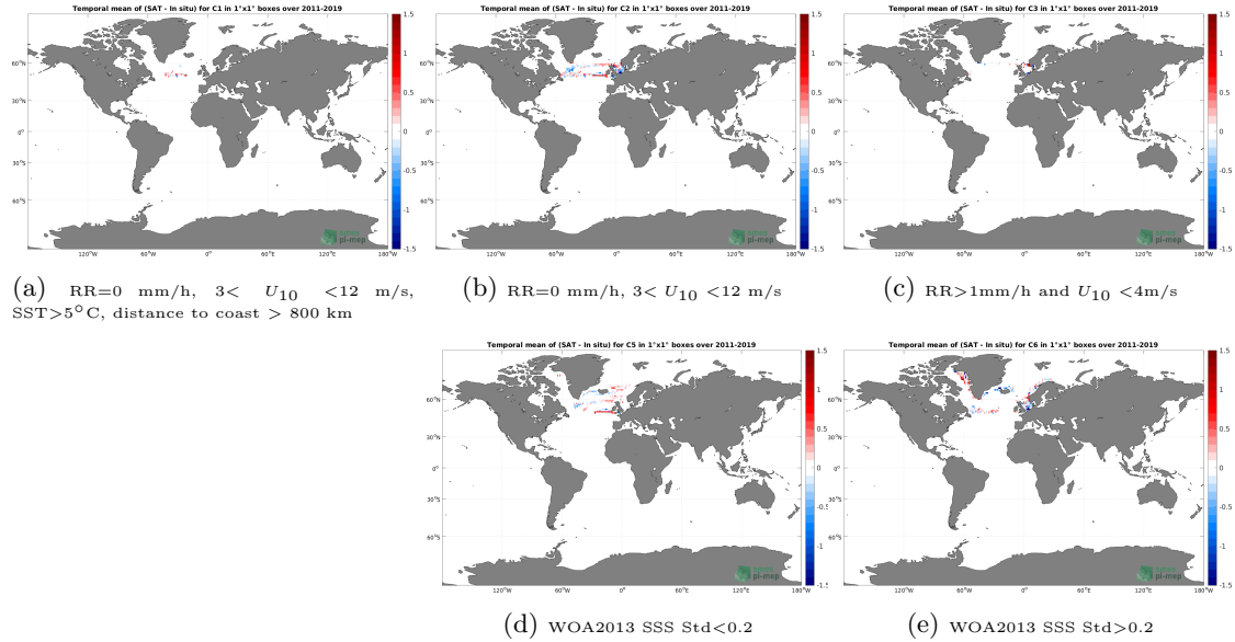
Figure 12: Temporal mean gridded over spatial boxes of size 1^{\circ}\times 1^{\circ} of \Delta\text{SSS} (SMOS SSS L3 Arctic v3.1 - 9 Days (BEC) - TSG (LEGOS-DM)) for 5 different subdatasets corresponding to:RR=0 mm/h, 3 < U_{10} < 12 m/s, SST >5^{\circ}\text{C} , distance to coast > 800 km (a), RR=0 mm/h, 3 < U_{10} < 12 m/s (b), RR >1 mm/h and U_{10} < 4 m/s (c), WOA2013 SSS Std <0.2 (d), WOA2013 SSS Std >0.2 (e).
