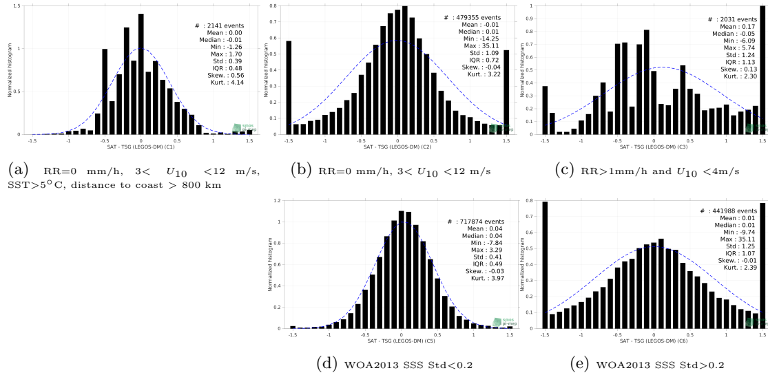
Figure 13: Normalized histogram of \Delta SSS (SMOS SSS L3 Arctic v3.1 - 9 Days (BEC) - TSG (LEGOS-DM)) for 5 different subdatasets corresponding to: RR=0 mm/h, 3 < U_{10} < 12 m/s, SST > 5°C, distance to coast > 800 km (a), RR=0 mm/h, 3 < U_{10} < 12 m/s (b), RR > 1mm/h and U_{10} < 4 m/s (c), WOA2013 SSS Std < 0.2 (d), WOA2013 SSS Std > 0.2 (e).
