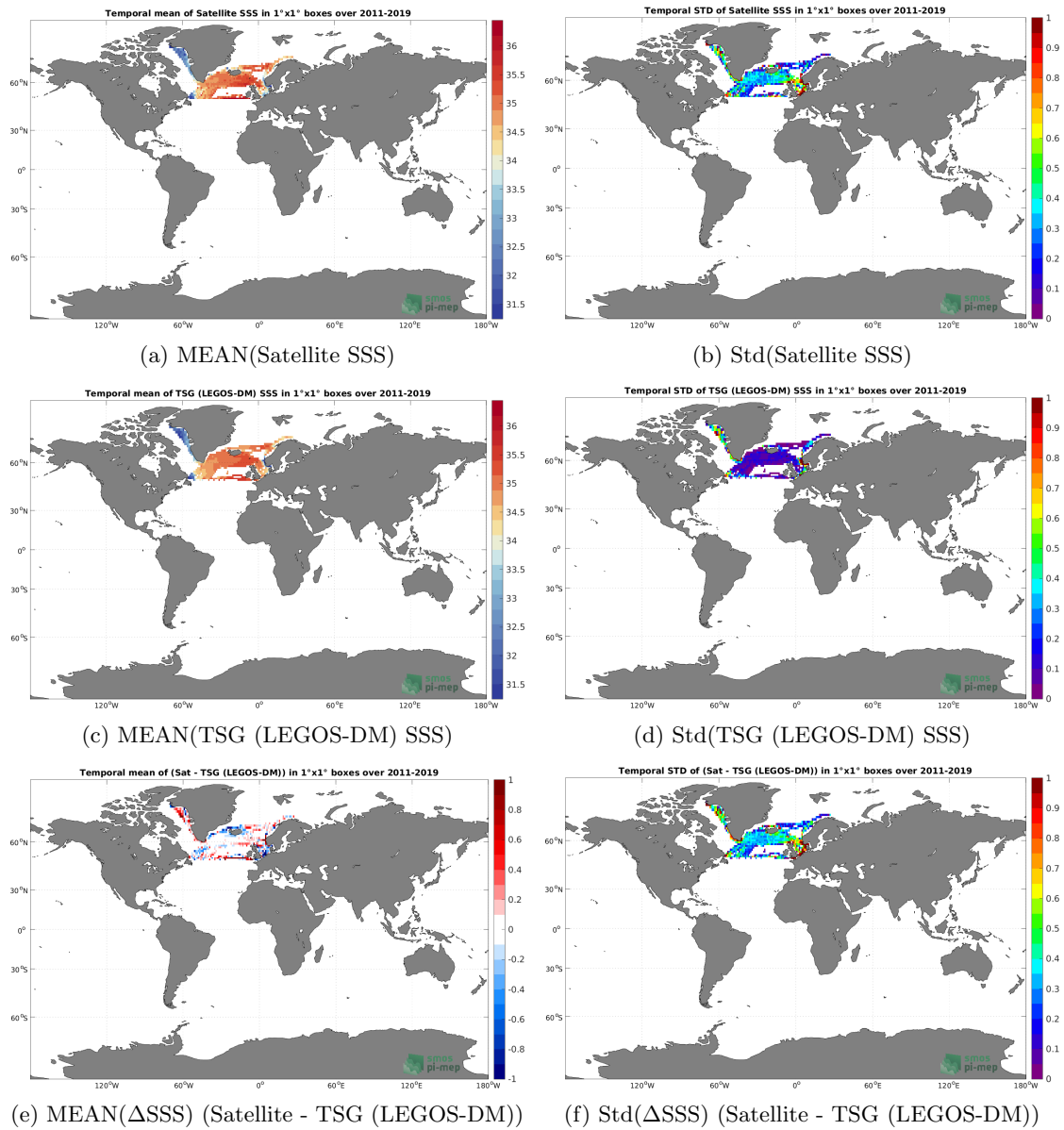
Figure 6: Temporal mean (left) and Std (right) of SSS from SMOS SSS L3 Arctic v3.1 - 9 Days (BEC) (top), TSG (LEGOS-DM) (middle), and of \Delta SSS (Satellite - TSG (LEGOS-DM)). Only match-up pairs are used to generate these maps.
