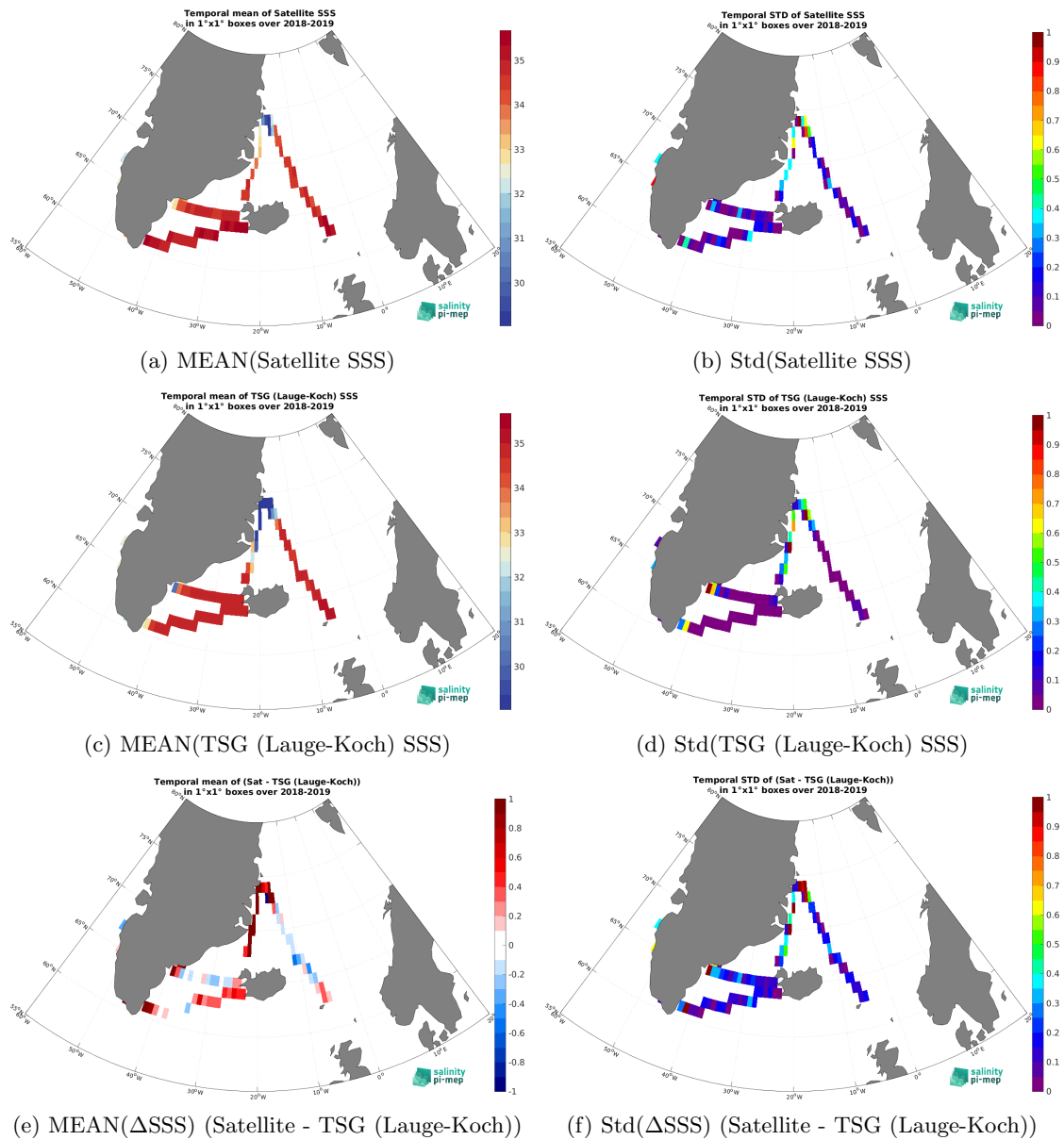
Figure 6: Temporal mean (left) and Std (right) of SSS from SMOS SSS L3 Arctic v3.1 - 9 Days (BEC) (top), TSG (Lauge-Koch) (middle), and of \Delta SSS (Satellite - TSG (Lauge-Koch)). Only match-up pairs are used to generate these maps.
