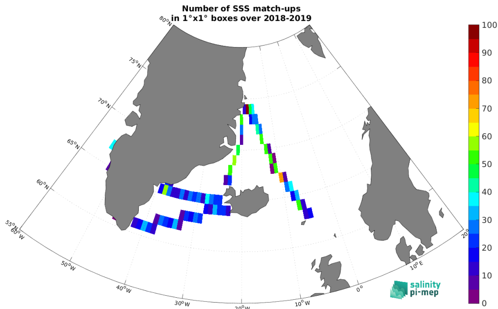
Figure 4: Number of SSS match-ups between TSG (Lauge-Koch) SSS and the SMOS SSS L3 Arctic v3.1 - 9 Days (BEC) SSS product for the Global Ocean Pi-MEP region over 1^\circ \times 1^\circ boxes and for the full satellite product period.
