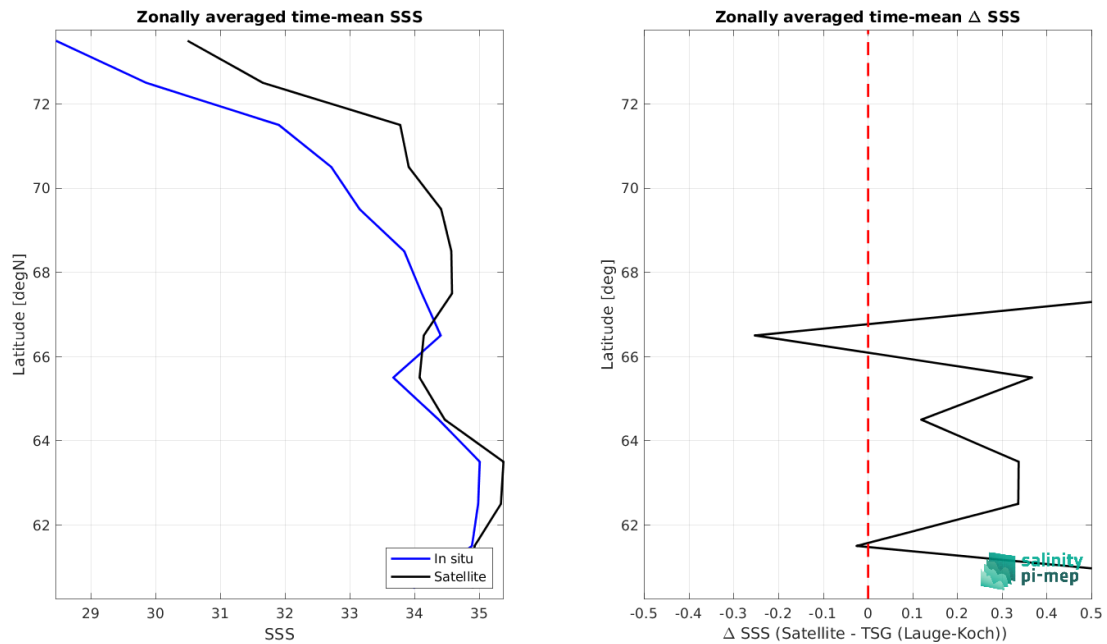
Figure 8: Left panel: Zonal mean SSS from SMOS SSS L3 Arctic v3.1 - 9 Days (BEC) satellite product (black) and from TSG (Lauge-Koch) (blue). Right panel: Zonal mean of \Delta SSS (Satellite - TSG (Lauge-Koch)) for all the collected Pi-MEP match-up pairs estimated over the full satellite product period.
