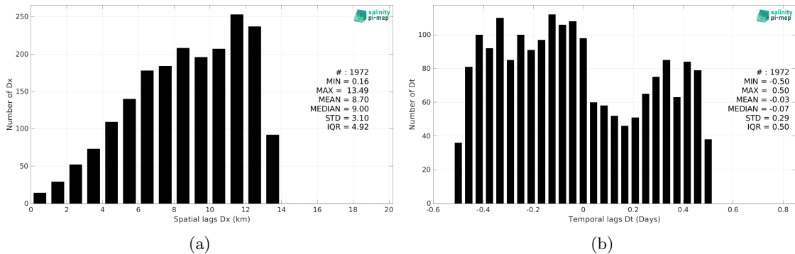
Figure 5: Histograms of the spatial (a) and temporal (b) lags between the location/time of the TSG (Lauge-Koch) measurement and the date of the corresponding SMOS SSS L3 Arctic v3.1 - 9 Days (BEC) SSS pixel.
