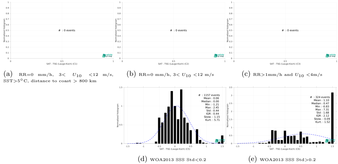
Figure 13: Normalized histogram of \Delta SSS (SMOS SSS L3 Arctic v3.1 - 9 Days (BEC) - TSG (Laue-Koch)) for 5 different subdatasets corresponding to: RR=0 mm/h, 3 < U_{10} < 12 m/s, SST > 5°C, distance to coast > 800 km (a), RR=0 mm/h, 3 < U_{10} < 12 m/s (b), RR > 1mm/h and U_{10} < 4 m/s (c), WOA2013 SSS Std < 0.2 (d), WOA2013 SSS Std > 0.2 (e).
