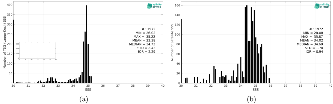
Figure 2: Histograms of SSS from TSG (Lauge-Koch) (a) and SMOS SSS L3 Arctic v3.1 - 9 Days (BEC) (b) considering all match-up pairs per bins of 0.1 over the Global Ocean Pi-MEP region and for the full satellite product period.
