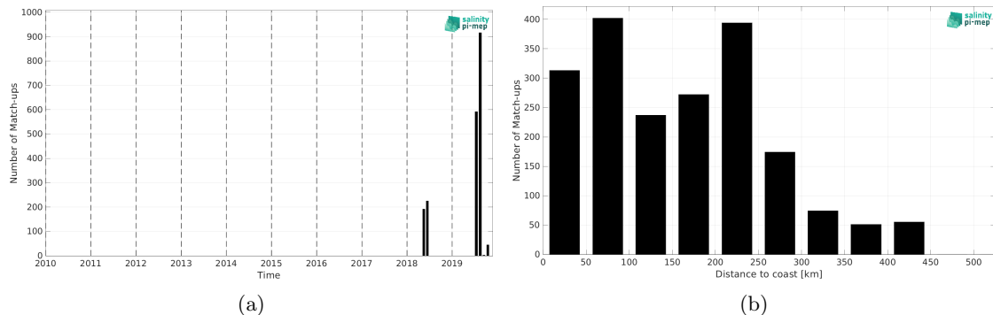
Figure 1: Number of match-ups between TSG (Lauge-Koch) and SMOS SSS L3 Arctic v3.1 - 9 Days (BEC) SSS as a function of time (a) and as function of the distance to coast (b) over the Global Ocean Pi-MEP region and for the full satellite product period.
