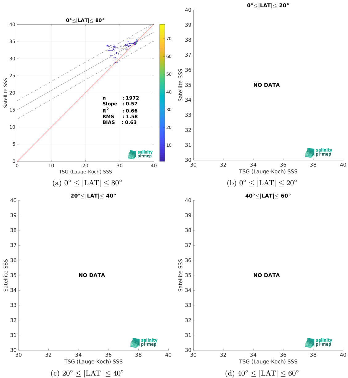
Figure 9: Contour maps of the concentration of SMOS SSS L3 Arctic v3.1 - 9 Days (BEC) SSS (y-axis) versus TSG (Lauge-Koch) SSS (x-axis) at match-up pairs for different latitude bands. For each plot, the red line shows x=y . The black thin and dashed lines indicate a linear fit through the data cloud and the \pm 95\% confidence levels, respectively. The number match-up pairs n , the slope and R^2 coefficient of the linear fit, the root mean square (RMS) and the mean bias between satellite and in situ data are indicated for each latitude band in each plots.
