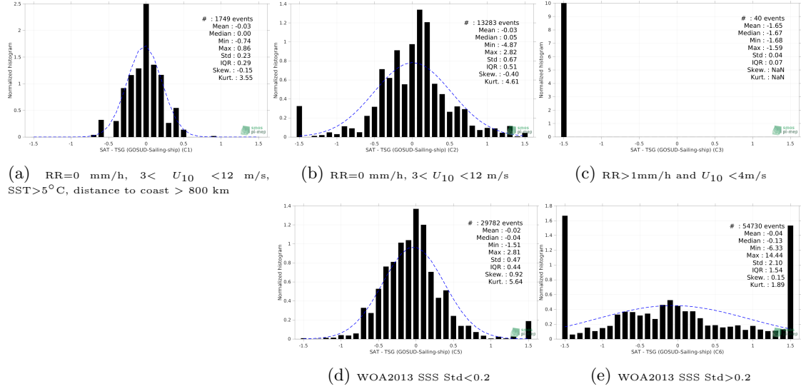
Figure 13: Normalized histogram of \Delta SSS (SMOS SSS L3 Arctic v3.1 - 9 Days (BEC) - TSG (GOSUD-Sailing-ship)) for 5 different subdatasets corresponding to: RR=0 mm/h, 3 < U_{10} < 12 m/s, SST>5°C, distance to coast > 800 km (a), RR=0 mm/h, 3 < U_{10} < 12 m/s (b), RR>1mm/h and U_{10} < 4 m/s (c), WOA2013 SSS Std<0.2 (d), WOA2013 SSS Std>0.2 (e).
