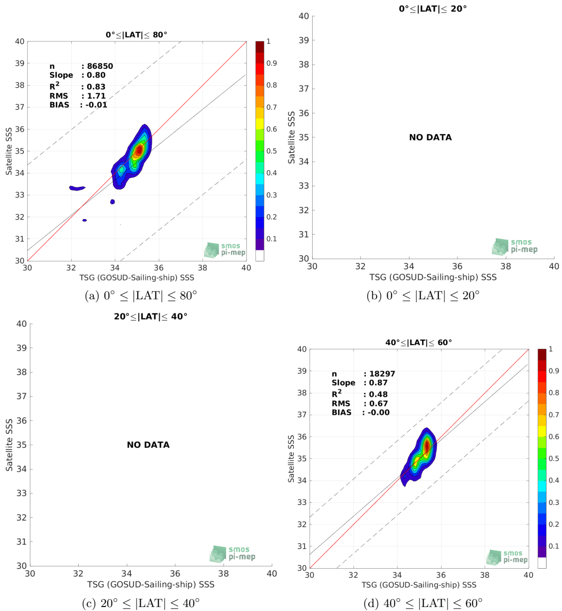
Figure 9: Contour maps of the concentration of SMOS SSS L3 Arctic v3.1 - 9 Days (BEC) SSS (y-axis) versus TSG (GOSUD-Sailing-ship) SSS (x-axis) at match-up pairs for different latitude bands. For each plot, the red line shows x=y . The black thin and dashed lines indicate a linear fit through the data cloud and the \pm 95\% confidence levels, respectively. The number match-up pairs n , the slope and R^2 coefficient of the linear fit, the root mean square (RMS) and the mean bias between satellite and in situ data are indicated for each latitude band in each plots.
