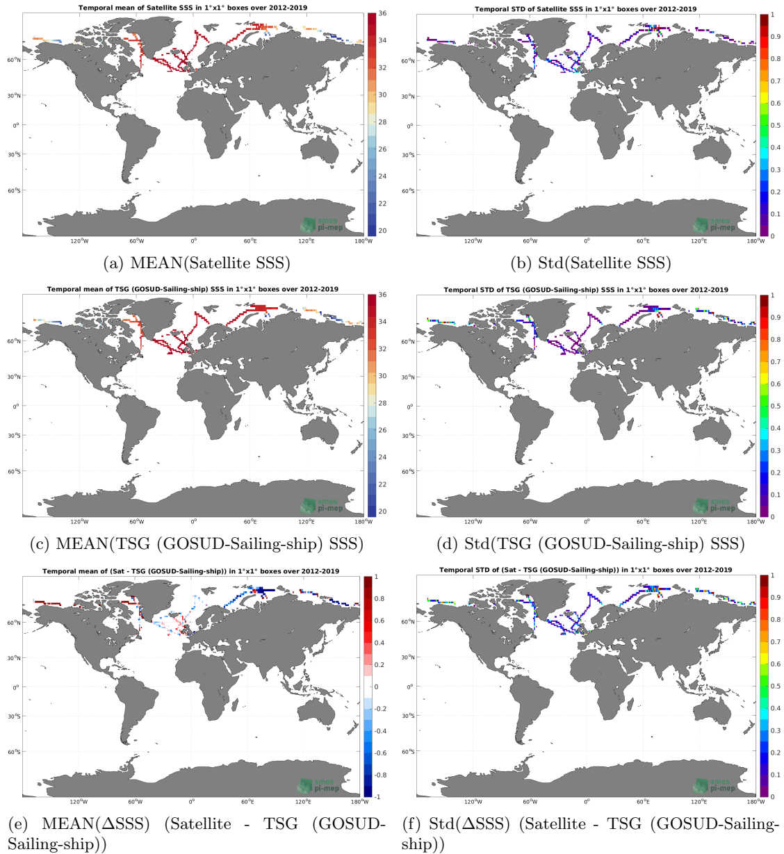
Figure 6: Temporal mean (left) and Std (right) of SSS from SMOS SSS L3 Arctic v3.1 - 9 Days (BEC) (top), TSG (GOSUD-Sailing-ship) (middle), and of \Delta SSS (Satellite - TSG (GOSUD-Sailing-ship)). Only match-up pairs are used to generate these maps.
