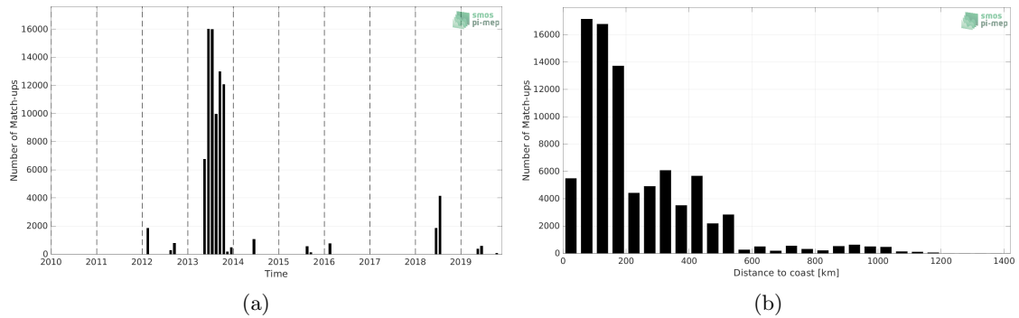
Figure 1: Number of match-ups between TSG (GOSUD-Sailing-ship) and SMOS SSS L3 Arctic v3.1 - 9 Days (BEC) SSS as a function of time (a) and as function of the distance to coast (b) over the Global Ocean Pi-MEP region and for the full satellite product period.
