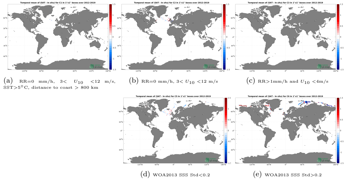
Figure 12: Temporal mean gridded over spatial boxes of size 1^{\circ}\times 1^{\circ} of \Delta SSS (SMOS SSS L3 Arctic v3.1 - 9 Days (BEC) - TSG (GOSUD-Sailing-ship)) for 5 different subdatasets corresponding to:RR=0 mm/h, 3 < U_{10} < 12 m/s, SST >5^{\circ}\text{C} , distance to coast > 800 km (a), RR=0 mm/h, 3 < U_{10} < 12 m/s (b), RR >1 mm/h and U_{10} < 4 m/s (c), WOA2013 SSS Std <0.2 (d), WOA2013 SSS Std >0.2 (e).
