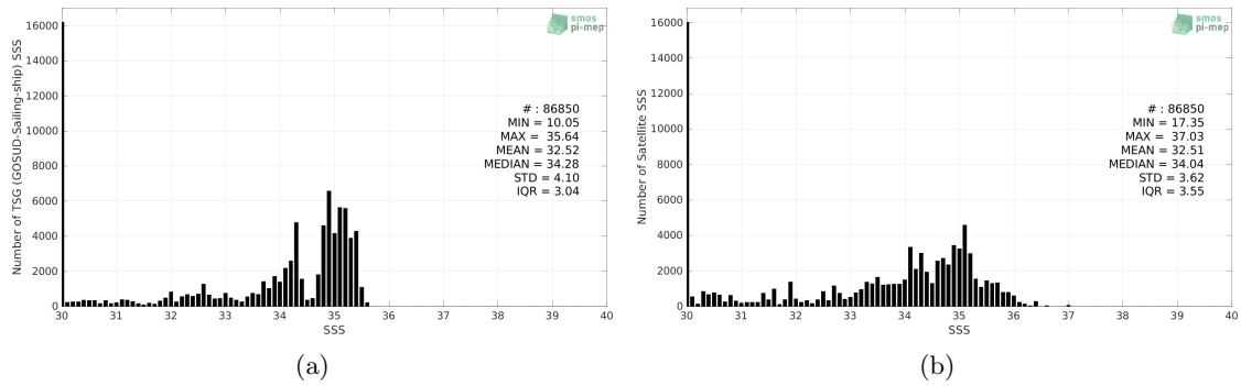
Figure 2: Histograms of SSS from TSG (GOSUD-Sailing-ship) (a) and SMOS SSS L3 Arctic v3.1 - 9 Days (BEC) (b) considering all match-up pairs per bins of 0.1 over the Global Ocean Pi-MEP region and for the full satellite product period.
