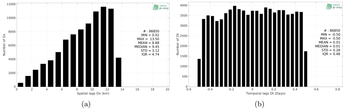
Figure 5: Histograms of the spatial (a) and temporal (b) lags between the location/time of the TSG (GOSUD-Sailing-ship) measurement and the date of the corresponding SMOS SSS L3 Arctic v3.1 - 9 Days (BEC) SSS pixel.
