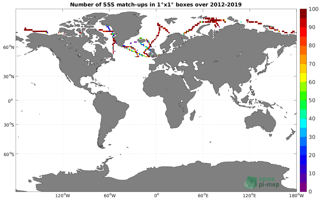
Figure 4: Number of SSS match-ups between TSG (GOSUD-Sailing-ship) SSS and the SMOS SSS L3 Arctic v3.1 - 9 Days (BEC) SSS product for the Global Ocean Pi-MEP region over 1^\circ \times 1^\circ boxes and for the full satellite product period.
