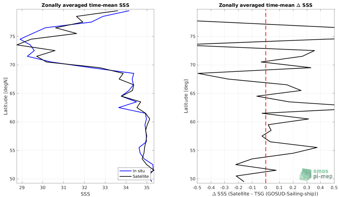
Figure 8: Left panel: Zonal mean SSS from SMOS SSS L3 Arctic v3.1 - 9 Days (BEC) satellite product (black) and from TSG (GOSUD-Sailing-ship) (blue). Right panel: Zonal mean of \Delta SSS (Satellite - TSG (GOSUD-Sailing-ship)) for all the collected Pi-MEP match-up pairs estimated over the full satellite product period.
