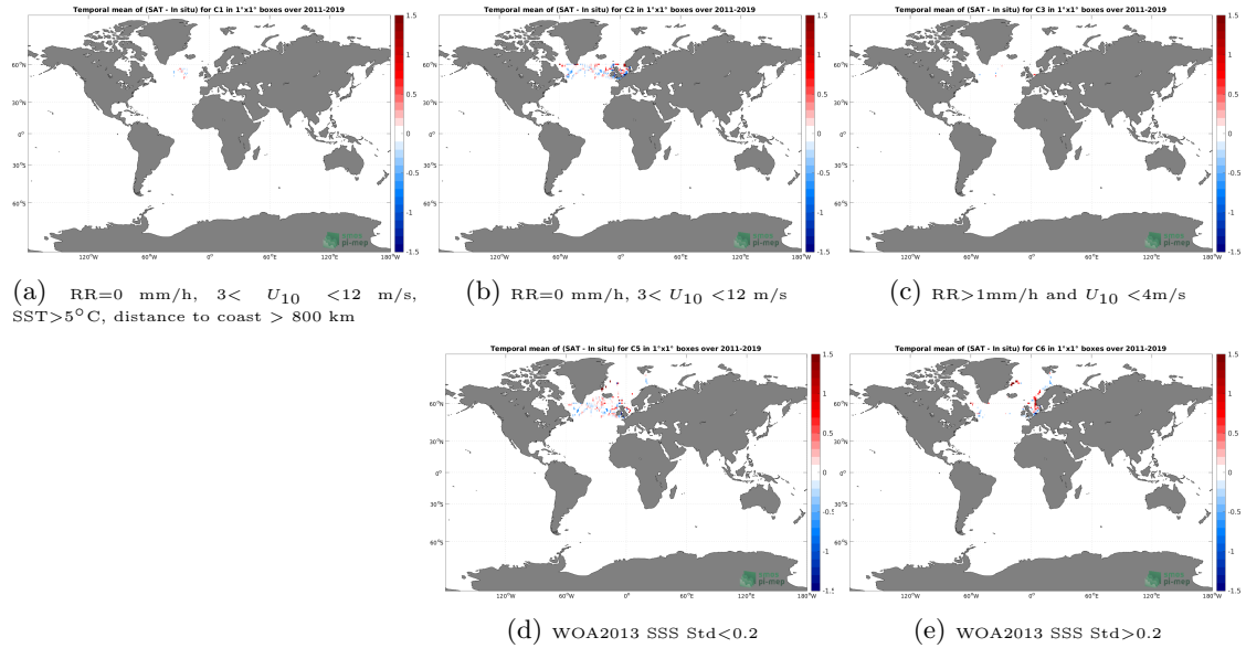
Figure 12: Temporal mean gridded over spatial boxes of size 1^{\circ}\times 1^{\circ} of \Delta SSS (SMOS SSS L3 Arctic v3.1 - 9 Days (BEC) - TSG (GOSUD-Research-vessel)) for 5 different subdatasets corresponding to:RR=0 mm/h, 3 < U_{10} < 12 m/s, SST >5^{\circ}\text{C} , distance to coast > 800 km (a), RR=0 mm/h, 3 < U_{10} < 12 m/s (b), RR >1 mm/h and U_{10} < 4 m/s (c), WOA2013 SSS Std <0.2 (d), WOA2013 SSS Std >0.2 (e).
