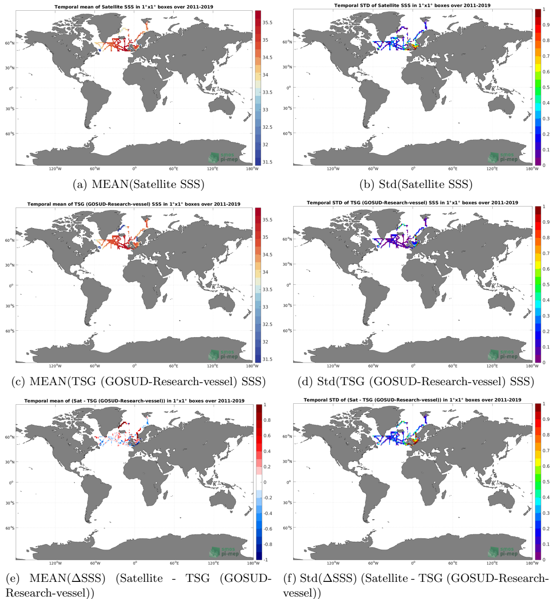
Figure 6: Temporal mean (left) and Std (right) of SSS from SMOS SSS L3 Arctic v3.1 - 9 Days (BEC) (top), TSG (GOSUD-Research-vessel) (middle), and of \Delta SSS (Satellite - TSG (GOSUD-Research-vessel)). Only match-up pairs are used to generate these maps.
