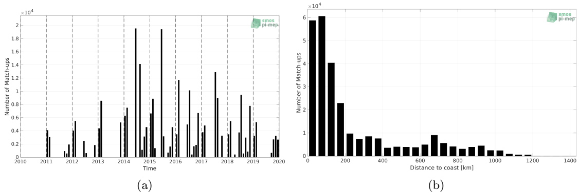
Figure 1: Number of match-ups between TSG (GOSUD-Research-vessel) and SMOS SSS L3 Arctic v3.1 - 9 Days (BEC) SSS as a function of time (a) and as function of the distance to coast (b) over the Global Ocean Pi-MEP region and for the full satellite product period.
