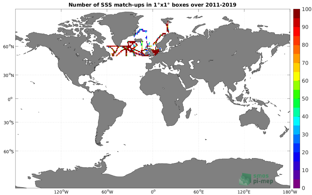
Figure 4: Number of SSS match-ups between TSG (GOSUD-Research-vessel) SSS and the SMOS SSS L3 Arctic v3.1 - 9 Days (BEC) SSS product for the Global Ocean Pi-MEP region over 1^\circ \times 1^\circ boxes and for the full satellite product period.
