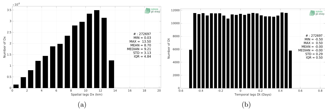
Figure 5: Histograms of the spatial (a) and temporal (b) lags between the location/time of the TSG (GOSUD-Research-vessel) measurement and the date of the corresponding SMOS SSS L3 Arctic v3.1 - 9 Days (BEC) SSS pixel.
