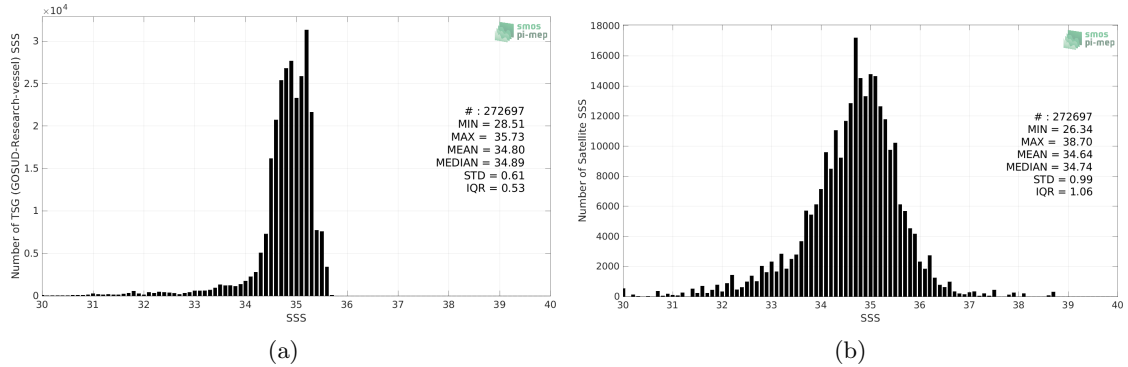
Figure 2: Histograms of SSS from TSG (GOSUD-Research-vessel) (a) and SMOS SSS L3 Arctic v3.1 - 9 Days (BEC) (b) considering all match-up pairs per bins of 0.1 over the Global Ocean Pi-MEP region and for the full satellite product period.
