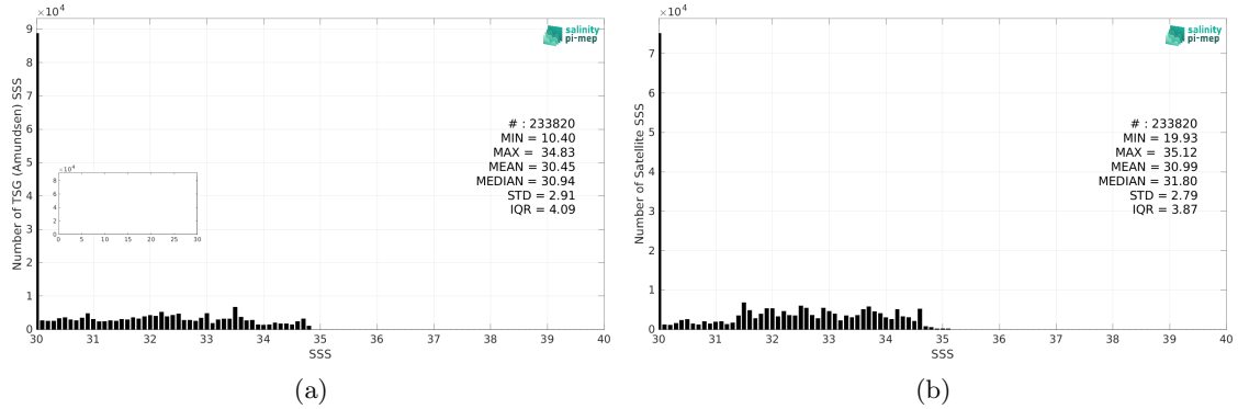
Figure 2: Histograms of SSS from TSG (Amundsen) (a) and SMOS SSS L3 Arctic v3.1 - 9 Days (BEC) (b) considering all match-up pairs per bins of 0.1 over the Global Ocean Pi-MEP region and for the full satellite product period.
