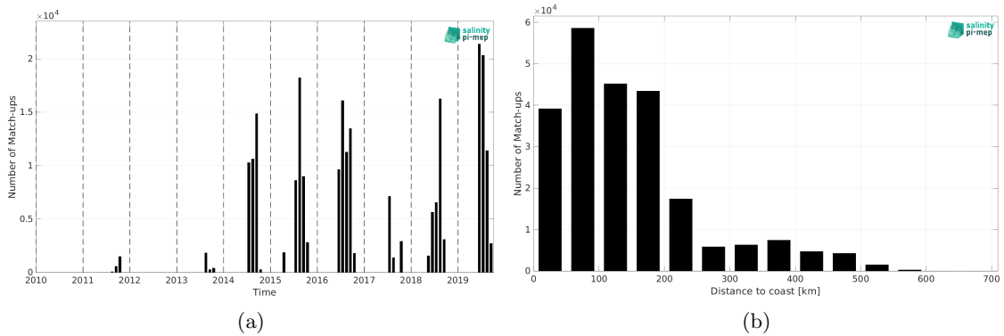
Figure 1: Number of match-ups between TSG (Amundsen) and SMOS SSS L3 Arctic v3.1 - 9 Days (BEC) SSS as a function of time (a) and as function of the distance to coast (b) over the Global Ocean Pi-MEP region and for the full satellite product period.
