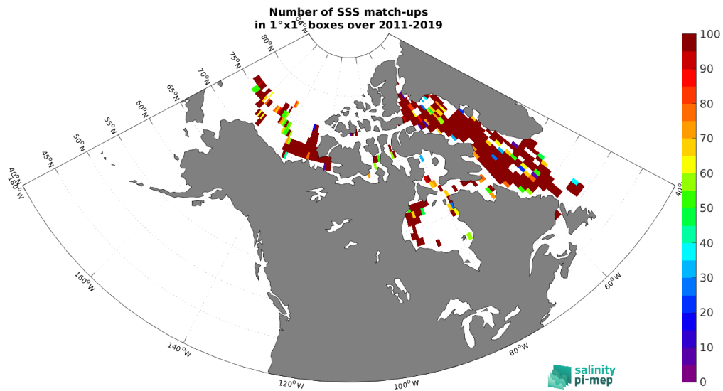
Figure 4: Number of SSS match-ups between TSG (Amundsen) SSS and the SMOS SSS L3 Arctic v3.1 - 9 Days (BEC) SSS product for the Global Ocean Pi-MEP region over 1°×1° boxes and for the full satellite product period.
