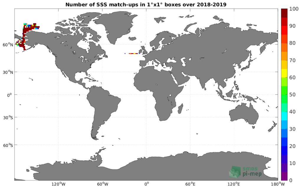
Figure 4: Number of SSS match-ups between Saildrone SSS and the SMOS SSS L3 Arctic v3.1 - 9 Days (BEC) SSS product for the Global Ocean Pi-MEP region over 1^\circ \times 1^\circ boxes and for the full satellite product period.
