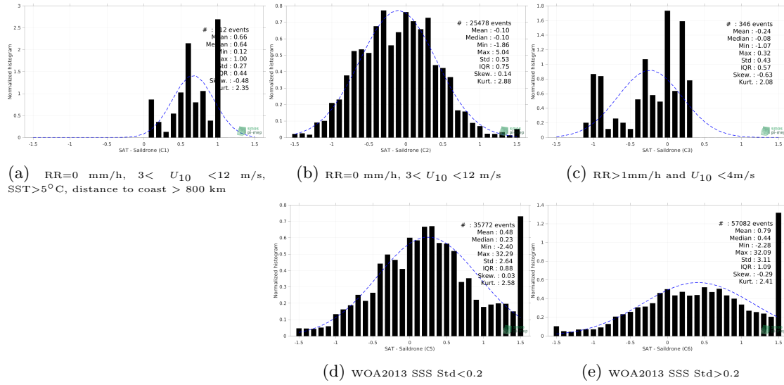
Figure 13: Normalized histogram of \Delta SSS (SMOS SSS L3 Arctic v3.1 - 9 Days (BEC) - Sairdrone) for 5 different subdatasets corresponding to: RR=0 mm/h, 3 < U_{10} < 12 m/s, SST > 5°C, distance to coast > 800 km (a), RR=0 mm/h, 3 < U_{10} < 12 m/s (b), RR > 1mm/h and U_{10} < 4 m/s (c), WOA2013 SSS Std < 0.2 (d), WOA2013 SSS Std > 0.2 (e).
