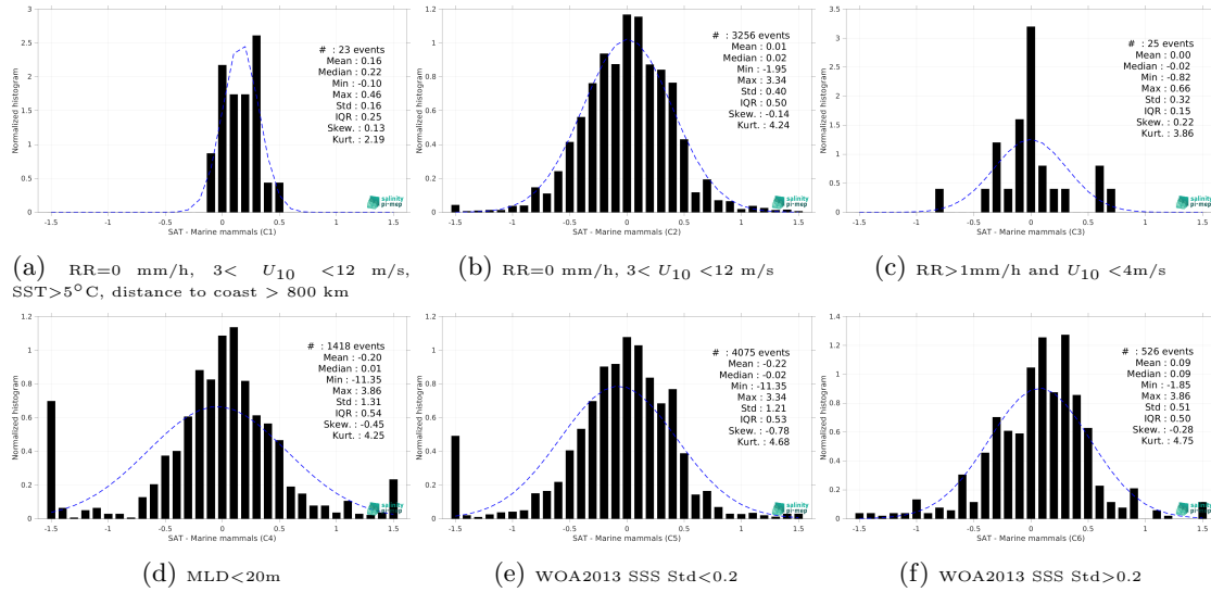
Figure 13: Normalized histogram of \Delta\text{SSS} (SMOS SSS L3 Arctic v3.1 - 9 Days (BEC) - Marine mammals) for 6 different subdatasets corresponding to: RR=0 mm/h, 3 < U_{10} < 12 m/s, SST>5°C, distance to coast > 800 km (a), RR=0 mm/h, 3 < U_{10} < 12 m/s (b), RR>1mm/h and U_{10} < 4 m/s (c), MLD<20m (d), WOA2013 SSS Std<0.2 (e), WOA2013 SSS Std>0.2 (f).
