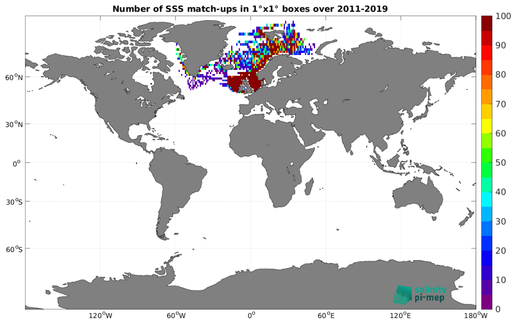
Figure 4: Number of SSS match-ups between ICES SSS and the SMOS SSS L3 Arctic v3.1 - 9 Days (BEC) SSS product for the Global Ocean Pi-MEP region over 1^\circ \times 1^\circ boxes and for the full satellite product period.
