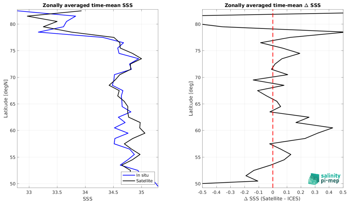
Figure 8: Left panel: Zonal mean SSS from SMOS SSS L3 Arctic v3.1 - 9 Days (BEC) satellite product (black) and from ICES (blue). Right panel: Zonal mean of \Delta SSS (Satellite - ICES) for all the collected Pi-MEP match-up pairs estimated over the full satellite product period.
