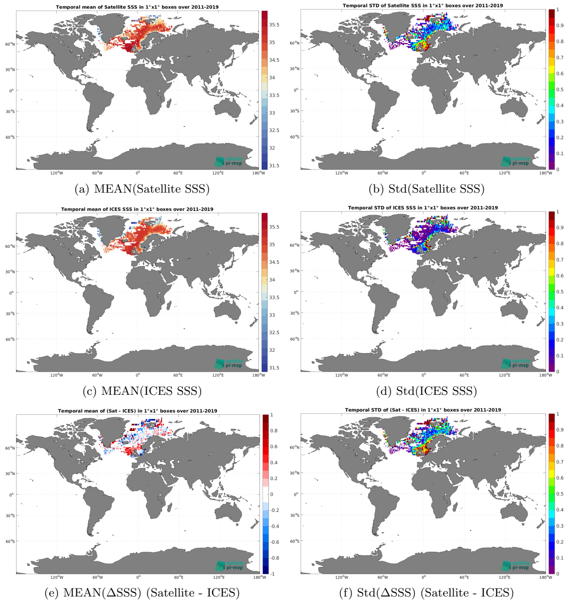
Figure 6: Temporal mean (left) and Std (right) of SSS from SMOS SSS L3 Arctic v3.1 - 9 Days (BEC) (top), ICES (middle), and of \Delta SSS (Satellite - ICES). Only match-up pairs are used to generate these maps.
