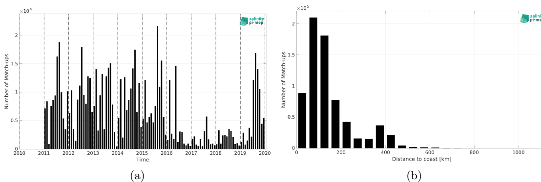
Figure 1: Number of match-ups between ICES and SMOS SSS L3 Arctic v3.1 - 9 Days (BEC) SSS as a function of time (a) and as function of the distance to coast (b) over the Global Ocean Pi-MEP region and for the full satellite product period.
