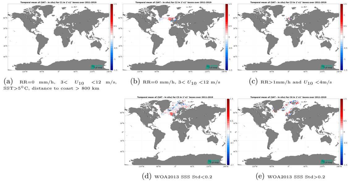
Figure 12: Temporal mean gridded over spatial boxes of size 1^{\circ}\times 1^{\circ} of \Delta\text{SSS} (SMOS SSS L3 Arctic v3.1 - 9 Days (BEC) - ICES) for 5 different subdatasets corresponding to:RR=0 mm/h, 3 < U_{10} < 12 m/s, SST >5^{\circ}\text{C} , distance to coast > 800 km (a), RR=0 mm/h, 3 < U_{10} < 12 m/s (b), RR >1 mm/h and U_{10} < 4 m/s (c), WOA2013 SSS Std <0.2 (d), WOA2013 SSS Std >0.2 (e).
