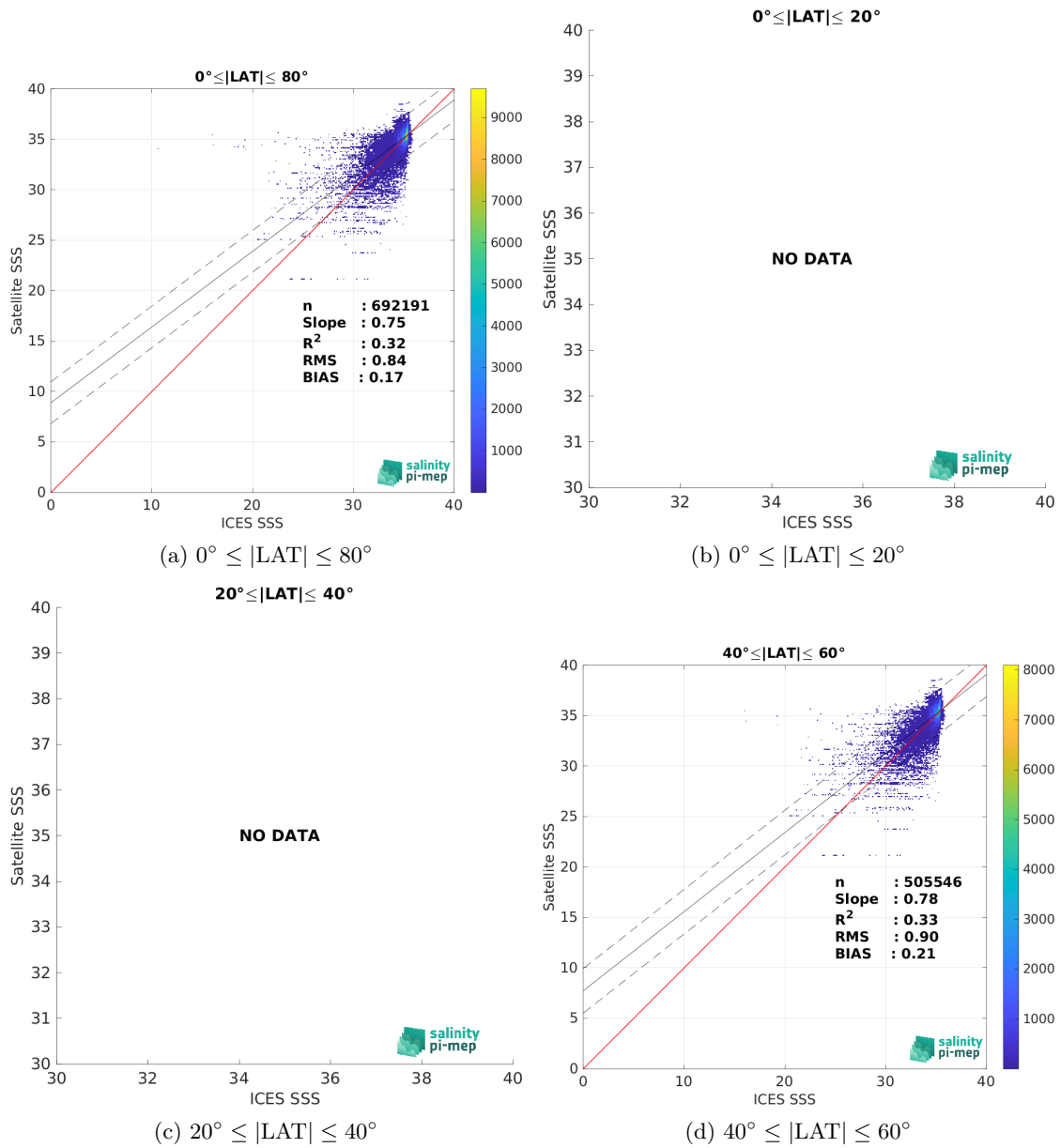
Figure 9: Contour maps of the concentration of SMOS SSS L3 Arctic v3.1 - 9 Days (BEC) SSS (y-axis) versus ICES SSS (x-axis) at match-up pairs for different latitude bands. For each plot, the red line shows x=y . The black thin and dashed lines indicate a linear fit through the data cloud and the \pm 95\% confidence levels, respectively. The number match-up pairs n , the slope and R^2 coefficient of the linear fit, the root mean square (RMS) and the mean bias between satellite and in situ data are indicated for each latitude band in each plots.
