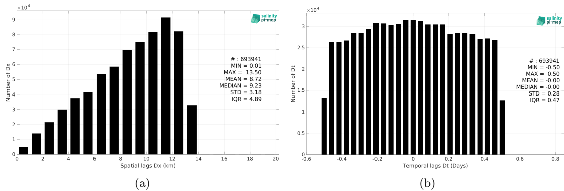
Figure 5: Histograms of the spatial (a) and temporal (b) lags between the location/time of the ICES measurement and the date of the corresponding SMOS SSS L3 Arctic v3.1 - 9 Days (BEC) SSS pixel.
