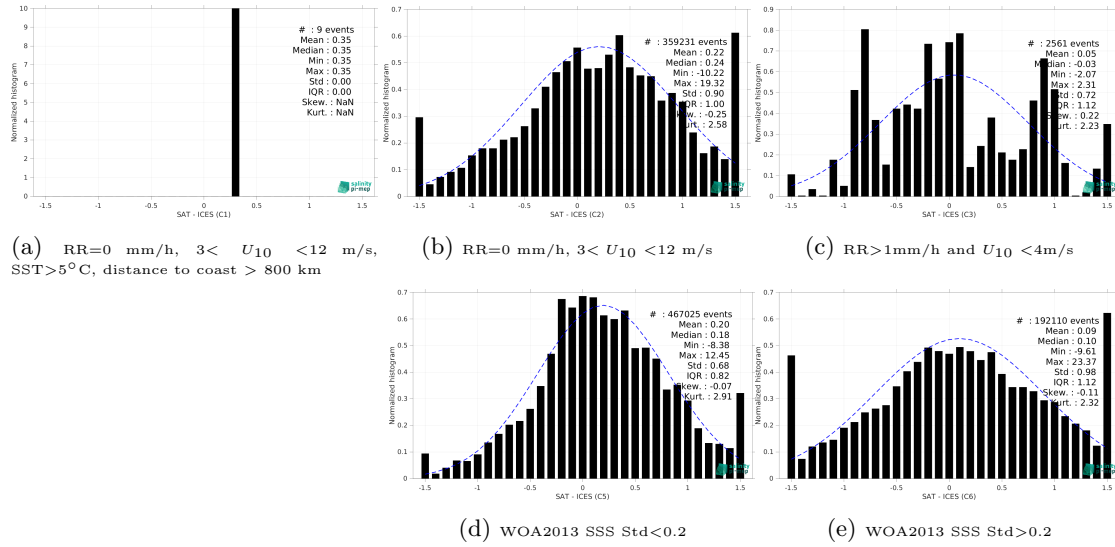
Figure 13: Normalized histogram of \Delta SSS (SMOS SSS L3 Arctic v3.1 - 9 Days (BEC) - ICES) for 5 different subdatasets corresponding to: RR=0 mm/h, 3 < U_{10} < 12 m/s, SST > 5°C, distance to coast > 800 km (a), RR=0 mm/h, 3 < U_{10} < 12 m/s (b), RR > 1mm/h and U_{10} < 4 m/s (c), WOA2013 SSS Std < 0.2 (d), WOA2013 SSS Std > 0.2 (e).
