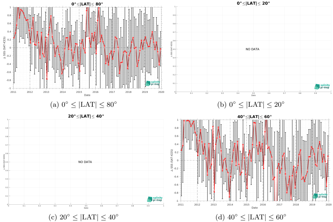
Figure 10: Monthly median (red curves) of \Delta SSS (Satellite - ICES) and \pm 1 Std (black vertical thick bars) as function of time for all the collected Pi-MEP match-up pairs estimated over the Global Ocean Pi-MEP region and for the full satellite product period are shown for different latitude bands: (a) 80^\circ\text{S}-80^\circ\text{N} , (b) 20^\circ\text{S}-20^\circ\text{N} , (c) 40^\circ\text{S}-20^\circ\text{S} and 20^\circ\text{N}-40^\circ\text{N} and (d) 60^\circ\text{S}-40^\circ\text{S} and 40^\circ\text{N}-60^\circ\text{N} .
