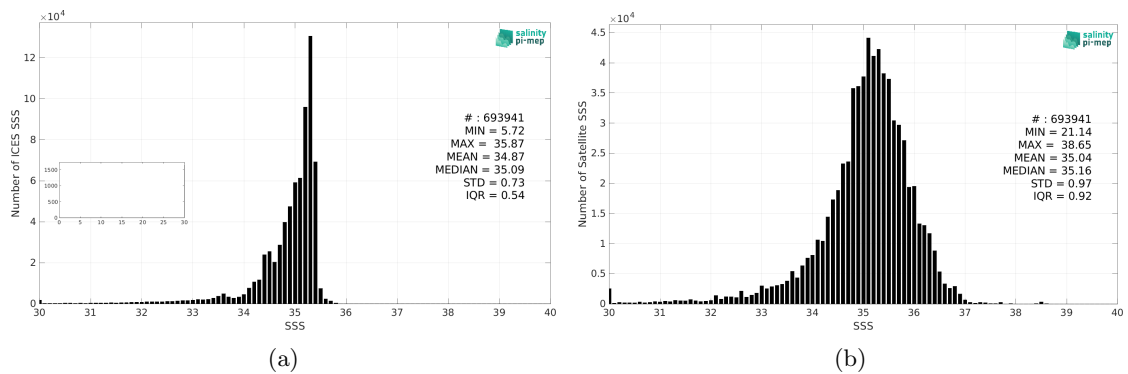
Figure 2: Histograms of SSS from ICES (a) and SMOS SSS L3 Arctic v3.1 - 9 Days (BEC) (b) considering all match-up pairs per bins of 0.1 over the Global Ocean Pi-MEP region and for the full satellite product period.
