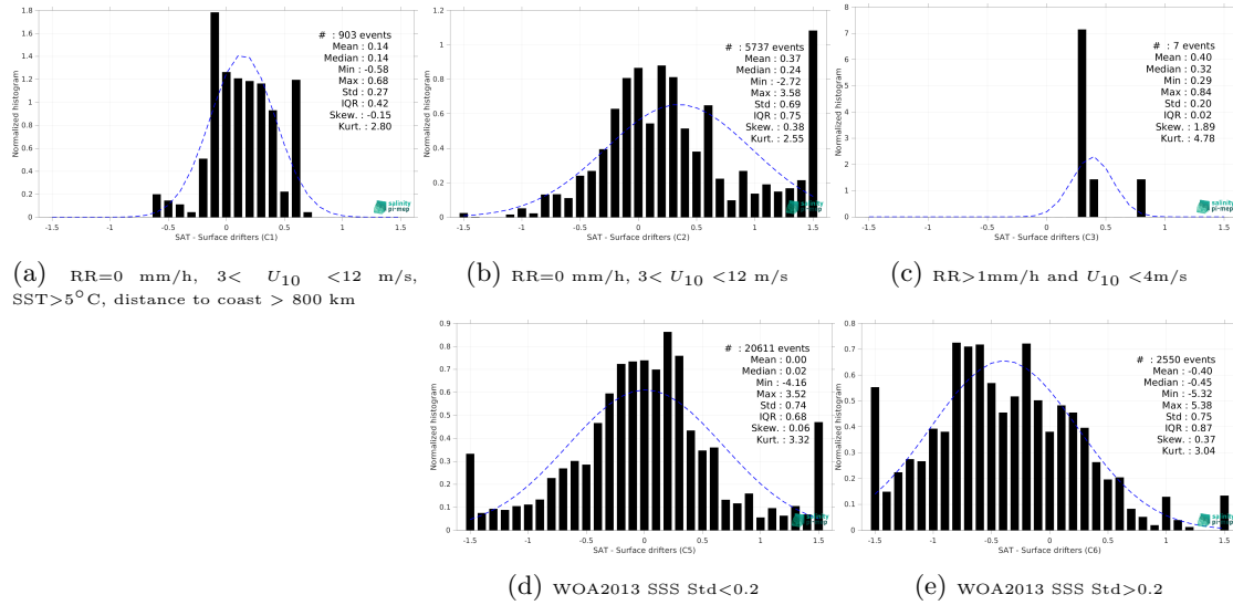
Figure 12: Normalized histogram of \Delta SSS (SMOS SSS L3 Arctic v3.1 - 9 Days (BEC) - Surface drifters) for 5 different subdatasets corresponding to: RR=0 mm/h, 3 < U_{10} < 12 m/s, SST>5°C, distance to coast > 800 km (a), RR=0 mm/h, 3 < U_{10} < 12 m/s (b), RR>1mm/h and U_{10} < 4 m/s (c), WOA2013 SSS Std<0.2 (d), WOA2013 SSS Std>0.2 (e).
