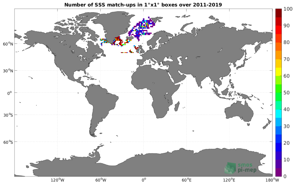
Figure 3: Number of SSS match-ups between Surface drifters SSS and the SMOS SSS L3 Arctic v3.1 - 9 Days (BEC) SSS product for the Global Ocean Pi-MEP region over 1^\circ \times 1^\circ boxes and for the full satellite product period.
