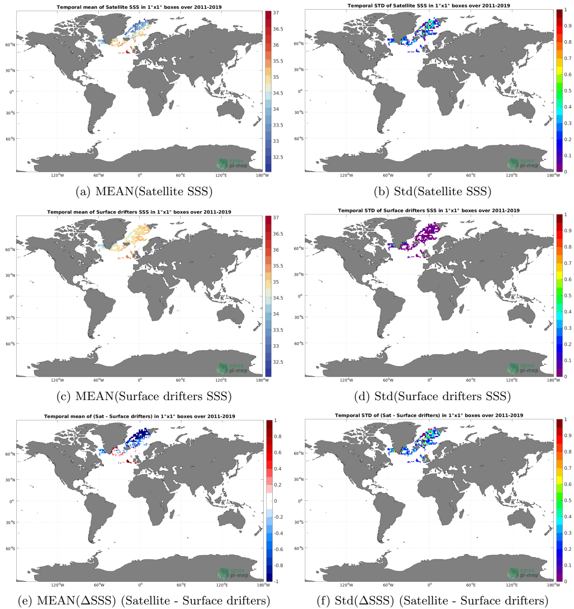
Figure 5: Temporal mean (left) and Std (right) of SSS from SMOS SSS L3 Arctic v3.1 - 9 Days (BEC) (top), Surface drifters (middle), and of \Delta SSS (Satellite - Surface drifters). Only match-up pairs are used to generate these maps.
