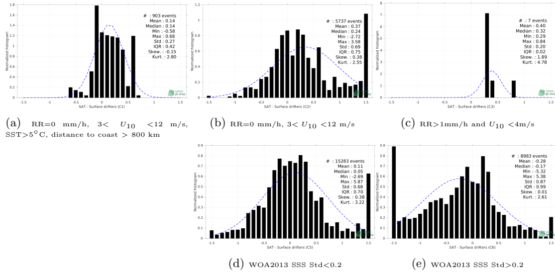
Figure 12: Normalized histogram of \Delta SSS (SMOS SSS L3 Arctic v3.1 - 9 Days (BEC) - Surface drifters) for 5 different subdatasets corresponding to: RR=0 mm/h, 3 < U_{10} < 12 m/s, SST > 5°C, distance to coast > 800 km (a), RR=0 mm/h, 3 < U_{10} < 12 m/s (b), RR > 1mm/h and U_{10} < 4 m/s (c), WOA2013 SSS Std < 0.2 (d), WOA2013 SSS Std > 0.2 (e).
