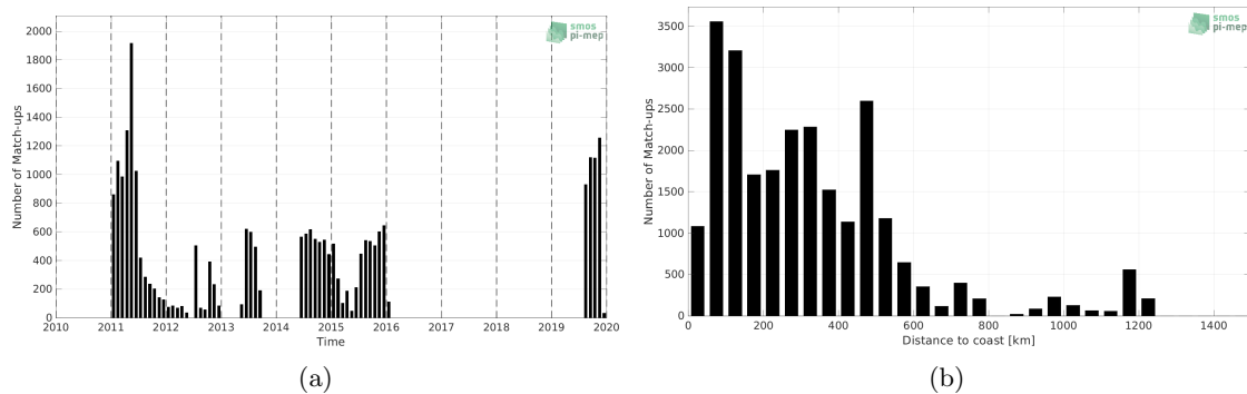
Figure 1: Number of match-ups between Surface drifters and SMOS SSS L3 Arctic v3.1 - 9 Days (BEC) SSS as a function of time (a) and as function of the distance to coast (b) over the Global Ocean Pi-MEP region and for the full satellite product period.
