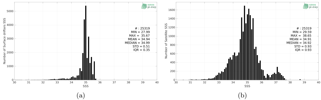
Figure 2: Histograms of SSS from Surface drifters (a) and SMOS SSS L3 Arctic v3.1 - 9 Days (BEC) (b) considering all match-up pairs per bins of 0.1 over the Global Ocean Pi-MEP region and for the full satellite product period.
