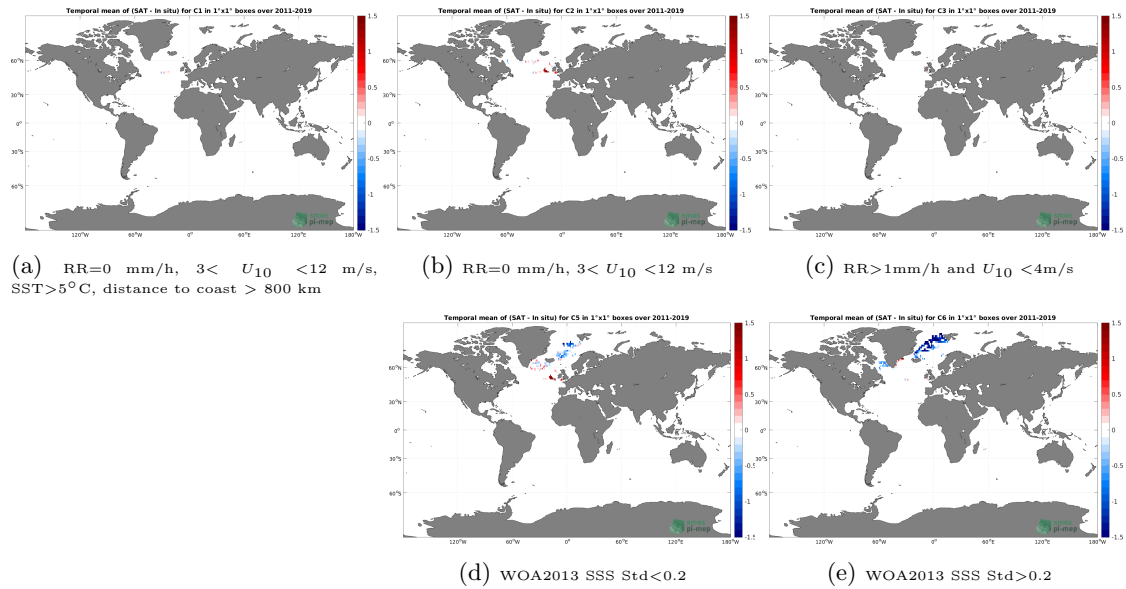
Figure 11: Temporal mean gridded over spatial boxes of size 1^{\circ}\times 1^{\circ} of \Delta\text{SSS} (SMOS SSS L3 Arctic v3.1 - 9 Days (BEC) - Surface drifters) for 5 different subdatasets corresponding to:RR=0 mm/h, 3 < U_{10} < 12 m/s, SST >5^{\circ}\text{C} , distance to coast > 800 km (a), RR=0 mm/h, 3 < U_{10} < 12 m/s (b), RR >1 mm/h and U_{10} < 4 m/s (c), WOA2013 SSS Std <0.2 (d), WOA2013 SSS Std >0.2 (e).
