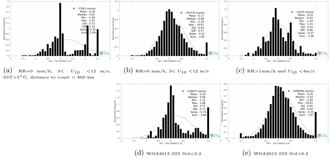
Figure 13: Normalized histogram of \Delta SSS (SMOS-L3-BEC-ARCTIC-OA-V2-9DAYS-0.25DEG - TSG-SAMOS) for 5 different subdatasets corresponding to: RR=0 mm/h, 3 < U_{10} < 12 m/s, SST>5°C, distance to coast > 800 km (a), RR=0 mm/h, 3 < U_{10} < 12 m/s (b), RR>1mm/h and U_{10} < 4 m/s (c), WOA2013 SSS Std<0.2 (d), WOA2013 SSS Std>0.2 (e).
