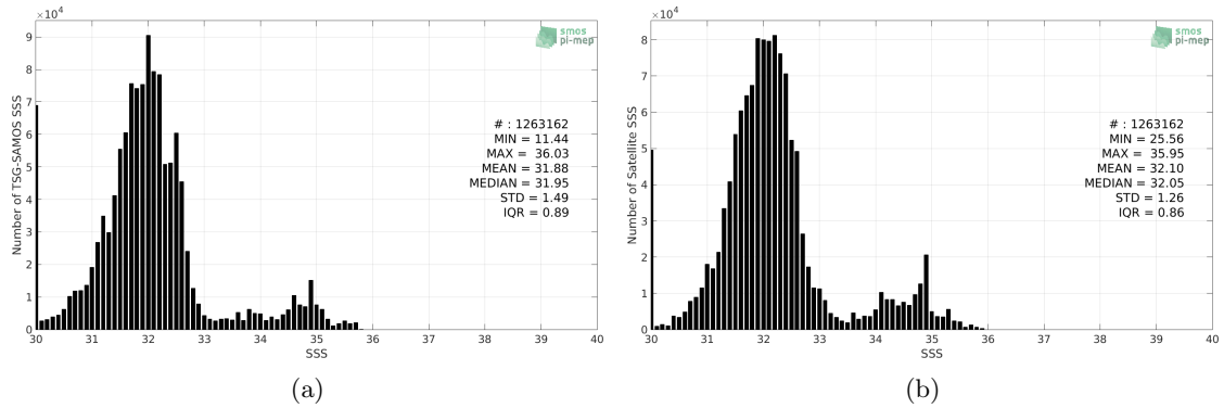
Figure 2: Histograms of SSS from TSG-SAMOS (a) and SMOS-L3-BEC-ARCTIC-OA-V2-9DAYS-0.25DEG (b) considering all match-up pairs per bins of 0.1 over the Global Ocean Pi-MEP region and for the full satellite product period.
