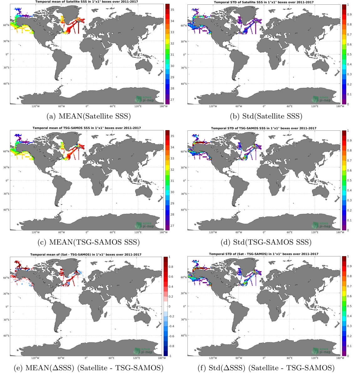
Figure 6: Temporal mean (left) and Std (right) of SSS from SMOS-L3-BEC-ARCTIC-OA-V2-9DAYS-0.25DEG (top), TSG-SAMOS (middle), and of \Delta SSS (Satellite - TSG-SAMOS). Only match-up pairs are used to generate these maps.
