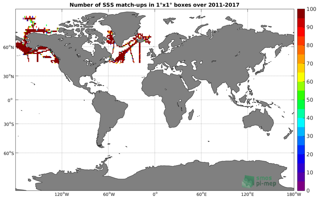
Figure 4: Number of SSS match-ups between TSG-SAMOS SSS and the SMOS-L3-BEC-ARCTIC-OA-V2-9DAYS-0.25DEG SSS product for the Global Ocean Pi-MEP region over 1^\circ \times 1^\circ boxes and for the full satellite product period.
