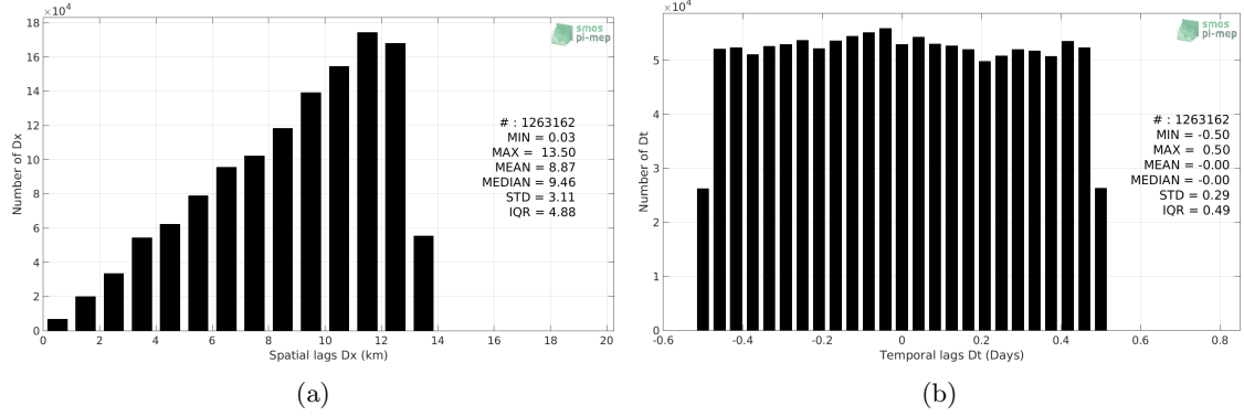
Figure 5: Histograms of the spatial (a) and temporal (b) lags between the time of the TSG-SAMOS measurements and the date of the corresponding SMOS-L3-BEC-ARCTIC-OA-V2-9DAYS-0.25DEG SSS product.
