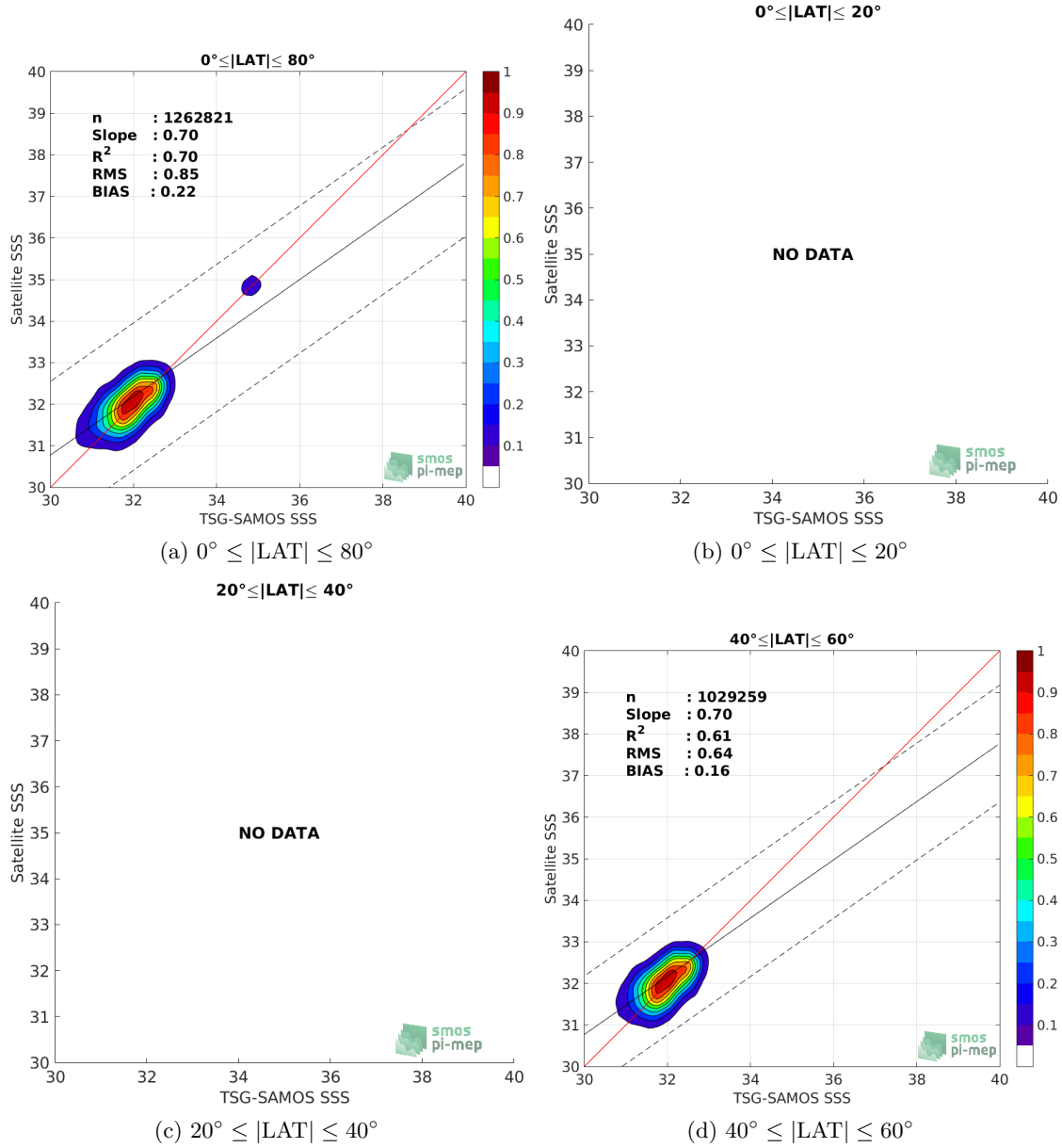
Figure 9: Contour maps of the concentration of SMOS-L3-BEC-ARCTIC-OA-V2-9DAYS-0.25DEG SSS (y-axis) versus TSG-SAMOS SSS (x-axis) at match-up pairs for different latitude bands. For each plot, the red line shows x=y . The black thin and dashed lines indicate a linear fit through the data cloud and the \pm 95\% confidence levels, respectively. The number match-up pairs n , the slope and R^2 coefficient of the linear fit, the root mean square (RMS) and the mean bias between satellite and in situ data are indicated for each latitude band in each plots.
