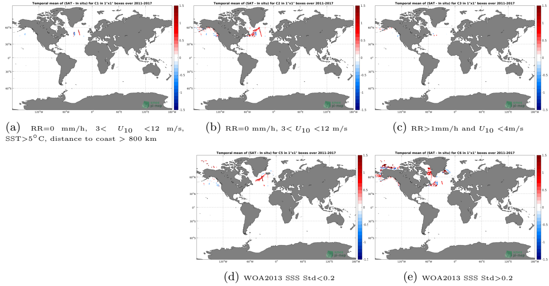
Figure 12: Temporal mean gridded over spatial boxes of size 1^\circ \times 1^\circ of \Delta SSS (SMOS-L3-BEC-ARCTIC-OA-V2-9DAYS-0.25DEG - TSG-SAMOS) for 5 different subdatasets corresponding to: RR=0 mm/h, 3 < U_{10} < 12 m/s, SST > 5^\circ C , distance to coast > 800 km (a), RR=0 mm/h, 3 < U_{10} < 12 m/s (b), RR > 1 mm/h and U_{10} < 4 m/s (c), WOA2013 SSS Std < 0.2 (d), WOA2013 SSS Std > 0.2 (e).
