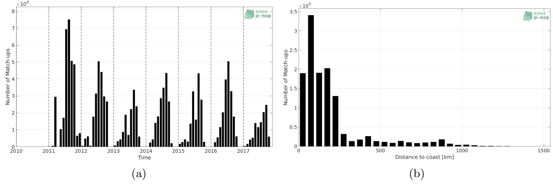
Figure 1: Number of match-ups between TSG-SAMOS and SMOS-L3-BEC-ARCTIC-OA-V2-9DAYS-0.25DEG SSS as a function of time (a) and as function of the distance to coast (b) over the Global Ocean Pi-MEP region and for the full satellite product period.
