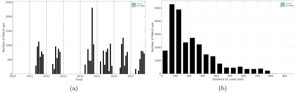
Figure 1: Number of match-ups between TSG-POLARSTERN and SMOS L3 Arctic OA v2 - 9 Days (BEC) SSS as a function of time (a) and as function of the distance to coast (b) over the Global Ocean Pi-MEP region and for the full satellite product period.
