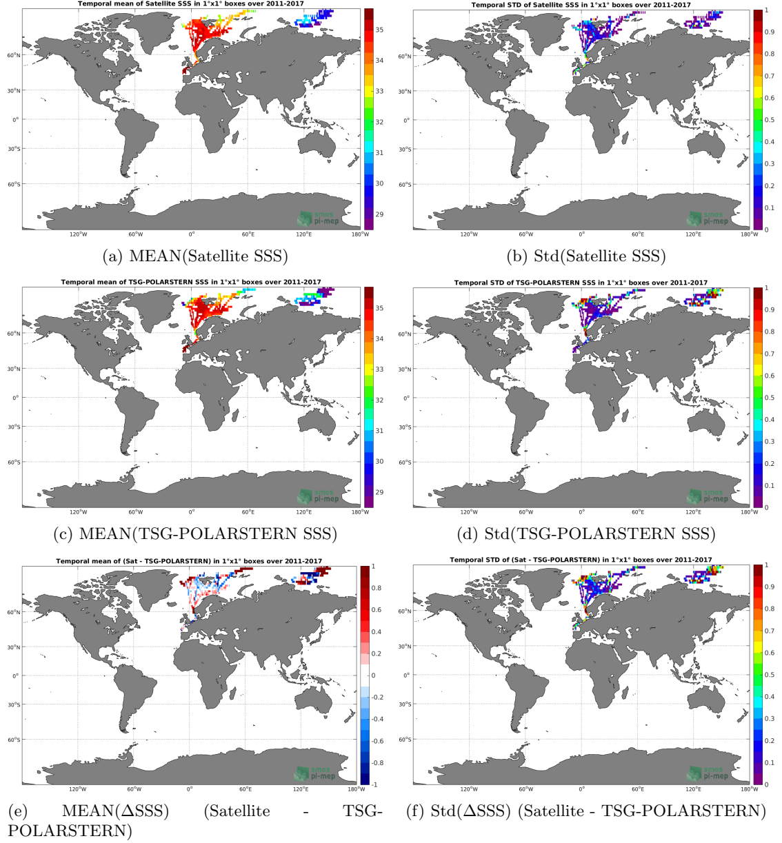
Figure 6: Temporal mean (left) and Std (right) of SSS from SMOS L3 Arctic OA v2 - 9 Days (BEC) (top), TSG-POLARSTERN (middle), and of \Delta SSS (Satellite - TSG-POLARSTERN). Only match-up pairs are used to generate these maps.
