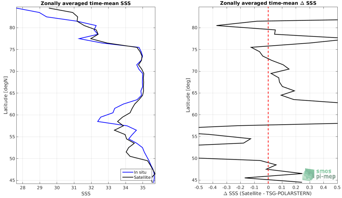
Figure 8: Left panel: Zonal mean SSS from SMOS L3 Arctic OA v2 - 9 Days (BEC) satellite product (black) and from TSG-POLARSTERN (blue). Right panel: Zonal mean of \Delta SSS (Satellite - TSG-POLARSTERN) for all the collected Pi-MEP match-up pairs estimated over the full satellite product period.
