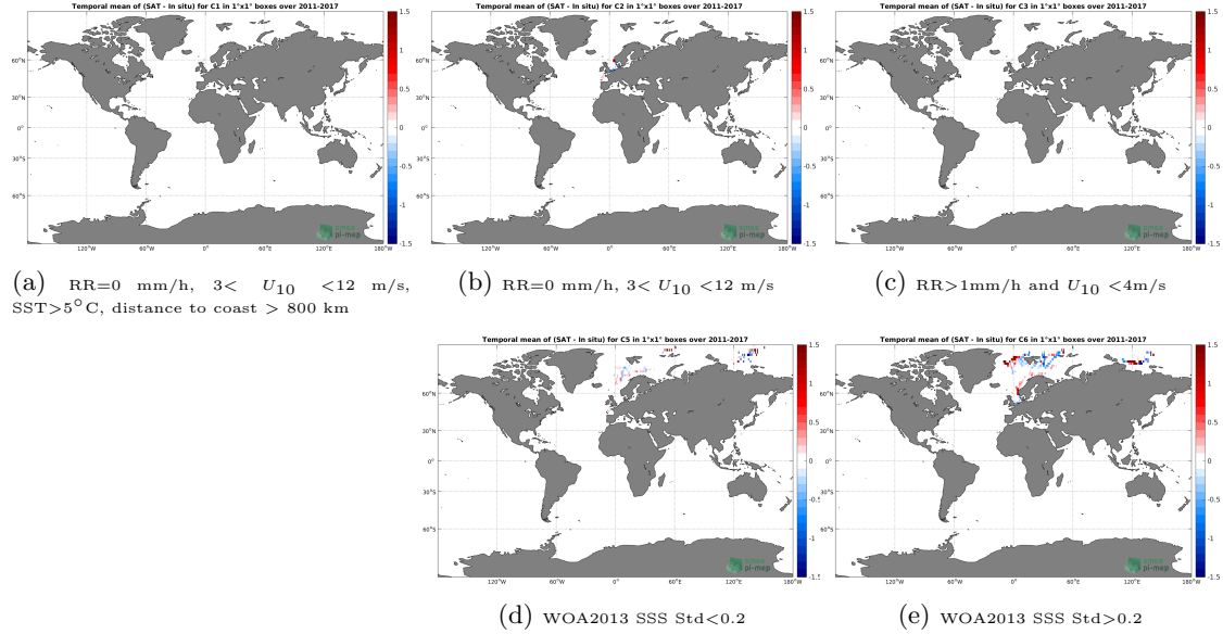
Figure 12: Temporal mean gridded over spatial boxes of size 1^{\circ}\times 1^{\circ} of \Delta\text{SSS} (SMOS L3 Arctic OA v2 - 9 Days (BEC) - TSG-POLARSTERN) for 5 different subdatasets corresponding to:RR=0 mm/h, 3 < U_{10} < 12 m/s, SST >5^{\circ}\text{C} , distance to coast > 800 km (a), RR=0 mm/h, 3 < U_{10} < 12 m/s (b), RR >1 mm/h and U_{10} < 4 m/s (c), WOA2013 SSS Std <0.2 (d), WOA2013 SSS Std >0.2 (e).
