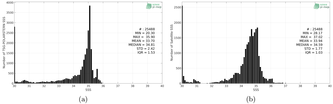
Figure 2: Histograms of SSS from TSG-POLARSTERN (a) and SMOS L3 Arctic OA v2 - 9 Days (BEC) (b) considering all match-up pairs per bins of 0.1 over the Global Ocean Pi-MEP region and for the full satellite product period.
