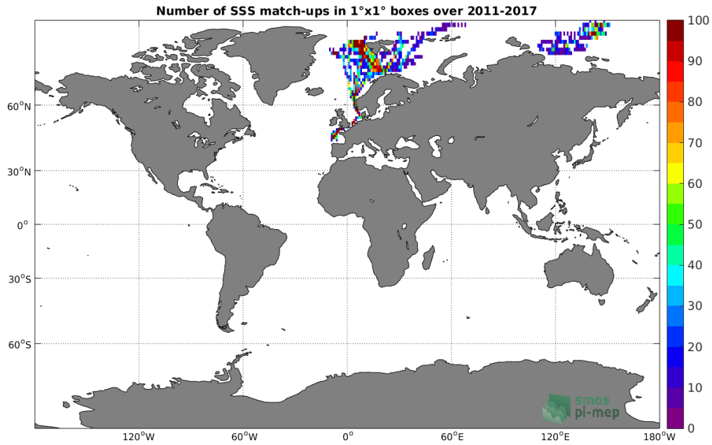
Figure 4: Number of SSS match-ups between TSG-POLARSTERN SSS and the SMOS L3 Arctic OA v2 - 9 Days (BEC) SSS product for the Global Ocean Pi-MEP region over 1°x1° boxes and for the full satellite product period.
