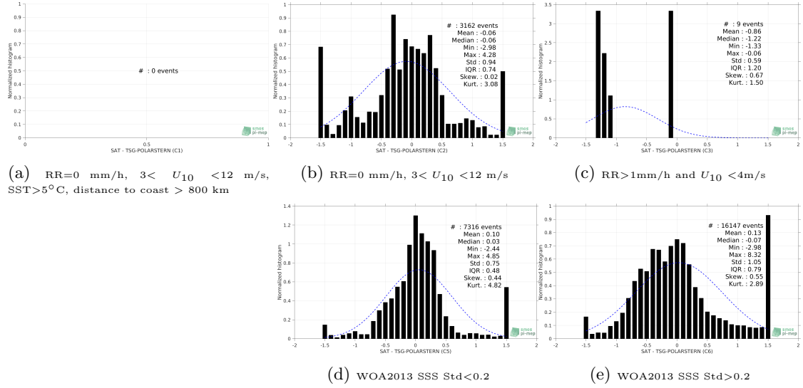
Figure 13: Normalized histogram of \Delta SSS (SMOS L3 Arctic OA v2 - 9 Days (BEC) - TSG-POLARSTERN) for 5 different subdatasets corresponding to: RR=0 mm/h, 3 < U_{10} < 12 m/s, SST>5°C, distance to coast > 800 km (a), RR=0 mm/h, 3 < U_{10} < 12 m/s (b), RR>1mm/h and U_{10} < 4 m/s (c), WOA2013 SSS Std<0.2 (d), WOA2013 SSS Std>0.2 (e).
