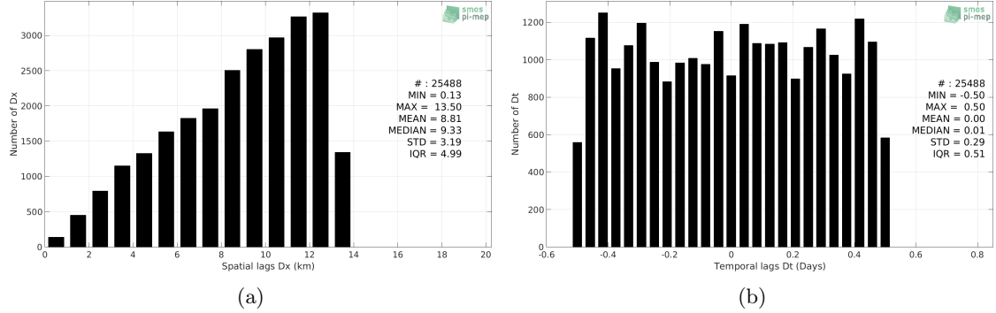
Figure 5: Histograms of the spatial (a) and temporal (b) lags between the time of the TSG-POLARSTERN measurements and the date of the corresponding SMOS L3 Arctic OA v2 - 9 Days (BEC) SSS product.
