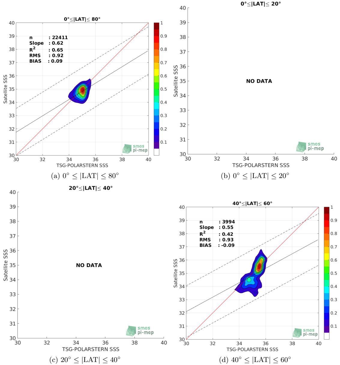
Figure 9: Contour maps of the concentration of SMOS L3 Arctic OA v2 - 9 Days (BEC) SSS (y-axis) versus TSG-POLARSTERN SSS (x-axis) at match-up pairs for different latitude bands. For each plot, the red line shows x=y . The black thin and dashed lines indicate a linear fit through the data cloud and the \pm 95\% confidence levels, respectively. The number match-up pairs n , the slope and R^2 coefficient of the linear fit, the root mean square (RMS) and the mean bias between satellite and in situ data are indicated for each latitude band in each plots.
