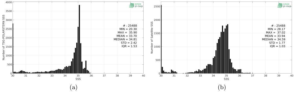
Figure 2: Histograms of SSS from TSG-POLARSTERN (a) and SMOS-L3-BEC-ARCTIC-OA-V2-9DAYS-0.25DEG (b) considering all match-up pairs per bins of 0.1 over the Global Ocean Pi-MEP region and for the full satellite product period.
