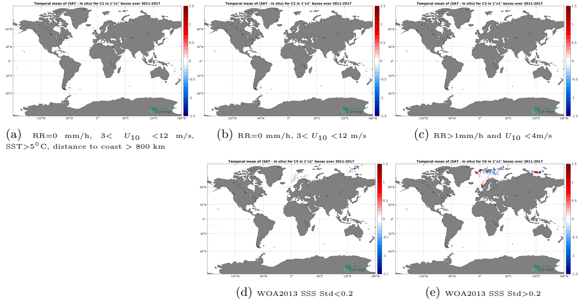
Figure 12: Temporal mean gridded over spatial boxes of size 1^\circ \times 1^\circ of \Delta SSS (SMOS-L3-BEC-ARCTIC-OA-V2-9DAYS-0.25DEG - TSG-POLARSTERN) for 5 different subdatasets corresponding to: RR=0 mm/h, 3 < U_{10} < 12 m/s, SST > 5^\circ C , distance to coast > 800 km (a), RR=0 mm/h, 3 < U_{10} < 12 m/s (b), RR > 1 mm/h and U_{10} < 4 m/s (c), WOA2013 SSS Std < 0.2 (d), WOA2013 SSS Std > 0.2 (e).
