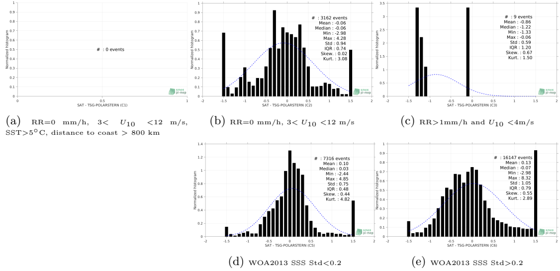
Figure 13: Normalized histogram of \Delta\text{SSS} (SMOS-L3-BEC-ARCTIC-OA-V2-9DAYS-0.25DEG - TSG-POLARSTERN) for 5 different subdatasets corresponding to: RR=0 mm/h, 3 < U_{10} < 12 m/s, SST > 5^{\circ}\text{C} , distance to coast > 800 km (a), RR=0 mm/h, 3 < U_{10} < 12 m/s (b), RR > 1\text{mm/h} and U_{10} < 4\text{m/s} (c), WOA2013 SSS Std<0.2 (d), WOA2013 SSS Std>0.2 (e).
