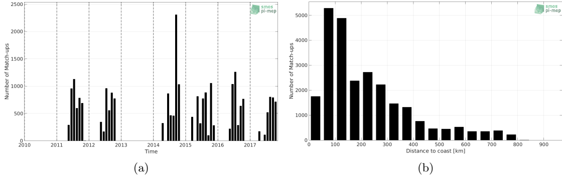
Figure 1: Number of match-ups between TSG-POLARSTERN and SMOS-L3-BEC-ARCTIC-OA-V2-9DAYS-0.25DEG SSS as a function of time (a) and as function of the distance to coast (b) over the Global Ocean Pi-MEP region and for the full satellite product period.
