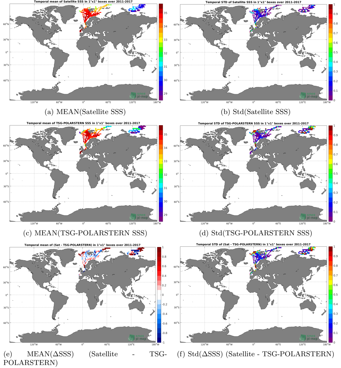
Figure 6: Temporal mean (left) and Std (right) of SSS from SMOS-L3-BEC-ARCTIC-OA-V2-9DAYS-0.25DEG (top), TSG-POLARSTERN (middle), and of \Delta SSS (Satellite - TSG-POLARSTERN). Only match-up pairs are used to generate these maps.
