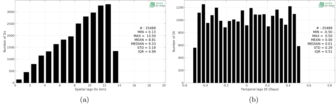
Figure 5: Histograms of the spatial (a) and temporal (b) lags between the time of the TSG-POLARSTERN measurements and the date of the corresponding SMOS-L3-BEC-ARCTIC-OA-V2-9DAYS-0.25DEG SSS product.
