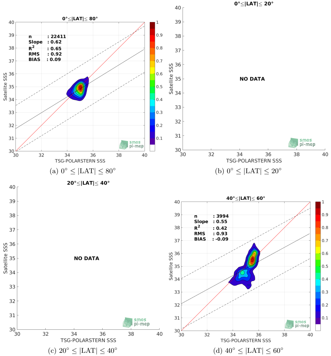
Figure 9: Contour maps of the concentration of SMOS-L3-BEC-ARCTIC-OA-V2-9DAYS-0.25DEG SSS (y-axis) versus TSG-POLARSTERN SSS (x-axis) at match-up pairs for different latitude bands. For each plot, the red line shows x=y . The black thin and dashed lines indicate a linear fit through the data cloud and the \pm 95\% confidence levels, respectively. The number of match-up pairs n , the slope and R^2 coefficient of the linear fit, the root mean square (RMS) and the mean bias between satellite and in situ data are indicated for each latitude band in each plot.
