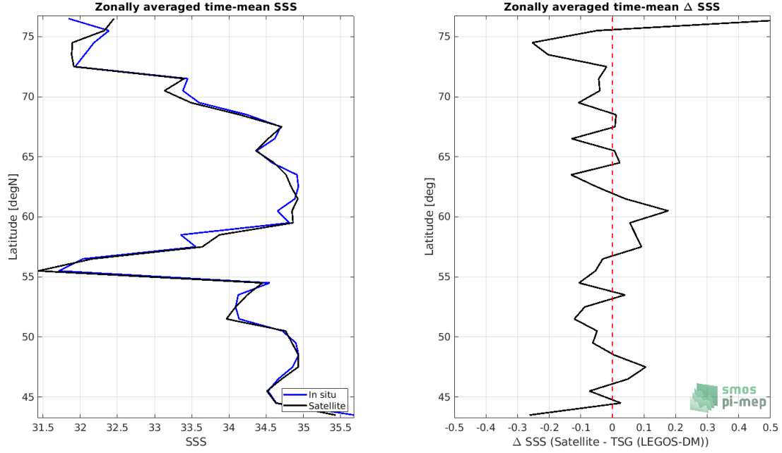
Figure 8: Left panel: Zonal mean SSS from SMOS SSS L3 Arctic OA v2 - 9 Days (BEC) satellite product (black) and from TSG (LEGOS-DM) (blue). Right panel: Zonal mean of \Delta SSS (Satellite - TSG (LEGOS-DM)) for all the collected Pi-MEP match-up pairs estimated over the full satellite product period.
