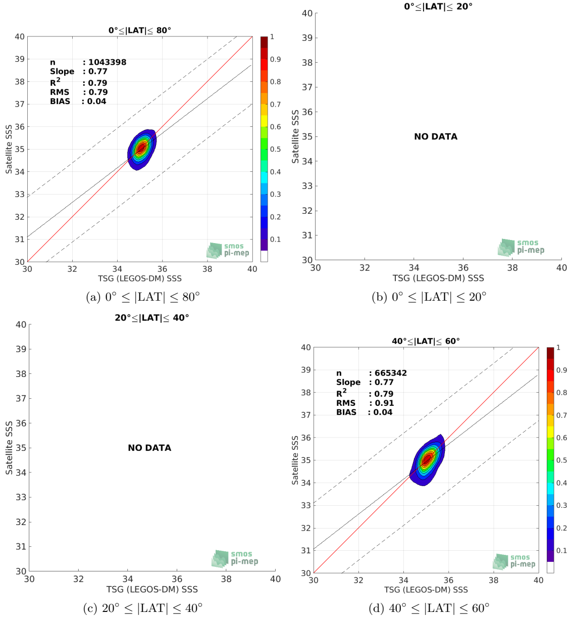
Figure 9: Contour maps of the concentration of SMOS SSS L3 Arctic OA v2 - 9 Days (BEC) SSS (y-axis) versus TSG (LEGOS-DM) SSS (x-axis) at match-up pairs for different latitude bands. For each plot, the red line shows x=y . The black thin and dashed lines indicate a linear fit through the data cloud and the \pm 95\% confidence levels, respectively. The number match-up pairs n , the slope and R^2 coefficient of the linear fit, the root mean square (RMS) and the mean bias between satellite and in situ data are indicated for each latitude band in each plots.
