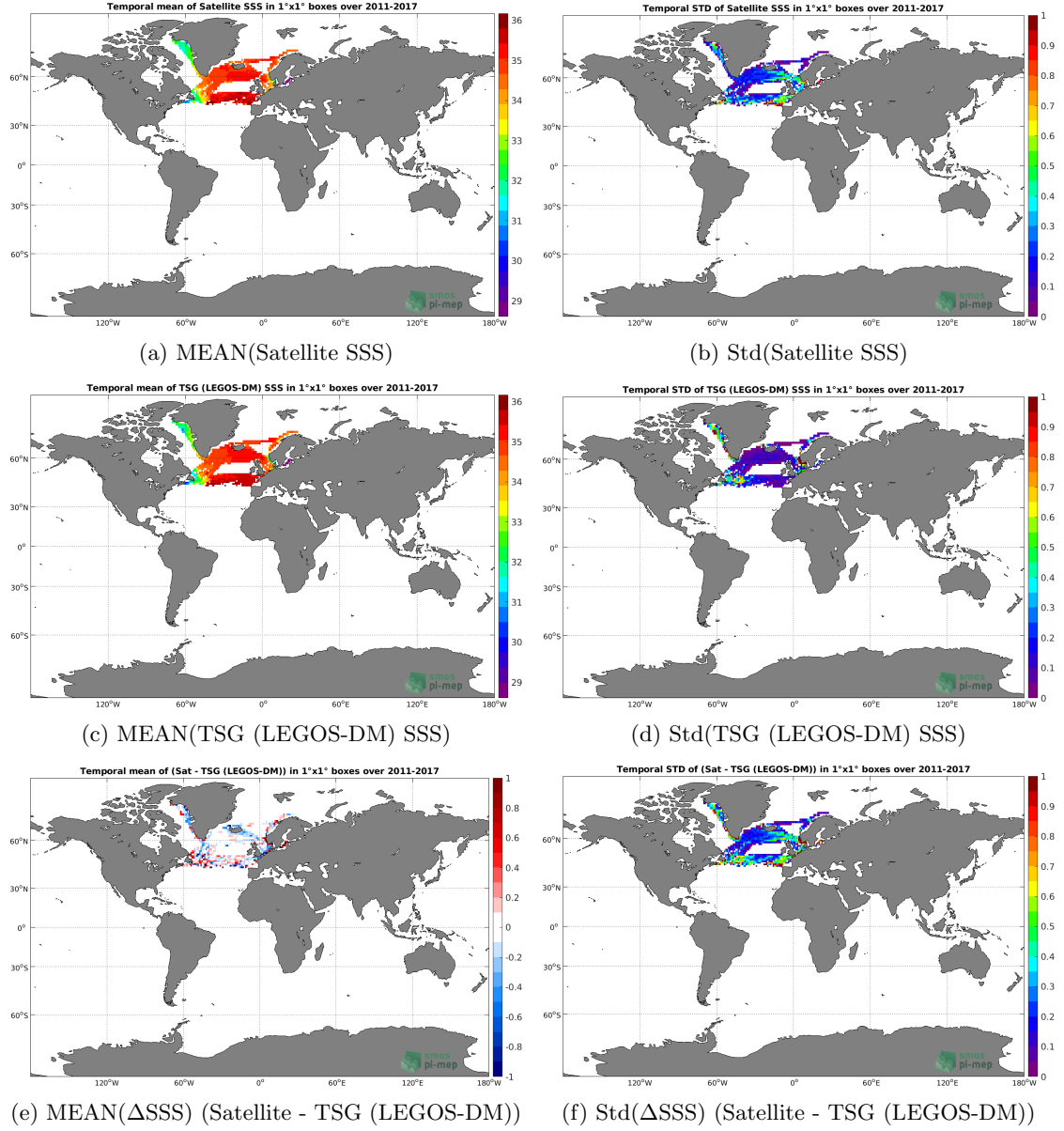
Figure 6: Temporal mean (left) and Std (right) of SSS from SMOS SSS L3 Arctic OA v2 - 9 Days (BEC) (top), TSG (LEGOS-DM) (middle), and of \Delta SSS (Satellite - TSG (LEGOS-DM)). Only match-up pairs are used to generate these maps.
