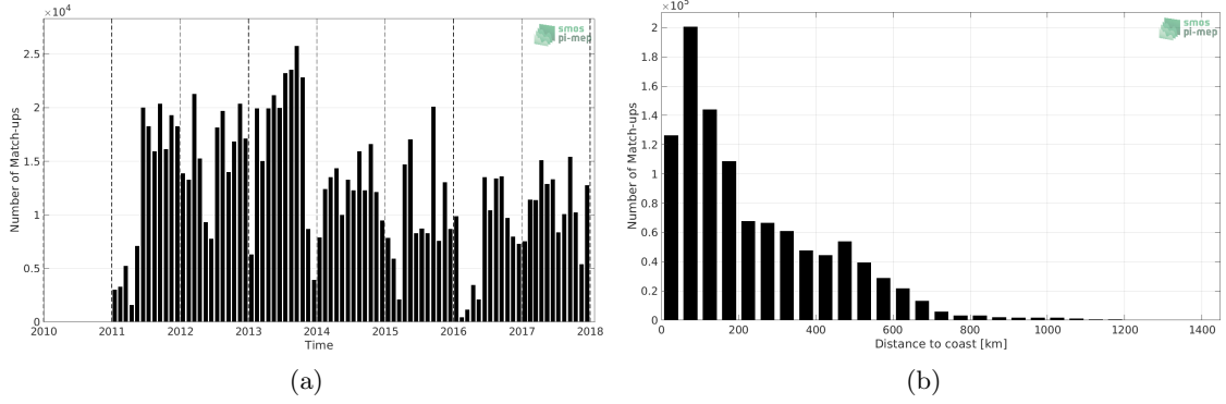
Figure 1: Number of match-ups between TSG (LEGOS-DM) and SMOS SSS L3 Arctic OA v2 - 9 Days (BEC) SSS as a function of time (a) and as function of the distance to coast (b) over the Global Ocean Pi-MEP region and for the full satellite product period.
