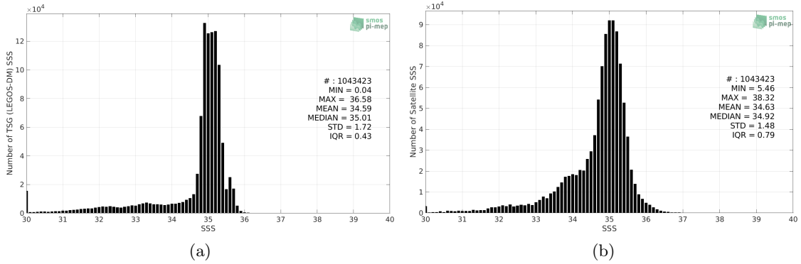
Figure 2: Histograms of SSS from TSG (LEGOS-DM) (a) and SMOS SSS L3 Arctic OA v2 - 9 Days (BEC) (b) considering all match-up pairs per bins of 0.1 over the Global Ocean Pi-MEP region and for the full satellite product period.
