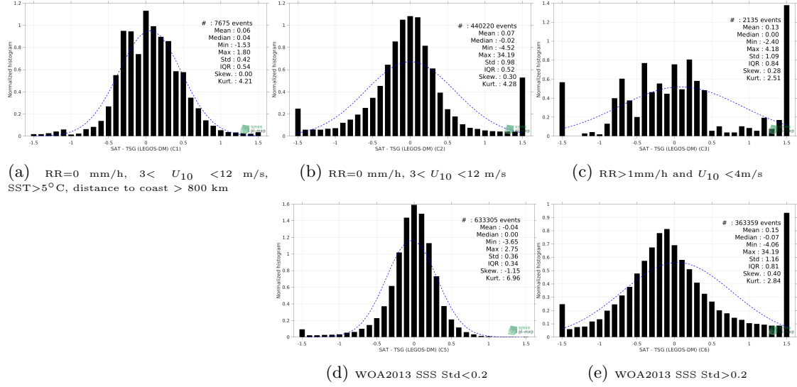
Figure 13: Normalized histogram of \Delta SSS (SMOS SSS L3 Arctic OA v2 - 9 Days (BEC) - TSG (LEGOS-DM)) for 5 different subdatasets corresponding to: RR=0 mm/h, 3 < U_{10} < 12 m/s, SST>5°C, distance to coast > 800 km (a), RR=0 mm/h, 3 < U_{10} < 12 m/s (b), RR>1mm/h and U_{10} < 4 m/s (c), WOA2013 SSS Std<0.2 (d), WOA2013 SSS Std>0.2 (e).
