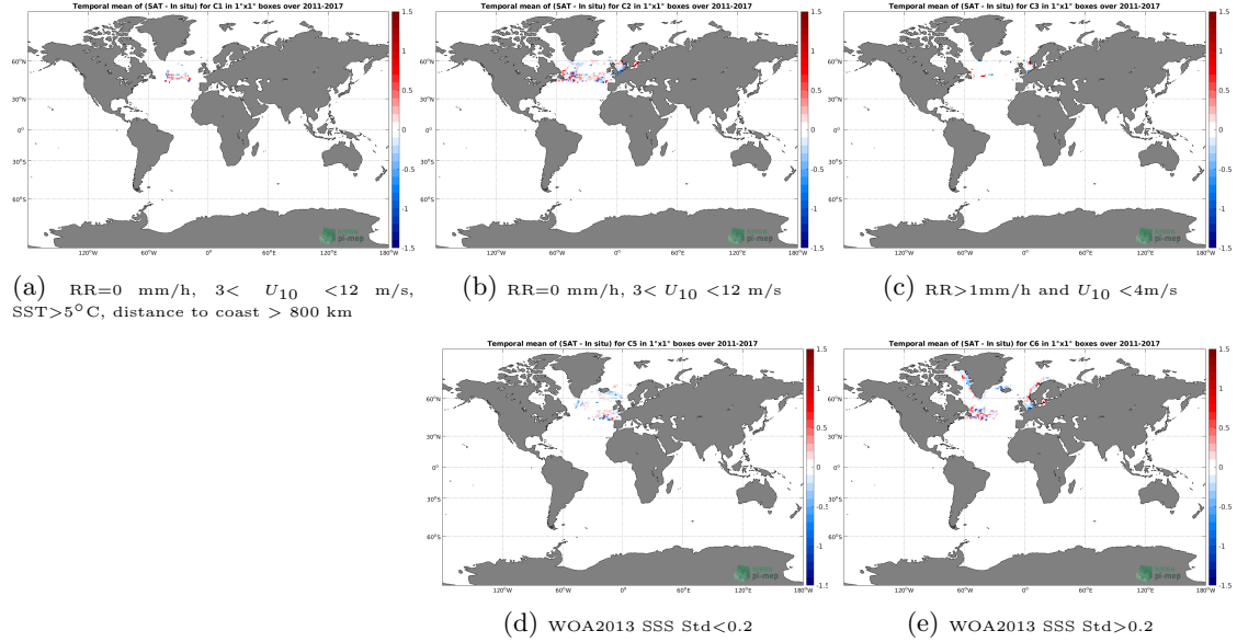
Figure 12: Temporal mean gridded over spatial boxes of size 1^{\circ}\times 1^{\circ} of \Delta\text{SSS} (SMOS SSS L3 Arctic OA v2 - 9 Days (BEC) - TSG (LEGOS-DM)) for 5 different subdatasets corresponding to: \text{RR}=0 mm/h, 3 < U_{10} < 12 m/s, \text{SST} > 5^{\circ}\text{C} , distance to coast > 800 km (a), \text{RR}=0 mm/h, 3 < U_{10} < 12 m/s (b), \text{RR} > 1\text{mm/h} and U_{10} < 4\text{m/s} (c), WOA2013 SSS Std < 0.2 (d), WOA2013 SSS Std > 0.2 (e).
