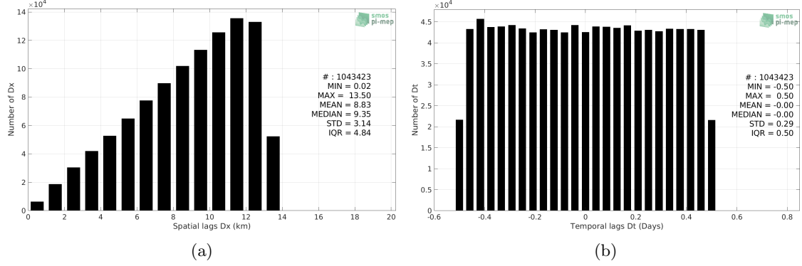
Figure 5: Histograms of the spatial (a) and temporal (b) lags between the location/time of the TSG (LEGOS-DM) measurement and the date of the corresponding SMOS SSS L3 Arctic OA v2 - 9 Days (BEC) SSS pixel.
