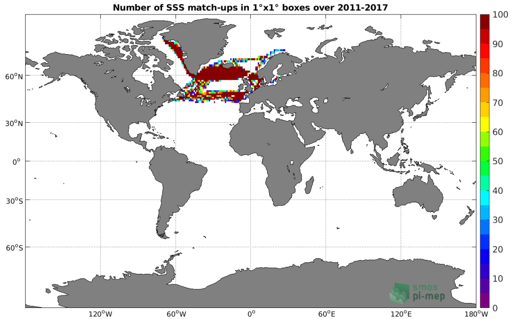
Figure 4: Number of SSS match-ups between TSG (LEGOS-DM) SSS and the SMOS SSS L3 Arctic OA v2 - 9 Days (BEC) SSS product for the Global Ocean Pi-MEP region over 1^\circ \times 1^\circ boxes and for the full satellite product period.
