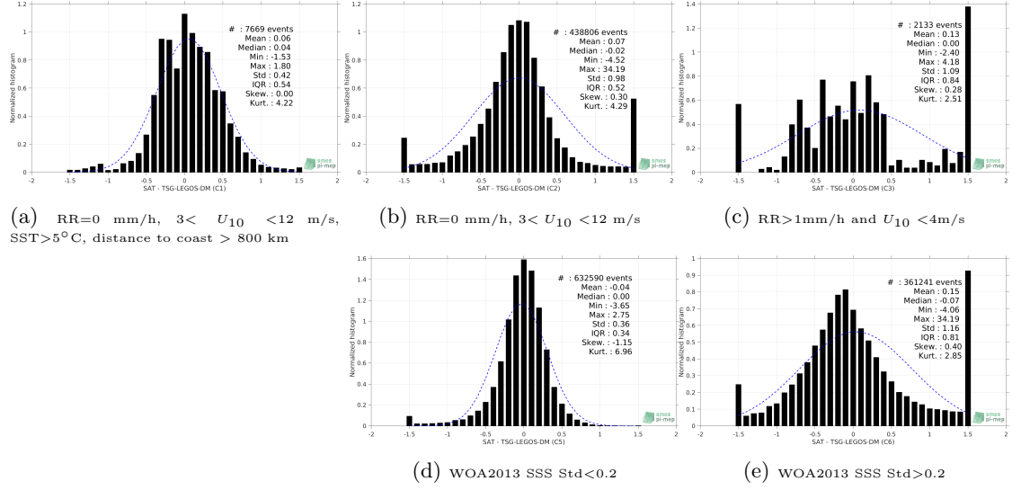
Figure 13: Normalized histogram of \Delta SSS (SMOS L3 Arctic OA v2 - 9 Days (BEC) - TSG-LEGOS-DM) for 5 different subdatasets corresponding to: RR=0 mm/h, 3 < U_{10} < 12 m/s, SST>5°C, distance to coast > 800 km (a), RR=0 mm/h, 3 < U_{10} < 12 m/s (b), RR>1mm/h and U_{10} < 4 m/s (c), WOA2013 SSS Std<0.2 (d), WOA2013 SSS Std>0.2 (e).
