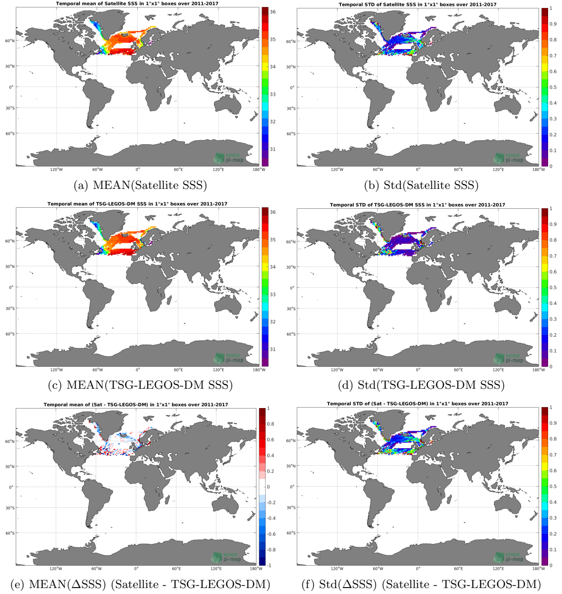
Figure 6: Temporal mean (left) and Std (right) of SSS from SMOS L3 Arctic OA v2 - 9 Days (BEC) (top), TSG-LEGOS-DM (middle), and of \Delta SSS (Satellite - TSG-LEGOS-DM). Only match-up pairs are used to generate these maps.
