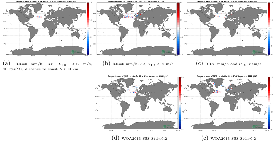
Figure 12: Temporal mean gridded over spatial boxes of size 1^{\circ}\times 1^{\circ} of \Delta\text{SSS} (SMOS L3 Arctic OA v2 - 9 Days (BEC) - TSG-LEGOS-DM) for 5 different subdatasets corresponding to:RR=0 mm/h, 3 < U_{10} < 12 m/s, SST >5^{\circ}\text{C} , distance to coast > 800 km (a), RR=0 mm/h, 3 < U_{10} < 12 m/s (b), RR >1 mm/h and U_{10} < 4 m/s (c), WOA2013 SSS Std <0.2 (d), WOA2013 SSS Std >0.2 (e).
