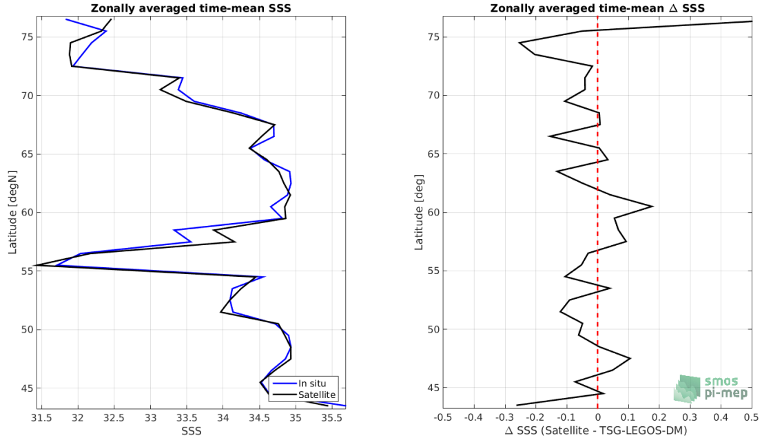
Figure 8: Left panel: Zonal mean SSS from SMOS L3 Arctic OA v2 - 9 Days (BEC) satellite product (black) and from TSG-LEGOS-DM (blue). Right panel: Zonal mean of \Delta SSS (Satellite - TSG-LEGOS-DM) for all the collected Pi-MEP match-up pairs estimated over the full satellite product period.
