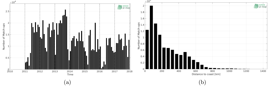
Figure 1: Number of match-ups between TSG-LEGOS-DM and SMOS L3 Arctic OA v2 - 9 Days (BEC) SSS as a function of time (a) and as function of the distance to coast (b) over the Global Ocean Pi-MEP region and for the full satellite product period.
