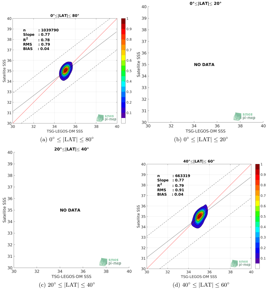
Figure 9: Contour maps of the concentration of SMOS L3 Arctic OA v2 - 9 Days (BEC) SSS (y-axis) versus TSG-LEGOS-DM SSS (x-axis) at match-up pairs for different latitude bands. For each plot, the red line shows x=y . The black thin and dashed lines indicate a linear fit through the cloud and the \pm 95\% confidence levels, respectively. The number match-up pairs n , the slope and R^2 coefficient of the linear fit, the root mean square (RMS) and the mean bias between satellite and in situ data are indicated for each latitude band in each plots.
