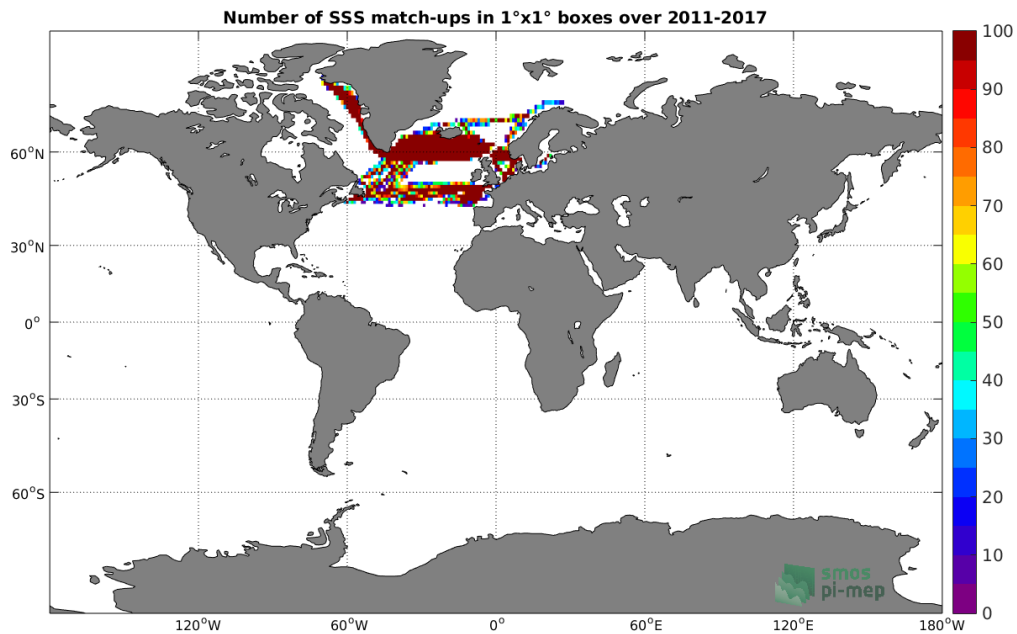
Figure 4: Number of SSS match-ups between TSG-LEGOS-DM SSS and the SMOS L3 Arctic OA v2 - 9 Days (BEC) SSS product for the Global Ocean Pi-MEP region over 1^\circ \times 1^\circ boxes and for the full satellite product period.
