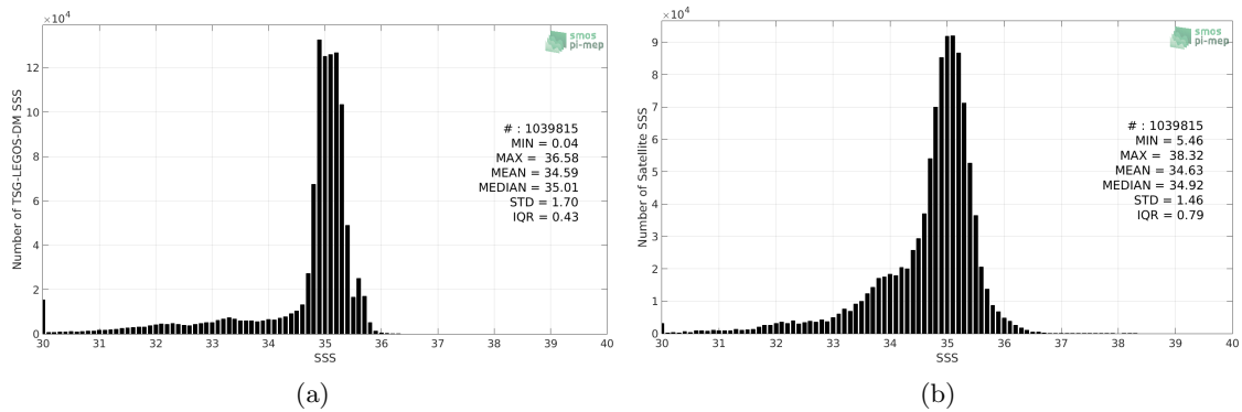
Figure 2: Histograms of SSS from TSG-LEGOS-DM (a) and SMOS L3 Arctic OA v2 - 9 Days (BEC) (b) considering all match-up pairs per bins of 0.1 over the Global Ocean Pi-MEP region and for the full satellite product period.
