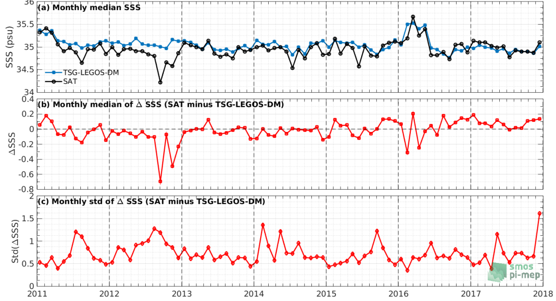
Figure 7: Time series of the monthly median SSS (top), median of \Delta\text{SSS} (Satellite - TSG-LEGOS-DM) and Std of \Delta\text{SSS} (Satellite - TSG-LEGOS-DM) over the Global Ocean Pi-MEP region considering all match-ups collected by the Pi-MEP.
