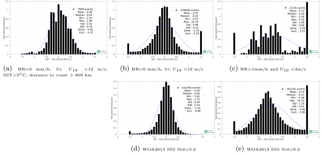
Figure 13: Normalized histogram of \Delta SSS (SMOS-L3-BEC-ARCTIC-OA-V2-9DAYS-0.25DEG - TSG-LEGOS-DM) for 5 different subdatasets corresponding to: RR=0 mm/h, 3 < U_{10} < 12 m/s, SST>5°C, distance to coast > 800 km (a), RR=0 mm/h, 3 < U_{10} < 12 m/s (b), RR>1mm/h and U_{10} < 4 m/s (c), WOA2013 SSS Std<0.2 (d), WOA2013 SSS Std>0.2 (e).
