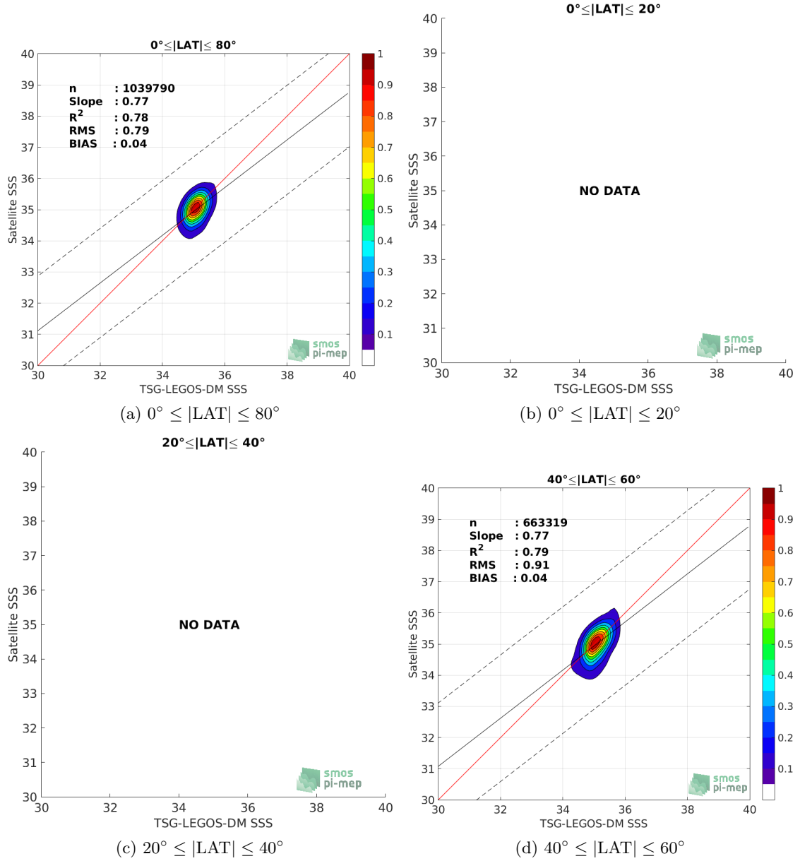
Figure 9: Contour maps of the concentration of SMOS-L3-BEC-ARCTIC-OA-V2-9DAYS-0.25DEG SSS (y-axis) versus TSG-LEGOS-DM SSS (x-axis) at match-up pairs for different latitude bands. For each plot, the red line shows x=y . The black thin and dashed lines indicate a linear fit through the data cloud and the \pm 95\% confidence levels, respectively. The number match-up pairs n , the slope and R^2 coefficient of the linear fit, the root mean square (RMS) and the mean bias between satellite and in situ data are indicated for each latitude band in each plots.
