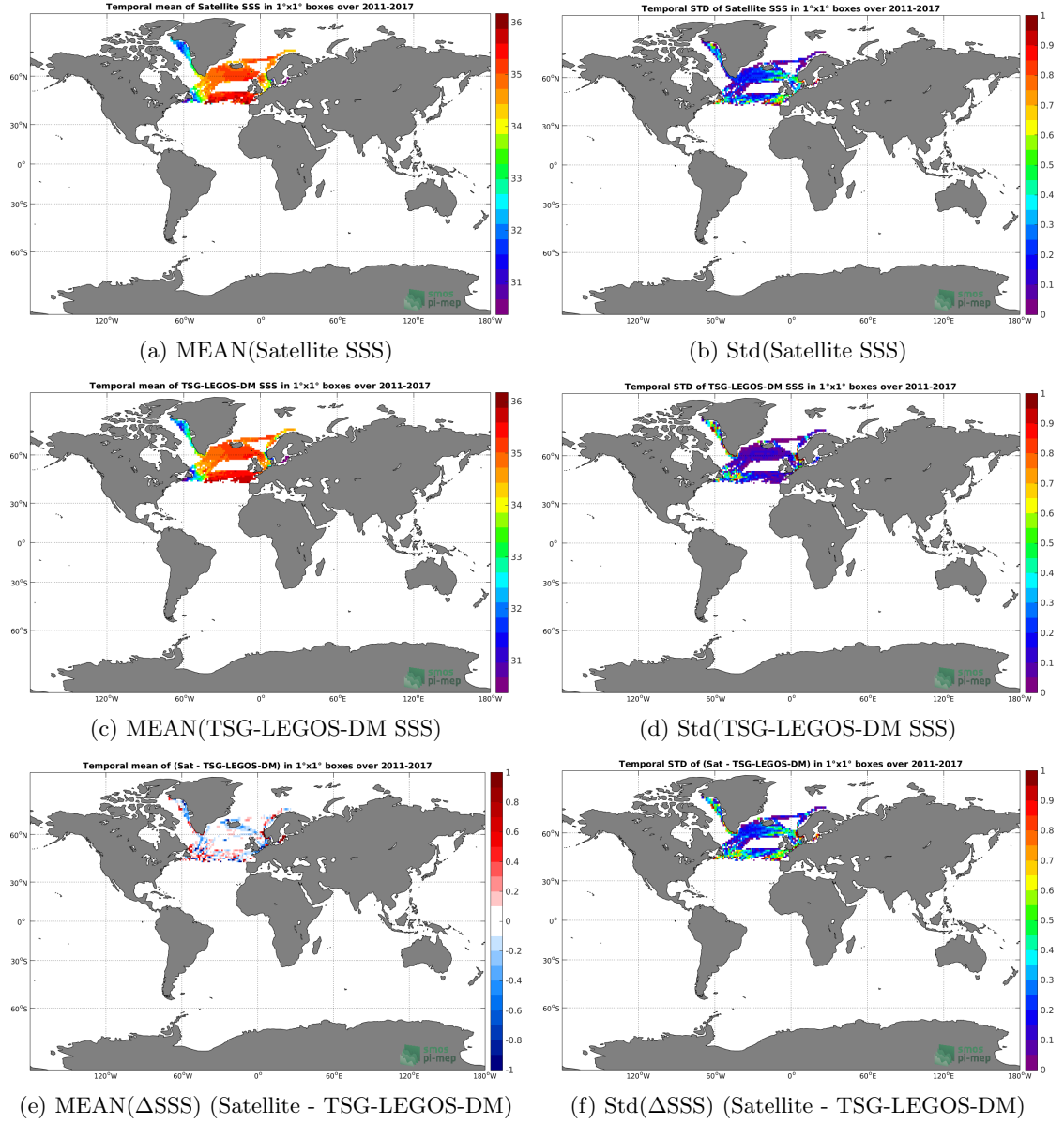
Figure 6: Temporal mean (left) and Std (right) of SSS from SMOS-L3-BEC-ARCTIC-OA-V2-9DAYS-0.25DEG (top), TSG-LEGOS-DM (middle), and of \Delta SSS (Satellite - TSG-LEGOS-DM). Only match-up pairs are used to generate these maps.
