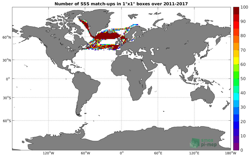
Figure 4: Number of SSS match-ups between TSG-LEGOS-DM SSS and the SMOS-L3-BEC-ARCTIC-OA-V2-9DAYS-0.25DEG SSS product for the Global Ocean Pi-MEP region over 1^\circ \times 1^\circ boxes and for the full satellite product period.
