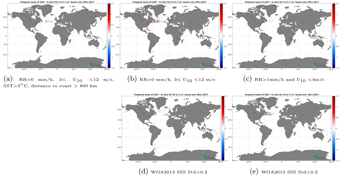
Figure 12: Temporal mean gridded over spatial boxes of size 1^\circ \times 1^\circ of \Delta SSS (SMOS-L3-BEC-ARCTIC-OA-V2-9DAYS-0.25DEG - TSG-LEGOS-DM) for 5 different subdatasets corresponding to: RR=0 mm/h, 3 < U_{10} < 12 m/s, SST >5^\circ C, distance to coast > 800 km (a), RR=0 mm/h, 3 < U_{10} < 12 m/s (b), RR >1 mm/h and U_{10} < 4 m/s (c), WOA2013 SSS Std <0.2 (d), WOA2013 SSS Std >0.2 (e).
