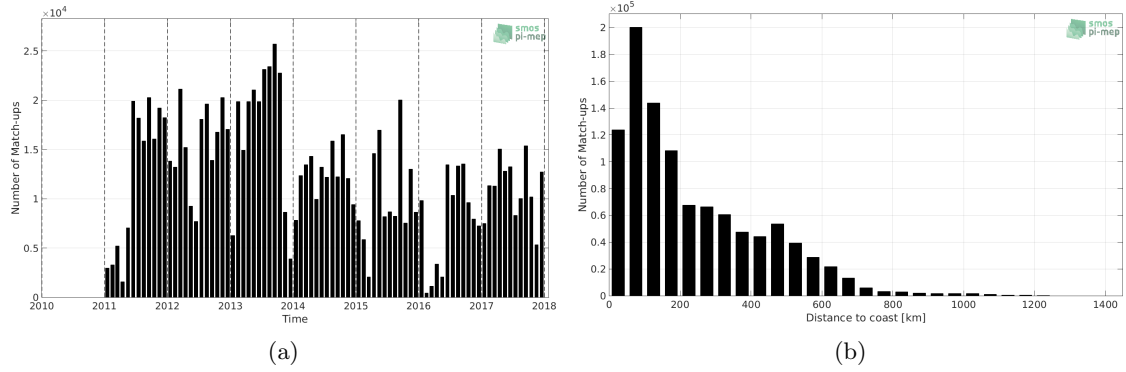
Figure 1: Number of match-ups between TSG-LEGOS-DM and SMOS-L3-BEC-ARCTIC-OA-V2-9DAYS-0.25DEG SSS as a function of time (a) and as function of the distance to coast (b) over the Global Ocean Pi-MEP region and for the full satellite product period.
