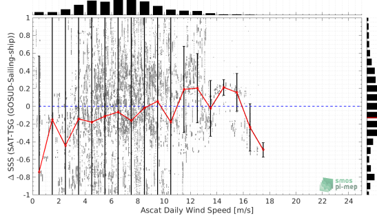
(c) ASCAT Wind Speed
