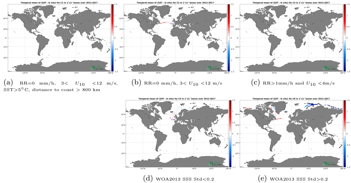
Figure 12: Temporal mean gridded over spatial boxes of size 1^\circ \times 1^\circ of \Delta SSS (SMOS SSS L3 Arctic OA v2 - 9 Days (BEC) - TSG (GOSUD-Sailing-ship)) for 5 different subdatasets corresponding to: RR=0 mm/h, 3 < U_{10} < 12 m/s, SST >5^\circ\text{C} , distance to coast > 800 km (a), RR=0 mm/h, 3 < U_{10} < 12 m/s (b), RR >1 mm/h and U_{10} < 4 m/s (c), WOA2013 SSS Std <0.2 (d), WOA2013 SSS Std >0.2 (e).
