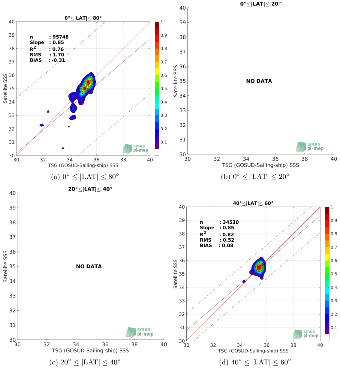
Figure 9: Contour maps of the concentration of SMOS SSS L3 Arctic OA v2 - 9 Days (BEC) SSS (y-axis) versus TSG (GOSUD-Sailing-ship) SSS (x-axis) at match-up pairs for different latitude bands. For each plot, the red line shows x=y . The black thin and dashed lines indicate a linear fit through the data cloud and the \pm 95\% confidence levels, respectively. The number match-up pairs n , the slope and R^2 coefficient of the linear fit, the root mean square (RMS) and the mean bias between satellite and in situ data are indicated for each latitude band in each plots.
