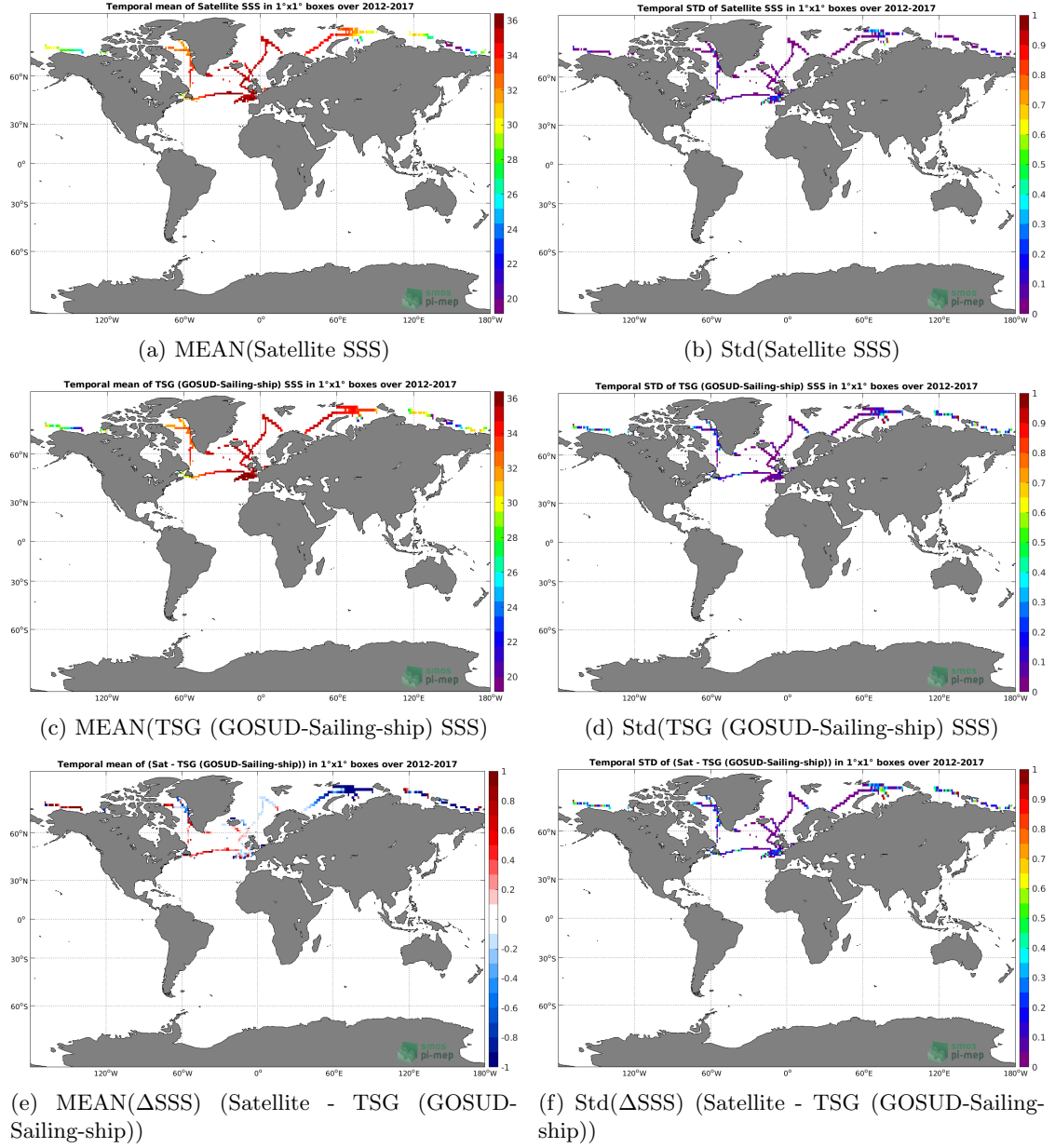
Figure 6: Temporal mean (left) and Std (right) of SSS from SMOS SSS L3 Arctic OA v2 - 9 Days (BEC) (top), TSG (GOSUD-Sailing-ship) (middle), and of \Delta SSS (Satellite - TSG (GOSUD-Sailing-ship)). Only match-up pairs are used to generate these maps.
