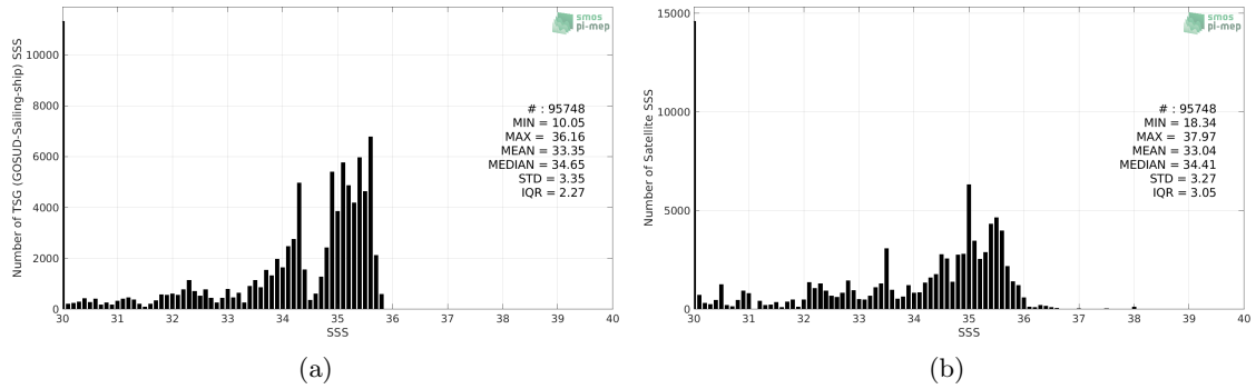
Figure 2: Histograms of SSS from TSG (GOSUD-Sailing-ship) (a) and SMOS SSS L3 Arctic OA v2 - 9 Days (BEC) (b) considering all match-up pairs per bins of 0.1 over the Global Ocean Pi-MEP region and for the full satellite product period.
