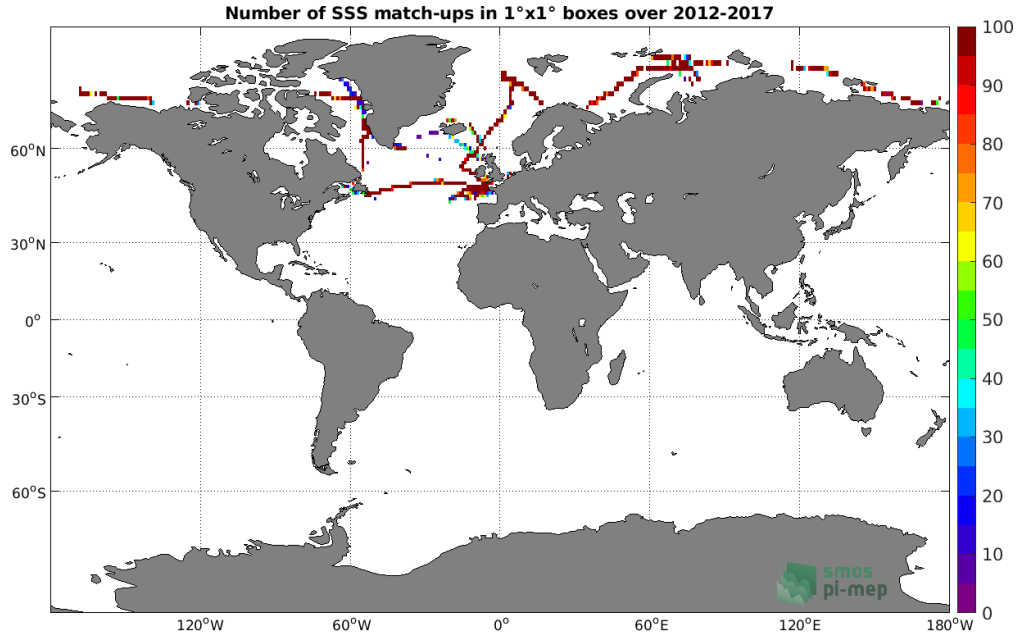
Figure 4: Number of SSS match-ups between TSG (GOSUD-Sailing-ship) SSS and the SMOS SSS L3 Arctic OA v2 - 9 Days (BEC) SSS product for the Global Ocean Pi-MEP region over 1^\circ \times 1^\circ boxes and for the full satellite product period.
