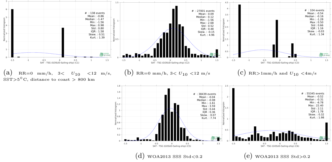
Figure 13: Normalized histogram of \Delta\text{SSS} (SMOS SSS L3 Arctic OA v2 - 9 Days (BEC) - TSG (GOSUD-Sailing-ship)) for 5 different subdatasets corresponding to: RR=0 mm/h, 3 < U_{10} < 12 m/s, SST>5°C, distance to coast > 800 km (a), RR=0 mm/h, 3 < U_{10} < 12 m/s (b), RR>1mm/h and U_{10} < 4 m/s (c), WOA2013 SSS Std<0.2 (d), WOA2013 SSS Std>0.2 (e).
