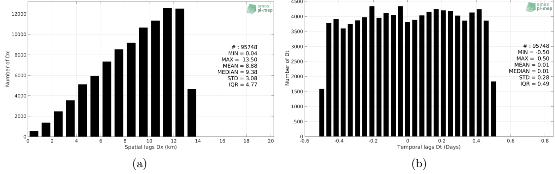
Figure 5: Histograms of the spatial (a) and temporal (b) lags between the location/time of the TSG (GOSUD-Sailing-ship) measurement and the date of the corresponding SMOS SSS L3 Arctic OA v2 - 9 Days (BEC) SSS pixel.
