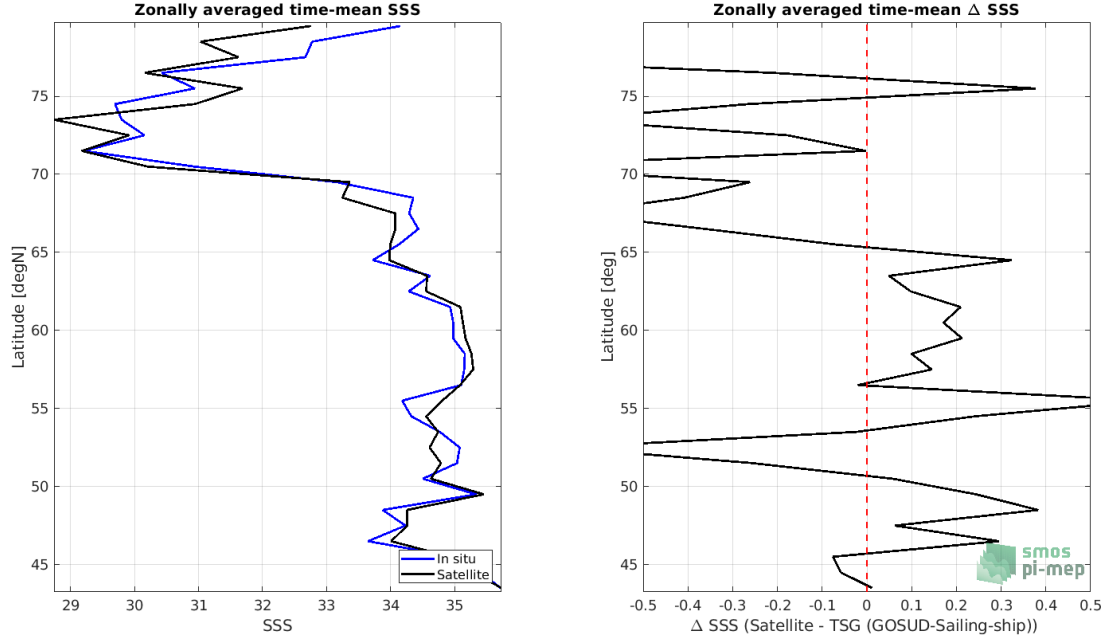
Figure 8: Left panel: Zonal mean SSS from SMOS SSS L3 Arctic OA v2 - 9 Days (BEC) satellite product (black) and from TSG (GOSUD-Sailing-ship) (blue). Right panel: Zonal mean of \Delta SSS (Satellite - TSG (GOSUD-Sailing-ship)) for all the collected Pi-MEP match-up pairs estimated over the full satellite product period.
