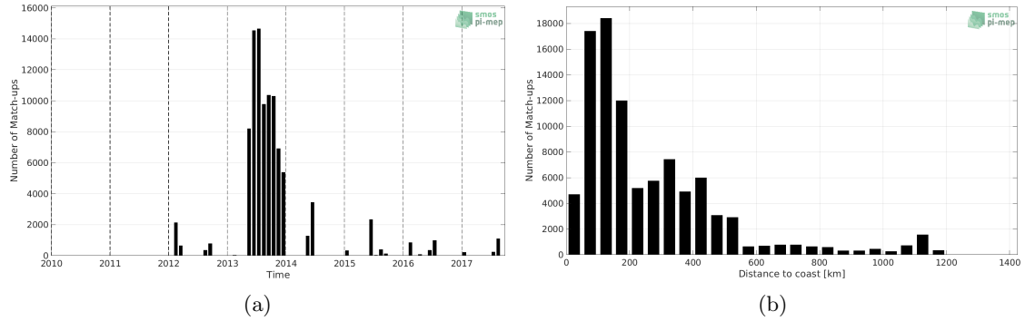
Figure 1: Number of match-ups between TSG (GOSUD-Sailing-ship) and SMOS SSS L3 Arctic OA v2 - 9 Days (BEC) SSS as a function of time (a) and as function of the distance to coast (b) over the Global Ocean Pi-MEP region and for the full satellite product period.
