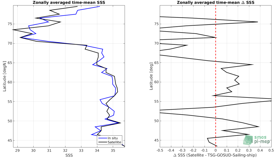
Figure 8: Left panel: Zonal mean SSS from SMOS L3 Arctic OA v2 - 9 Days (BEC) satellite product (black) and from TSG-GOSUD-Sailing-ship (blue). Right panel: Zonal mean of \Delta SSS (Satellite - TSG-GOSUD-Sailing-ship) for all the collected Pi-MEP match-up pairs estimated over the full satellite product period.
