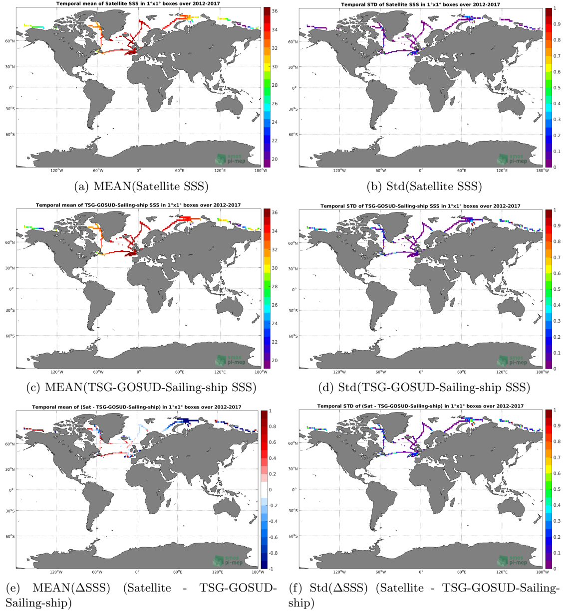
Figure 6: Temporal mean (left) and Std (right) of SSS from SMOS L3 Arctic OA v2 - 9 Days (BEC) (top), TSG-GOSUD-Sailing-ship (middle), and of \Delta SSS (Satellite - TSG-GOSUD-Sailing-ship). Only match-up pairs are used to generate these maps.
