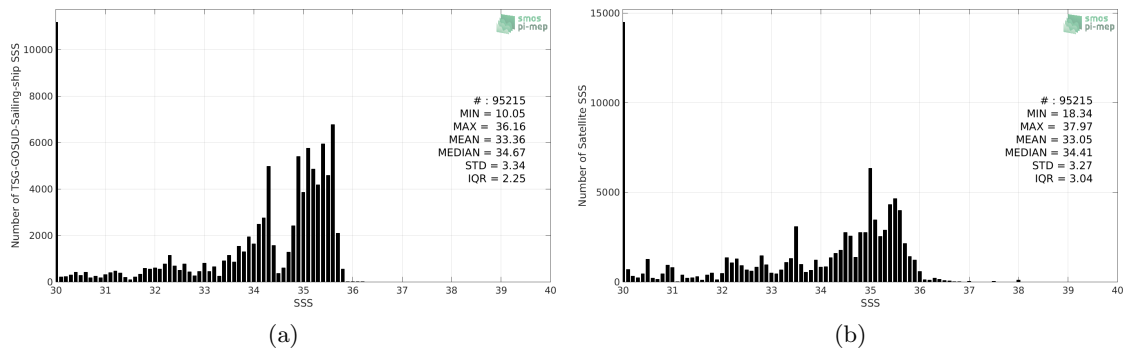
Figure 2: Histograms of SSS from TSG-GOSUD-Sailing-ship (a) and SMOS L3 Arctic OA v2 - 9 Days (BEC) (b) considering all match-up pairs per bins of 0.1 over the Global Ocean Pi-MEP region and for the full satellite product period.
