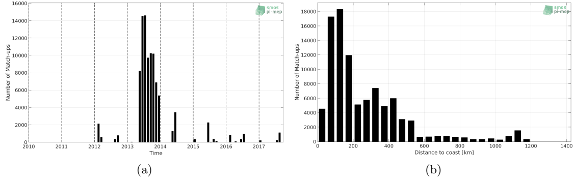
Figure 1: Number of match-ups between TSG-GOSUD-Sailing-ship and SMOS L3 Arctic OA v2 - 9 Days (BEC) SSS as a function of time (a) and as function of the distance to coast (b) over the Global Ocean Pi-MEP region and for the full satellite product period.
