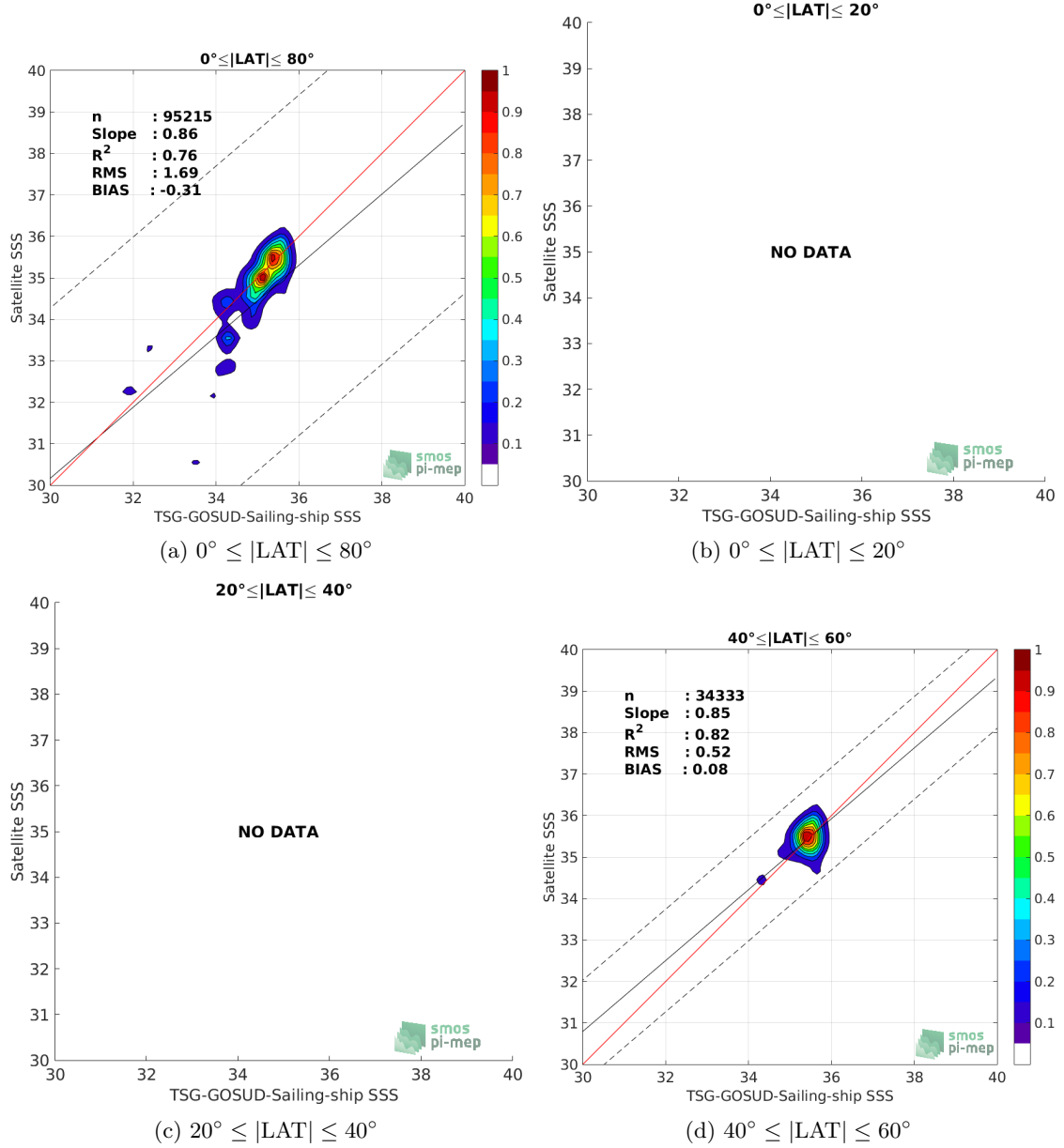
Figure 9: Contour maps of the concentration of SMOS L3 Arctic OA v2 - 9 Days (BEC) SSS (y-axis) versus TSG-GOSUD-Sailing-ship SSS (x-axis) at match-up pairs for different latitude bands. For each plot, the red line shows x=y . The black thin and dashed lines indicate a linear fit through the data cloud and the \pm 95\% confidence levels, respectively. The number match-up pairs n , the slope and R^2 coefficient of the linear fit, the root mean square (RMS) and the mean bias between satellite and in situ data are indicated for each latitude band in each plots.
