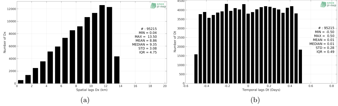
Figure 5: Histograms of the spatial (a) and temporal (b) lags between the time of the TSG-GOSUD-Sailing-ship measurements and the date of the corresponding SMOS L3 Arctic OA v2 - 9 Days (BEC) SSS product.
