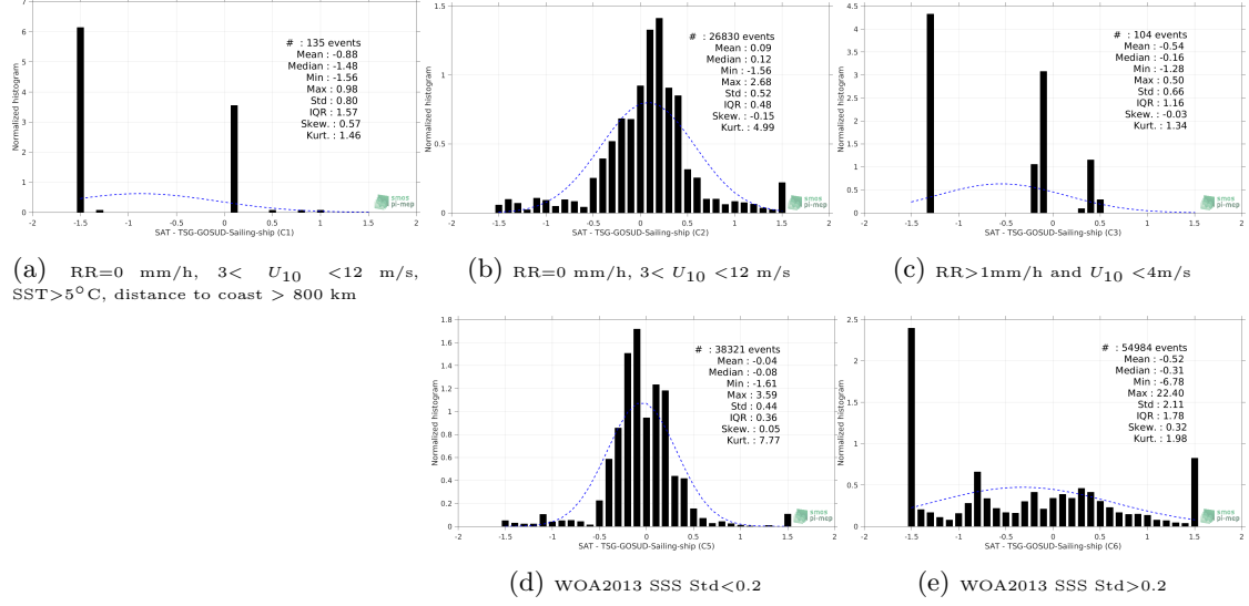
Figure 13: Normalized histogram of \Delta SSS (SMOS L3 Arctic OA v2 - 9 Days (BEC) - TSG-GOSUD-Sailing-ship) for 5 different subdatasets corresponding to: RR=0 mm/h, 3 < U_{10} < 12 m/s, SST > 5^\circ C , distance to coast > 800 km (a), RR=0 mm/h, 3 < U_{10} < 12 m/s (b), RR > 1 mm/h and U_{10} < 4 m/s (c), WOA2013 SSS Std < 0.2 (d), WOA2013 SSS Std > 0.2 (e).
