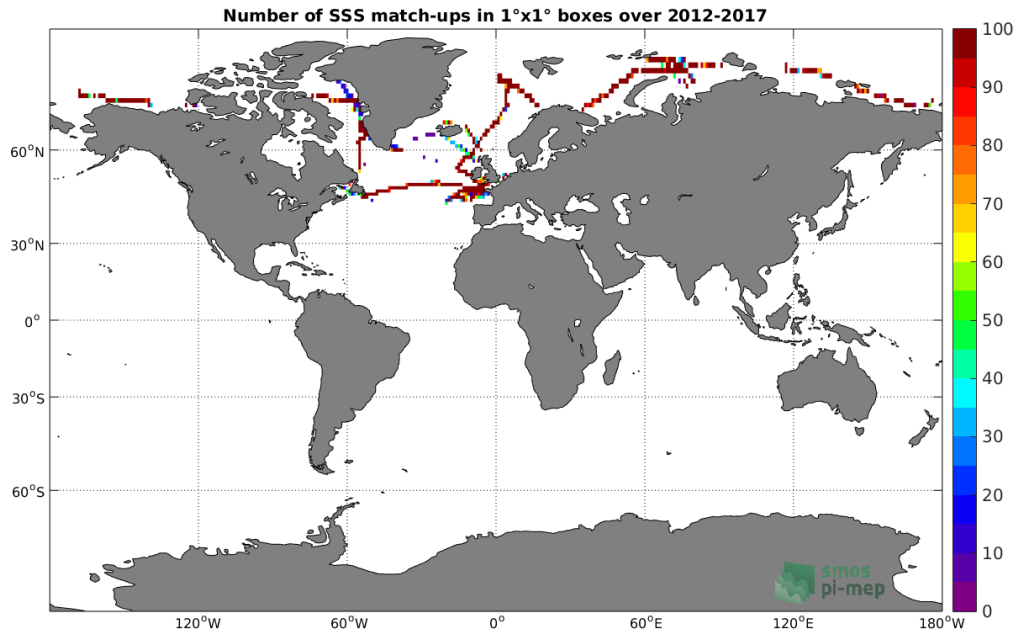
Figure 4: Number of SSS match-ups between TSG-GOSUD-Sailing-ship SSS and the SMOS-L3-BEC-ARCTIC-OA-V2-9DAYS-0.25DEG SSS product for the Global Ocean Pi-MEP region over 1^\circ \times 1^\circ boxes and for the full satellite product period.
