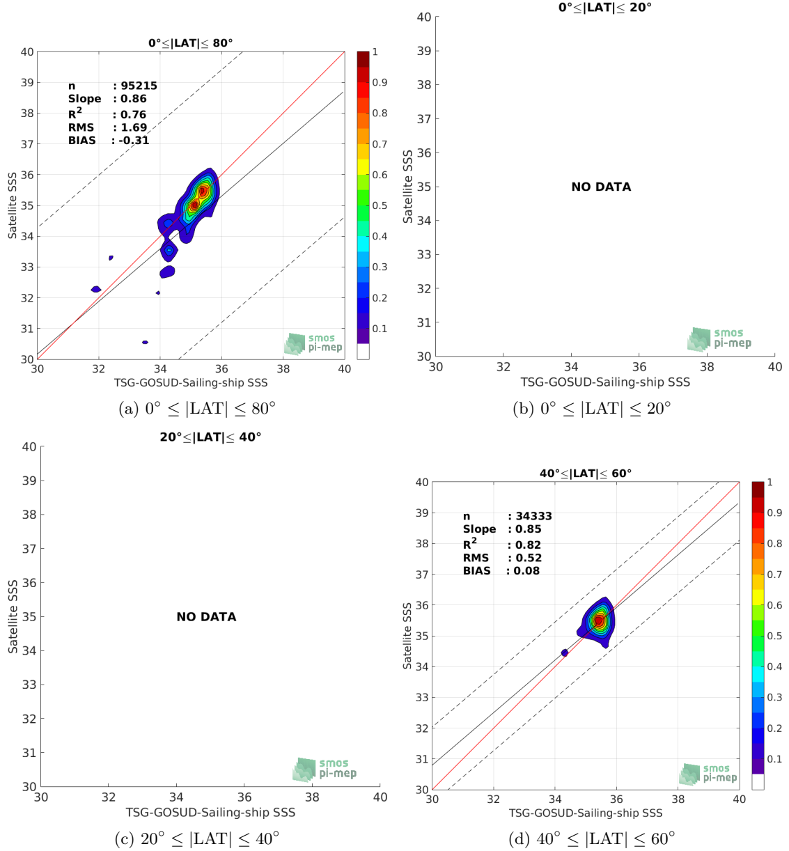
Figure 9: Contour maps of the concentration of SMOS-L3-BEC-ARCTIC-OA-V2-9DAYS-0.25DEG SSS (y-axis) versus TSG-GOSUD-Sailing-ship SSS (x-axis) at match-up pairs for different latitude bands. For each plot, the red line shows x=y . The black thin and dashed lines indicate a linear fit through the data cloud and the \pm 95\% confidence levels, respectively. The number match-up pairs n , the slope and R^2 coefficient of the linear fit, the root mean square (RMS) and the mean bias between satellite and in situ data are indicated for each latitude band in each plots.
