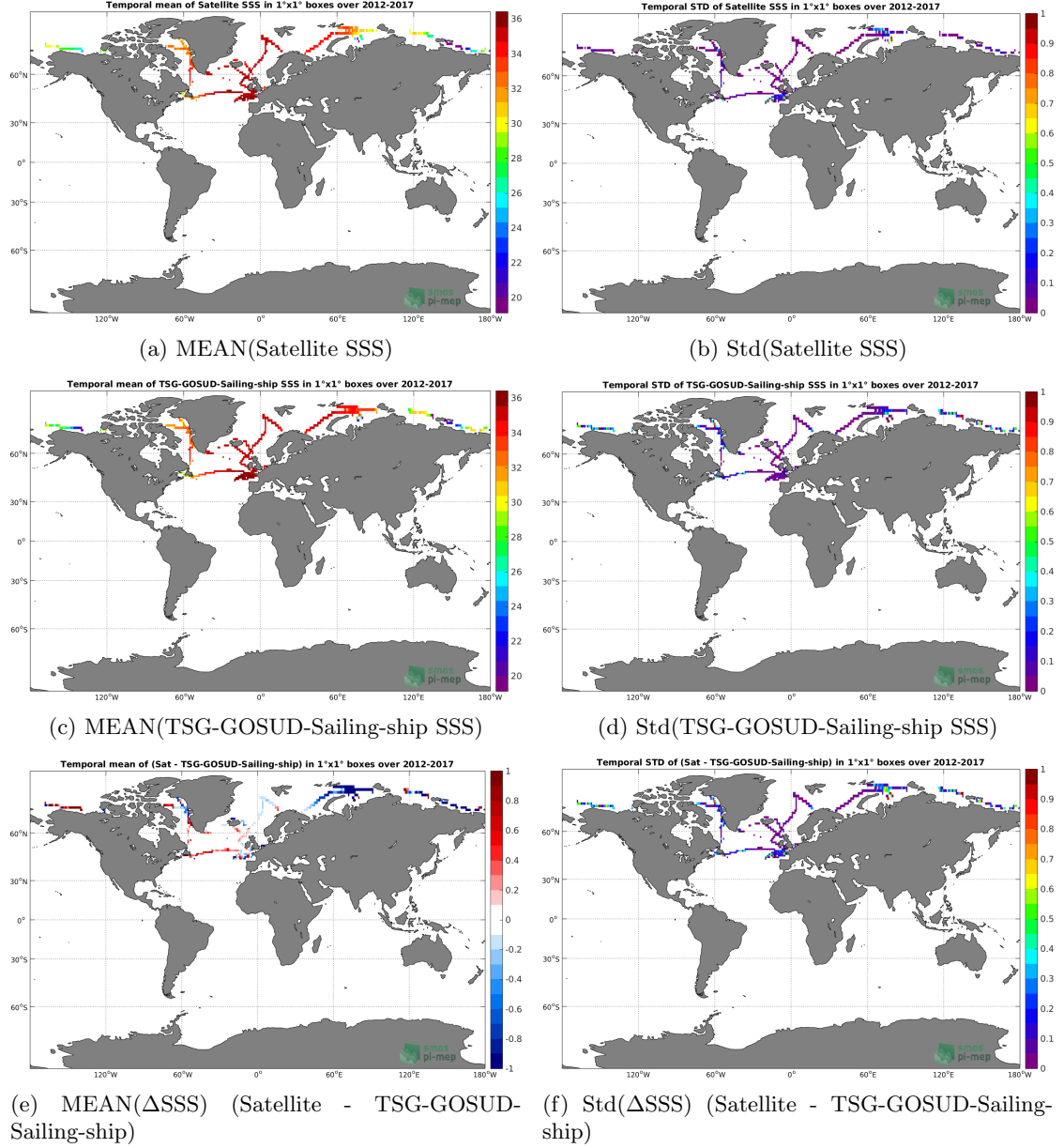
Figure 6: Temporal mean (left) and Std (right) of SSS from SMOS-L3-BEC-ARCTIC-OA-V2-9DAYS-0.25DEG (top), TSG-GOSUD-Sailing-ship (middle), and of \Delta SSS (Satellite - TSG-GOSUD-Sailing-ship). Only match-up pairs are used to generate these maps.
