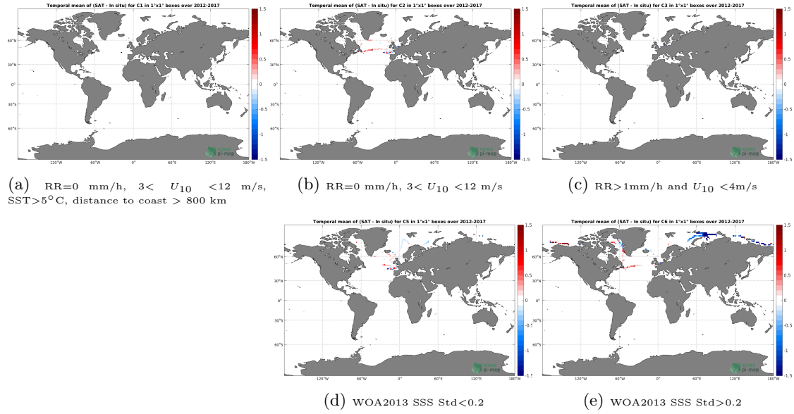
Figure 12: Temporal mean gridded over spatial boxes of size 1^\circ \times 1^\circ of \Delta SSS (SMOS-L3-BEC-ARCTIC-OA-V2-9DAYS-0.25DEG - TSG-GOSUD-Sailing-ship) for 5 different subdatasets corresponding to: RR=0 mm/h, 3 < U_{10} < 12 m/s, SST >5^\circ\text{C} , distance to coast > 800 km (a), RR=0 mm/h, 3 < U_{10} < 12 m/s (b), RR >1 mm/h and U_{10} < 4 m/s (c), WOA2013 SSS Std <0.2 (d), WOA2013 SSS Std >0.2 (e).
