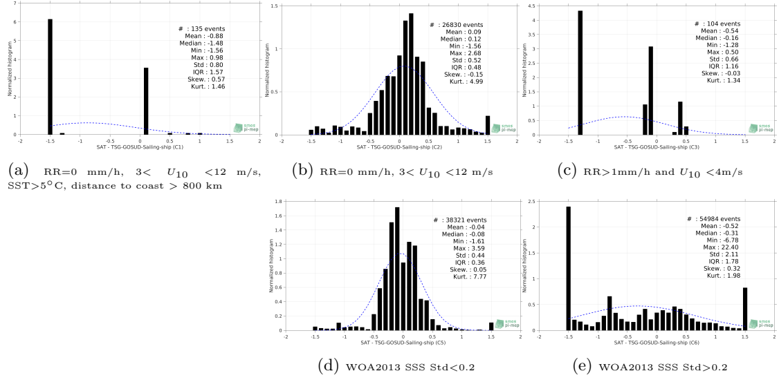
Figure 13: Normalized histogram of \Delta SSS (SMOS-L3-BEC-ARCTIC-OA-V2-9DAYS-0.25DEG - TSG-GOSUD-Sailing-ship) for 5 different subdatasets corresponding to: RR=0 mm/h, 3 < U_{10} < 12 m/s, SST > 5^\circ C , distance to coast > 800 km (a), RR=0 mm/h, 3 < U_{10} < 12 m/s (b), RR > 1 mm/h and U_{10} < 4 m/s (c), WOA2013 SSS Std < 0.2 (d), WOA2013 SSS Std > 0.2 (e).
