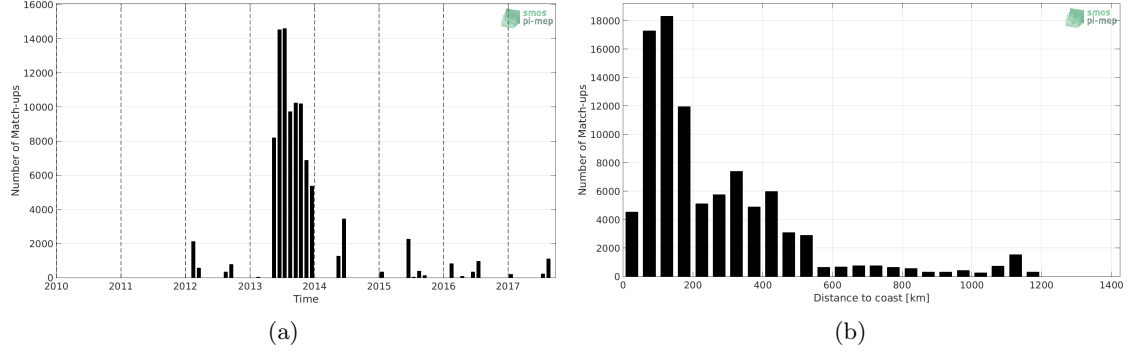
Figure 1: Number of match-ups between TSG-GOSUD-Sailing-ship and SMOS-L3-BEC-ARCTIC-OA-V2-9DAYS-0.25DEG SSS as a function of time (a) and as function of the distance to coast (b) over the Global Ocean Pi-MEP region and for the full satellite product period.
