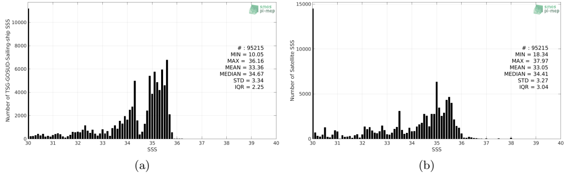
Figure 2: Histograms of SSS from TSG-GOSUD-Sailing-ship (a) and SMOS-L3-BEC-ARCTIC-OA-V2-9DAYS-0.25DEG (b) considering all match-up pairs per bins of 0.1 over the Global Ocean Pi-MEP region and for the full satellite product period.
