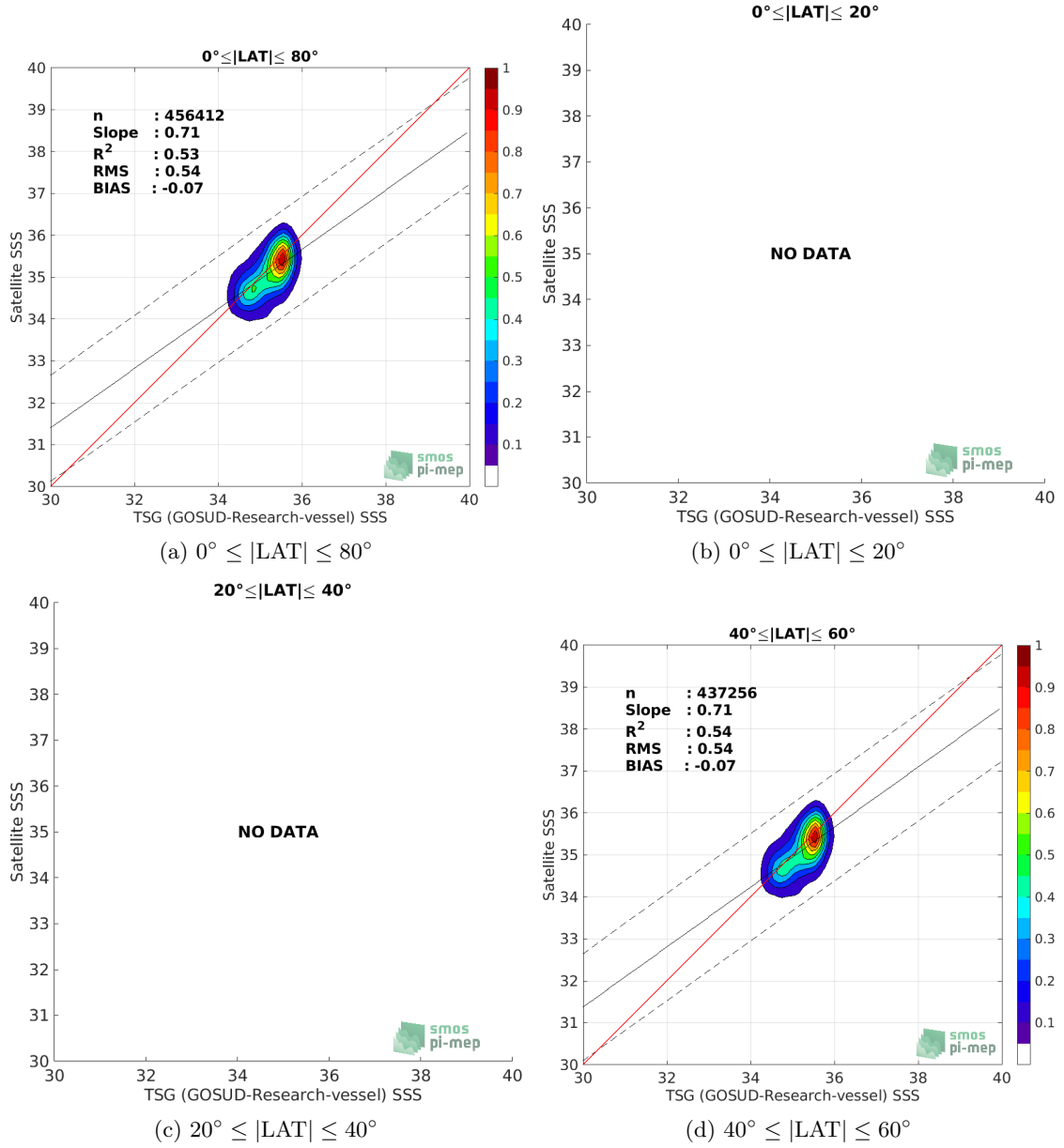
Figure 9: Contour maps of the concentration of SMOS SSS L3 Arctic OA v2 - 9 Days (BEC) SSS (y-axis) versus TSG (GOSUD-Research-vessel) SSS (x-axis) at match-up pairs for different latitude bands. For each plot, the red line shows x=y . The black thin and dashed lines indicate a linear fit through the data cloud and the \pm 95\% confidence levels, respectively. The number match-up pairs n , the slope and R^2 coefficient of the linear fit, the root mean square (RMS) and the mean bias between satellite and in situ data are indicated for each latitude band in each plots.
