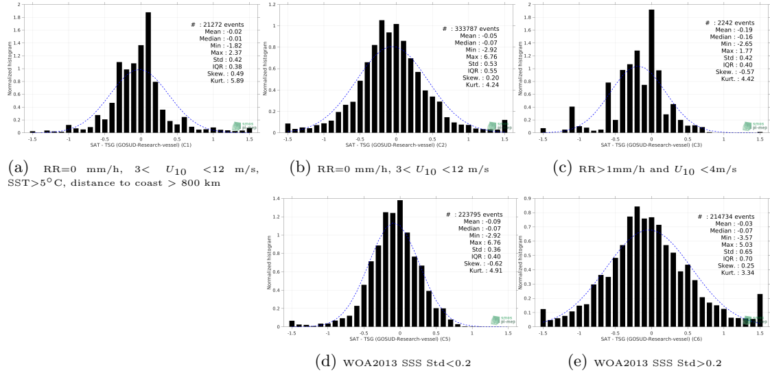
Figure 13: Normalized histogram of \Delta SSS (SMOS SSS L3 Arctic OA v2 - 9 Days (BEC) - TSG (GOSUD-Research-vessel)) for 5 different subdatasets corresponding to: RR=0 mm/h, 3 < U_{10} < 12 m/s, SST>5°C, distance to coast > 800 km (a), RR=0 mm/h, 3 < U_{10} < 12 m/s (b), RR>1mm/h and U_{10} < 4 m/s (c), WOA2013 SSS Std<0.2 (d), WOA2013 SSS Std>0.2 (e).
