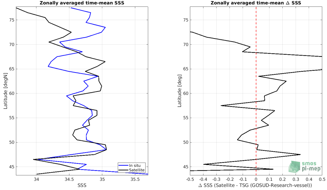
Figure 8: Left panel: Zonal mean SSS from SMOS SSS L3 Arctic OA v2 - 9 Days (BEC) satellite product (black) and from TSG (GOSUD-Research-vessel) (blue). Right panel: Zonal mean of \Delta SSS (Satellite - TSG (GOSUD-Research-vessel)) for all the collected Pi-MEP match-up pairs estimated over the full satellite product period.
