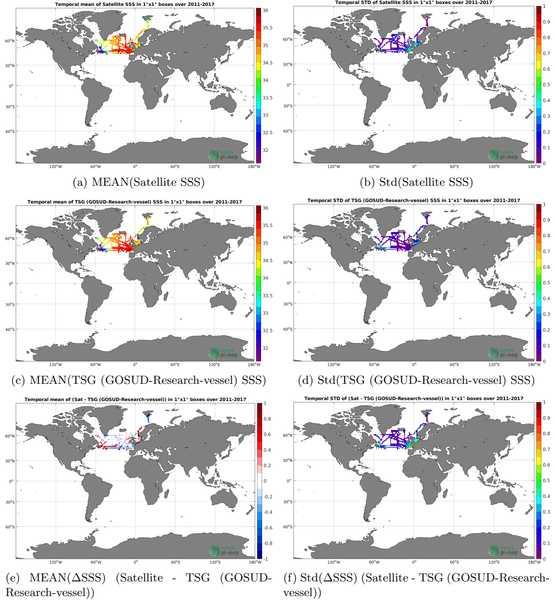
Figure 6: Temporal mean (left) and Std (right) of SSS from SMOS SSS L3 Arctic OA v2 - 9 Days (BEC) (top), TSG (GOSUD-Research-vessel) (middle), and of \Delta SSS (Satellite - TSG (GOSUD-Research-vessel)). Only match-up pairs are used to generate these maps.
