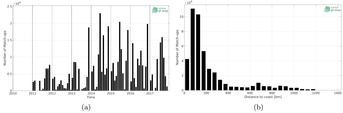
Figure 1: Number of match-ups between TSG (GOSUD-Research-vessel) and SMOS SSS L3 Arctic OA v2 - 9 Days (BEC) SSS as a function of time (a) and as function of the distance to coast (b) over the Global Ocean Pi-MEP region and for the full satellite product period.
