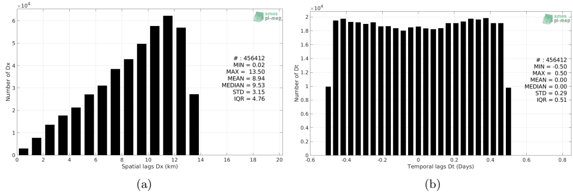
Figure 5: Histograms of the spatial (a) and temporal (b) lags between the location/time of the TSG (GOSUD-Research-vessel) measurement and the date of the corresponding SMOS SSS L3 Arctic OA v2 - 9 Days (BEC) SSS pixel.
