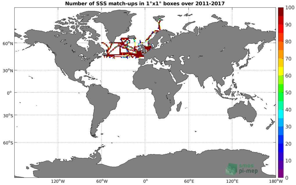
Figure 4: Number of SSS match-ups between TSG (GOSUD-Research-vessel) SSS and the SMOS SSS L3 Arctic OA v2 - 9 Days (BEC) SSS product for the Global Ocean Pi-MEP region over 1^\circ \times 1^\circ boxes and for the full satellite product period.
