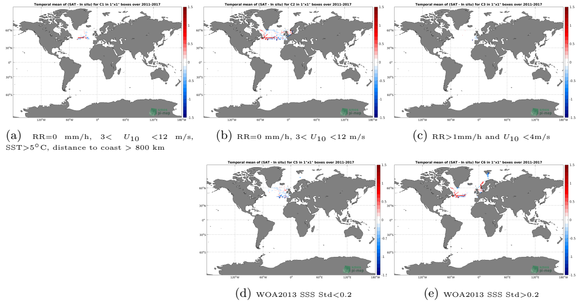
Figure 12: Temporal mean gridded over spatial boxes of size 1^\circ \times 1^\circ of \Delta SSS (SMOS SSS L3 Arctic OA v2 - 9 Days (BEC) - TSG (GOSUD-Research-vessel)) for 5 different subdatasets corresponding to: RR=0 mm/h, 3 < U_{10} < 12 m/s, SST >5^\circ\text{C} , distance to coast > 800 km (a), RR=0 mm/h, 3 < U_{10} < 12 m/s (b), RR >1 mm/h and U_{10} < 4 m/s (c), WOA2013 SSS Std <0.2 (d), WOA2013 SSS Std >0.2 (e).
