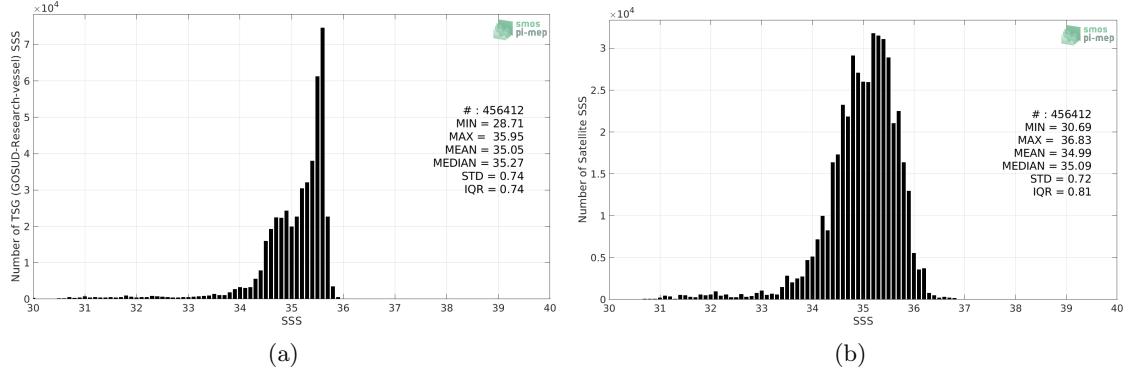
Figure 2: Histograms of SSS from TSG (GOSUD-Research-vessel) (a) and SMOS SSS L3 Arctic OA v2 - 9 Days (BEC) (b) considering all match-up pairs per bins of 0.1 over the Global Ocean Pi-MEP region and for the full satellite product period.
