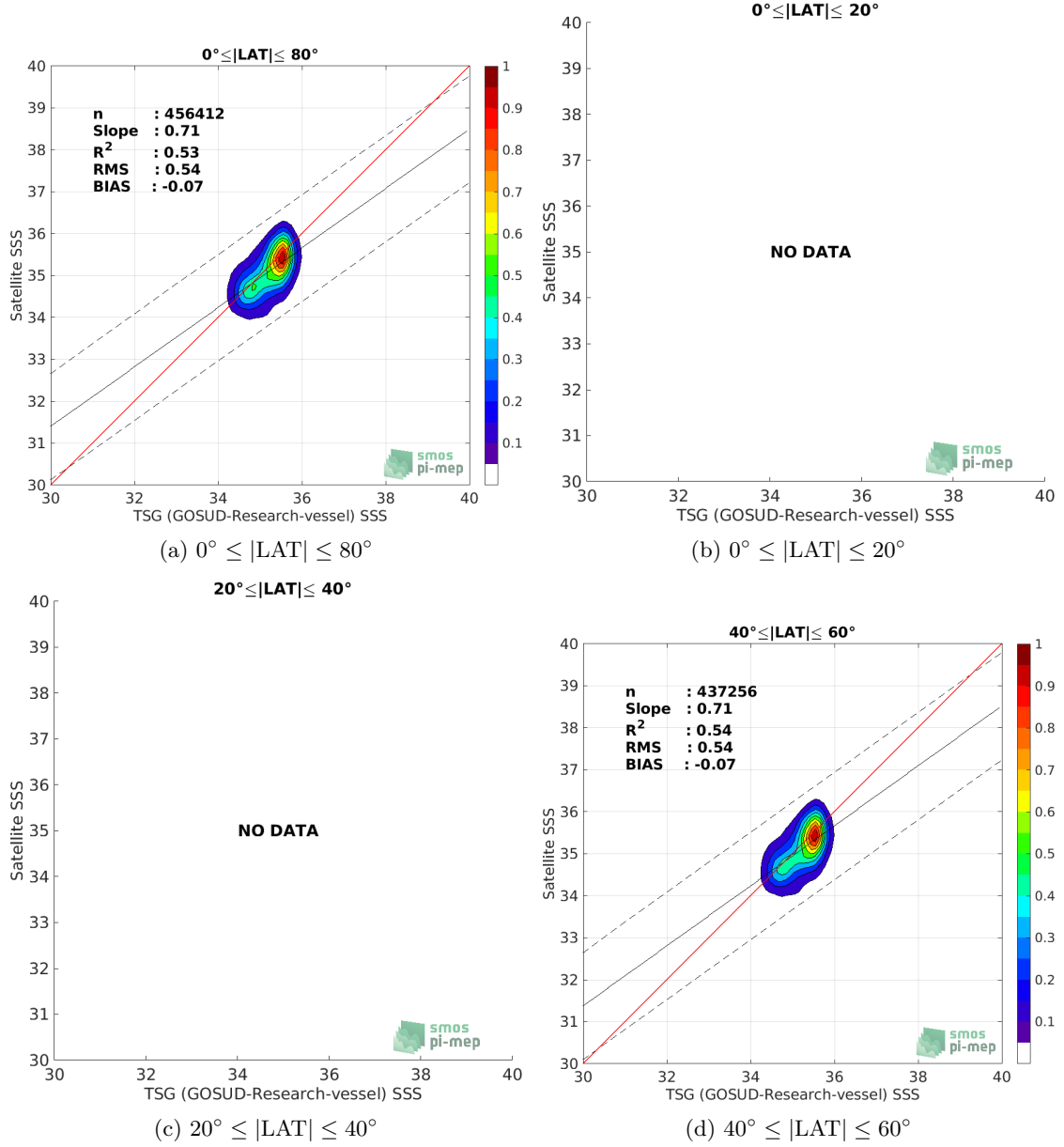
Figure 9: Contour maps of the concentration of SMOS SSS L3 Arctic OA v2 - 9 Days (BEC) SSS (y-axis) versus TSG (GOSUD-Research-vessel) SSS (x-axis) at match-up pairs for different latitude bands. For each plot, the red line shows x=y . The black thin and dashed lines indicate a linear fit through the data cloud and the \pm 95\% confidence levels, respectively. The number match-up pairs n , the slope and R^2 coefficient of the linear fit, the root mean square (RMS) and the mean bias between satellite and in situ data are indicated for each latitude band in each plots.
