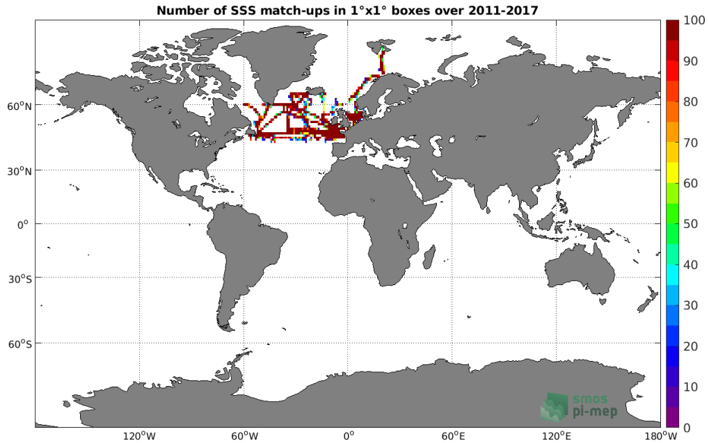
Figure 4: Number of SSS match-ups between TSG (GOSUD-Research-vessel) SSS and the SMOS SSS L3 Arctic OA v2 - 9 Days (BEC) SSS product for the Global Ocean Pi-MEP region over 1°x1° boxes and for the full satellite product period.
