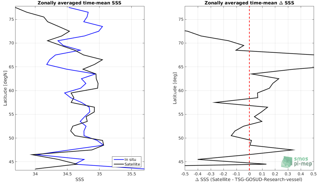
Figure 8: Left panel: Zonal mean SSS from SMOS L3 Arctic OA v2 - 9 Days (BEC) satellite product (black) and from TSG-GOSUD-Research-vessel (blue). Right panel: Zonal mean of \Delta SSS (Satellite - TSG-GOSUD-Research-vessel) for all the collected Pi-MEP match-up pairs estimated over the full satellite product period.
