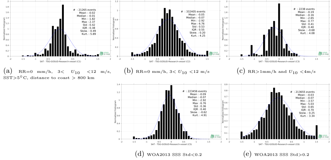
Figure 13: Normalized histogram of \Delta SSS (SMOS L3 Arctic OA v2 - 9 Days (BEC) - TSG-GOSUD-Research-vessel) for 5 different subdatasets corresponding to: RR=0 mm/h, 3 < U_{10} < 12 m/s, SST > 5°C, distance to coast > 800 km (a), RR=0 mm/h, 3 < U_{10} < 12 m/s (b), RR > 1 mm/h and U_{10} < 4 m/s (c), WOA2013 SSS Std < 0.2 (d), WOA2013 SSS Std > 0.2 (e).
