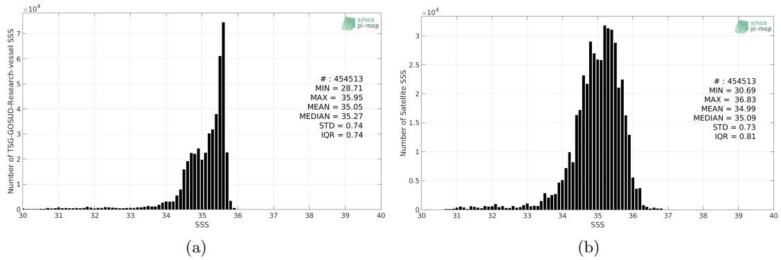
Figure 2: Histograms of SSS from TSG-GOSUD-Research-vessel (a) and SMOS L3 Arctic OA v2 - 9 Days (BEC) (b) considering all match-up pairs per bins of 0.1 over the Global Ocean Pi-MEP region and for the full satellite product period.
