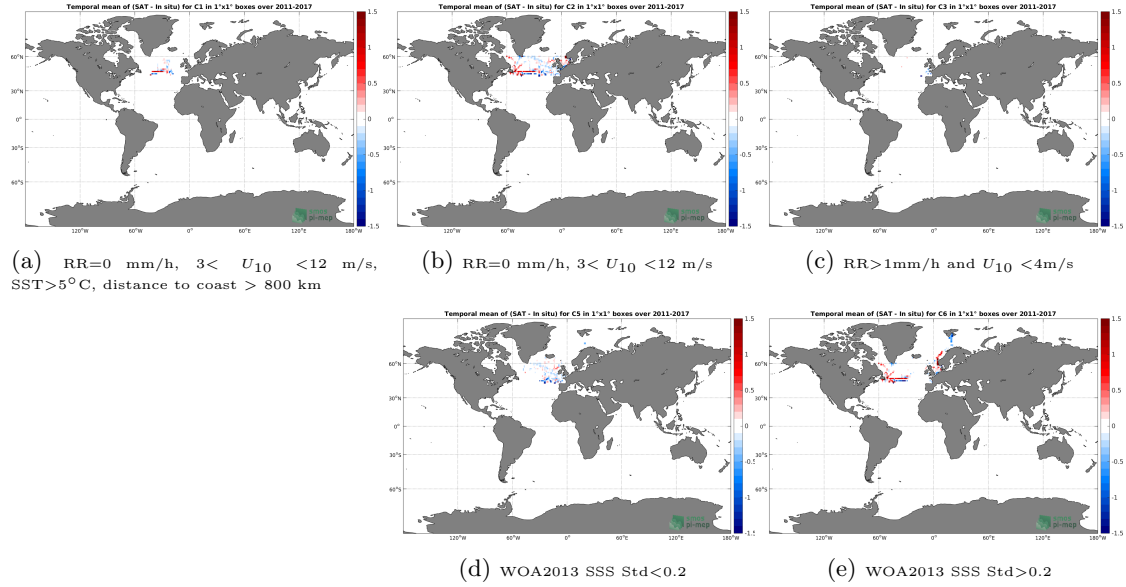
Figure 12: Temporal mean gridded over spatial boxes of size 1^{\circ}\times 1^{\circ} of \Delta SSS (SMOS L3 Arctic OA v2 - 9 Days (BEC) - TSG-GOSUD-Research-vessel) for 5 different subdatasets corresponding to: RR=0 mm/h, 3 < U_{10} < 12 m/s, SST >5^{\circ}\text{C} , distance to coast > 800 km (a), RR=0 mm/h, 3 < U_{10} < 12 m/s (b), RR >1 mm/h and U_{10} < 4 m/s (c), WOA2013 SSS Std <0.2 (d), WOA2013 SSS Std >0.2 (e).
