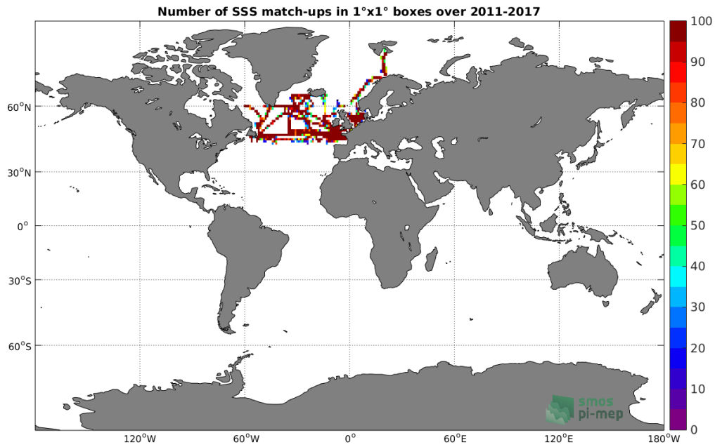
Figure 4: Number of SSS match-ups between TSG-GOSUD-Research-vessel SSS and the SMOS L3 Arctic OA v2 - 9 Days (BEC) SSS product for the Global Ocean Pi-MEP region over 1°x1° boxes and for the full satellite product period.
