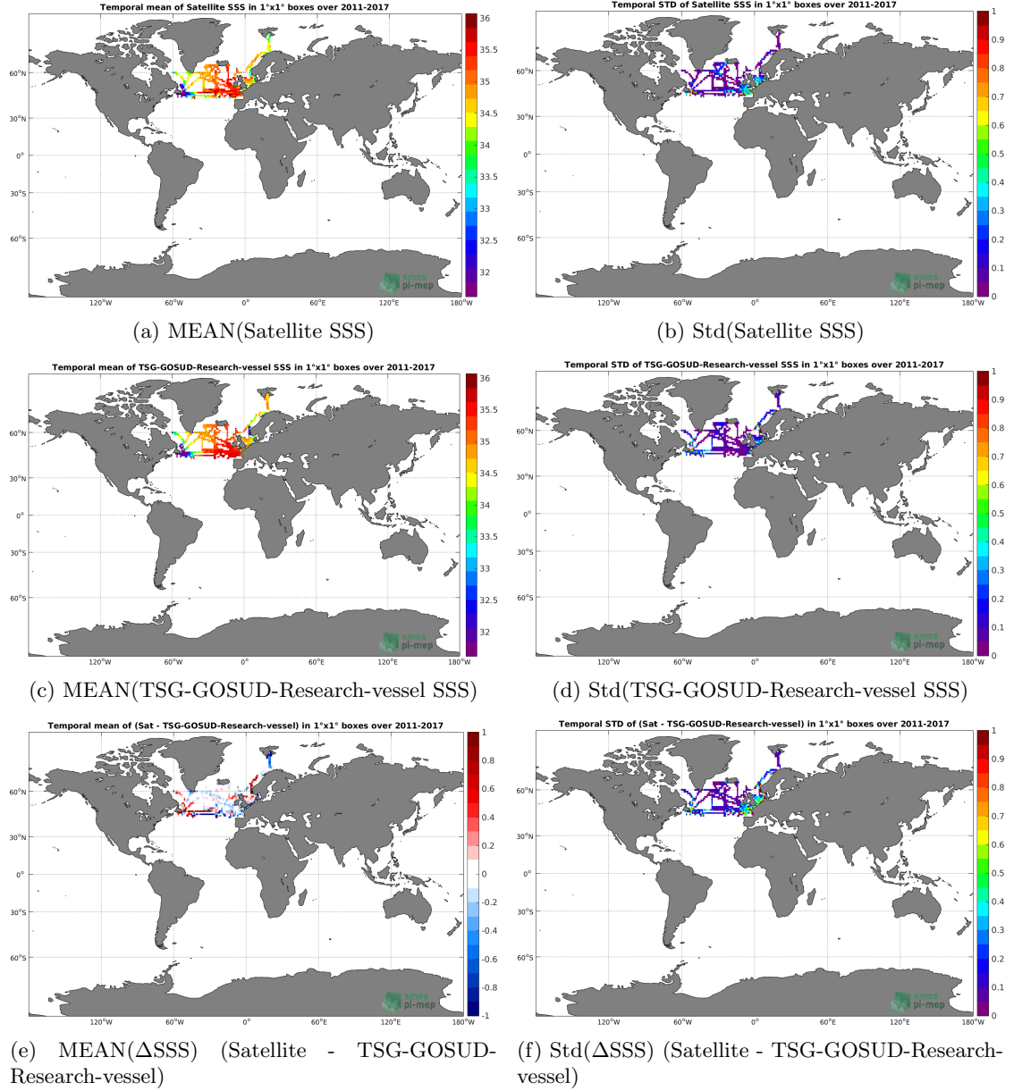
Figure 6: Temporal mean (left) and Std (right) of SSS from SMOS L3 Arctic OA v2 - 9 Days (BEC) (top), TSG-GOSUD-Research-vessel (middle), and of \Delta SSS (Satellite - TSG-GOSUD-Research-vessel). Only match-up pairs are used to generate these maps.
