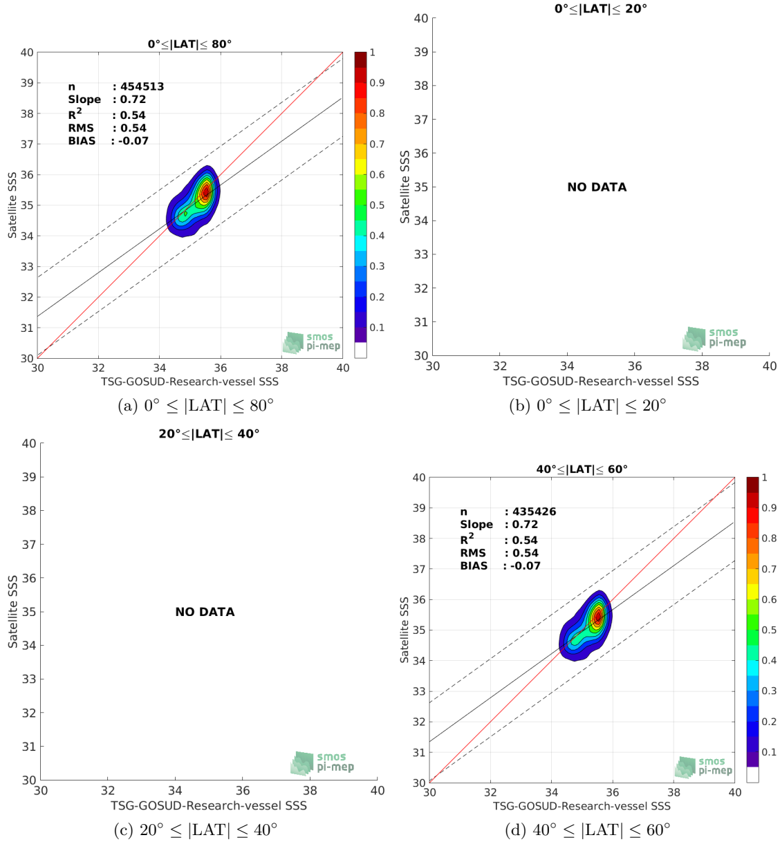
Figure 9: Contour maps of the concentration of SMOS L3 Arctic OA v2 - 9 Days (BEC) SSS (y-axis) versus TSG-GOSUD-Research-vessel SSS (x-axis) at match-up pairs for different latitude bands. For each plot, the red line shows x=y . The black thin and dashed lines indicate a linear fit through the data cloud and the \pm 95\% confidence levels, respectively. The number match-up pairs n , the slope and R^2 coefficient of the linear fit, the root mean square (RMS) and the mean bias between satellite and in situ data are indicated for each latitude band in each plots.
