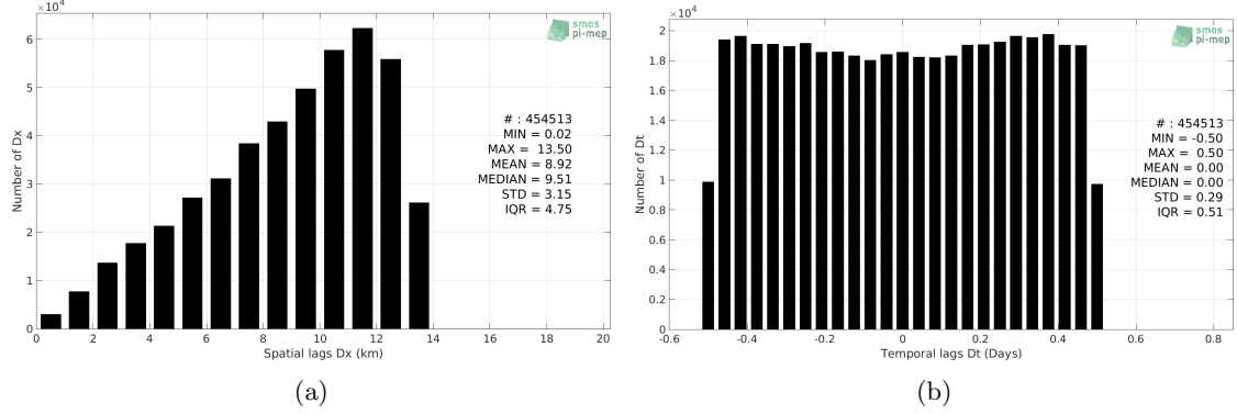
Figure 5: Histograms of the spatial (a) and temporal (b) lags between the time of the TSG-GOSUD-Research-vessel measurements and the date of the corresponding SMOS L3 Arctic OA v2 - 9 Days (BEC) SSS product.
