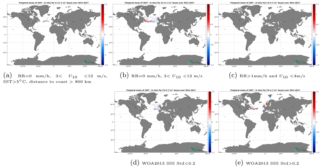
Figure 12: Temporal mean gridded over spatial boxes of size 1^\circ \times 1^\circ of \Delta SSS (SMOS-L3-BEC-ARCTIC-OA-V2-9DAYS-0.25DEG - TSG-GOSUD-Research-vessel) for 5 different subdatasets corresponding to:RR=0 mm/h, 3 < U_{10} < 12 m/s, SST >5^\circ\text{C} , distance to coast > 800 km (a), RR=0 mm/h, 3 < U_{10} < 12 m/s (b), RR >1 mm/h and U_{10} < 4 m/s (c), WOA2013 SSS Std <0.2 (d), WOA2013 SSS Std >0.2 (e).
