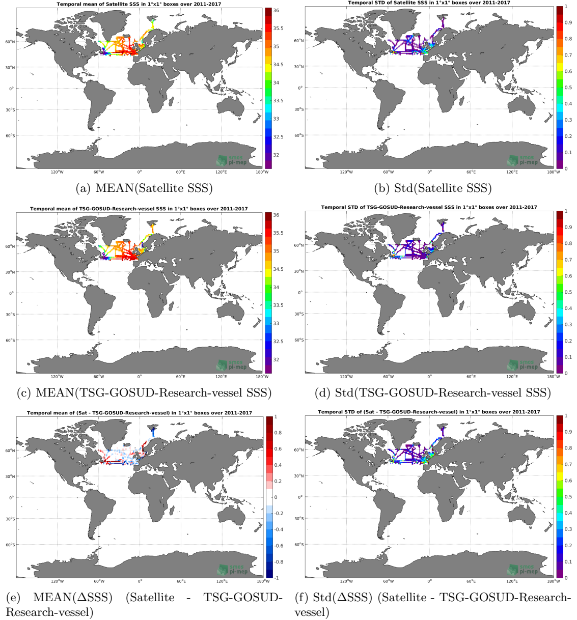
Figure 6: Temporal mean (left) and Std (right) of SSS from SMOS-L3-BEC-ARCTIC-OA-V2-9DAYS-0.25DEG (top), TSG-GOSUD-Research-vessel (middle), and of \Delta SSS (Satellite - TSG-GOSUD-Research-vessel). Only match-up pairs are used to generate these maps.
