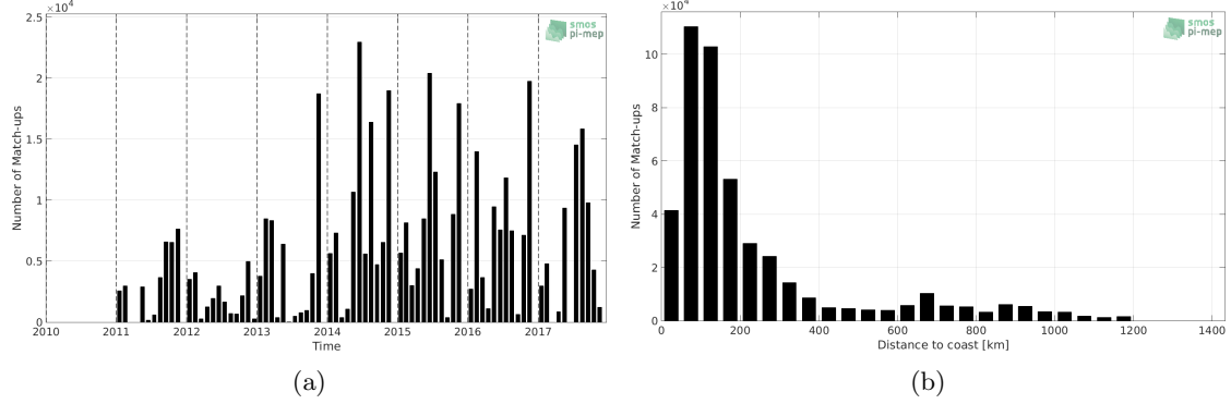
Figure 1: Number of match-ups between TSG-GOSUD-Research-vessel and SMOS-L3-BEC-ARCTIC-OA-V2-9DAYS-0.25DEG SSS as a function of time (a) and as function of the distance to coast (b) over the Global Ocean Pi-MEP region and for the full satellite product period.
