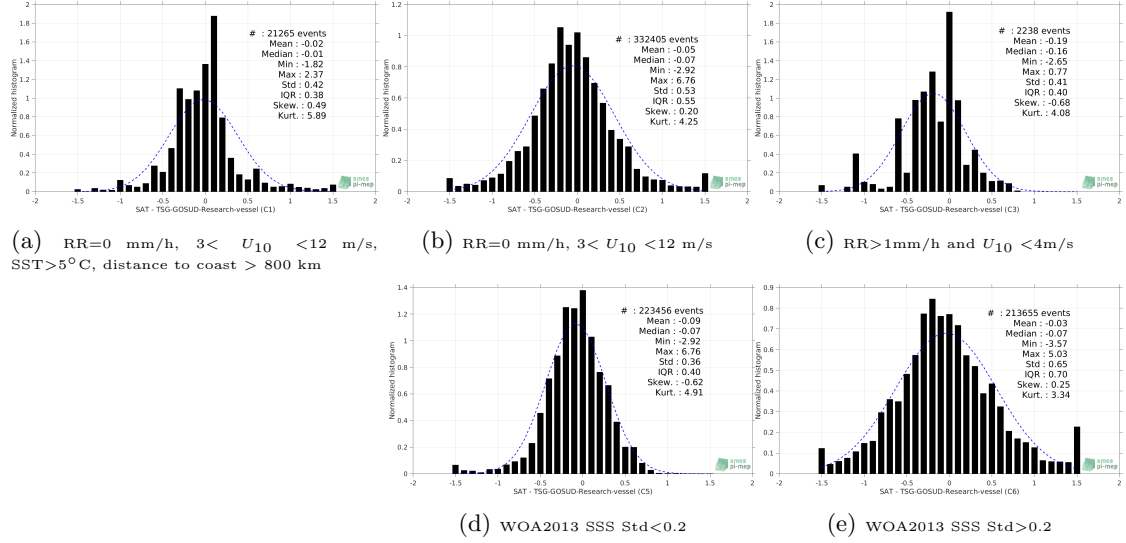
Figure 13: Normalized histogram of \Delta SSS (SMOS-L3-BEC-ARCTIC-OA-V2-9DAYS-0.25DEG - TSG-GOSUD-Research-vessel) for 5 different subdatasets corresponding to: RR=0 mm/h, 3 < U_{10} < 12 m/s, SST > 5°C, distance to coast > 800 km (a), RR=0 mm/h, 3 < U_{10} < 12 m/s (b), RR > 1mm/h and U_{10} < 4 m/s (c), WOA2013 SSS Std < 0.2 (d), WOA2013 SSS Std > 0.2 (e).
