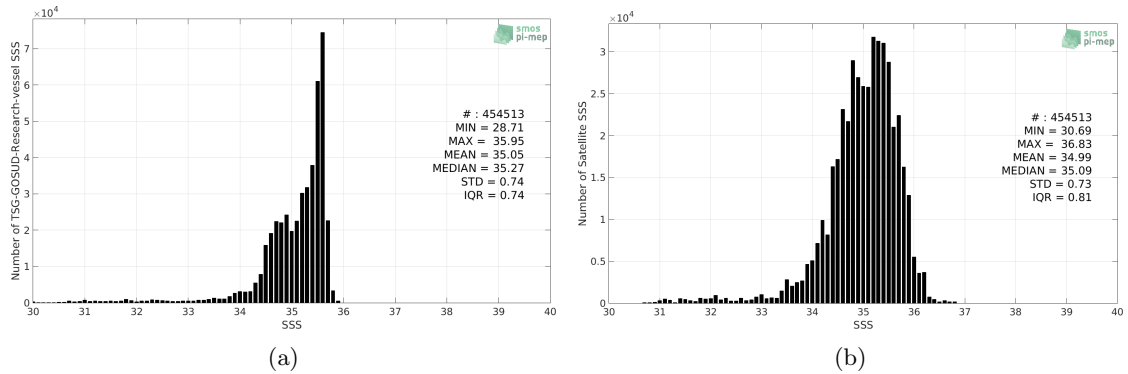
Figure 2: Histograms of SSS from TSG-GOSUD-Research-vessel (a) and SMOS-L3-BEC-ARCTIC-OA-V2-9DAYS-0.25DEG (b) considering all match-up pairs per bins of 0.1 over the Global Ocean Pi-MEP region and for the full satellite product period.
