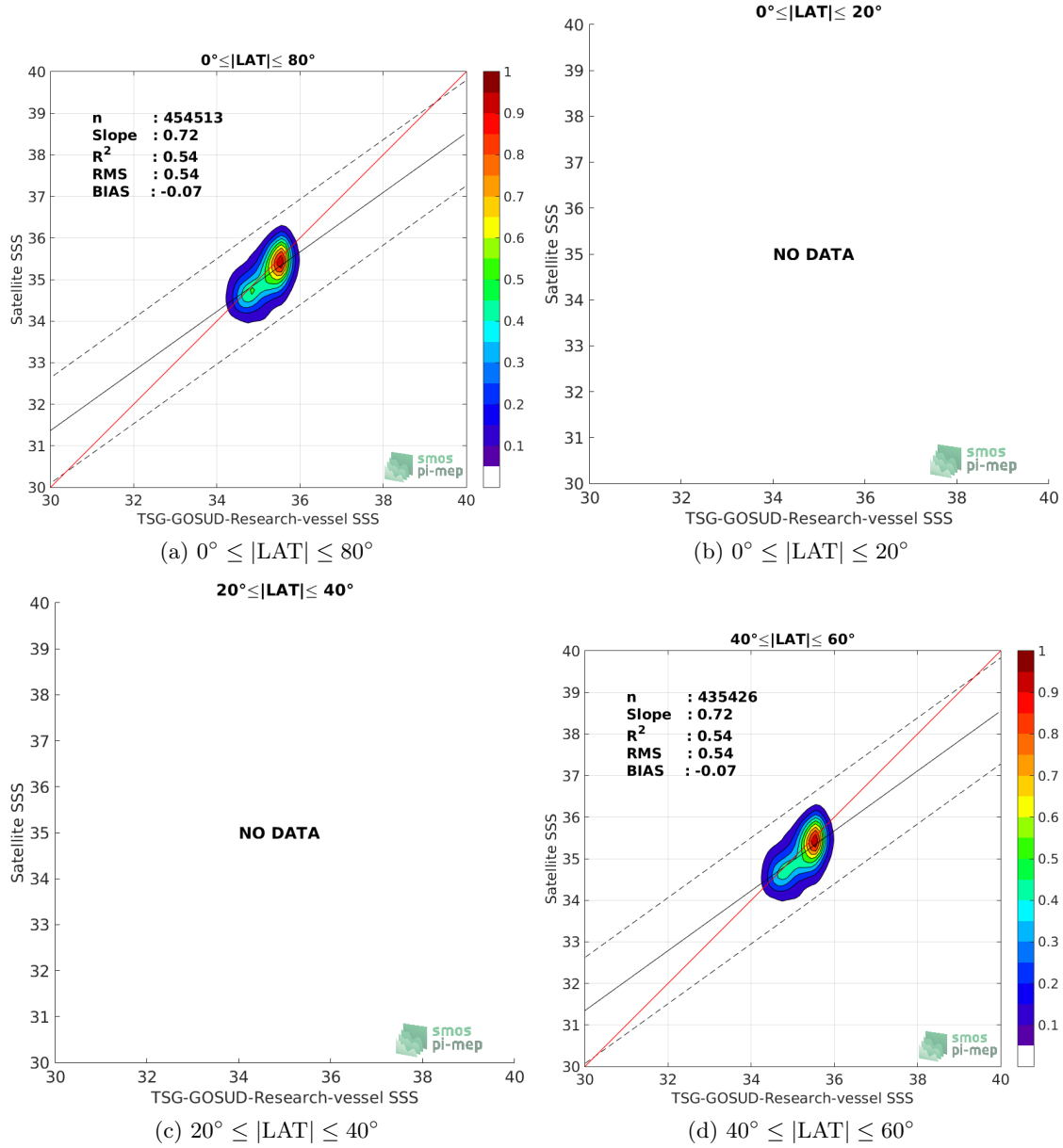
Figure 9: Contour maps of the concentration of SMOS-L3-BEC-ARCTIC-OA-V2-9DAYS-0.25DEG SSS (y-axis) versus TSG-GOSUD-Research-vessel SSS (x-axis) at match-up pairs for different latitude bands. For each plot, the red line shows x=y . The black thin and dashed lines indicate a linear fit through the data cloud and the \pm 95\% confidence levels, respectively. The number match-up pairs n , the slope and R^2 coefficient of the linear fit, the root mean square (RMS) and the mean bias between satellite and in situ data are indicated for each latitude band in each plots.
