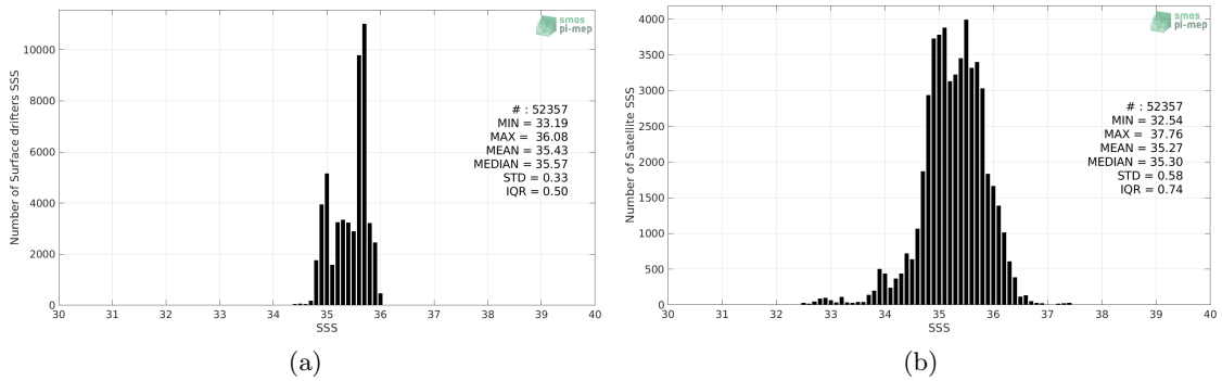
Figure 2: Histograms of SSS from Surface drifters (a) and SMOS SSS L3 Arctic OA v2 - 9 Days (BEC) (b) considering all match-up pairs per bins of 0.1 over the Global Ocean Pi-MEP region and for the full satellite product period.
