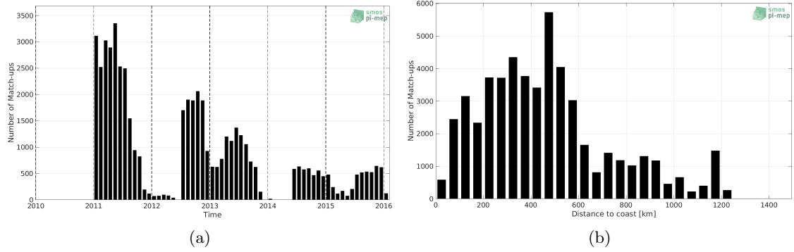
Figure 1: Number of match-ups between Surface drifters and SMOS SSS L3 Arctic OA v2 - 9 Days (BEC) SSS as a function of time (a) and as function of the distance to coast (b) over the Global Ocean Pi-MEP region and for the full satellite product period.
