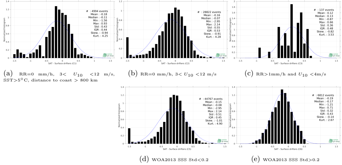
Figure 12: Normalized histogram of \Delta SSS (SMOS SSS L3 Arctic OA v2 - 9 Days (BEC) - Surface drifters) for 5 different subdatasets corresponding to: RR=0 mm/h, 3 < U_{10} < 12 m/s, SST>5°C, distance to coast > 800 km (a), RR=0 mm/h, 3 < U_{10} < 12 m/s (b), RR>1mm/h and U_{10} < 4 m/s (c), WOA2013 SSS Std<0.2 (d), WOA2013 SSS Std>0.2 (e).
