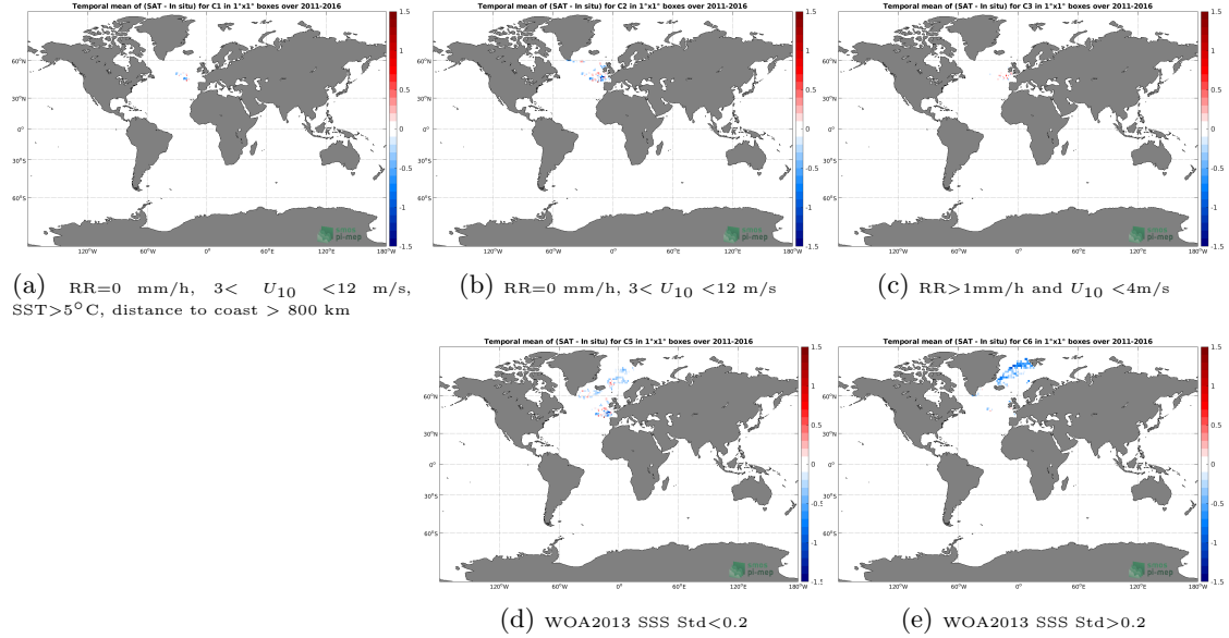
Figure 11: Temporal mean gridded over spatial boxes of size 1^{\circ}\times 1^{\circ} of \Delta\text{SSS} (SMOS SSS L3 Arctic OA v2 - 9 Days (BEC) - Surface drifters) for 5 different subdatasets corresponding to:RR=0 mm/h, 3 < U_{10} < 12 m/s, SST > 5^{\circ}\text{C} , distance to coast > 800 km (a), RR=0 mm/h, 3 < U_{10} < 12 m/s (b), RR > 1 mm/h and U_{10} < 4 m/s (c), WOA2013 SSS Std < 0.2 (d), WOA2013 SSS Std > 0.2 (e).
