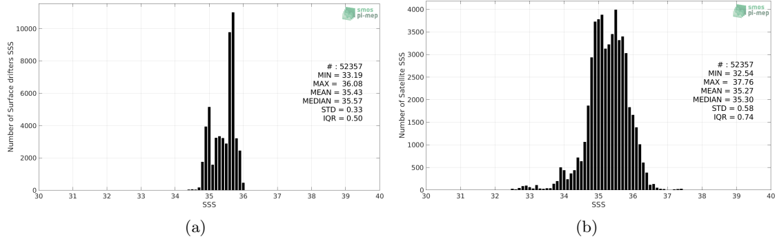
Figure 2: Histograms of SSS from Surface drifters (a) and SMOS SSS L3 Arctic OA v2 - 9 Days (BEC) (b) considering all match-up pairs per bins of 0.1 over the Global Ocean Pi-MEP region and for the full satellite product period.
