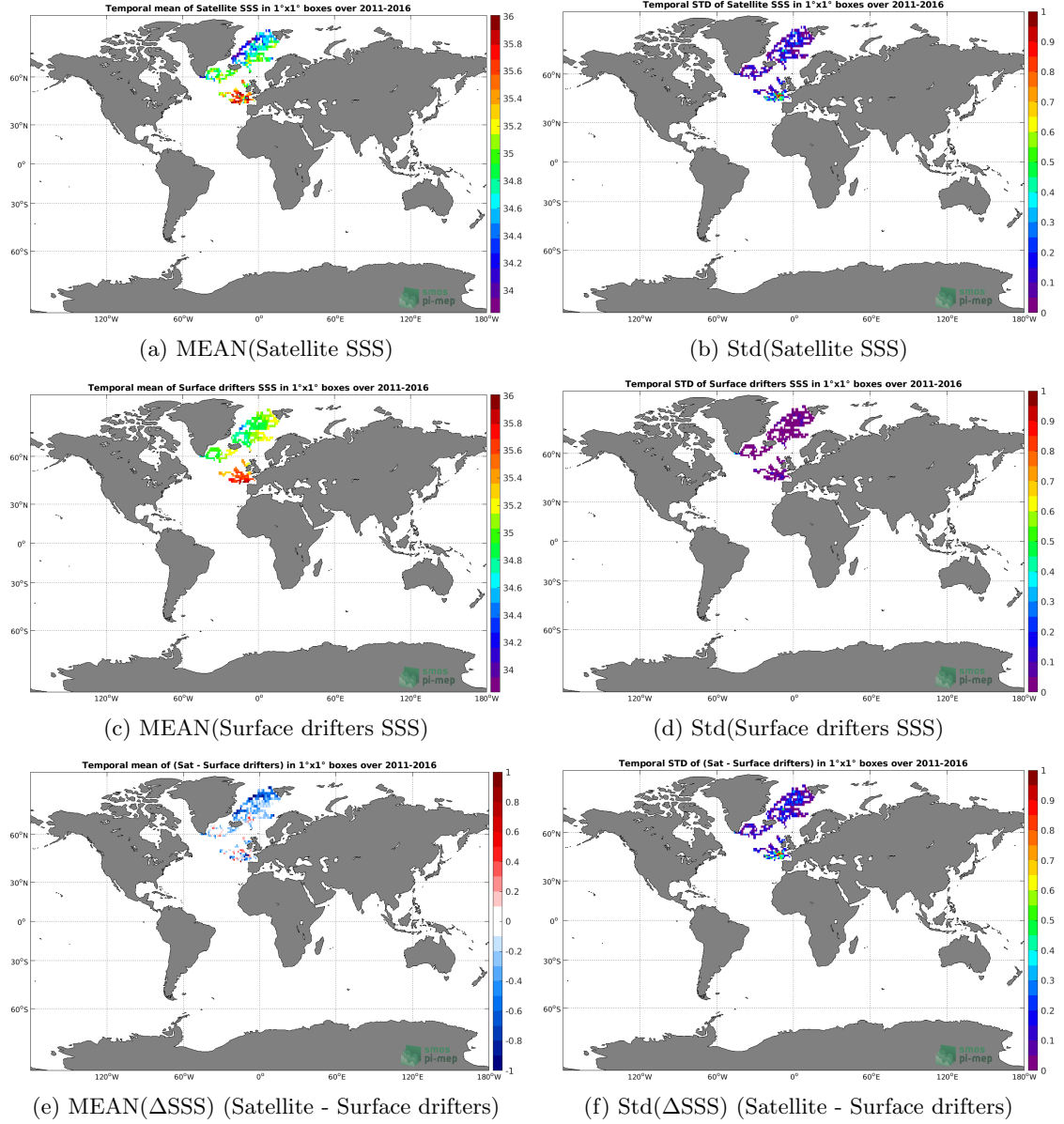
Figure 5: Temporal mean (left) and Std (right) of SSS from SMOS SSS L3 Arctic OA v2 - 9 Days (BEC) (top), Surface drifters (middle), and of \Delta SSS (Satellite - Surface drifters). Only match-up pairs are used to generate these maps.
