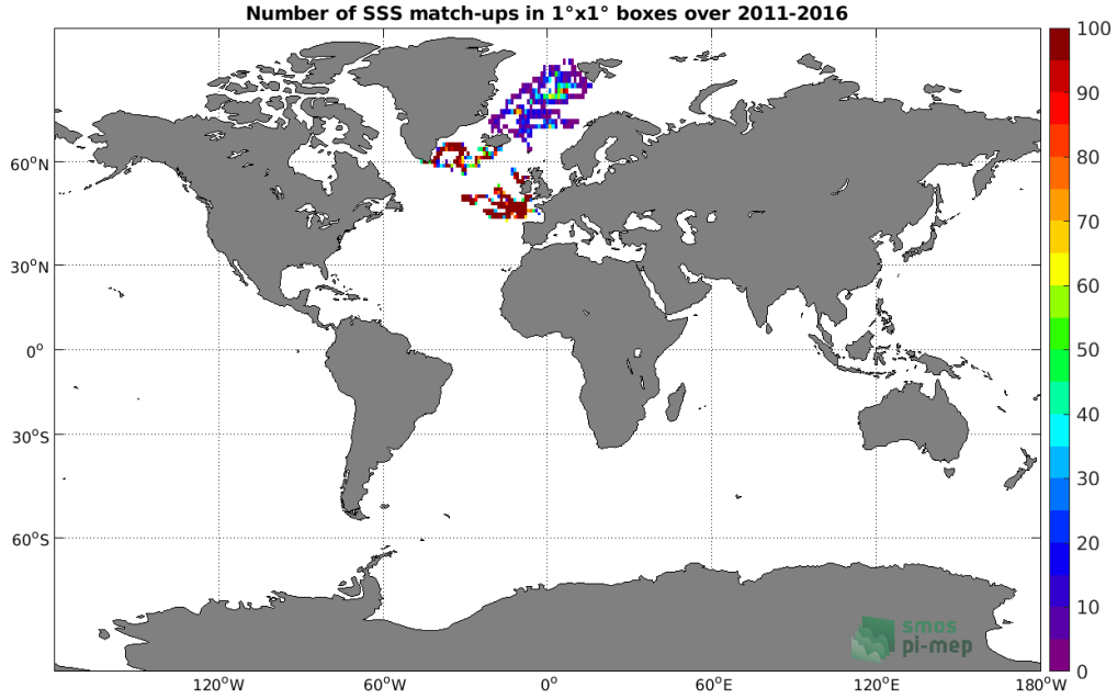
Figure 3: Number of SSS match-ups between Surface drifters SSS and the SMOS SSS L3 Arctic OA v2 - 9 Days (BEC) SSS product for the Global Ocean Pi-MEP region over 1^\circ \times 1^\circ boxes and for the full satellite product period.
