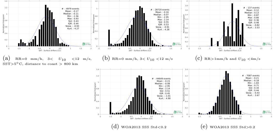
Figure 12: Normalized histogram of \Delta SSS (SMOS L3 Arctic OA v2 - 9 Days (BEC) - Surface drifters) for 5 different subdatasets corresponding to: RR=0 mm/h, 3 < U_{10} < 12 m/s, SST > 5°C, distance to coast > 800 km (a), RR=0 mm/h, 3 < U_{10} < 12 m/s (b), RR > 1mm/h and U_{10} < 4 m/s (c), WOA2013 SSS Std < 0.2 (d), WOA2013 SSS Std > 0.2 (e).
