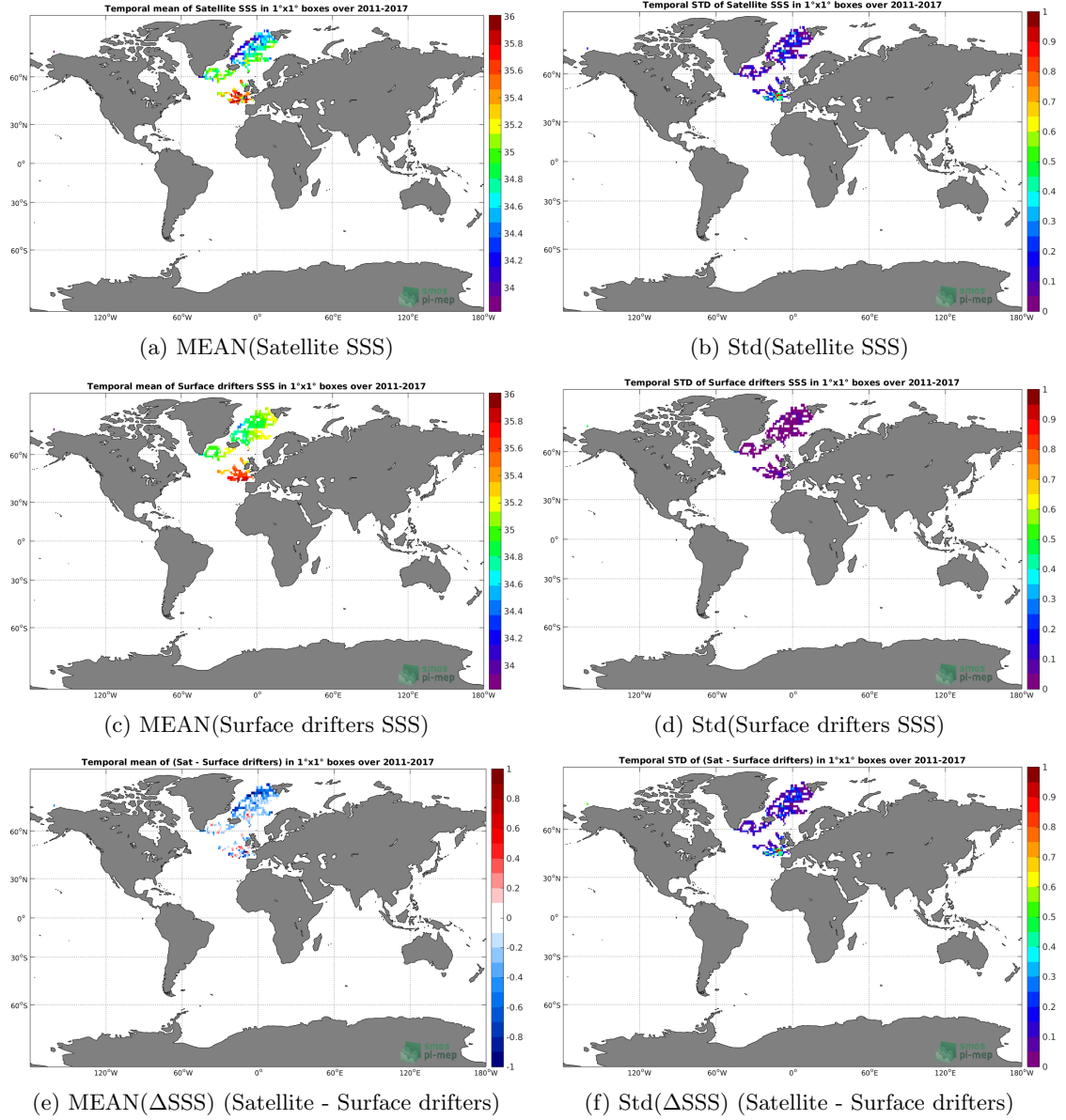
Figure 5: Temporal mean (left) and Std (right) of SSS from SMOS L3 Arctic OA v2 - 9 Days (BEC) (top), Surface drifters (middle), and of \Delta SSS (Satellite - Surface drifters). Only match-up pairs are used to generate these maps.
