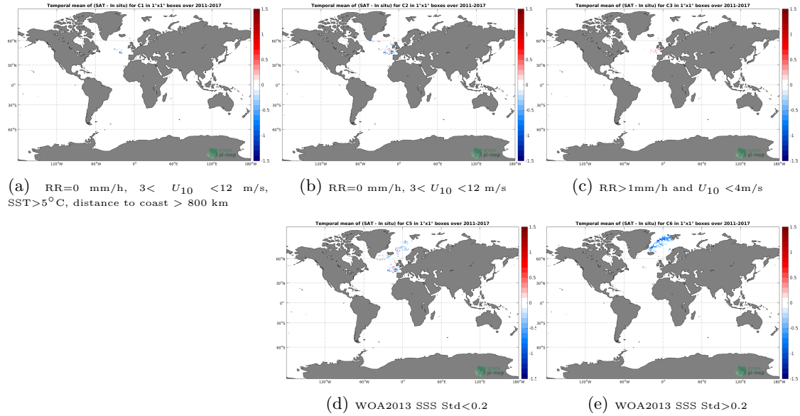
Figure 11: Temporal mean gridded over spatial boxes of size 1^{\circ}\times 1^{\circ} of \Delta\text{SSS} (SMOS L3 Arctic OA v2 - 9 Days (BEC) - Surface drifters) for 5 different subdatasets corresponding to:RR=0 mm/h, 3 < U_{10} < 12 m/s, SST >5^{\circ}\text{C} , distance to coast > 800 km (a), RR=0 mm/h, 3 < U_{10} < 12 m/s (b), RR >1 mm/h and U_{10} < 4 m/s (c), WOA2013 SSS Std <0.2 (d), WOA2013 SSS Std >0.2 (e).
