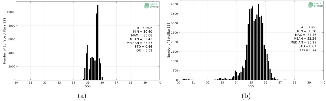
Figure 2: Histograms of SSS from Surface drifters (a) and SMOS L3 Arctic OA v2 - 9 Days (BEC) (b) considering all match-up pairs per bins of 0.1 over the Global Ocean Pi-MEP region and for the full satellite product period.
