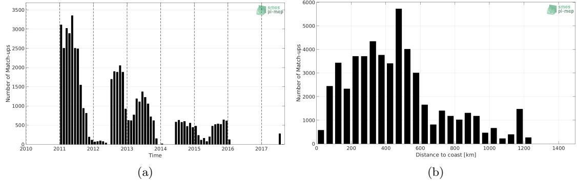
Figure 1: Number of match-ups between Surface drifters and SMOS L3 Arctic OA v2 - 9 Days (BEC) SSS as a function of time (a) and as function of the distance to coast (b) over the Global Ocean Pi-MEP region and for the full satellite product period.
