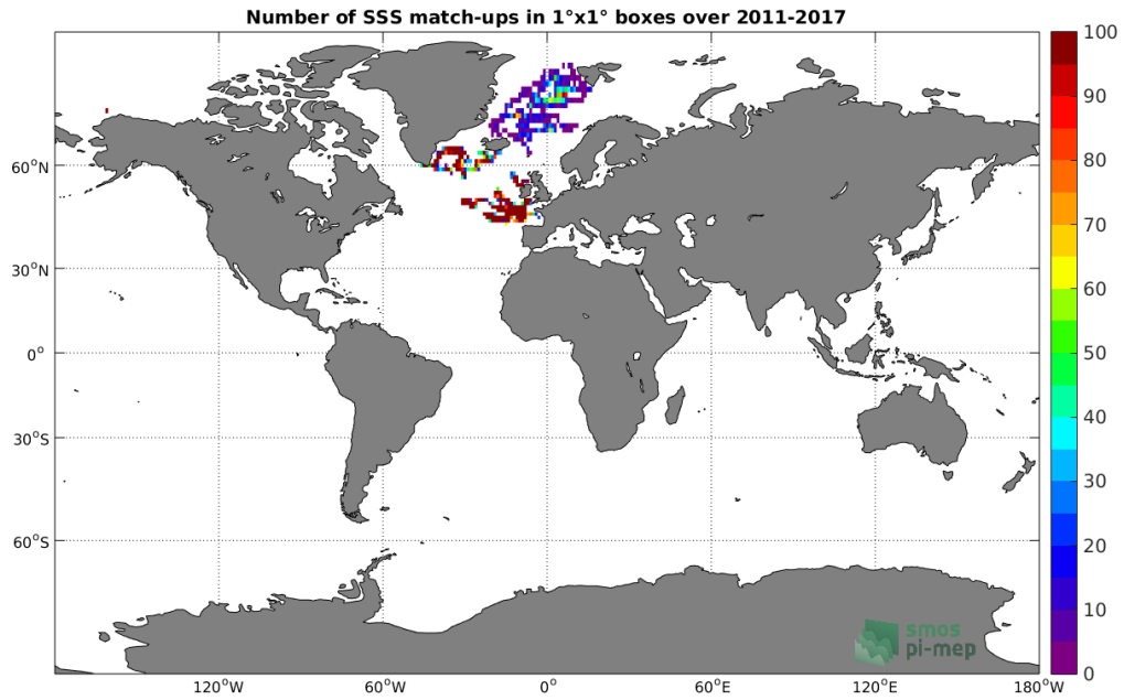
Figure 3: Number of SSS match-ups between Surface drifters SSS and the SMOS L3 Arctic OA v2 - 9 Days (BEC) SSS product for the Global Ocean Pi-MEP region over 1^\circ \times 1^\circ boxes and for the full satellite product period.
