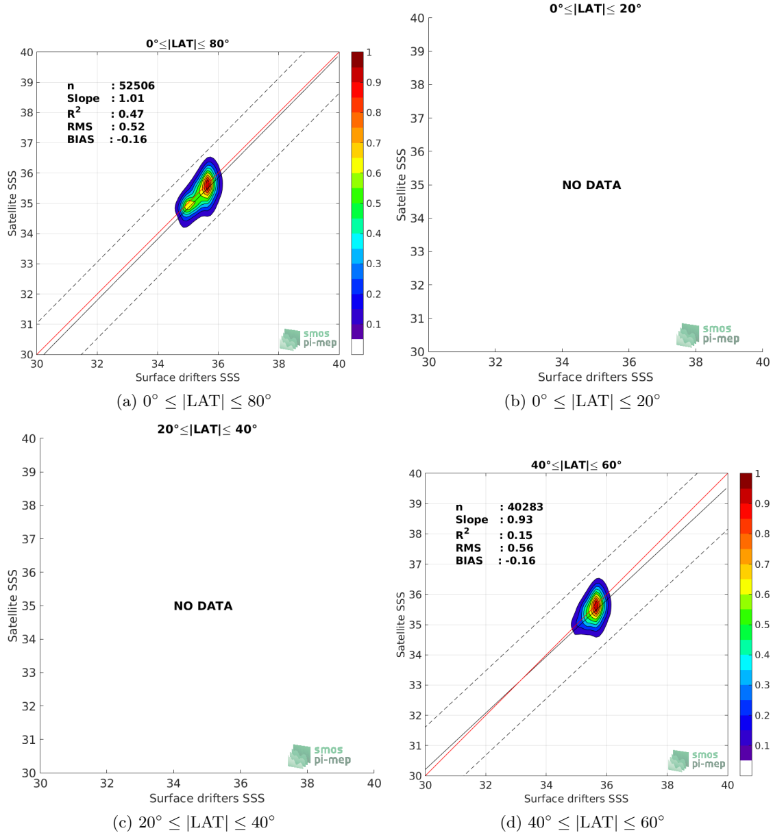
Figure 8: Contour maps of the concentration of SMOS-L3-BEC-ARCTIC-OA-V2-9DAYS-0.25DEG SSS (y-axis) versus Surface drifters SSS (x-axis) at match-up pairs for different latitude bands. For each plot, the red line shows x=y . The black thin and dashed lines indicate a linear fit through the data cloud and the \pm 95\% confidence levels, respectively. The number match-up pairs n , the slope and R^2 coefficient of the linear fit, the root mean square (RMS) and the mean bias between satellite and in situ data are indicated for each latitude band in each plots.
