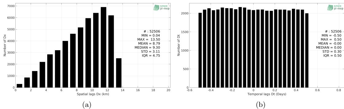
Figure 4: Histograms of the spatial (a) and temporal (b) lags between the time of the Surface drifters measurements and the date of the corresponding SMOS-L3-BEC-ARCTIC-OA-V2-9DAYS-0.25DEG SSS product.
