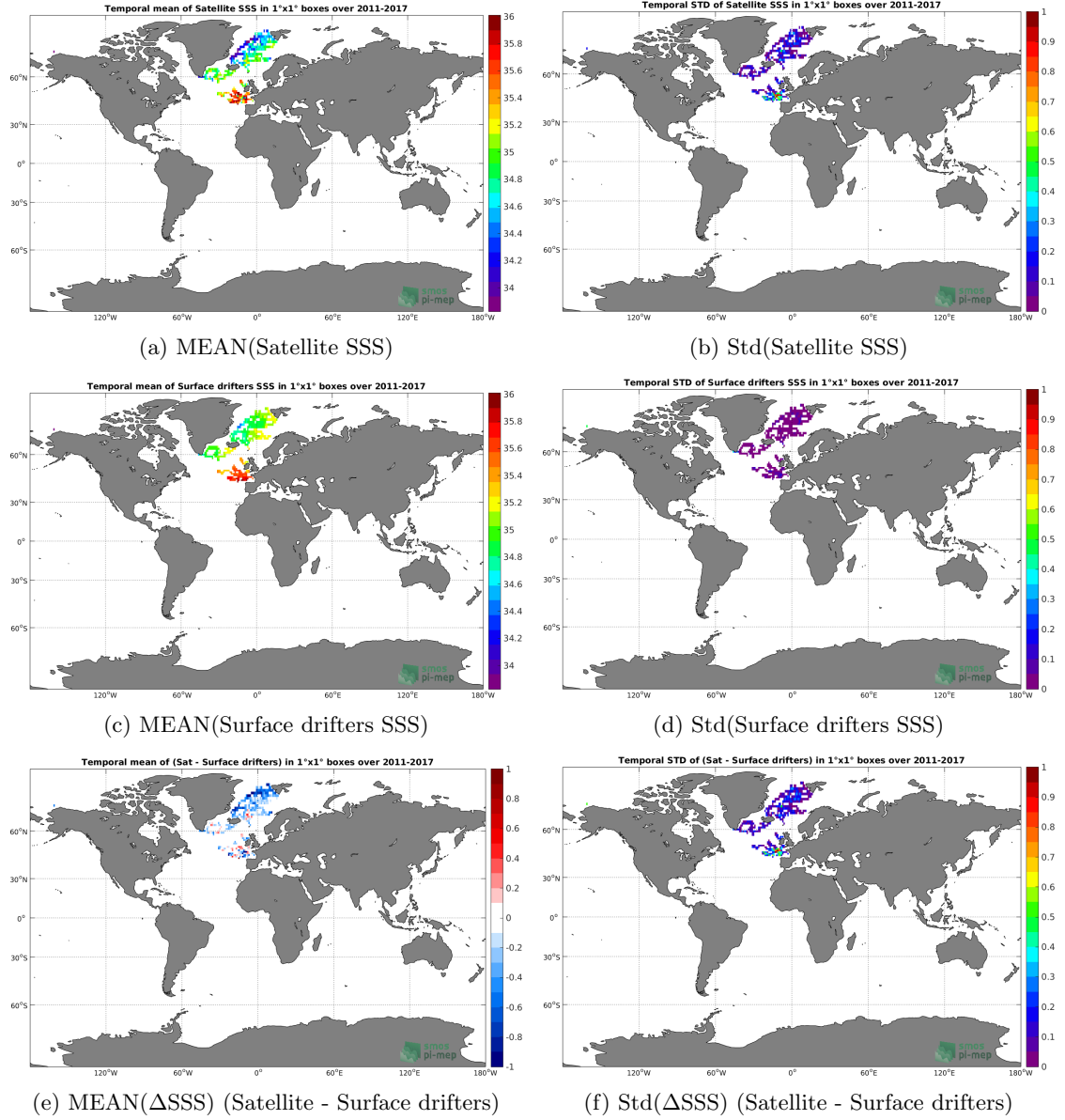
Figure 5: Temporal mean (left) and Std (right) of SSS from SMOS-L3-BEC-ARCTIC-OA-V2-9DAYS-0.25DEG (top), Surface drifters (middle), and of \Delta SSS (Satellite - Surface drifters). Only match-up pairs are used to generate these maps.
