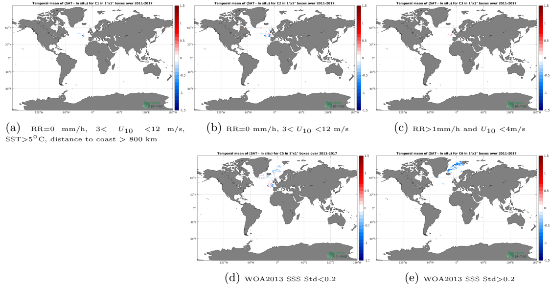
Figure 11: Temporal mean gridded over spatial boxes of size 1^\circ \times 1^\circ of \Delta SSS (SMOS-L3-BEC-ARCTIC-OA-V2-9DAYS-0.25DEG - Surface drifters) for 5 different subdatasets corresponding to: RR=0 mm/h, 3 < U_{10} < 12 m/s, SST > 5^\circ C , distance to coast > 800 km (a), RR=0 mm/h, 3 < U_{10} < 12 m/s (b), RR > 1 mm/h and U_{10} < 4 m/s (c), WOA2013 SSS Std < 0.2 (d), WOA2013 SSS Std > 0.2 (e).
