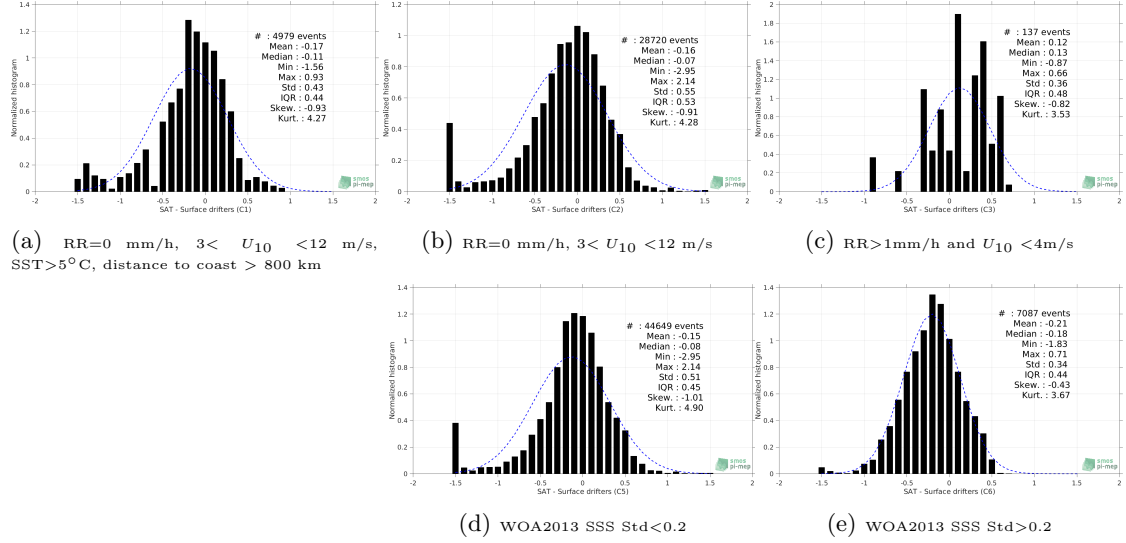
Figure 12: Normalized histogram of \Delta SSS (SMOS-L3-BEC-ARCTIC-OA-V2-9DAYS-0.25DEG - Surface drifters) for 5 different subdatasets corresponding to: RR=0 mm/h, 3 < U_{10} < 12 m/s, SST>5°C, distance to coast > 800 km (a), RR=0 mm/h, 3 < U_{10} < 12 m/s (b), RR>1mm/h and U_{10} < 4 m/s (c), WOA2013 SSS Std<0.2 (d), WOA2013 SSS Std>0.2 (e).
