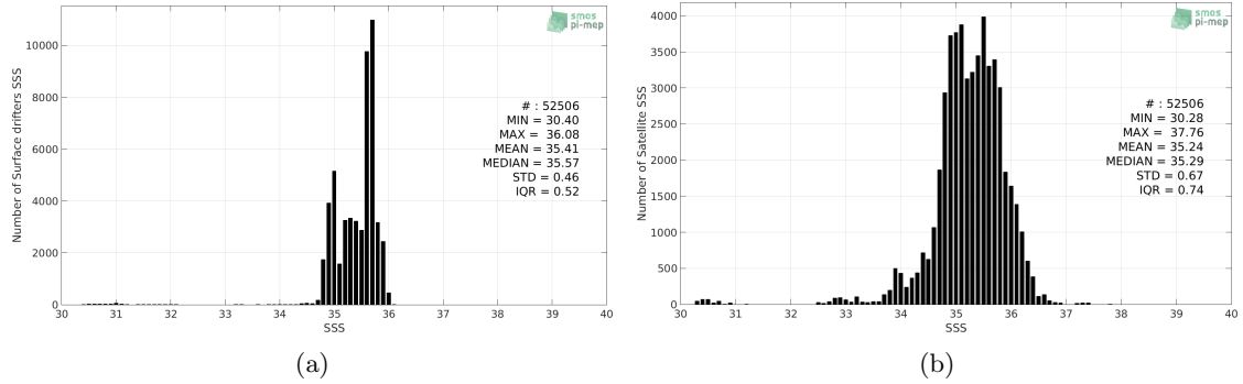
Figure 2: Histograms of SSS from Surface drifters (a) and SMOS-L3-BEC-ARCTIC-OA-V2-9DAYS-0.25DEG (b) considering all match-up pairs per bins of 0.1 over the Global Ocean Pi-MEP region and for the full satellite product period.
