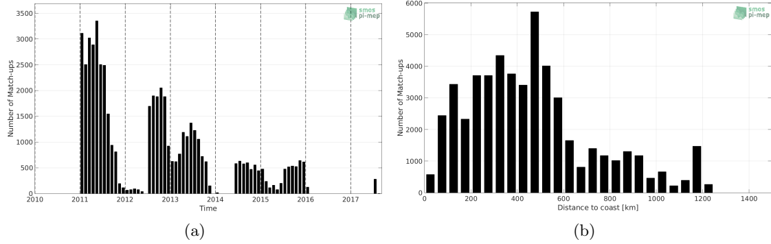
Figure 1: Number of match-ups between Surface drifters and SMOS-L3-BEC-ARCTIC-OA-V2-9DAYS-0.25DEG SSS as a function of time (a) and as function of the distance to coast (b) over the Global Ocean Pi-MEP region and for the full satellite product period.
