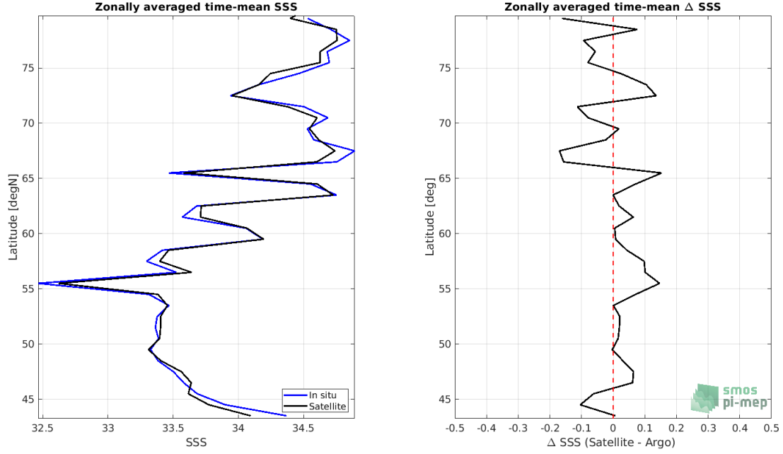
Figure 8: Left panel: Zonal mean SSS from SMOS SSS L3 Arctic OA v2 - 9 Days (BEC) satellite product (black) and from Argo (blue). Right panel: Zonal mean of \Delta SSS (Satellite - Argo) for all the collected Pi-MEP match-up pairs estimated over the full satellite product period.
