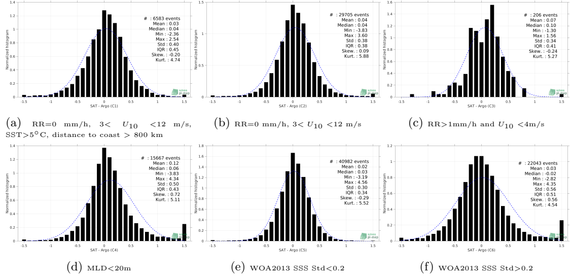
Figure 13: Normalized histogram of \Delta SSS (SMOS SSS L3 Arctic OA v2 - 9 Days (BEC) - Argo) for 6 different subdatasets corresponding to: RR=0 mm/h, 3 < U_{10} < 12 m/s, SST>5°C, distance to coast > 800 km (a), RR=0 mm/h, 3 < U_{10} < 12 m/s (b), RR>1mm/h and U_{10} < 4 m/s (c), MLD<20m (d), WOA2013 SSS Std<0.2 (e), WOA2013 SSS Std>0.2 (f).
