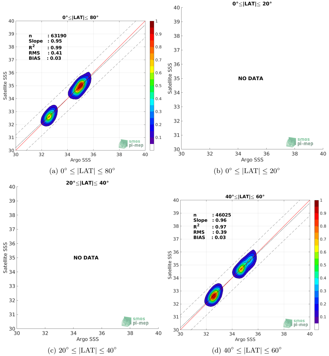
Figure 9: Contour maps of the concentration of SMOS SSS L3 Arctic OA v2 - 9 Days (BEC) SSS (y-axis) versus Argo SSS (x-axis) at match-up pairs for different latitude bands. For each plot, the red line shows x=y . The black thin and dashed lines indicate a linear fit through the data cloud and the \pm 95\% confidence levels, respectively. The number match-up pairs n , the slope and R^2 coefficient of the linear fit, the root mean square (RMS) and the mean bias between satellite and in situ data are indicated for each latitude band in each plots.
