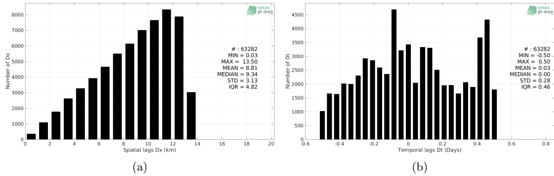
Figure 5: Histograms of the spatial (a) and temporal (b) lags between the location/time of the Argo measurement and the date of the corresponding SMOS SSS L3 Arctic OA v2 - 9 Days (BEC) SSS pixel.
