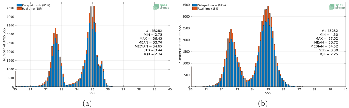
Figure 2: Histograms of SSS from Argo (a) and SMOS SSS L3 Arctic OA v2 - 9 Days (BEC) (b) considering all match-up pairs per bins of 0.1 over the Global Ocean Pi-MEP region and for the full satellite product period.
