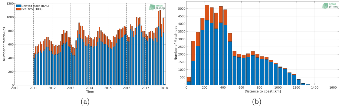
Figure 1: Number of match-ups between Argo and SMOS SSS L3 Arctic OA v2 - 9 Days (BEC) SSS as a function of time (a) and as function of the distance to coast (b) over the Global Ocean Pi-MEP region and for the full satellite product period.
