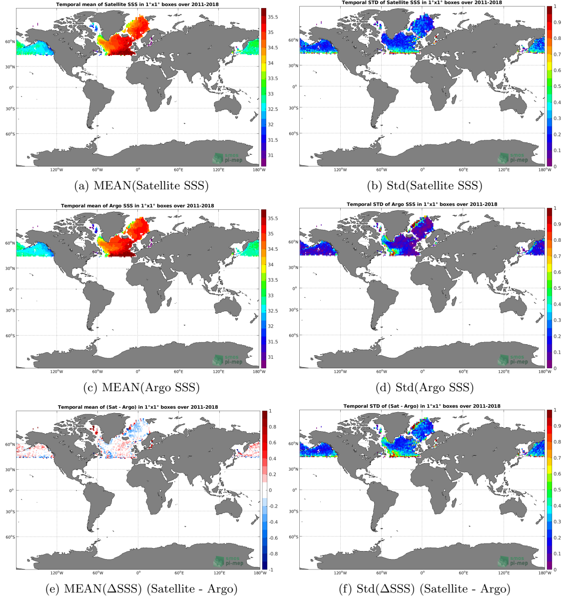
Figure 6: Temporal mean (left) and Std (right) of SSS from SMOS SSS L3 Arctic OA v2 - 9 Days (BEC) (top), Argo (middle), and of \Delta SSS (Satellite - Argo). Only match-up pairs are used to generate these maps.
