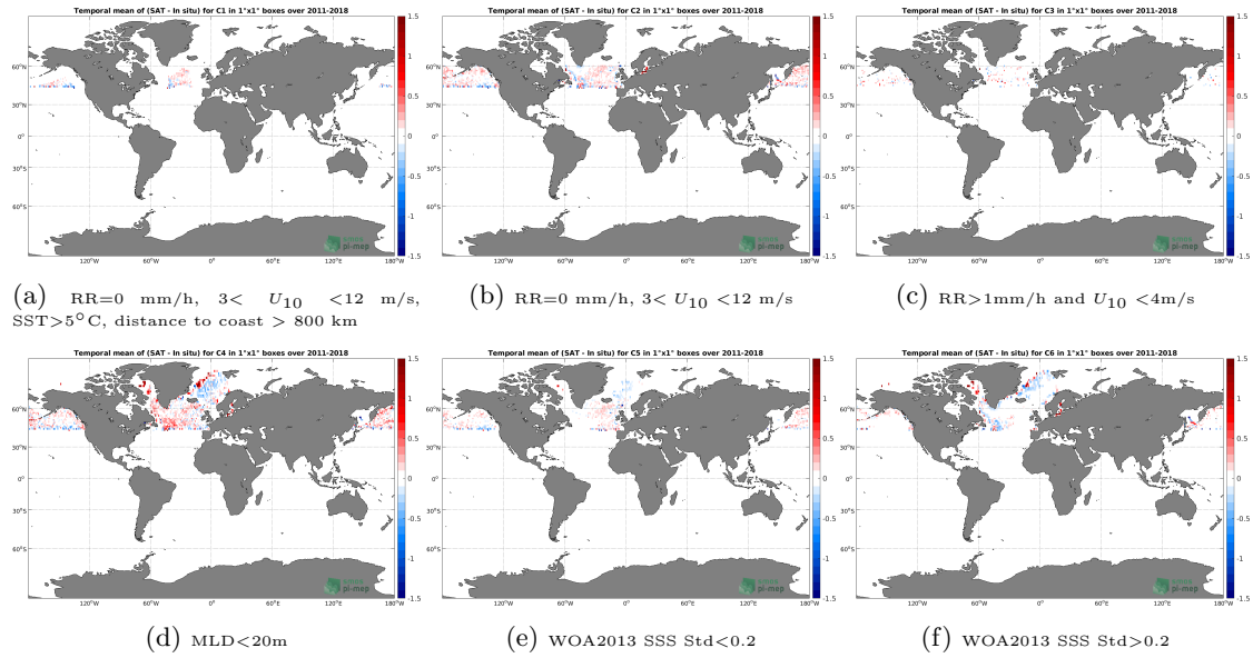
Figure 12: Temporal mean gridded over spatial boxes of size 1^{\circ} \times 1^{\circ} of \Delta\text{SSS} (SMOS SSS L3 Arctic OA v2 - 9 Days (BEC) - Argo) for 6 different subdatasets corresponding to: RR=0 mm/h, 3 < U_{10} < 12 m/s, SST > 5^{\circ}\text{C} , distance to coast > 800 km (a), RR=0 mm/h, 3 < U_{10} < 12 m/s (b), RR > 1\text{mm/h} and U_{10} < 4\text{m/s} (c), MLD < 20\text{m} (d), WOA2013 SSS Std < 0.2 (e), WOA2013 SSS Std > 0.2 (f).
