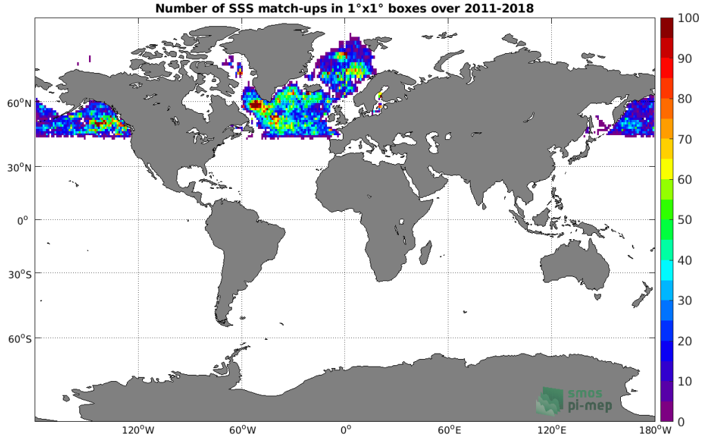
Figure 4: Number of SSS match-ups between Argo SSS and the SMOS SSS L3 Arctic OA v2 - 9 Days (BEC) SSS product for the Global Ocean Pi-MEP region over 1^\circ \times 1^\circ boxes and for the full satellite product period.
