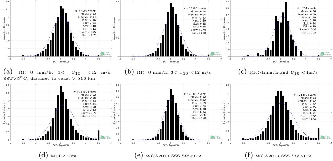
Figure 13: Normalized histogram of \Delta SSS (SMOS L3 Arctic OA v2 - 9 Days (BEC) - Argo) for 6 different subdatasets corresponding to: RR=0 mm/h, 3 < U_{10} < 12 m/s, SST>5°C, distance to coast > 800 km (a), RR=0 mm/h, 3 < U_{10} < 12 m/s (b), RR>1mm/h and U_{10} < 4 m/s (c), MLD<20m (d), WOA2013 SSS Std<0.2 (e), WOA2013 SSS Std>0.2 (f).
