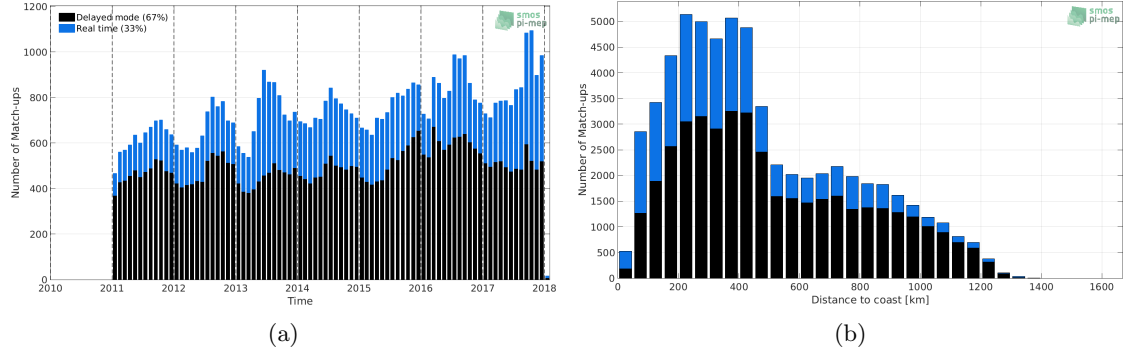
Figure 1: Number of match-ups between Argo and SMOS L3 Arctic OA v2 - 9 Days (BEC) SSS as a function of time (a) and as function of the distance to coast (b) over the Global Ocean Pi-MEP region and for the full satellite product period.
