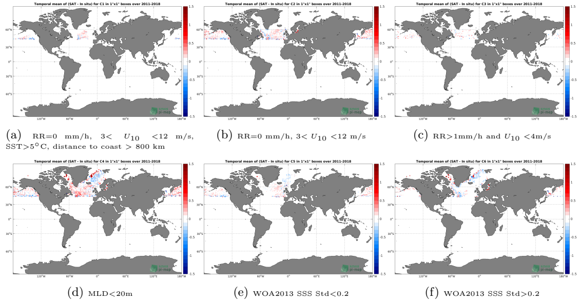
Figure 12: Temporal mean gridded over spatial boxes of size 1^{\circ}\times 1^{\circ} of \Delta\text{SSS} (SMOS L3 Arctic OA v2 - 9 Days (BEC) - Argo) for 6 different subdatasets corresponding to: \text{RR}=0 mm/h, 3 < U_{10} < 12 m/s, \text{SST} > 5^{\circ}\text{C} , distance to coast > 800 km (a), \text{RR}=0 mm/h, 3 < U_{10} < 12 m/s (b), \text{RR} > 1\text{mm/h} and U_{10} < 4\text{m/s} (c), \text{MLD} < 20\text{m} (d), \text{WOA2013 SSS Std} < 0.2 (e), \text{WOA2013 SSS Std} > 0.2 (f).
