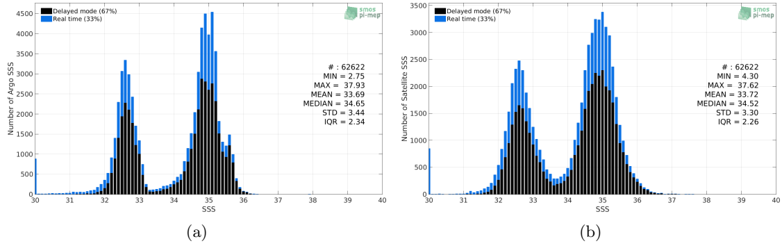
Figure 2: Histograms of SSS from Argo (a) and SMOS L3 Arctic OA v2 - 9 Days (BEC) (b) considering all match-up pairs per bins of 0.1 over the Global Ocean Pi-MEP region and for the full satellite product period.
