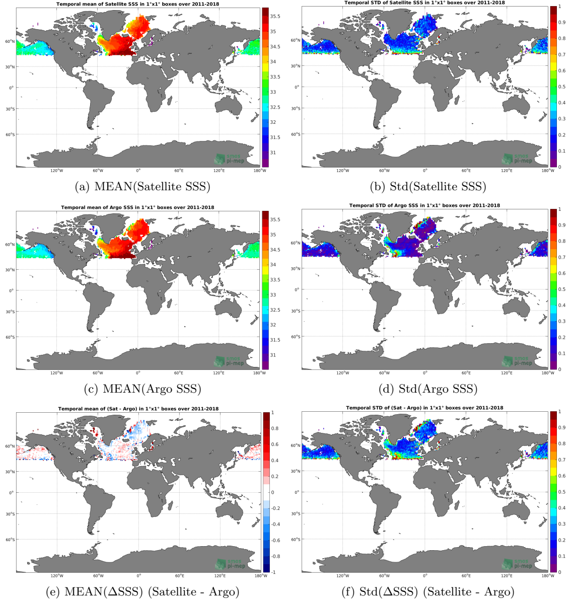
Figure 6: Temporal mean (left) and Std (right) of SSS from SMOS L3 Arctic OA v2 - 9 Days (BEC) (top), Argo (middle), and of \Delta SSS (Satellite - Argo). Only match-up pairs are used to generate these maps.
