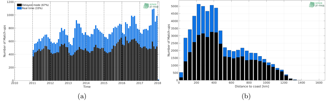
Figure 1: Number of match-ups between Argo and SMOS-L3-BEC-ARCTIC-OA-V2-9DAYS-0.25DEG SSS as a function of time (a) and as function of the distance to coast (b) over the Global Ocean Pi-MEP region and for the full satellite product period.
