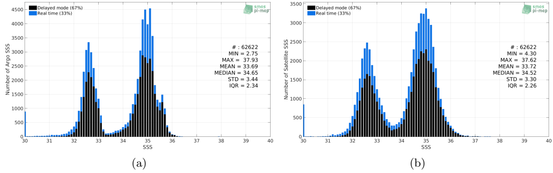
Figure 2: Histograms of SSS from Argo (a) and SMOS-L3-BEC-ARCTIC-OA-V2-9DAYS-0.25DEG (b) considering all match-up pairs per bins of 0.1 over the Global Ocean Pi-MEP region and for the full satellite product period.
