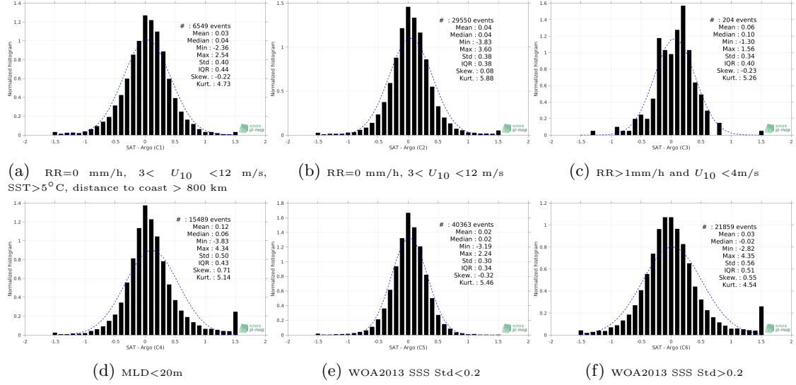
Figure 13: Normalized histogram of \Delta SSS (SMOS-L3-BEC-ARCTIC-OA-V2-9DAYS-0.25DEG - Argo) for 6 different subdatasets corresponding to: RR=0 mm/h, 3 < U_{10} < 12 m/s, SST>5°C, distance to coast > 800 km (a), RR=0 mm/h, 3 < U_{10} < 12 m/s (b), RR>1mm/h and U_{10} < 4 m/s (c), MLD<20m (d), WOA2013 SSS Std<0.2 (e), WOA2013 SSS Std>0.2 (f).
