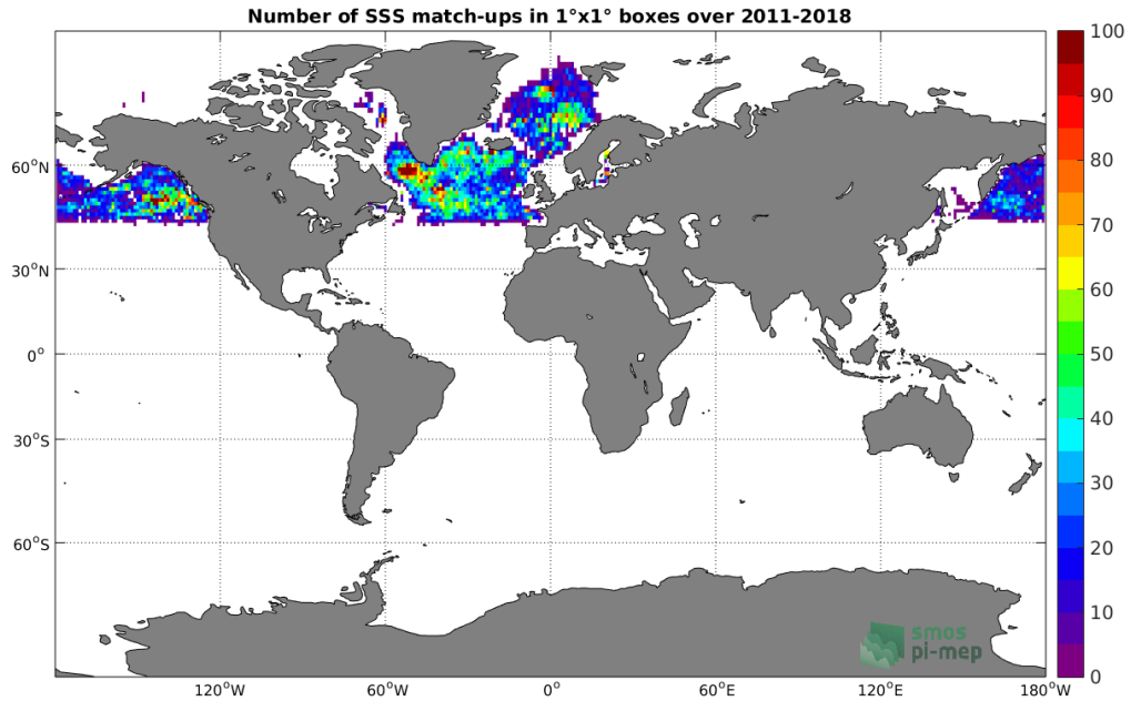
Figure 4: Number of SSS match-ups between Argo SSS and the SMOS-L3-BEC-ARCTIC-OA-V2-9DAYS-0.25DEG SSS product for the Global Ocean Pi-MEP region over 1°x1° boxes and for the full satellite product period.
