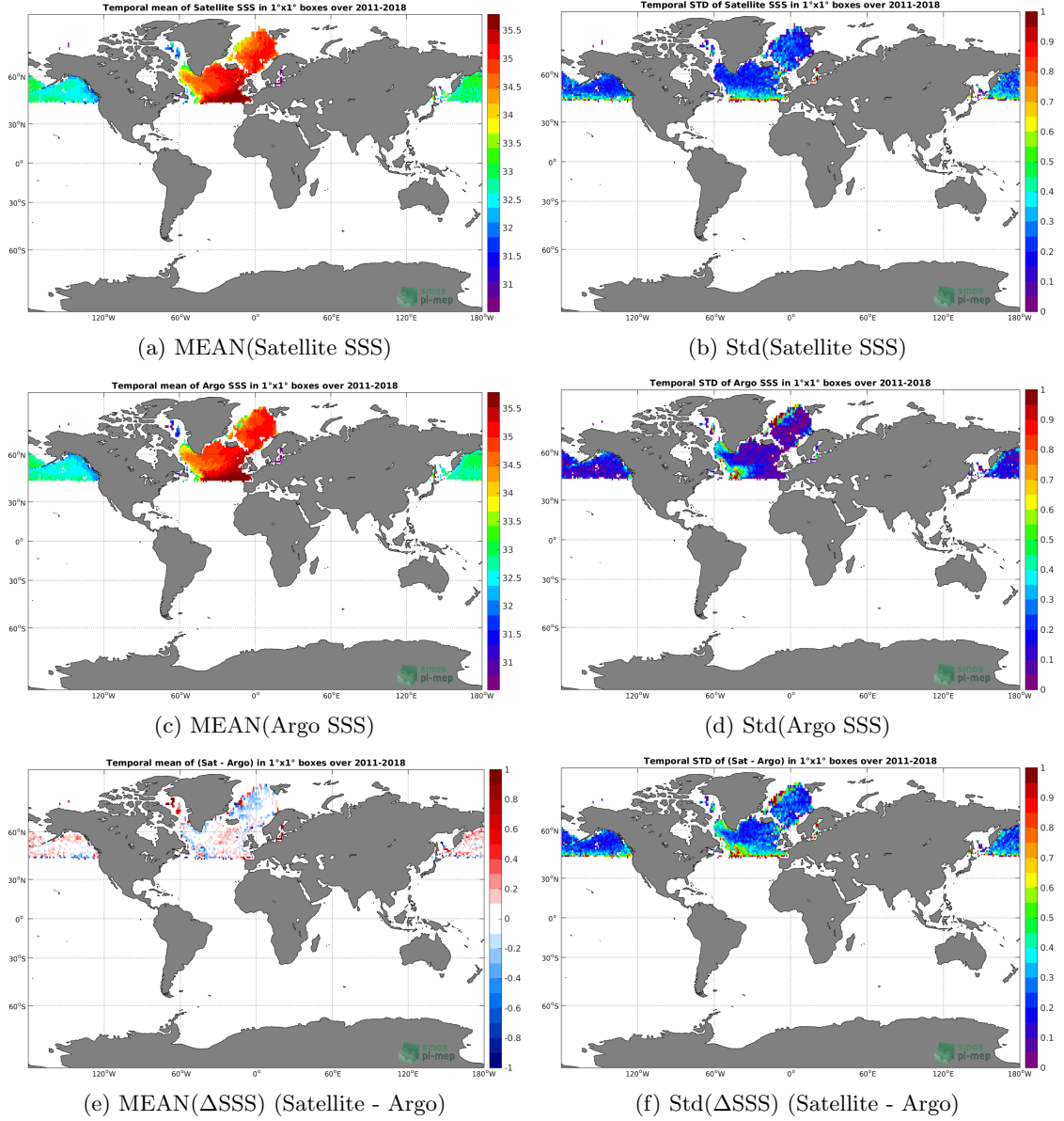
Figure 6: Temporal mean (left) and Std (right) of SSS from SMOS-L3-BEC-ARCTIC-OA-V2-9DAYS-0.25DEG (top), Argo (middle), and of \Delta SSS (Satellite - Argo). Only match-up pairs are used to generate these maps.
