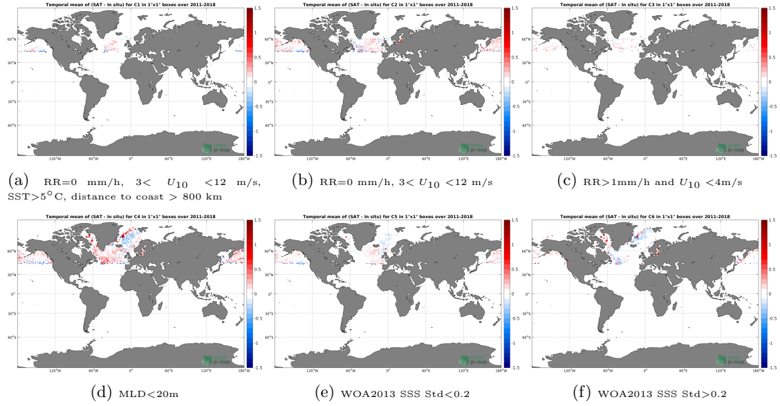
Figure 12: Temporal mean gridded over spatial boxes of size 1^\circ \times 1^\circ of \Delta SSS (SMOS-L3-BEC-ARCTIC-OA-V2-9DAYS-0.25DEG - Argo) for 6 different subdatasets corresponding to: RR=0 mm/h, 3 < U_{10} < 12 m/s, SST >5^\circ C, distance to coast > 800 km (a), RR=0 mm/h, 3 < U_{10} < 12 m/s (b), RR >1 mm/h and U_{10} < 4 m/s (c),MLD <20 m (d),WOA2013 SSS Std <0.2 (e),WOA2013 SSS Std >0.2 (f).
