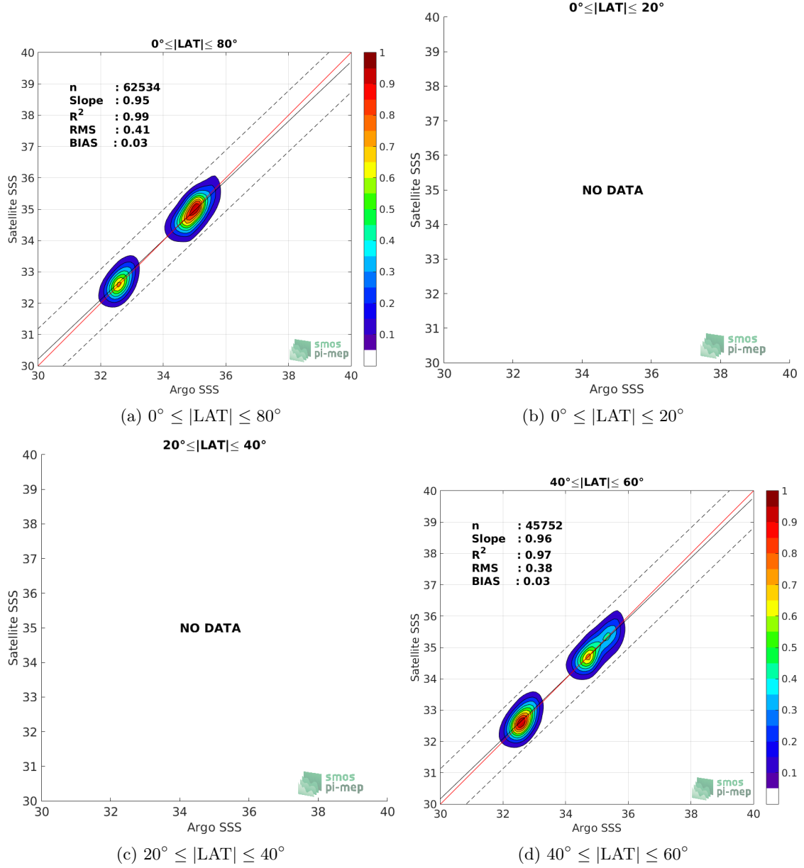
Figure 9: Contour maps of the concentration of SMOS-L3-BEC-ARCTIC-OA-V2-9DAYS-0.25DEG SSS (y-axis) versus Argo SSS (x-axis) at match-up pairs for different latitude bands. For each plot, the red line shows x=y . The black thin and dashed lines indicate a linear fit through the data cloud and the \pm 95\% confidence levels, respectively. The number match-up pairs n , the slope and R^2 coefficient of the linear fit, the root mean square (RMS) and the mean bias between satellite and in situ data are indicated for each latitude band in each plots.
