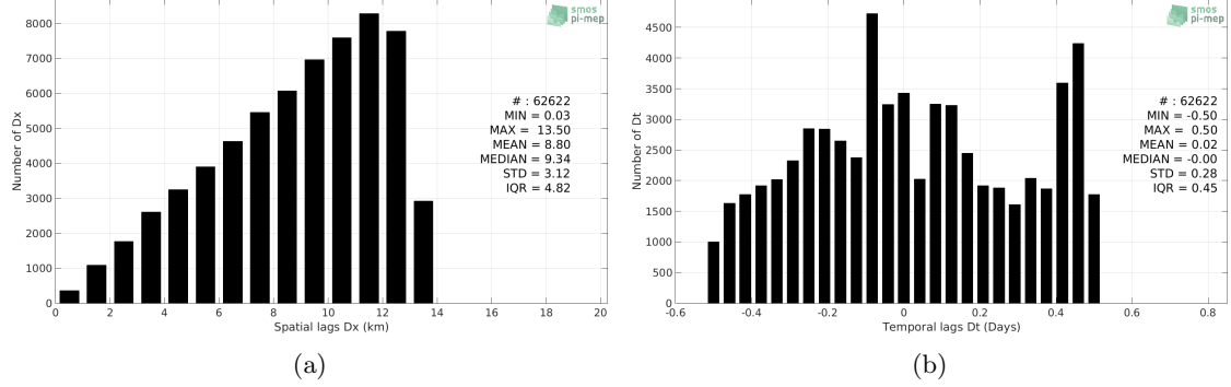
Figure 5: Histograms of the spatial (a) and temporal (b) lags between the time of the Argo measurements and the date of the corresponding SMOS-L3-BEC-ARCTIC-OA-V2-9DAYS-0.25DEG SSS product.
