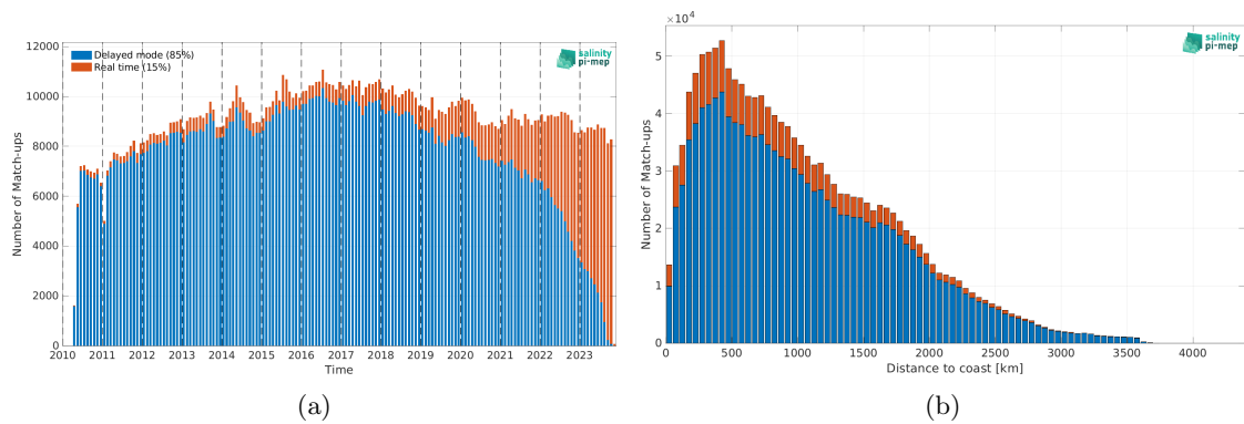
Figure 1: Number of match-ups between Argo and SMOS SSS L2-AVERAGED v700 (ESA) SSS as a function of time (a) and as function of the distance to coast (b) over the Global Ocean Pi-MEP region and for the full satellite product period.
