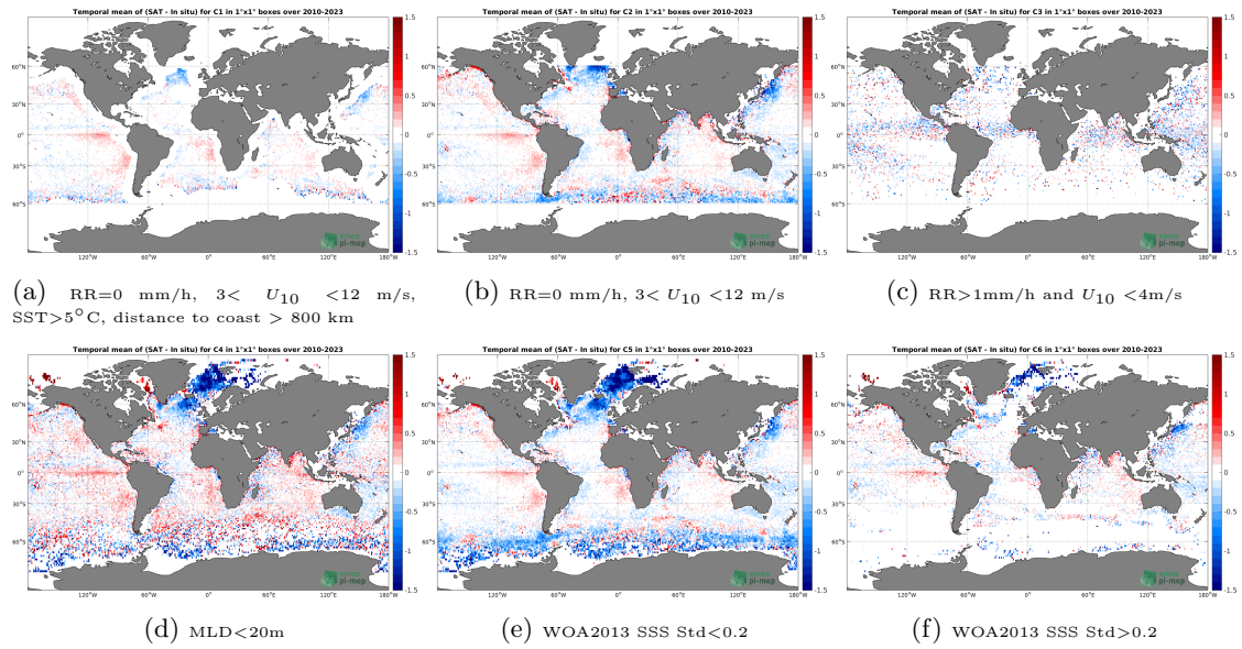
Figure 12: Temporal mean gridded over spatial boxes of size 1^\circ \times 1^\circ of \Delta SSS (SMOS SSS L2-AVERAGED v700 (ESA) - Argo) for 6 different subdatasets corresponding to: RR=0 mm/h, 3 < U_{10} < 12 m/s, SST > 5^\circ\text{C} , distance to coast > 800 km (a), RR=0 mm/h, 3 < U_{10} < 12 m/s (b), RR > 1 mm/h and U_{10} < 4 m/s (c), MLD < 20 m (d), WOA2013 SSS Std < 0.2 (e), WOA2013 SSS Std > 0.2 (f).
