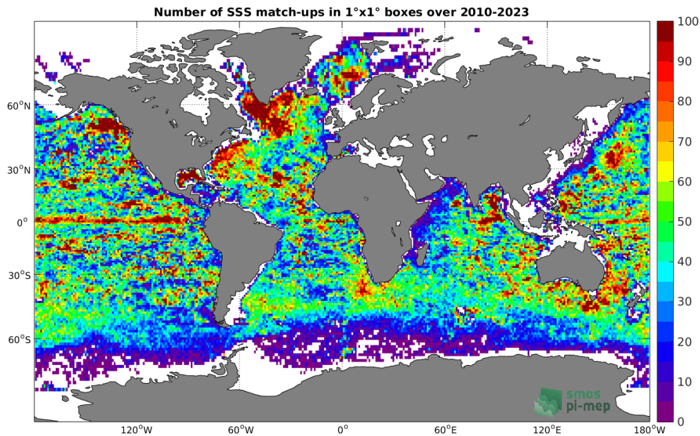
Figure 4: Number of SSS match-ups between Argo SSS and the SMOS SSS L2-AVERAGED v700 (ESA) SSS product for the Global Ocean Pi-MEP region over 1^\circ \times 1^\circ boxes and for the full satellite product period.
