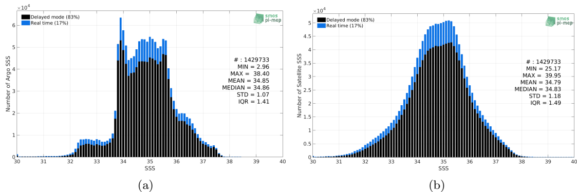
Figure 2: Histograms of SSS from Argo (a) and SMOS SSS L2-AVERAGED v700 (ESA) (b) considering all match-up pairs per bins of 0.1 over the Global Ocean Pi-MEP region and for the full satellite product period.
