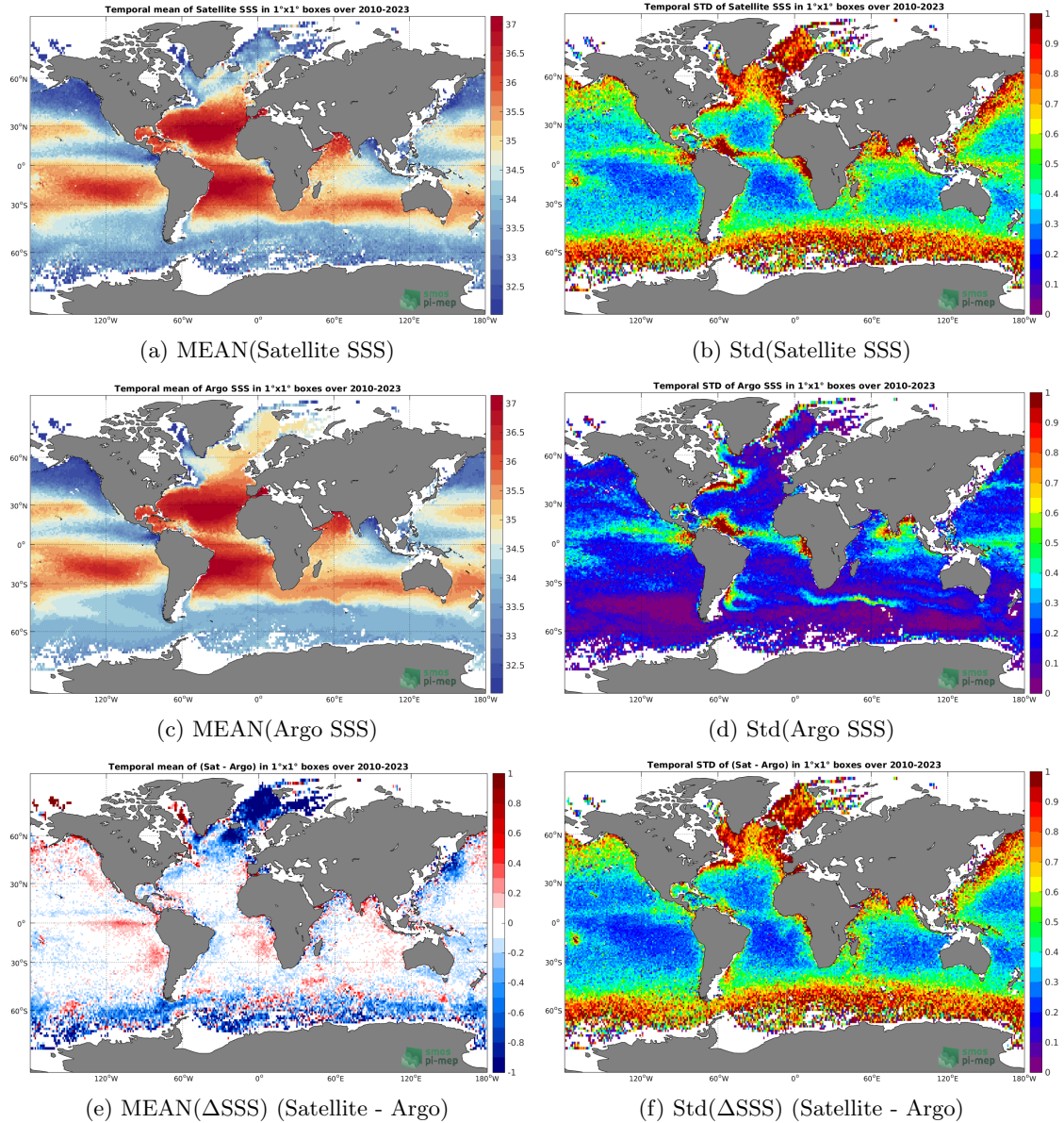
Figure 6: Temporal mean (left) and Std (right) of SSS from SMOS SSS L2-AVERAGED v700 (ESA) (top), Argo (middle), and of \Delta SSS (Satellite - Argo). Only match-up pairs are used to generate these maps.
