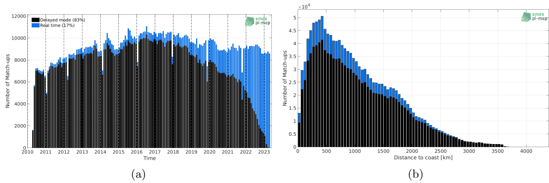
Figure 1: Number of match-ups between Argo and SMOS SSS L2-AVERAGED v700 (ESA) SSS as a function of time (a) and as function of the distance to coast (b) over the Global Ocean Pi-MEP region and for the full satellite product period.
