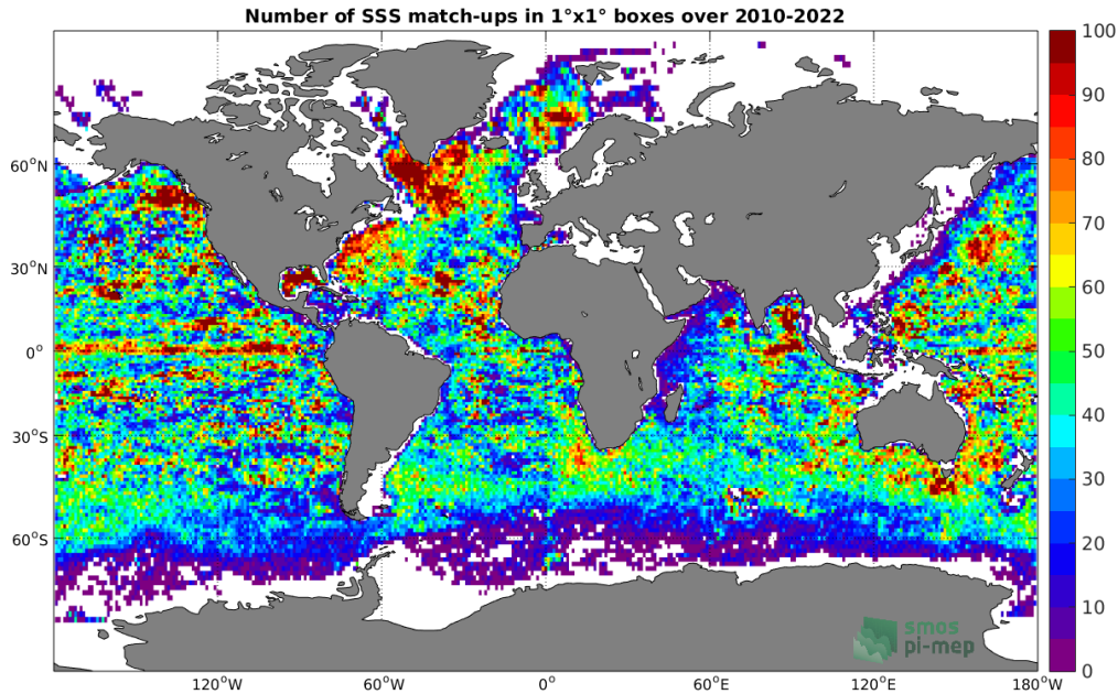
Figure 4: Number of SSS match-ups between Argo SSS and the SMOS SSS L2-AVERAGED v700 (ESA) SSS product for the Global Ocean Pi-MEP region over 1^\circ \times 1^\circ boxes and for the full satellite product period.
