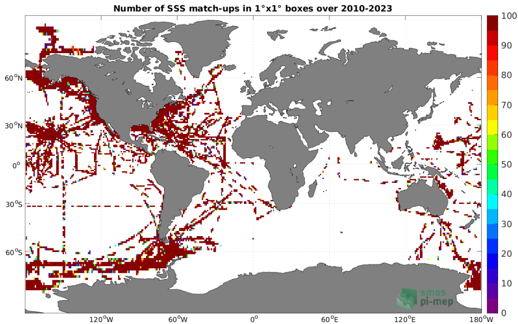
Figure 4: Number of SSS match-ups between TSG (SAMOS) SSS and the SMOS SSS L2 v700 (ESA) SSS product for the Global Ocean Pi-MEP region over 1^\circ \times 1^\circ boxes and for the full satellite product period.
