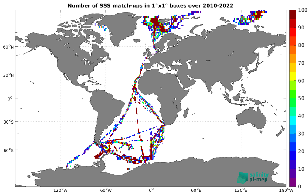
Figure 4: Number of SSS match-ups between TSG (Polarstern) SSS and the SMOS SSS L2 v700 (ESA) SSS product for the Global Ocean Pi-MEP region over 1^\circ \times 1^\circ boxes and for the full satellite product period.
