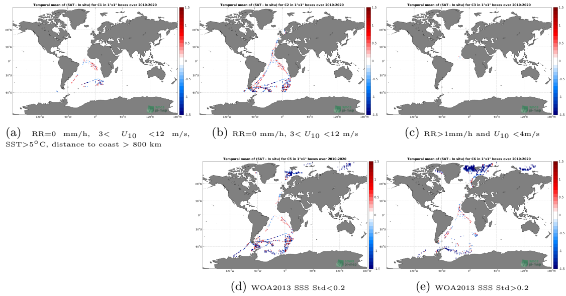
Figure 12: Temporal mean gridded over spatial boxes of size 1^\circ \times 1^\circ of \Delta SSS (SMOS SSS L2 v700 (ESA) - TSG (Polarstern)) for 5 different subdatasets corresponding to: RR=0 mm/h, 3 < U_{10} < 12 m/s, SST > 5^\circ C , distance to coast > 800 km (a), RR=0 mm/h, 3 < U_{10} < 12 m/s (b), RR > 1 mm/h and U_{10} < 4 m/s (c), WOA2013 SSS Std < 0.2 (d), WOA2013 SSS Std > 0.2 (e).
