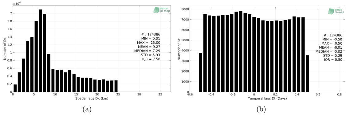
Figure 5: Histograms of the spatial (a) and temporal (b) lags between the location/time of the TSG (Polarstern) measurement and the date of the corresponding SMOS SSS L2 v700 (ESA) SSS pixel.
