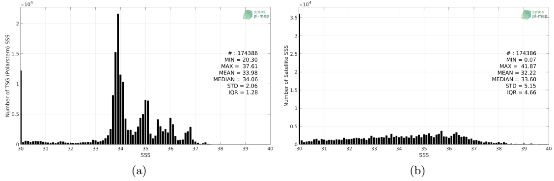
Figure 2: Histograms of SSS from TSG (Polarstern) (a) and SMOS SSS L2 v700 (ESA) (b) considering all match-up pairs per bins of 0.1 over the Global Ocean Pi-MEP region and for the full satellite product period.
