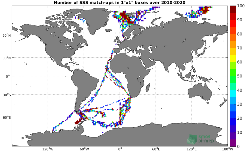
Figure 4: Number of SSS match-ups between TSG (Polarstern) SSS and the SMOS SSS L2 v700 (ESA) SSS product for the Global Ocean Pi-MEP region over 1^\circ \times 1^\circ boxes and for the full satellite product period.
