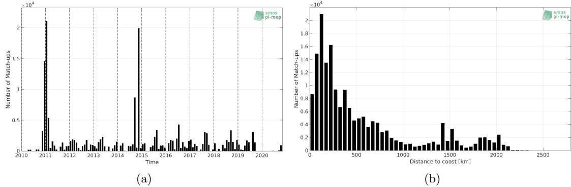
Figure 1: Number of match-ups between TSG (Polarstern) and SMOS SSS L2 v700 (ESA) SSS as a function of time (a) and as function of the distance to coast (b) over the Global Ocean Pi-MEP region and for the full satellite product period.
