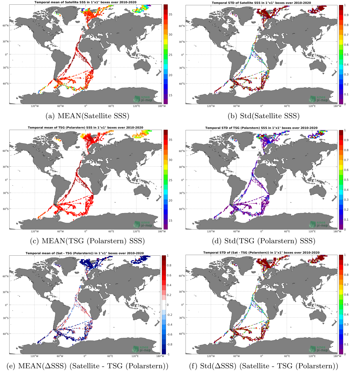
Figure 6: Temporal mean (left) and Std (right) of SSS from SMOS SSS L2 v700 (ESA) (top), TSG (Polarstern) (middle), and of \Delta SSS (Satellite - TSG (Polarstern)). Only match-up pairs are used to generate these maps.
