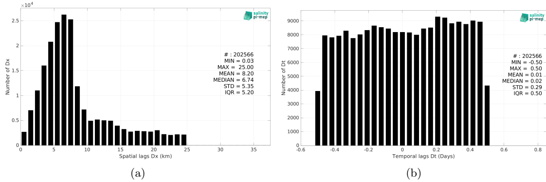
Figure 6: Histograms of the spatial (a) and temporal (b) lags between the location/time of the TSG (NCEI-0170743) measurement and the date of the corresponding SMOS SSS L2 v700 (ESA) SSS pixel.
