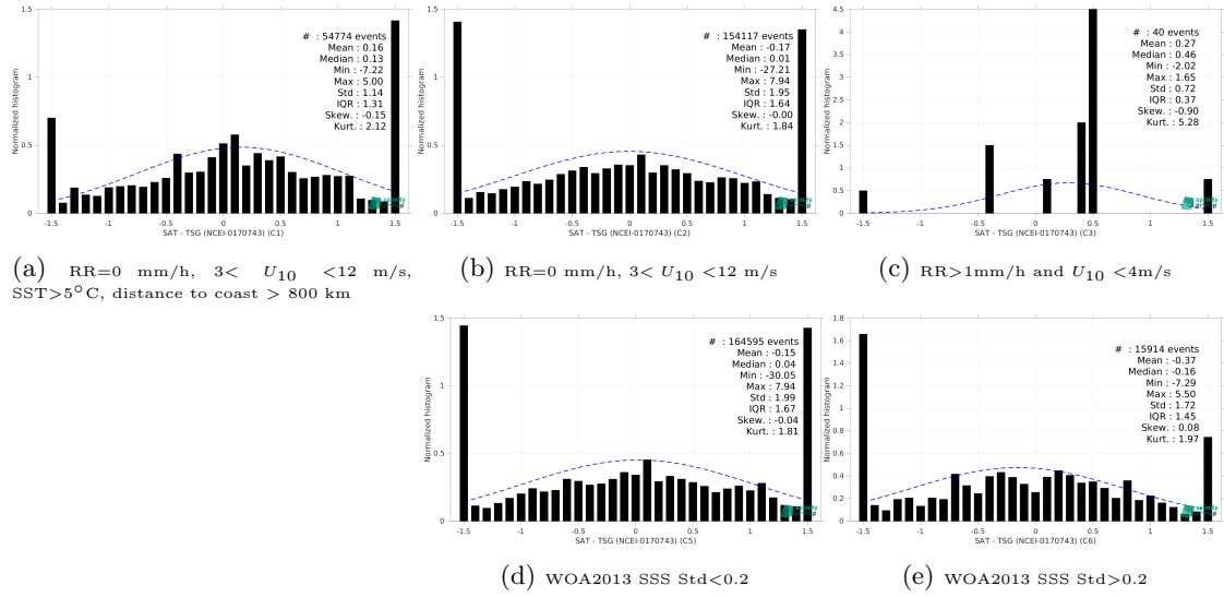
Figure 15: Normalized histogram of \Delta SSS (SMOS SSS L2 v700 (ESA) - TSG (NCEI-0170743)) for 5 different subdatasets corresponding to: RR=0 mm/h, 3 < U_{10} < 12 m/s, SST > 5°C, distance to coast > 800 km (a), RR=0 mm/h, 3 < U_{10} < 12 m/s (b), RR > 1mm/h and U_{10} < 4 m/s (c), WOA2013 SSS Std < 0.2 (d), WOA2013 SSS Std > 0.2 (e).
