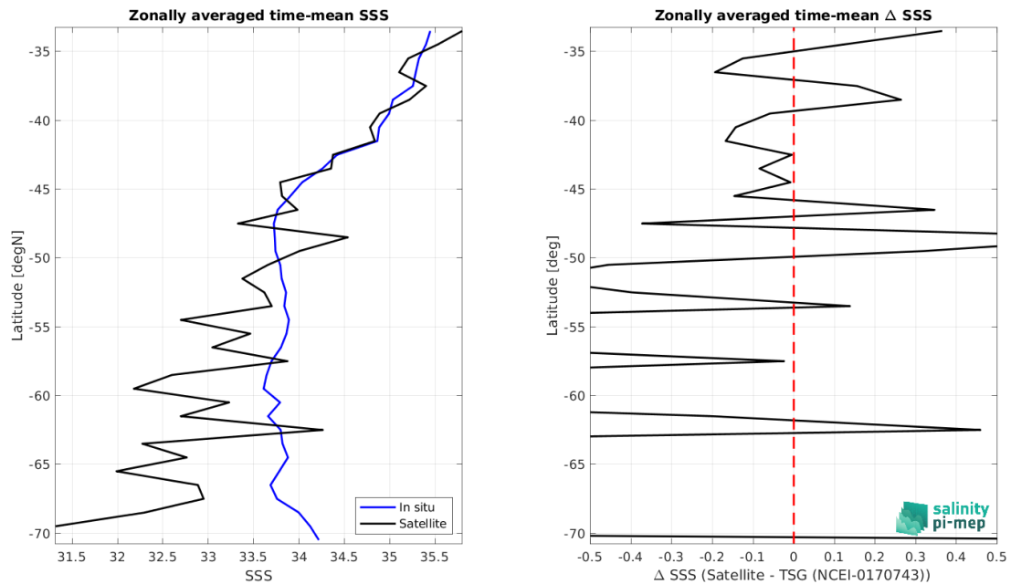
Figure 9: Left panel: Zonal mean SSS from SMOS SSS L2 v700 (ESA) satellite product (black) and from TSG (NCEI-0170743) (blue). Right panel: Zonal mean of \Delta SSS (Satellite - TSG (NCEI-0170743)) for all the collected Pi-MEP match-up pairs estimated over the full satellite product period.
