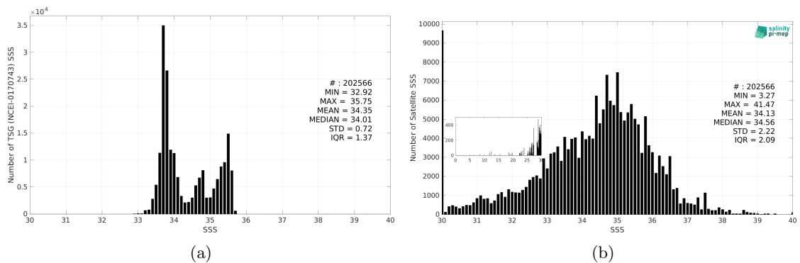
Figure 3: Histograms of SSS from TSG (NCEI-0170743) (a) and SMOS SSS L2 v700 (ESA) (b) considering all match-up pairs per bins of 0.1 over the Global Ocean Pi-MEP region and for the full satellite product period.
