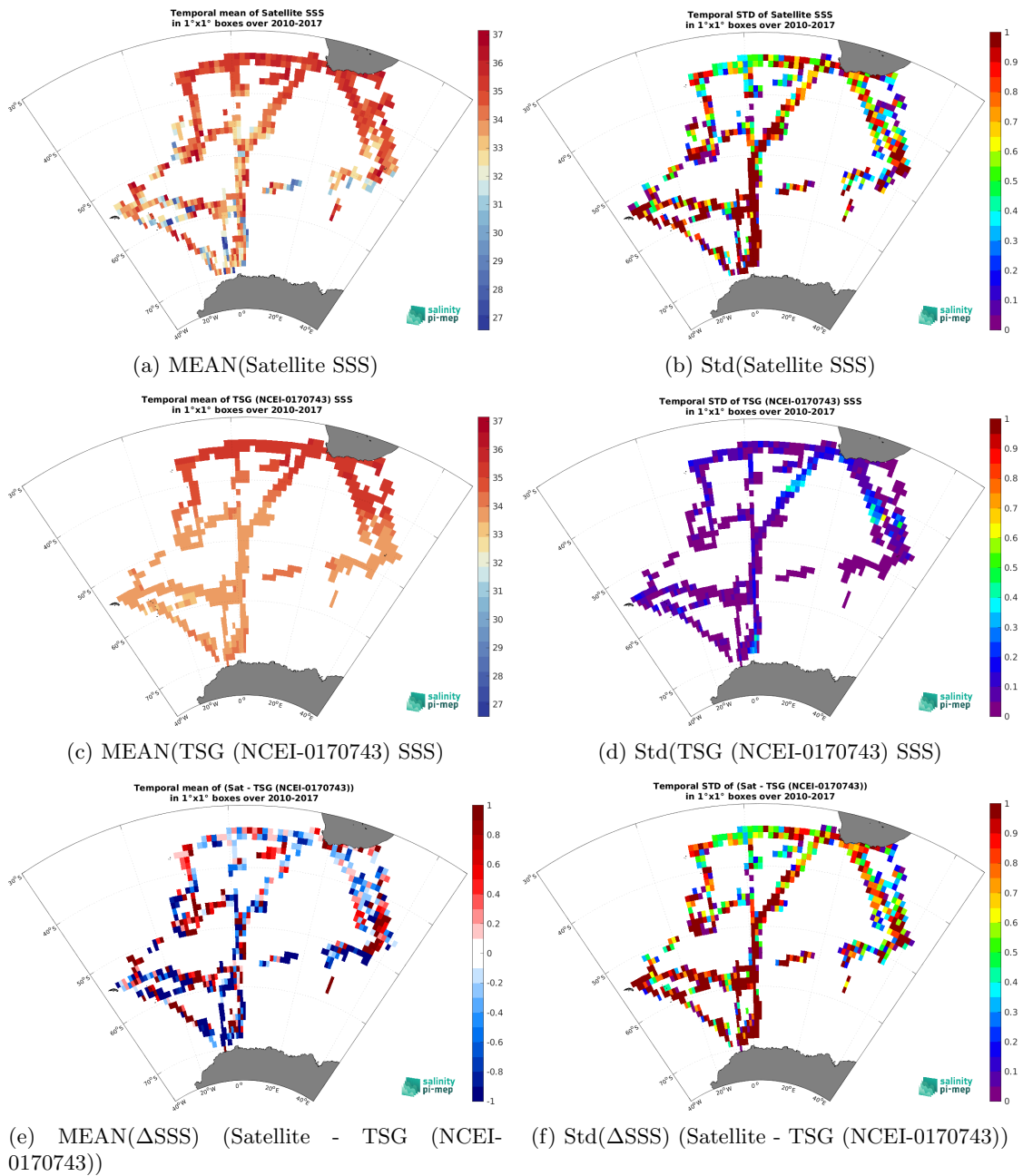
Figure 7: Temporal mean (left) and Std (right) of SSS from SMOS SSS L2 v700 (ESA) (top), TSG (NCEI-0170743) (middle), and of \Delta SSS (Satellite - TSG (NCEI-0170743)). Only match-up pairs are used to generate these maps.
