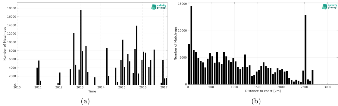
Figure 2: Number of match-ups between TSG (NCEI-0170743) and SMOS SSS L2 v700 (ESA) SSS as a function of time (a) and as function of the distance to coast (b) over the Global Ocean Pi-MEP region and for the full satellite product period.
