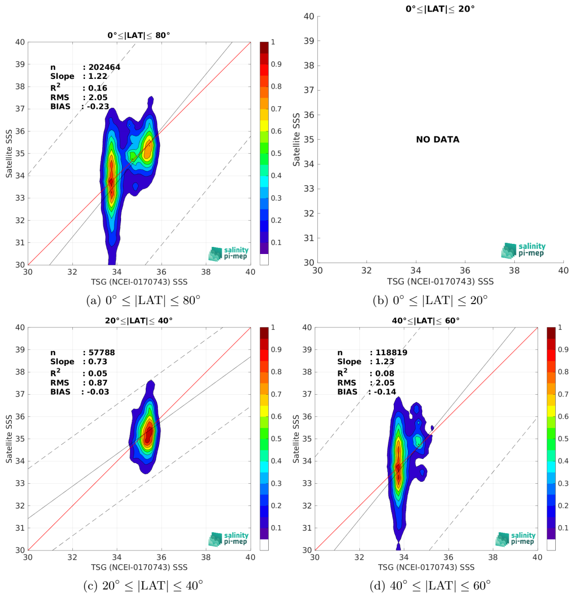
Figure 10: Contour maps of the concentration of SMOS SSS L2 v700 (ESA) SSS (y-axis) versus TSG (NCEI-0170743) SSS (x-axis) at match-up pairs for different latitude bands. For each plot, the red line shows x=y . The black thin and dashed lines indicate a linear fit through the data cloud and the \pm 95\% confidence levels, respectively. The number match-up pairs n , the slope and R^2 coefficient of the linear fit, the root mean square (RMS) and the mean bias between satellite and in situ data are indicated for each latitude band in each plots.
