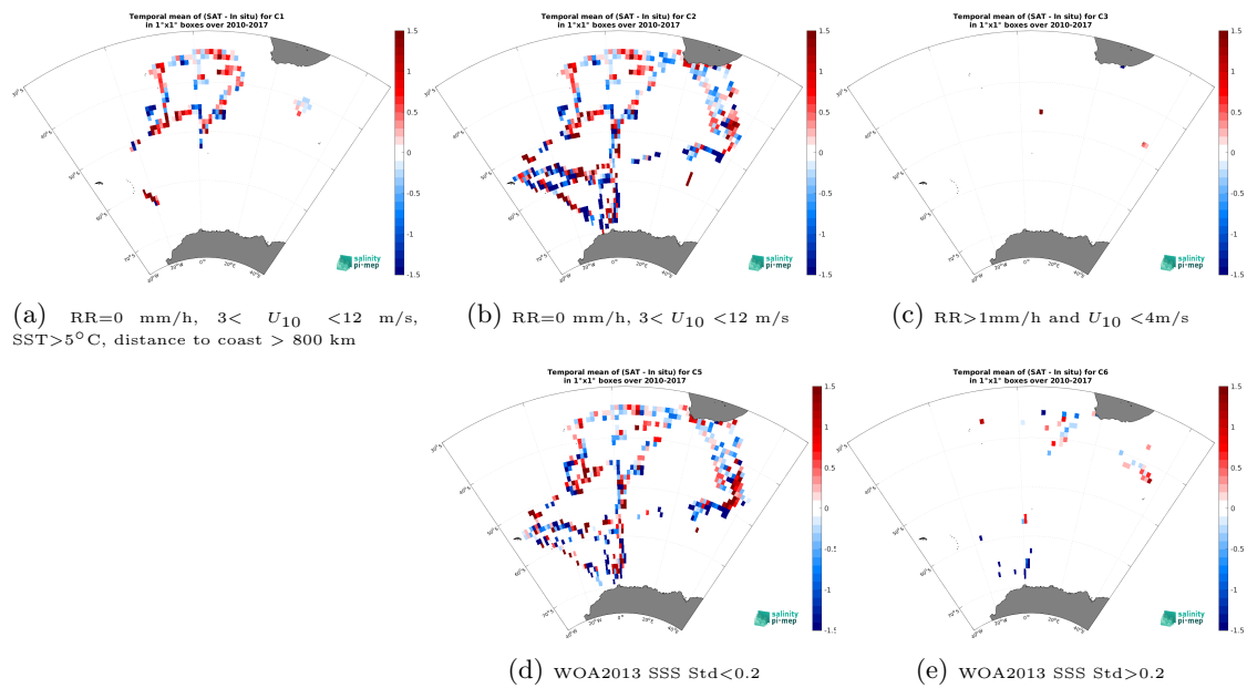
Figure 14: Temporal mean gridded over spatial boxes of size 1^\circ \times 1^\circ of \Delta SSS (SMOS SSS L2 v700 (ESA) - TSG (NCEI-0170743)) for 5 different subdatasets corresponding to:RR=0 mm/h, 3 < U_{10} < 12 m/s, SST >5^\circ\text{C} , distance to coast > 800 km (a), RR=0 mm/h, 3 < U_{10} < 12 m/s (b), RR >1 mm/h and U_{10} < 4 m/s (c), WOA2013 SSS Std <0.2 (d), WOA2013 SSS Std >0.2 (e).
