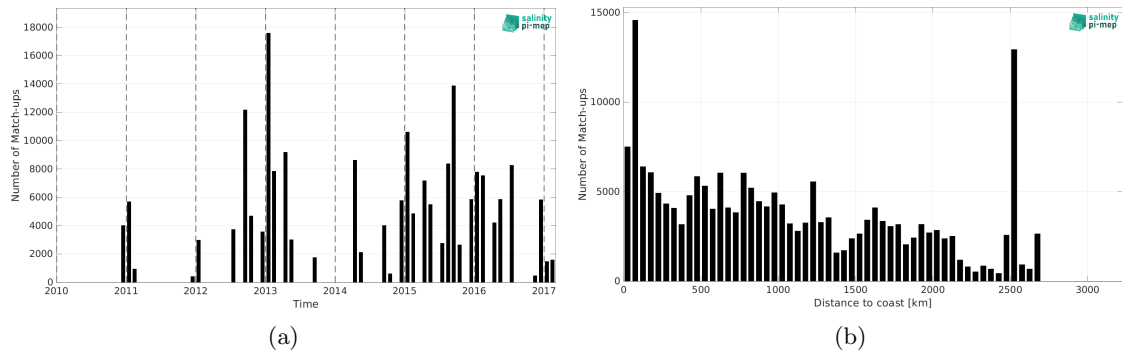
Figure 1: Number of match-ups between TSG (NCEI-0170743) and SMOS SSS L2 v700 (ESA) SSS as a function of time (a) and as function of the distance to coast (b) over the Global Ocean Pi-MEP region and for the full satellite product period.
