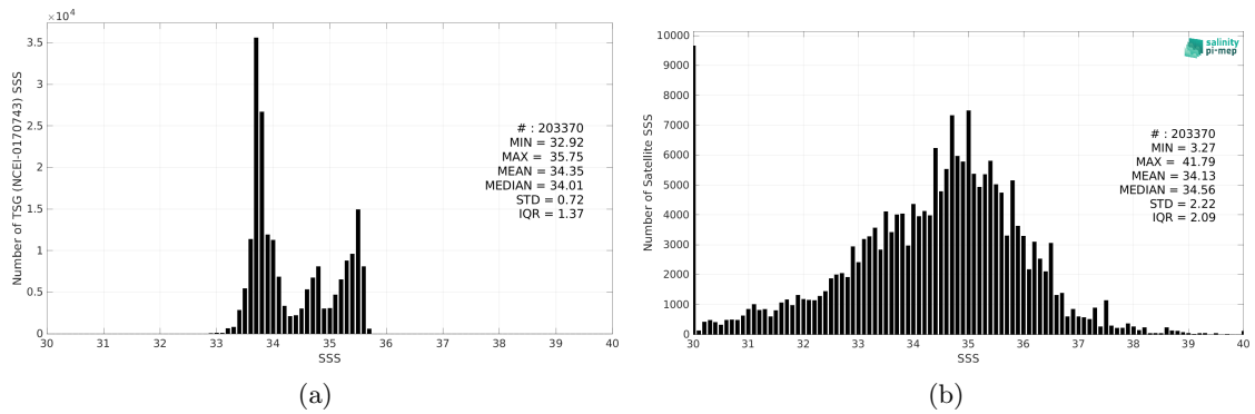
Figure 2: Histograms of SSS from TSG (NCEI-0170743) (a) and SMOS SSS L2 v700 (ESA) (b) considering all match-up pairs per bins of 0.1 over the Global Ocean Pi-MEP region and for the full satellite product period.
