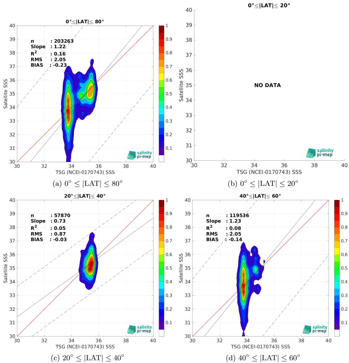
Figure 9: Contour maps of the concentration of SMOS SSS L2 v700 (ESA) SSS (y-axis) versus TSG (NCEI-0170743) SSS (x-axis) at match-up pairs for different latitude bands. For each plot, the red line shows x=y . The black thin and dashed lines indicate a linear fit through the data cloud and the \pm 95\% confidence levels, respectively. The number match-up pairs n , the slope and R^2 coefficient of the linear fit, the root mean square (RMS) and the mean bias between satellite and in situ data are indicated for each latitude band in each plots.
