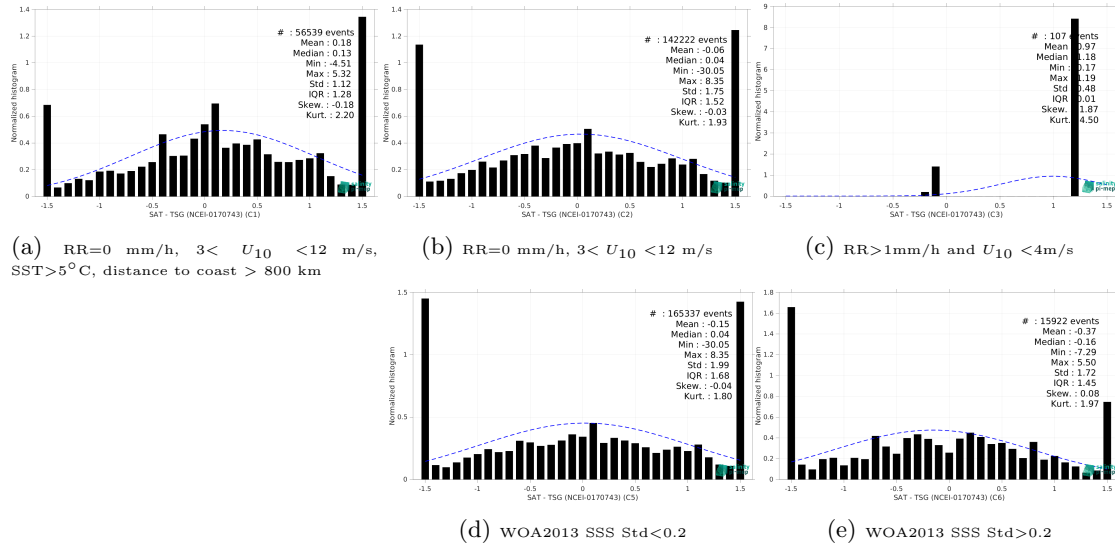
Figure 13: Normalized histogram of \Delta SSS (SMOS SSS L2 v700 (ESA) - TSG (NCEI-0170743)) for 5 different subdatasets corresponding to: RR=0 mm/h, 3 < U_{10} < 12 m/s, SST > 5°C, distance to coast > 800 km (a), RR=0 mm/h, 3 < U_{10} < 12 m/s (b), RR > 1mm/h and U_{10} < 4 m/s (c), WOA2013 SSS Std < 0.2 (d), WOA2013 SSS Std > 0.2 (e).
