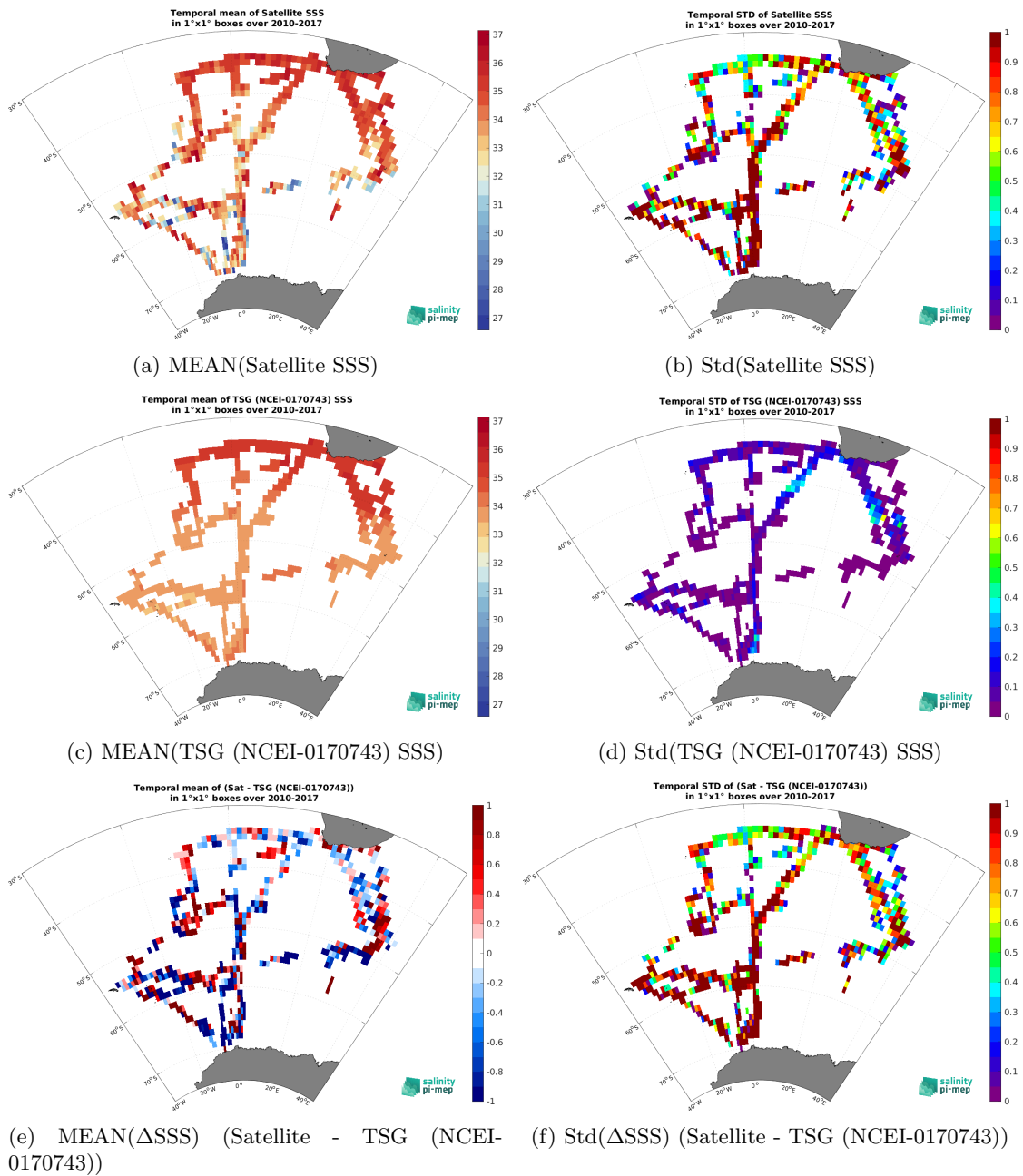
Figure 6: Temporal mean (left) and Std (right) of SSS from SMOS SSS L2 v700 (ESA) (top), TSG (NCEI-0170743) (middle), and of \Delta SSS (Satellite - TSG (NCEI-0170743)). Only match-up pairs are used to generate these maps.
