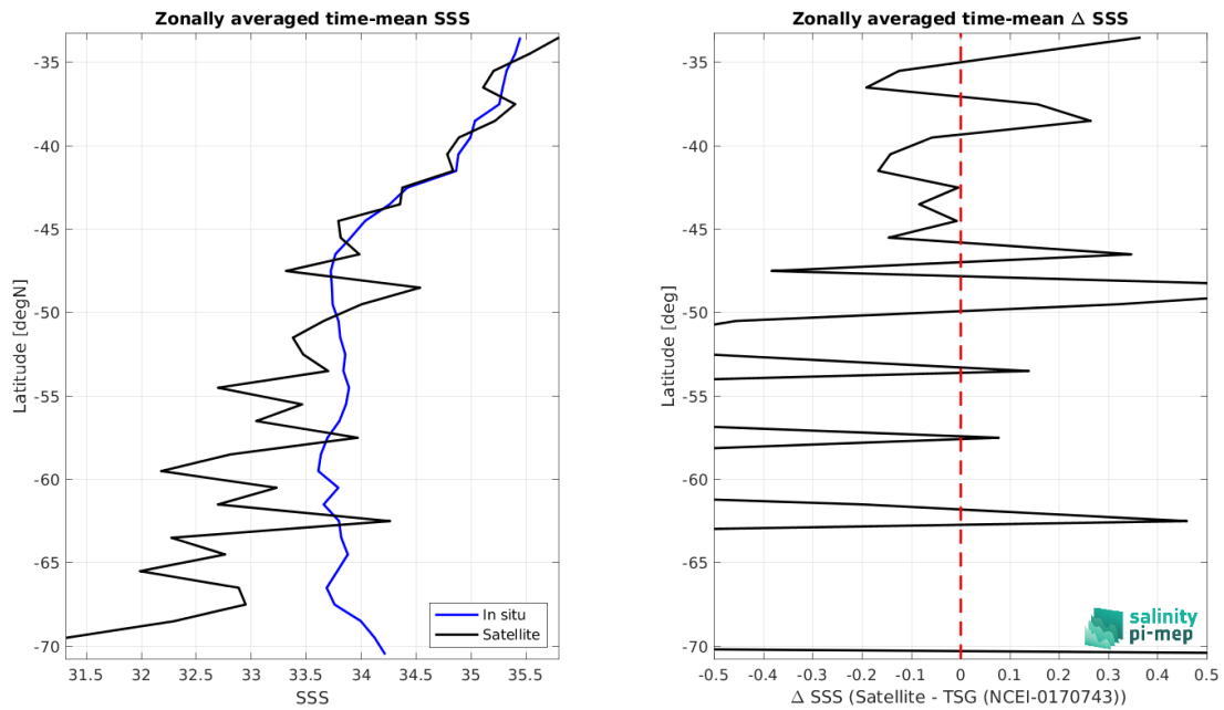
Figure 8: Left panel: Zonal mean SSS from SMOS SSS L2 v700 (ESA) satellite product (black) and from TSG (NCEI-0170743) (blue). Right panel: Zonal mean of \Delta SSS (Satellite - TSG (NCEI-0170743)) for all the collected Pi-MEP match-up pairs estimated over the full satellite product period.
