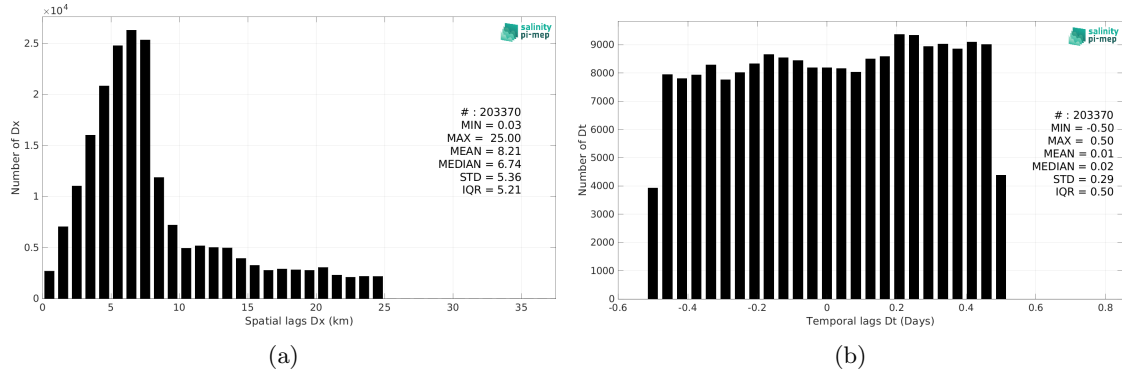
Figure 5: Histograms of the spatial (a) and temporal (b) lags between the location/time of the TSG (NCEI-0170743) measurement and the date of the corresponding SMOS SSS L2 v700 (ESA) SSS pixel.
