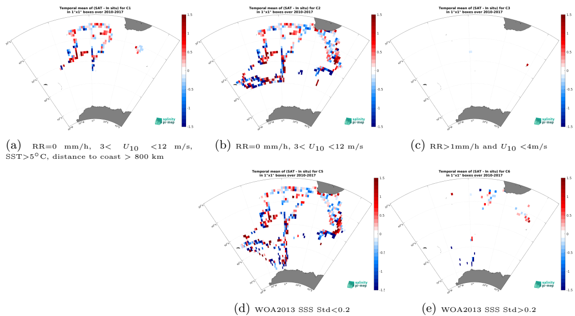
Figure 12: Temporal mean gridded over spatial boxes of size 1^\circ \times 1^\circ of \Delta SSS (SMOS SSS L2 v700 (ESA) - TSG (NCEI-0170743)) for 5 different subdatasets corresponding to:RR=0 mm/h, 3 < U_{10} < 12 m/s, SST >5^\circ C, distance to coast > 800 km (a), RR=0 mm/h, 3 < U_{10} < 12 m/s (b), RR >1 mm/h and U_{10} < 4 m/s (c), WOA2013 SSS Std <0.2 (d), WOA2013 SSS Std >0.2 (e).
