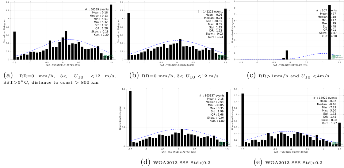
Figure 13: Normalized histogram of \Delta\text{SSS} (SMOS SSS L2 v700 (ESA) - TSG (NCEI-0170743)) for 5 different subdatasets corresponding to: RR=0 mm/h, 3 < U_{10} < 12 m/s, SST > 5^\circ\text{C} , distance to coast > 800 km (a), RR=0 mm/h, 3 < U_{10} < 12 m/s (b), RR > 1\text{mm/h} and U_{10} < 4\text{m/s} (c), WOA2013 SSS Std < 0.2 (d), WOA2013 SSS Std > 0.2 (e).
