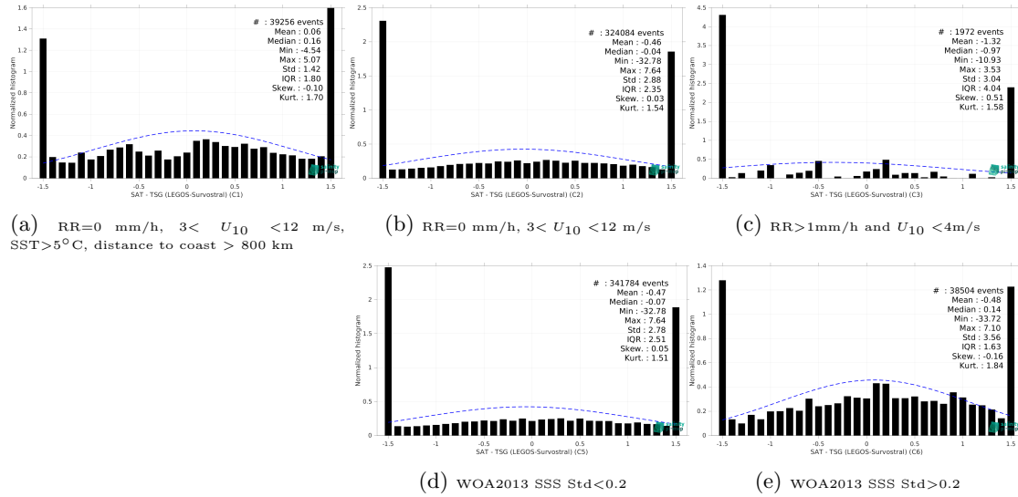
Figure 15: Normalized histogram of \Delta SSS (SMOS SSS L2 v700 (ESA) - TSG (LEGOS-Survostral)) for 5 different subdatasets corresponding to: RR=0 mm/h, 3 < U_{10} < 12 m/s, SST>5°C, distance to coast > 800 km (a), RR=0 mm/h, 3 < U_{10} < 12 m/s (b), RR>1mm/h and U_{10} < 4 m/s (c), WOA2013 SSS Std<0.2 (d), WOA2013 SSS Std>0.2 (e).
