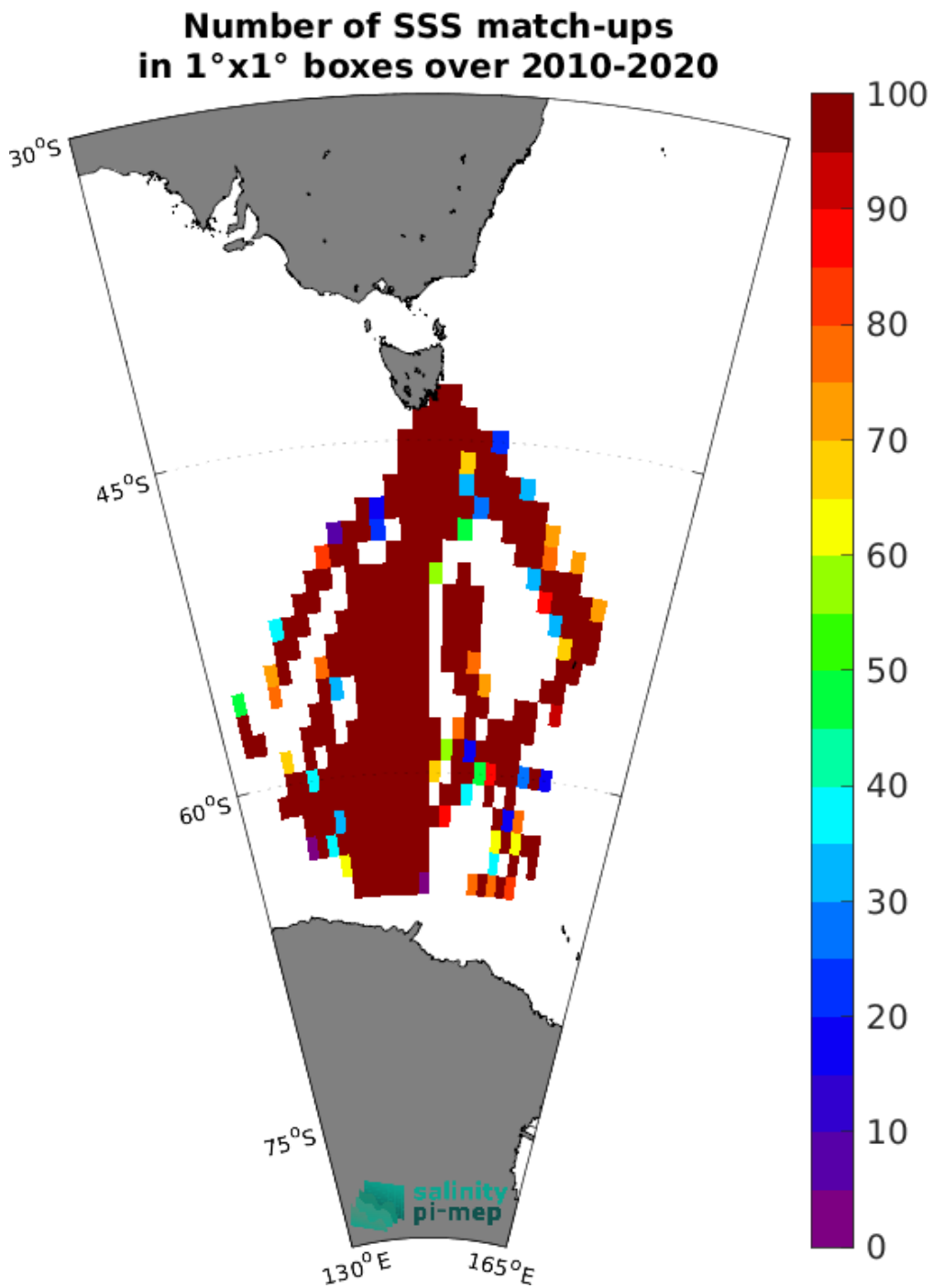
Figure 5: Number of SSS match-ups between TSG (LEGOS-Survostral) SSS and the SMOS SSS L2 v700 (ESA) SSS product for the Global Ocean Pi-MEP region over 1°x1° boxes and for the full satellite product period.
