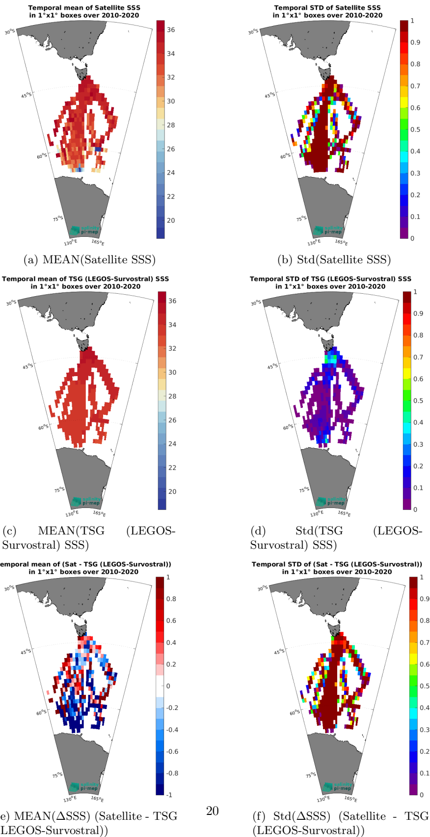
Figure 7: Temporal mean (left) and Std (right) of SSS from SMOS SSS L2 v700 (ESA) (top), TSG (LEGOS-Survostral) (middle), and of \Delta SSS (Satellite - TSG (LEGOS-Survostral)). Only match-up pairs are used to generate these maps.
