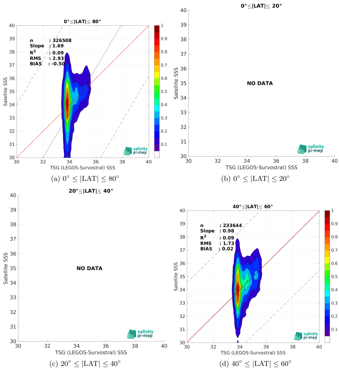
Figure 10: Contour maps of the concentration of SMOS SSS L2 v700 (ESA) SSS (y-axis) versus TSG (LEGOS-Survostral) SSS (x-axis) at match-up pairs for different latitude bands. For each plot, the red line shows x=y . The black thin and dashed lines indicate a linear fit through the data cloud and the \pm 95\% confidence levels, respectively. The number match-up pairs n , the slope and R^2 coefficient of the linear fit, the root mean square (RMS) and the mean bias between satellite and in situ data are indicated for each latitude band in each plots.
