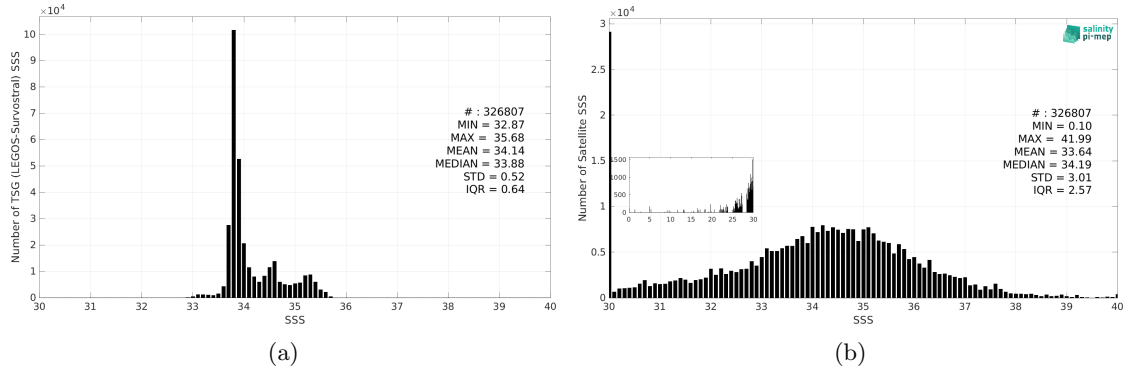
Figure 3: Histograms of SSS from TSG (LEGOS-Survostral) (a) and SMOS SSS L2 v700 (ESA) (b) considering all match-up pairs per bins of 0.1 over the Global Ocean Pi-MEP region and for the full satellite product period.
