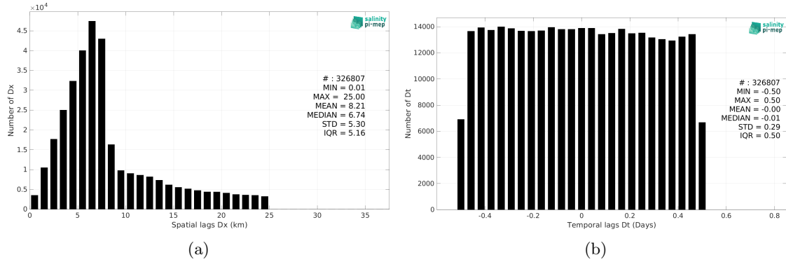
Figure 6: Histograms of the spatial (a) and temporal (b) lags between the location/time of the TSG (LEGOS-Survostral) measurement and the date of the corresponding SMOS SSS L2 v700 (ESA) SSS pixel.
