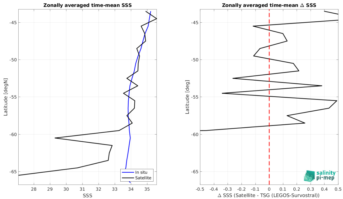
Figure 9: Left panel: Zonal mean SSS from SMOS SSS L2 v700 (ESA) satellite product (black) and from TSG (LEGOS-Survostral) (blue). Right panel: Zonal mean of \Delta SSS (Satellite - TSG (LEGOS-Survostral)) for all the collected Pi-MEP match-up pairs estimated over the full satellite product period.
