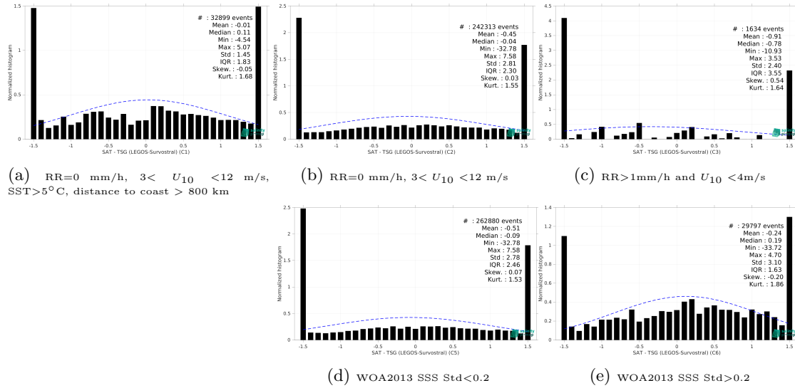
Figure 15: Normalized histogram of \Delta SSS (SMOS SSS L2 v700 (ESA) - TSG (LEGOS-Survostral)) for 5 different subdatasets corresponding to: RR=0 mm/h, 3 < U_{10} < 12 m/s, SST > 5°C, distance to coast > 800 km (a), RR=0 mm/h, 3 < U_{10} < 12 m/s (b), RR > 1mm/h and U_{10} < 4 m/s (c), WOA2013 SSS Std < 0.2 (d), WOA2013 SSS Std > 0.2 (e).
