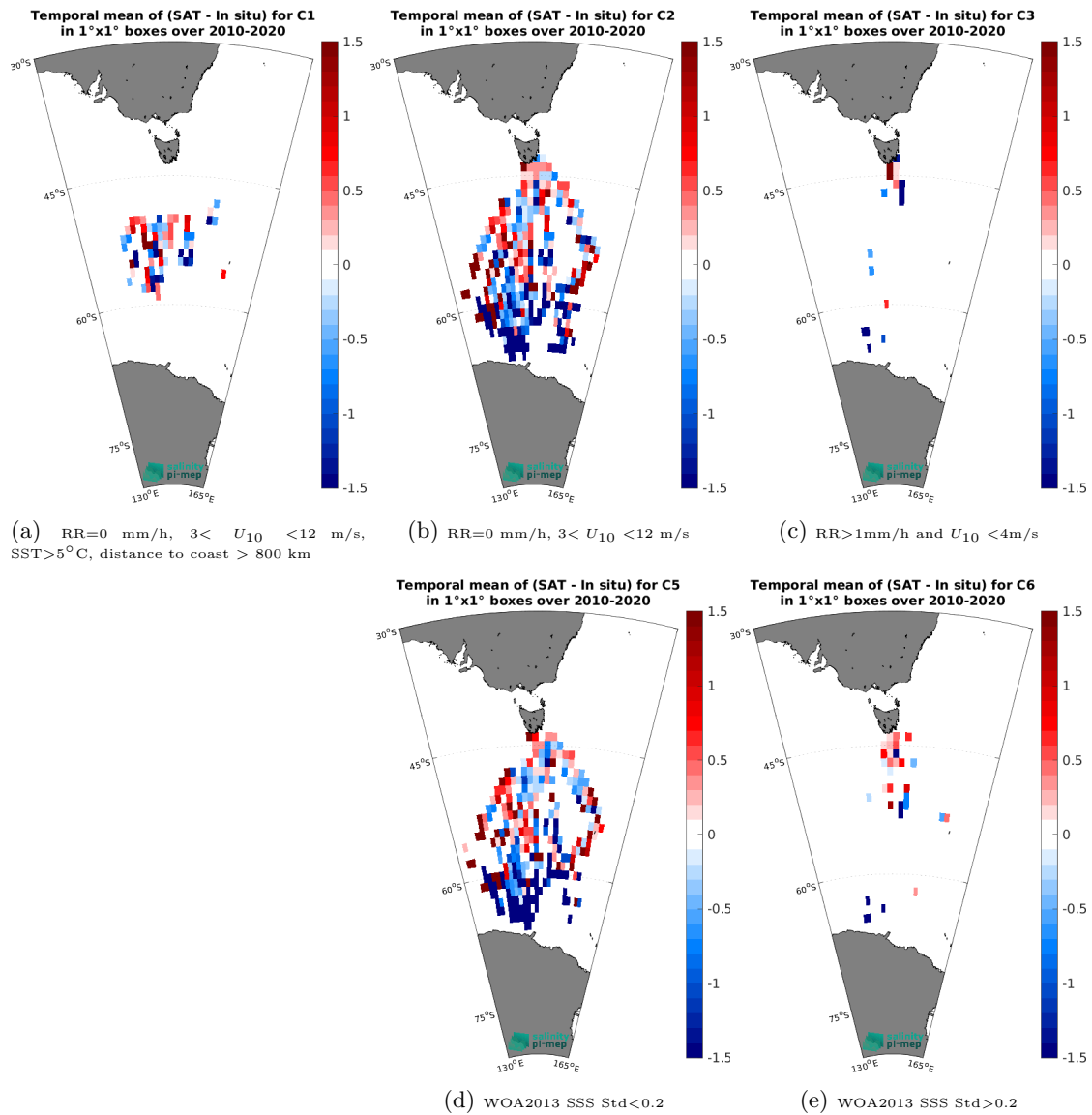
Figure 14: Temporal mean gridded over spatial boxes of size 1^\circ \times 1^\circ of \Delta SSS (SMOS SSS L2 v700 (ESA) - TSG (LEGOS-Survostral)) for 5 different subdatasets corresponding to:RR=0 mm/h, 3 < U_{10} < 12 m/s, SST>5°C, distance to coast > 800 km (a), RR=0 mm/h, 3 < U_{10} < 12 m/s (b), RR>1mm/h and U_{10} < 4 m/s (c), WOA2013 SSS Std<0.2 (d), WOA2013 SSS Std>0.2 (e).
