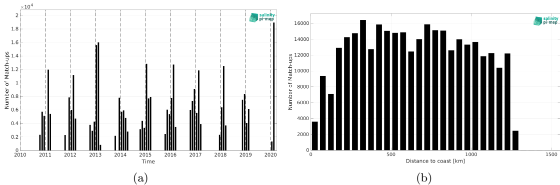
Figure 2: Number of match-ups between TSG (LEGOS-Survostral) and SMOS SSS L2 v700 (ESA) SSS as a function of time (a) and as function of the distance to coast (b) over the Global Ocean Pi-MEP region and for the full satellite product period.
