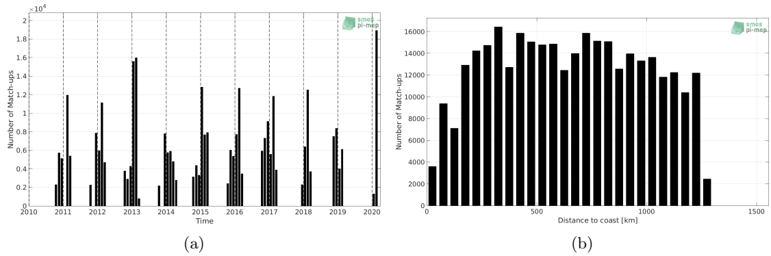
Figure 1: Number of match-ups between TSG (LEGOS-Survostral) and SMOS SSS L2 v700 (ESA) SSS as a function of time (a) and as function of the distance to coast (b) over the Global Ocean Pi-MEP region and for the full satellite product period.
