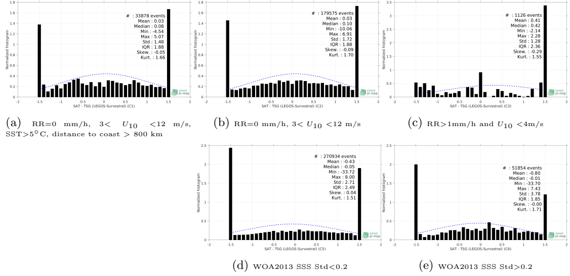
Figure 13: Normalized histogram of \Delta SSS (SMOS SSS L2 v700 (ESA) - TSG (LEGOS-Survostral)) for 5 different subdatasets corresponding to: RR=0 mm/h, 3 < U_{10} < 12 m/s, SST>5°C, distance to coast > 800 km (a), RR=0 mm/h, 3 < U_{10} < 12 m/s (b), RR>1mm/h and U_{10} < 4 m/s (c), WOA2013 SSS Std<0.2 (d), WOA2013 SSS Std>0.2 (e).
