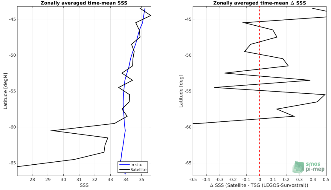
Figure 8: Left panel: Zonal mean SSS from SMOS SSS L2 v700 (ESA) satellite product (black) and from TSG (LEGOS-Survostral) (blue). Right panel: Zonal mean of \Delta SSS (Satellite - TSG (LEGOS-Survostral)) for all the collected Pi-MEP match-up pairs estimated over the full satellite product period.
