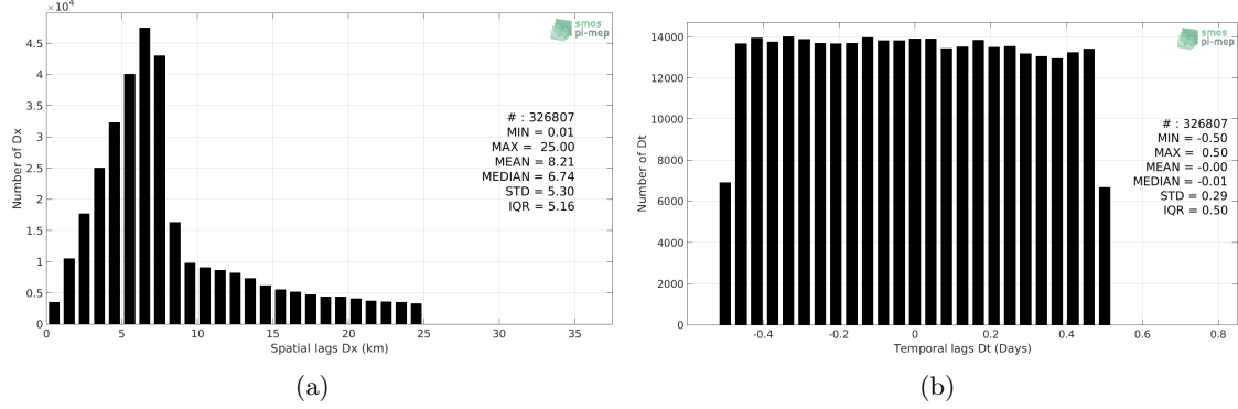
Figure 5: Histograms of the spatial (a) and temporal (b) lags between the location/time of the TSG (LEGOS-Survostral) measurement and the date of the corresponding SMOS SSS L2 v700 (ESA) SSS pixel.
