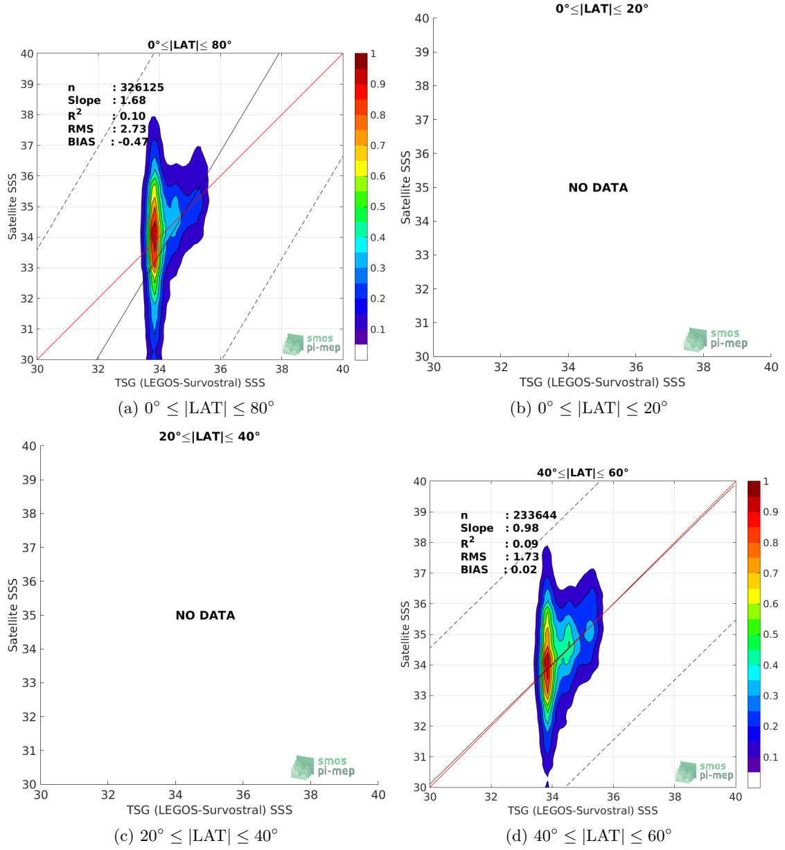
Figure 9: Contour maps of the concentration of SMOS SSS L2 v700 (ESA) SSS (y-axis) versus TSG (LEGOS-Survostral) SSS (x-axis) at match-up pairs for different latitude bands. For each plot, the red line shows x=y . The black thin and dashed lines indicate a linear fit through the data cloud and the \pm 95\% confidence levels, respectively. The number match-up pairs n , the slope and R^2 coefficient of the linear fit, the root mean square (RMS) and the mean bias between satellite and in situ data are indicated for each latitude band in each plots.
