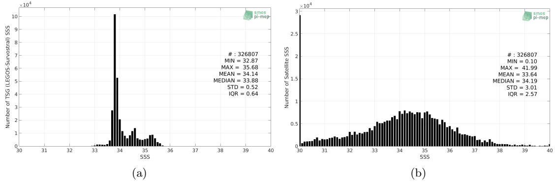
Figure 2: Histograms of SSS from TSG (LEGOS-Survostral) (a) and SMOS SSS L2 v700 (ESA) (b) considering all match-up pairs per bins of 0.1 over the Global Ocean Pi-MEP region and for the full satellite product period.
