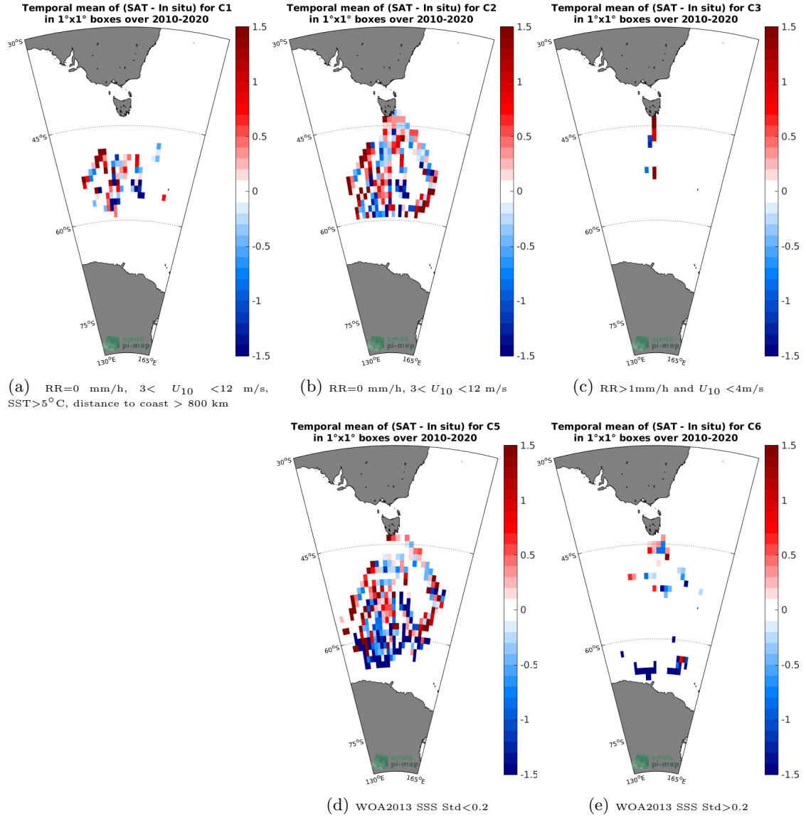
Figure 12: Temporal mean gridded over spatial boxes of size 1°x1° of \Delta\text{SSS} (SMOS SSS L2 v700 (ESA) - TSG (LEGOS-Survostral)) for 5 different subdatasets corresponding to: RR=0 mm/h, 3 < U_{10} < 12 m/s, SST > 5^\circ\text{C} , distance to coast > 800 km (a), RR=0 mm/h, 3 < U_{10} < 12 m/s (b), RR > 1 mm/h and U_{10} < 4 m/s (c), WOA2013 SSS Std < 0.2 (d), WOA2013 SSS Std > 0.2 (e).
