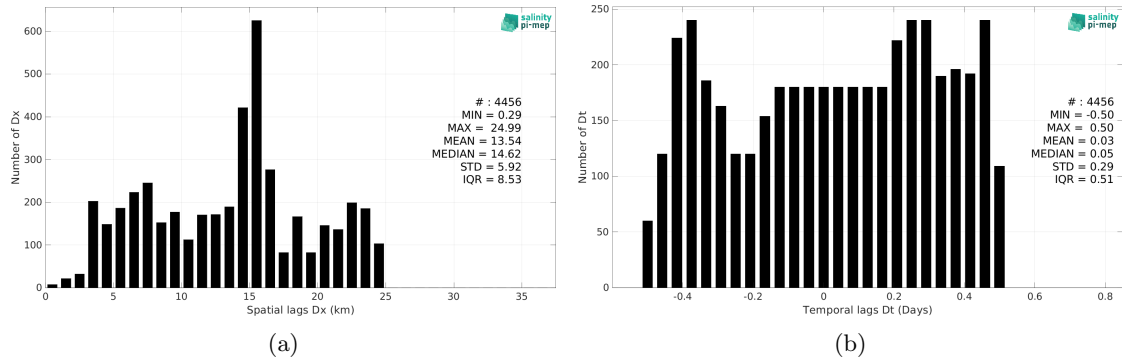
Figure 6: Histograms of the spatial (a) and temporal (b) lags between the location/time of the TSG (LEGOS-Surv-Adel) measurement and the date of the corresponding SMOS SSS L2 v700 (ESA) SSS pixel.
