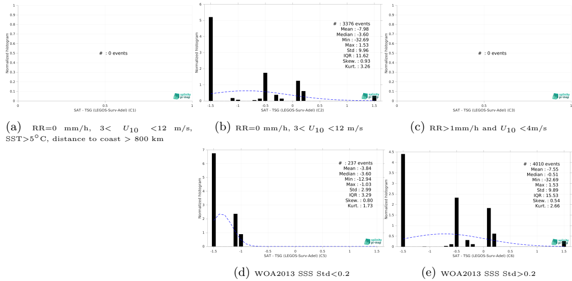
Figure 15: Normalized histogram of \Delta SSS (SMOS SSS L2 v700 (ESA) - TSG (LEGOS-Surv-Adel)) for 5 different subdatasets corresponding to: RR=0 mm/h, 3 < U_{10} < 12 m/s, SST > 5°C, distance to coast > 800 km (a), RR=0 mm/h, 3 < U_{10} < 12 m/s (b), RR > 1mm/h and U_{10} < 4 m/s (c), WOA2013 SSS Std < 0.2 (d), WOA2013 SSS Std > 0.2 (e).
