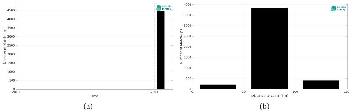
Figure 2: Number of match-ups between TSG (LEGOS-Surv-Adel) and SMOS SSS L2 v700 (ESA) SSS as a function of time (a) and as function of the distance to coast (b) over the Global Ocean Pi-MEP region and for the full satellite product period.
