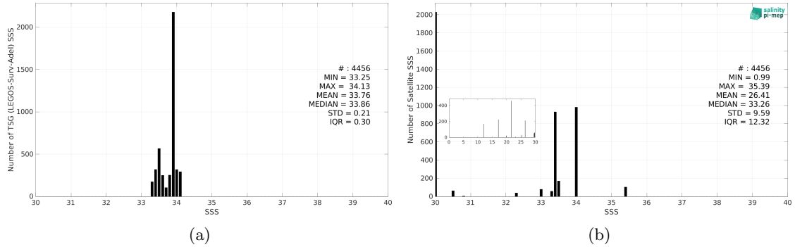
Figure 3: Histograms of SSS from TSG (LEGOS-Surv-Adel) (a) and SMOS SSS L2 v700 (ESA) (b) considering all match-up pairs per bins of 0.1 over the Global Ocean Pi-MEP region and for the full satellite product period.
