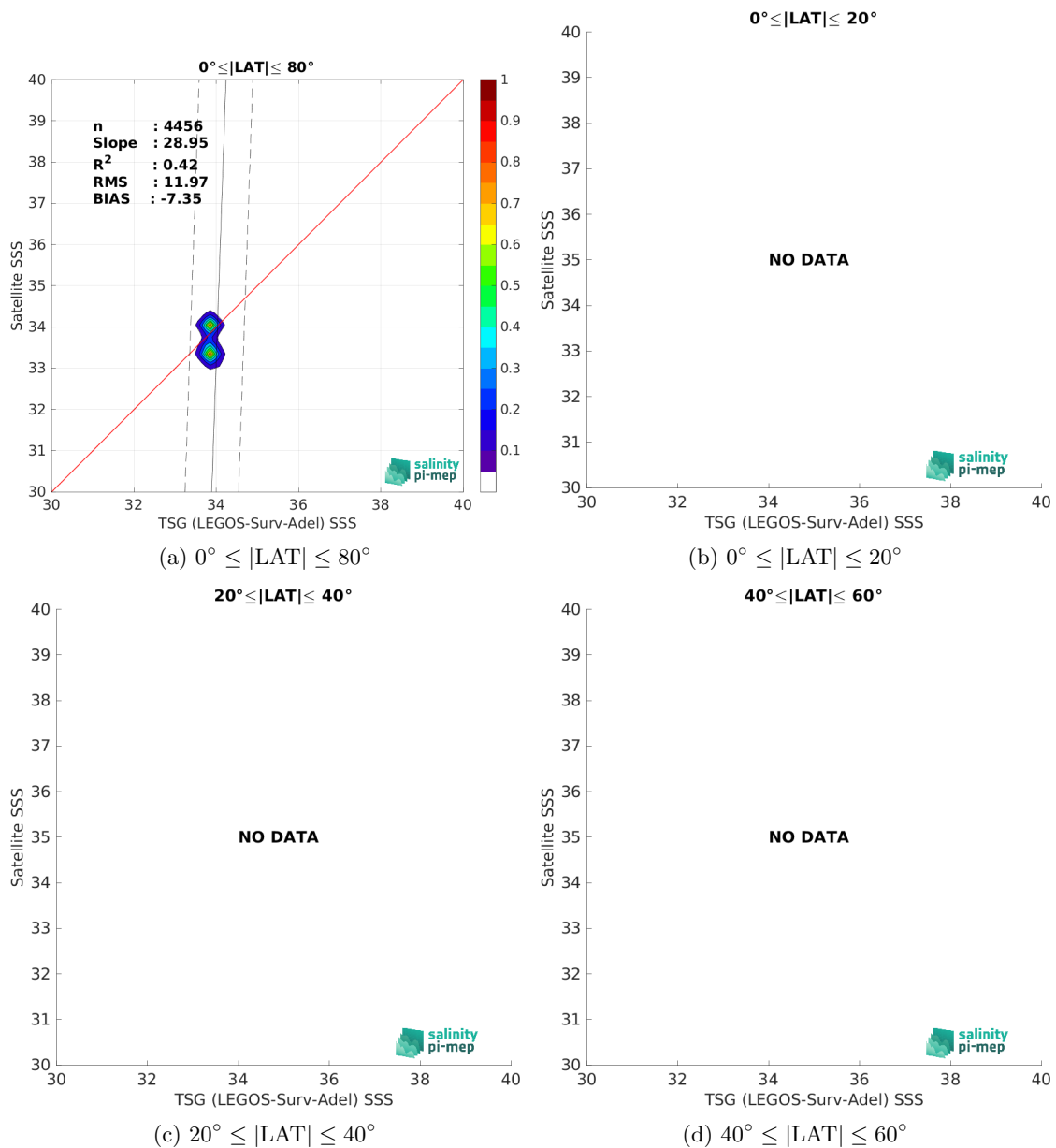
Figure 10: Contour maps of the concentration of SMOS SSS L2 v700 (ESA) SSS (y-axis) versus TSG (LEGOS-Surv-Adel) SSS (x-axis) at match-up pairs for different latitude bands. For each plot, the red line shows x=y . The black thin and dashed lines indicate a linear fit through the data cloud and the \pm 95\% confidence levels, respectively. The number match-up pairs n , the slope and R^2 coefficient of the linear fit, the root mean square (RMS) and the mean bias between satellite and in situ data are indicated for each latitude band in each plots.
