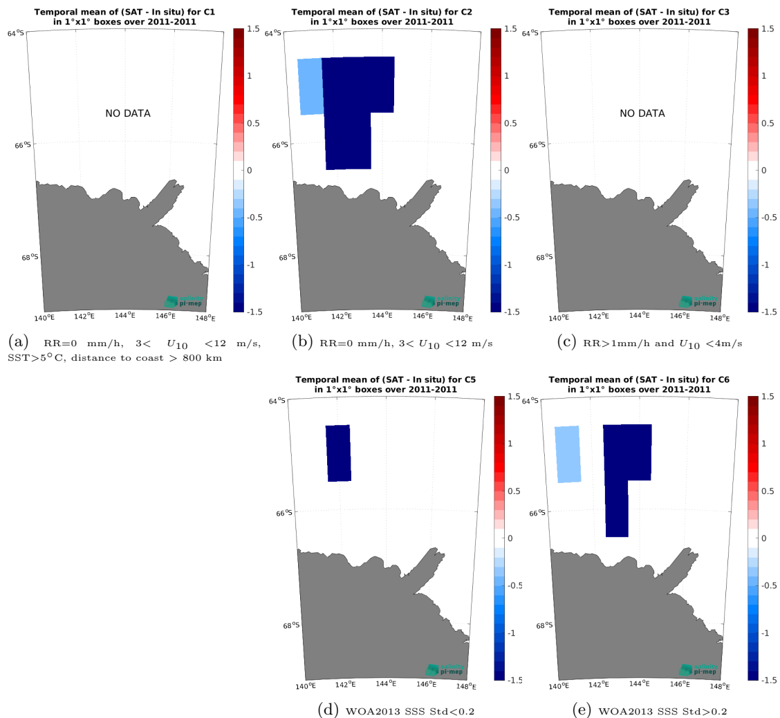
Figure 14: Temporal mean gridded over spatial boxes of size 1^\circ \times 1^\circ of \Delta\text{SSS} (SMOS SSS L2 v700 (ESA) - TSG (LEGOS-Surv-Adel)) for 5 different subdatasets corresponding to:RR=0 mm/h, 3 < U_{10} < 12 m/s, SST > 5°C, distance to coast > 800 km (a), RR=0 mm/h, 3 < U_{10} < 12 m/s (b), RR > 1mm/h and U_{10} < 4 m/s (c), WOA2013 SSS Std < 0.2 (d), WOA2013 SSS Std > 0.2 (e).
