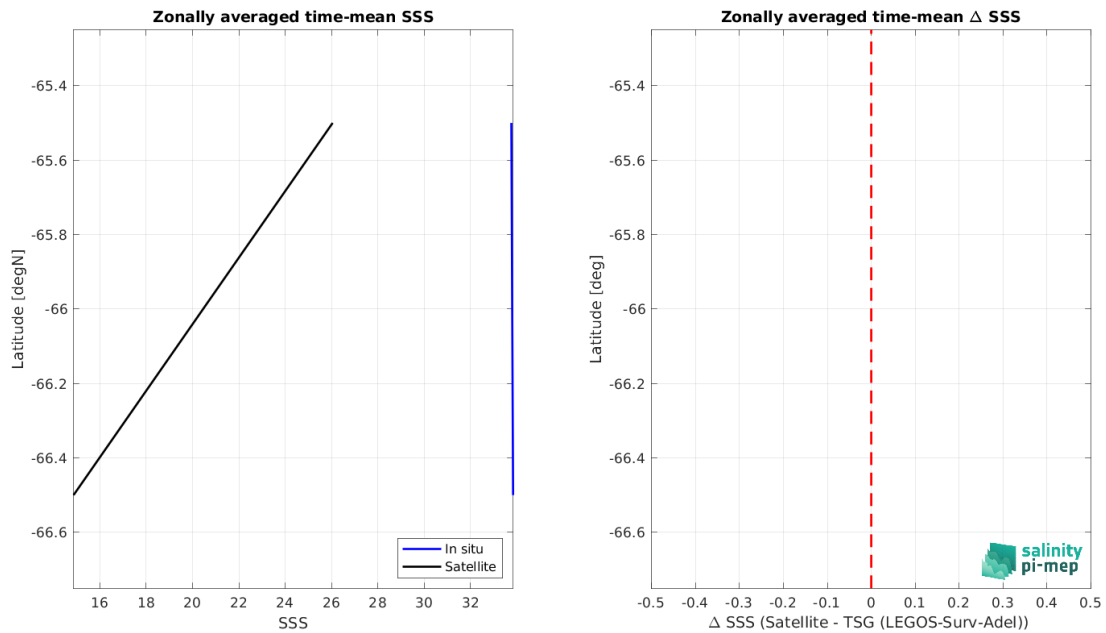
Figure 9: Left panel: Zonal mean SSS from SMOS SSS L2 v700 (ESA) satellite product (black) and from TSG (LEGOS-Surv-Adel) (blue). Right panel: Zonal mean of \Delta SSS (Satellite - TSG (LEGOS-Surv-Adel)) for all the collected Pi-MEP match-up pairs estimated over the full satellite product period.
