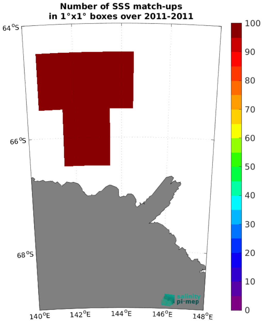
Figure 5: Number of SSS match-ups between TSG (LEGOS-Surv-Adel) SSS and the SMOS SSS L2 v700 (ESA) SSS product for the Global Ocean Pi-MEP region over 1^\circ \times 1^\circ boxes and for the full satellite product period.
