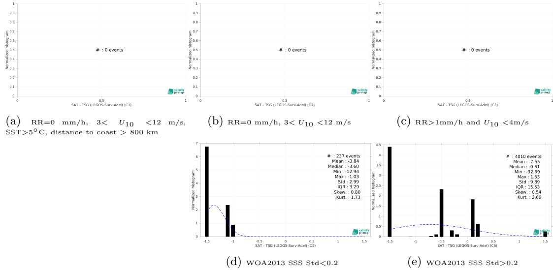
Figure 13: Normalized histogram of \Delta SSS (SMOS SSS L2 v700 (ESA) - TSG (LEGOS-Surv-Adel)) for 5 different subdatasets corresponding to: RR=0 mm/h, 3 < U_{10} < 12 m/s, SST >5^{\circ} C, distance to coast > 800 km (a), RR=0 mm/h, 3 < U_{10} < 12 m/s (b), RR >1 mm/h and U_{10} < 4 m/s (c), WOA2013 SSS Std <0.2 (d), WOA2013 SSS Std >0.2 (e).
