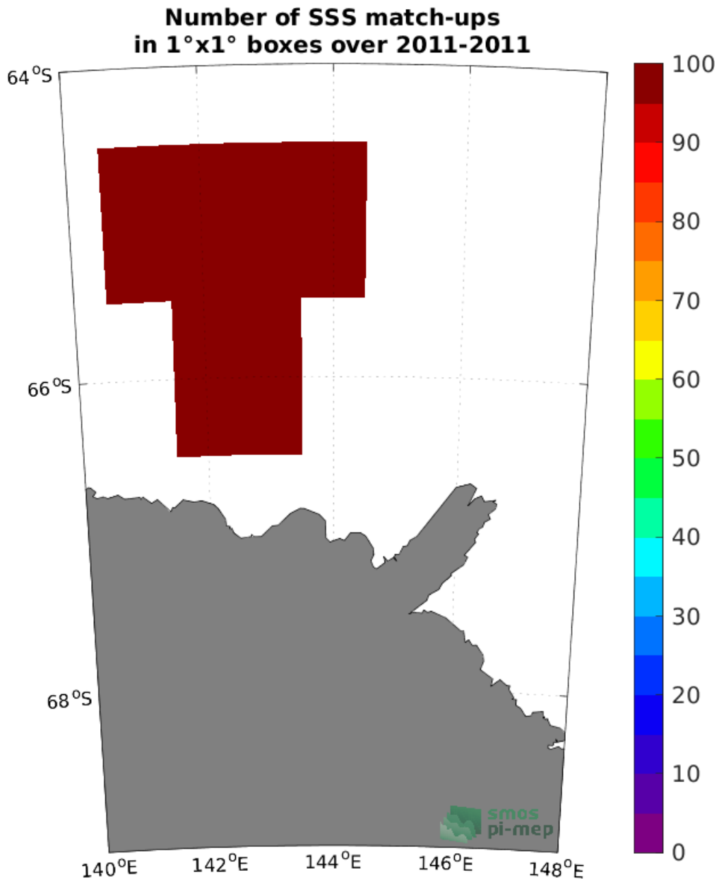
Figure 4: Number of SSS match-ups between TSG (LEGOS-Surv-Adel) SSS and the SMOS SSS L2 v700 (ESA) SSS product for the Global Ocean Pi-MEP region over 1°×1° boxes and for the full satellite product period.
