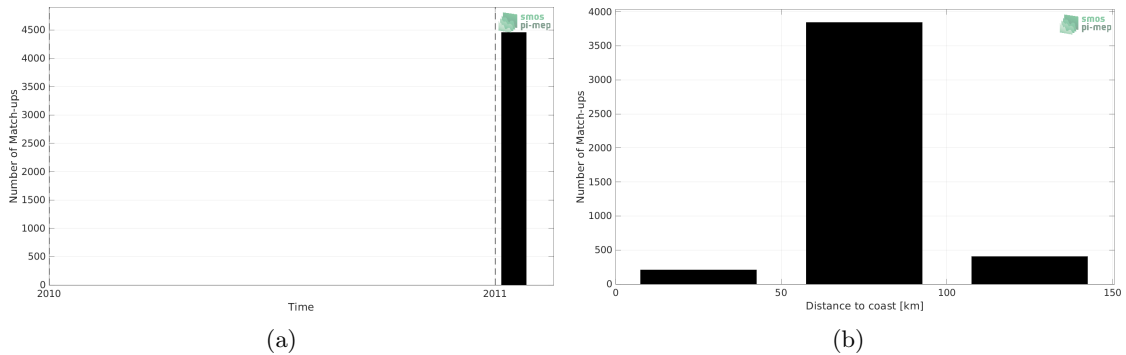
Figure 1: Number of match-ups between TSG (LEGOS-Surv-Adel) and SMOS SSS L2 v700 (ESA) SSS as a function of time (a) and as function of the distance to coast (b) over the Global Ocean Pi-MEP region and for the full satellite product period.
