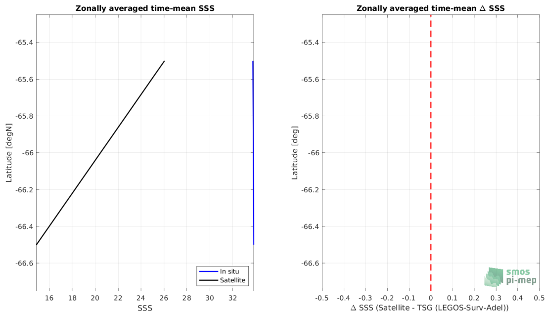
Figure 8: Left panel: Zonal mean SSS from SMOS SSS L2 v700 (ESA) satellite product (black) and from TSG (LEGOS-Surv-Adel) (blue). Right panel: Zonal mean of \Delta SSS (Satellite - TSG (LEGOS-Surv-Adel)) for all the collected Pi-MEP match-up pairs estimated over the full satellite product period.
