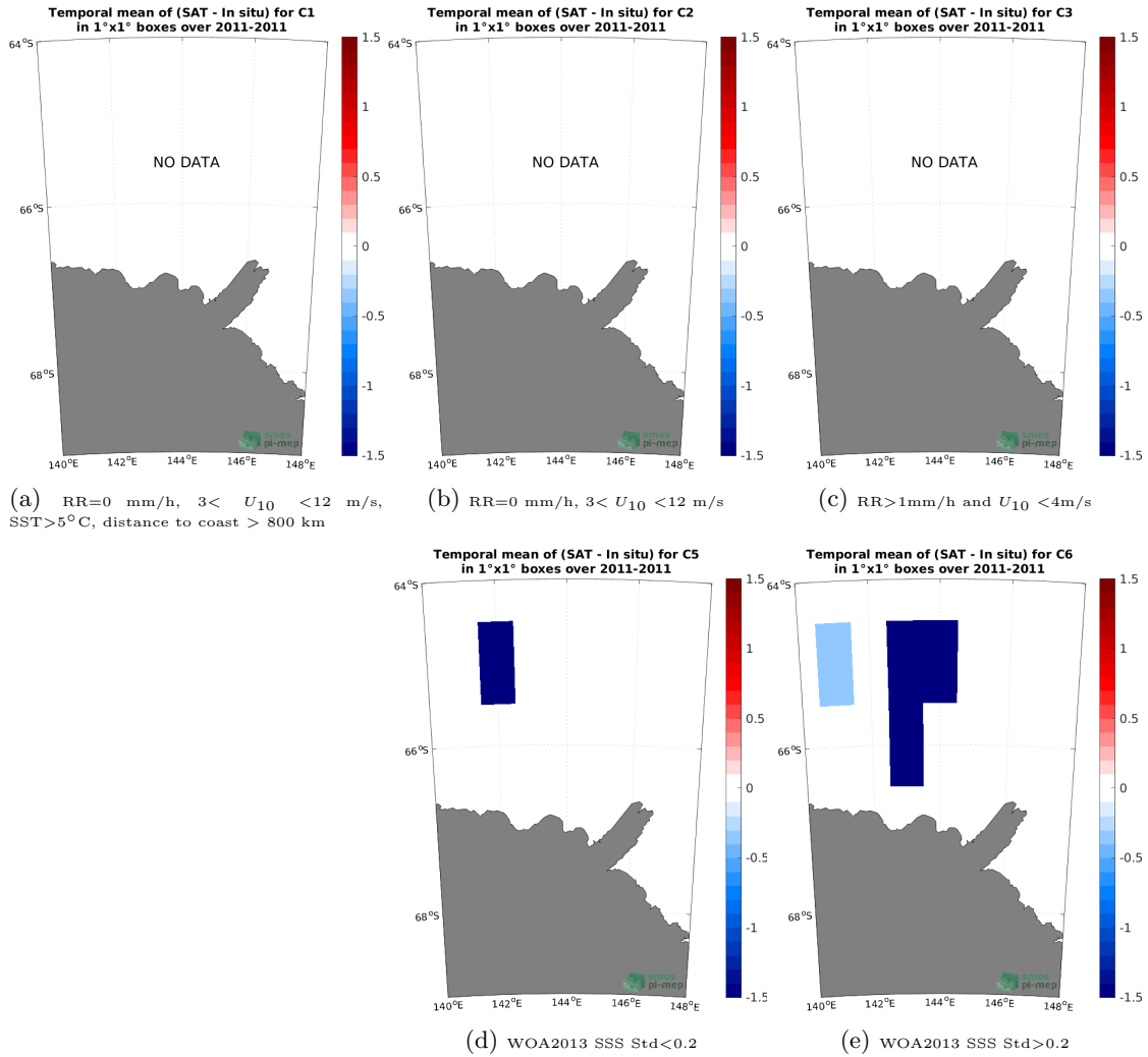
Figure 12: Temporal mean gridded over spatial boxes of size 1^\circ \times 1^\circ of \Delta SSS (SMOS SSS L2 v700 (ESA) - TSG (LEGOS-Surv-Adel)) for 5 different subdatasets corresponding to:RR=0 mm/h, 3 < U_{10} < 12 m/s, SST>5°C, distance to coast > 800 km (a), RR=0 mm/h, 3 < U_{10} < 12 m/s (b), RR>1mm/h and U_{10} < 4 m/s (c), WOA2013 SSS Std<0.2 (d), WOA2013 SSS Std>0.2 (e).
