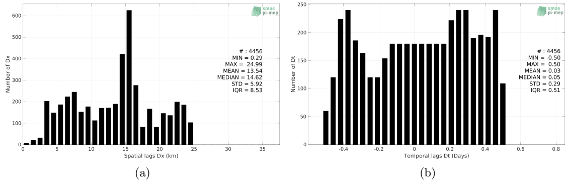
Figure 5: Histograms of the spatial (a) and temporal (b) lags between the location/time of the TSG (LEGOS-Surv-Adel) measurement and the date of the corresponding SMOS SSS L2 v700 (ESA) SSS pixel.
