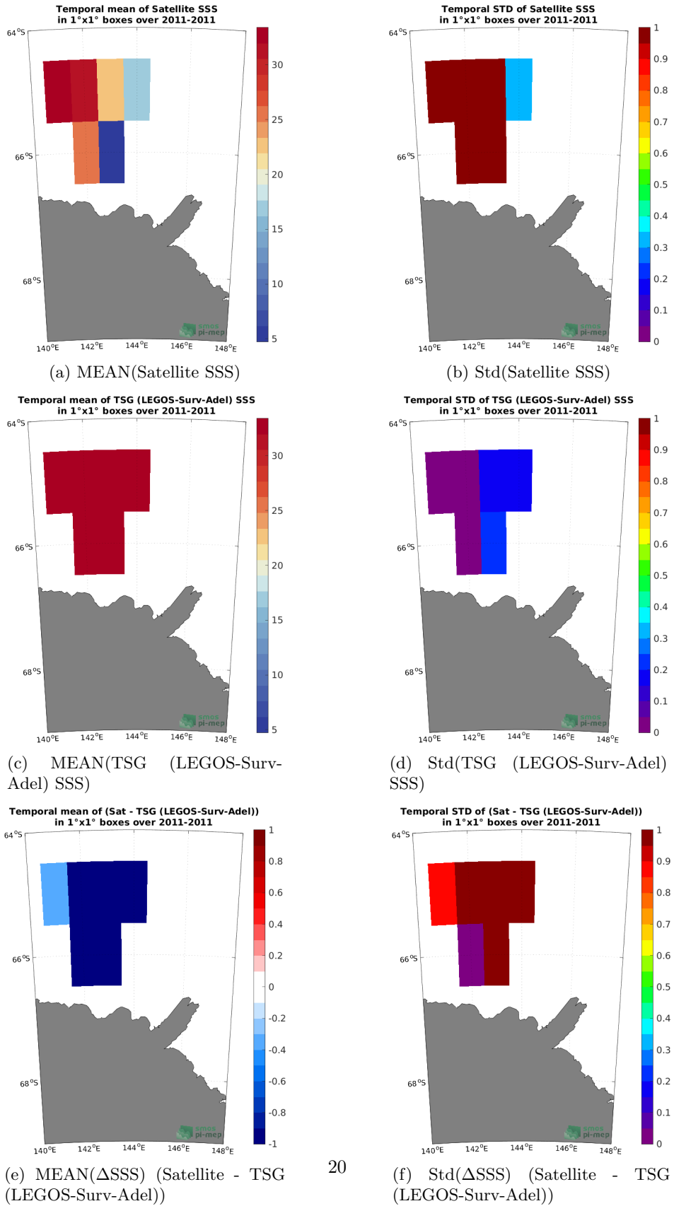
Figure 6: Temporal mean (left) and Std (right) of SSS from SMOS SSS L2 v700 (ESA) (top), TSG (LEGOS-Surv-Adel) (middle), and of \Delta SSS (Satellite - TSG (LEGOS-Surv-Adel)). Only match-up pairs are used to generate these maps.
