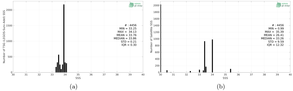
Figure 2: Histograms of SSS from TSG (LEGOS-Surv-Adel) (a) and SMOS SSS L2 v700 (ESA) (b) considering all match-up pairs per bins of 0.1 over the Global Ocean Pi-MEP region and for the full satellite product period.
