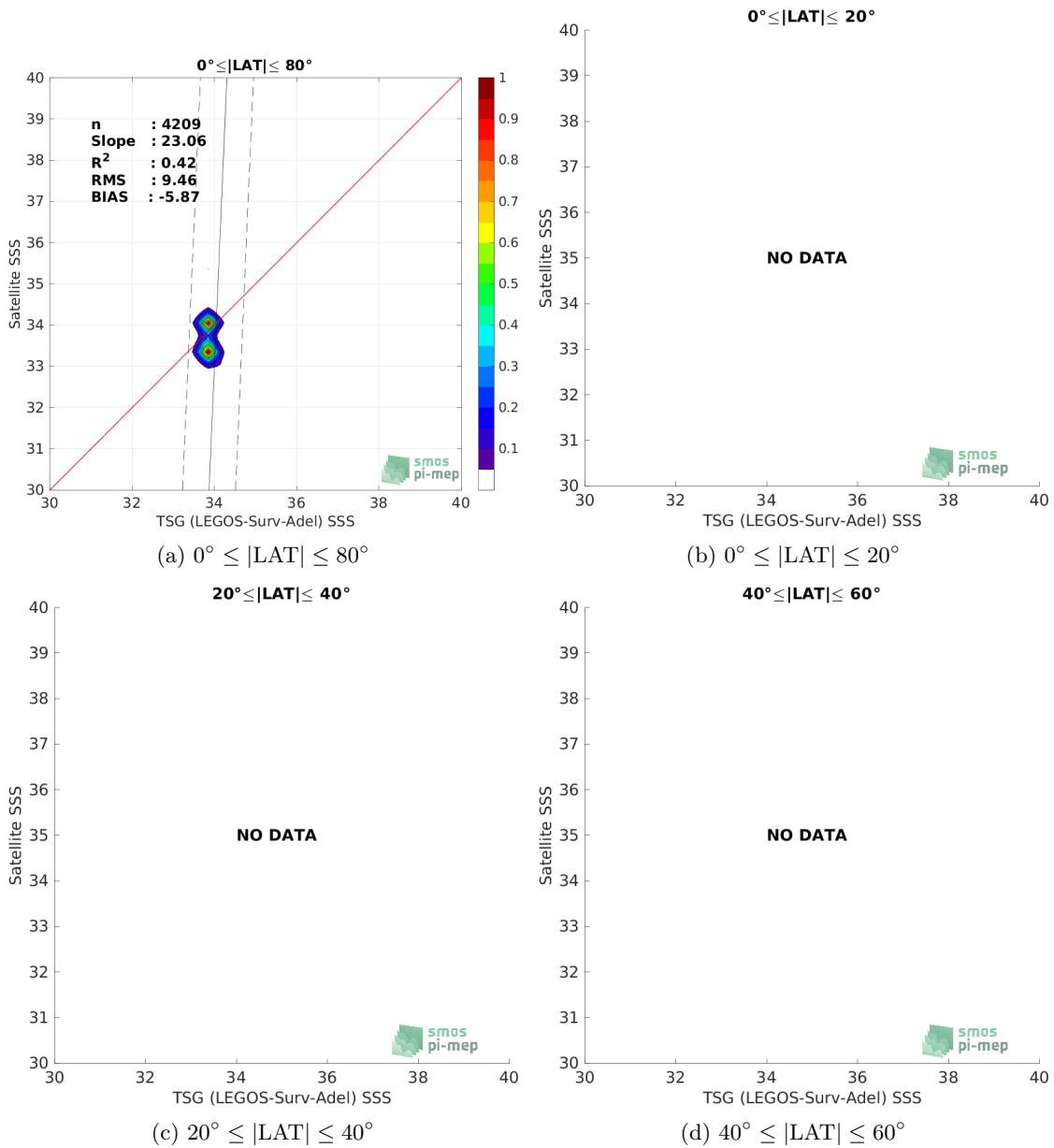
Figure 9: Contour maps of the concentration of SMOS SSS L2 v700 (ESA) SSS (y-axis) versus TSG (LEGOS-Surv-Adel) SSS (x-axis) at match-up pairs for different latitude bands. For each plot, the red line shows x=y . The black thin and dashed lines indicate a linear fit through the data cloud and the \pm 95\% confidence levels, respectively. The number match-up pairs n , the slope and R^2 coefficient of the linear fit, the root mean square (RMS) and the mean bias between satellite and in situ data are indicated for each latitude band in each plots.
