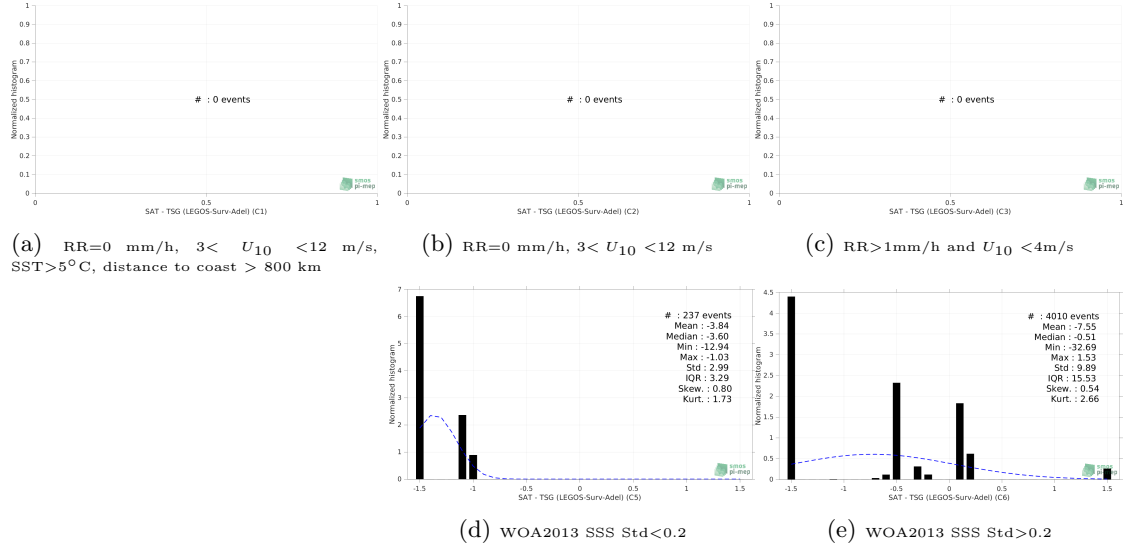
Figure 13: Normalized histogram of \Delta SSS (SMOS SSS L2 v700 (ESA) - TSG (LEGOS-Surv-Adel)) for 5 different subdatasets corresponding to: RR=0 mm/h, 3 < U_{10} < 12 m/s, SST>5°C, distance to coast > 800 km (a), RR=0 mm/h, 3 < U_{10} < 12 m/s (b), RR>1mm/h and U_{10} < 4 m/s (c), WOA2013 SSS Std<0.2 (d), WOA2013 SSS Std>0.2 (e).
